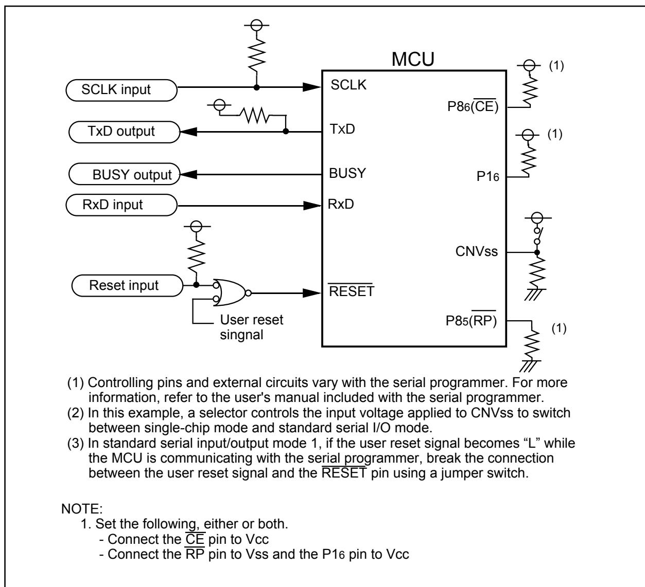
Figure 20.17 Circuit Application in Standard Serial I/O Mode 1
