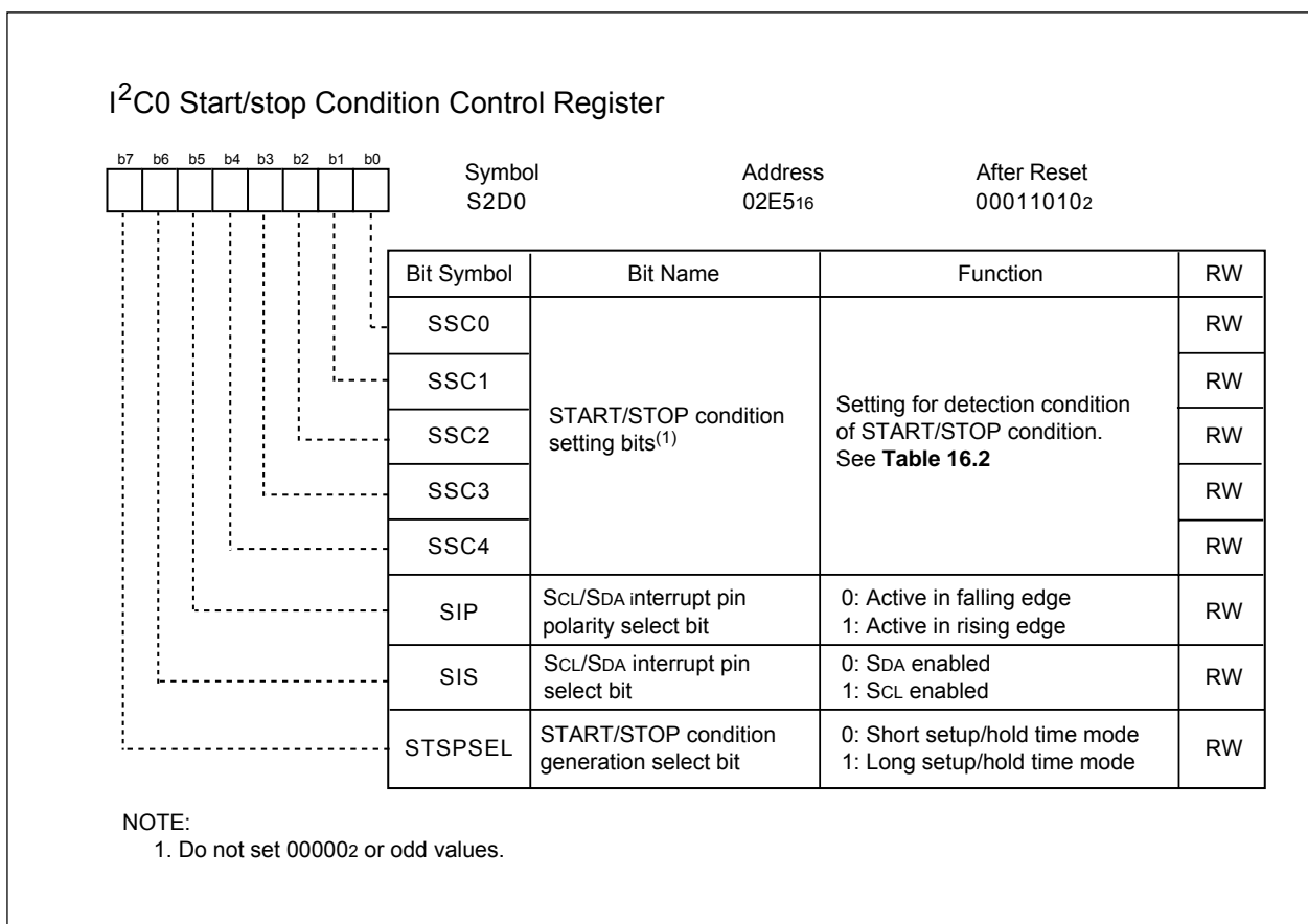
Figure 16.8 S2D0 Register
