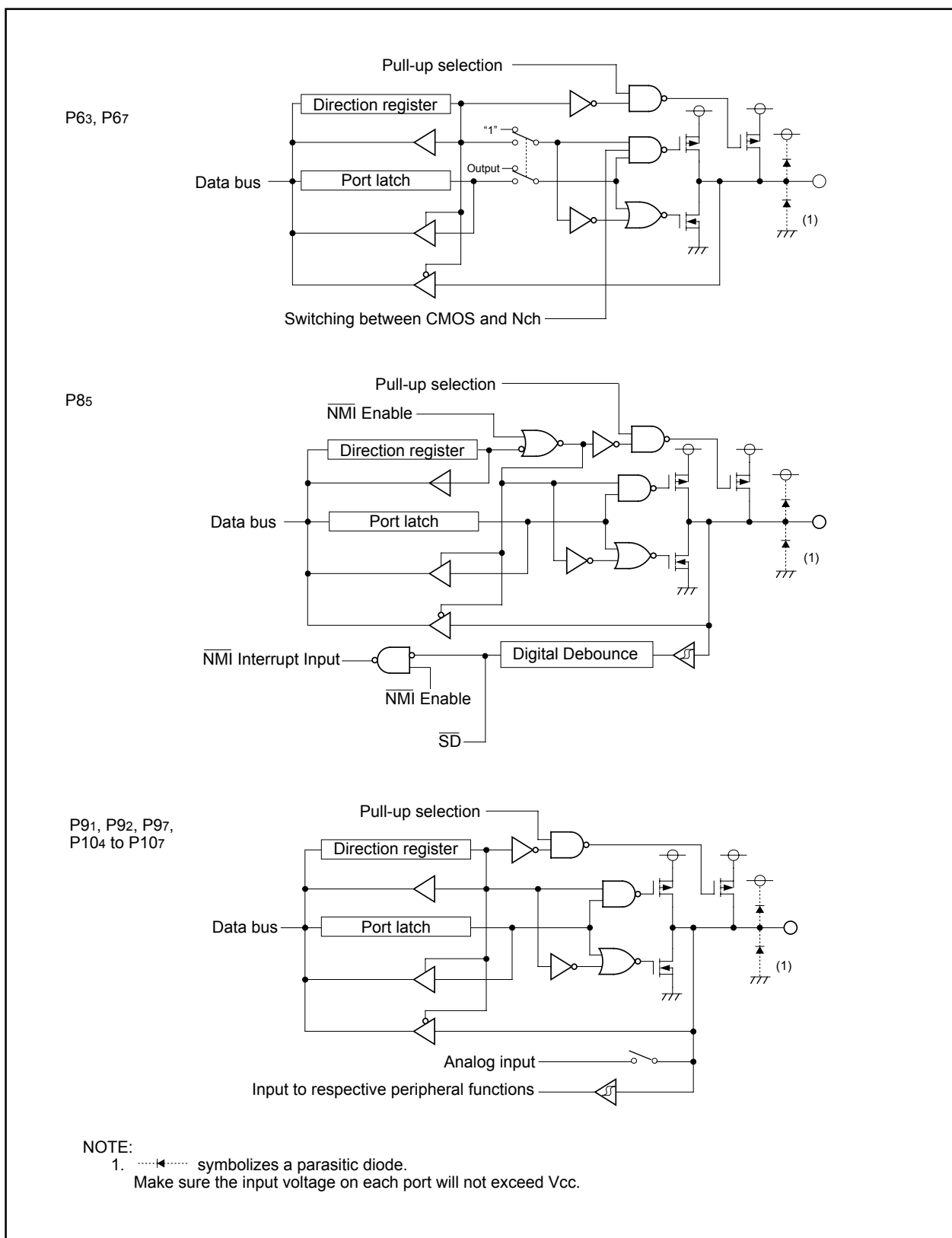
Figure 19.3 I/O Ports (3)
