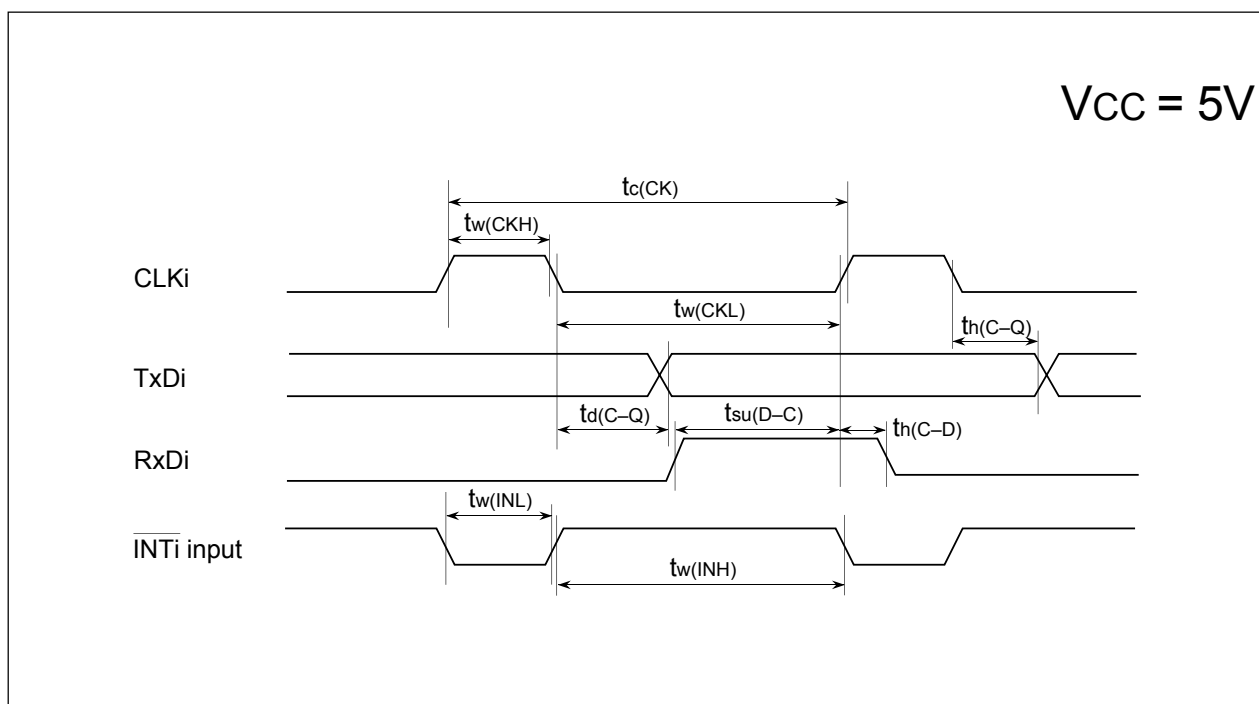
Figure 21.14 Timing Diagram (2)
