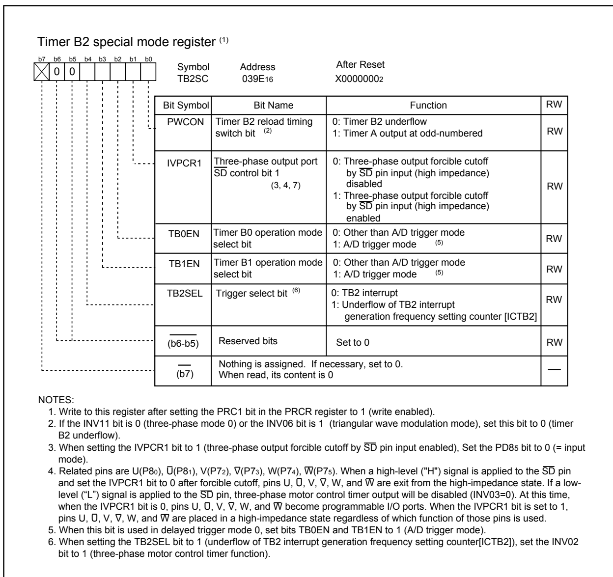
Figure 15.5 TB2SC Register
