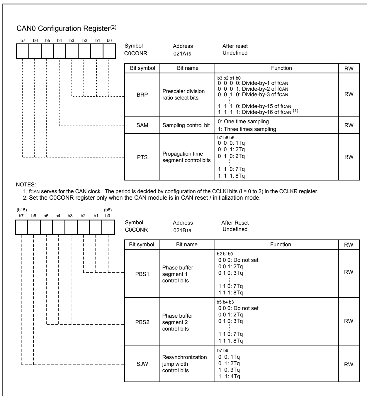
Figure 17.12 C0CONR Register
