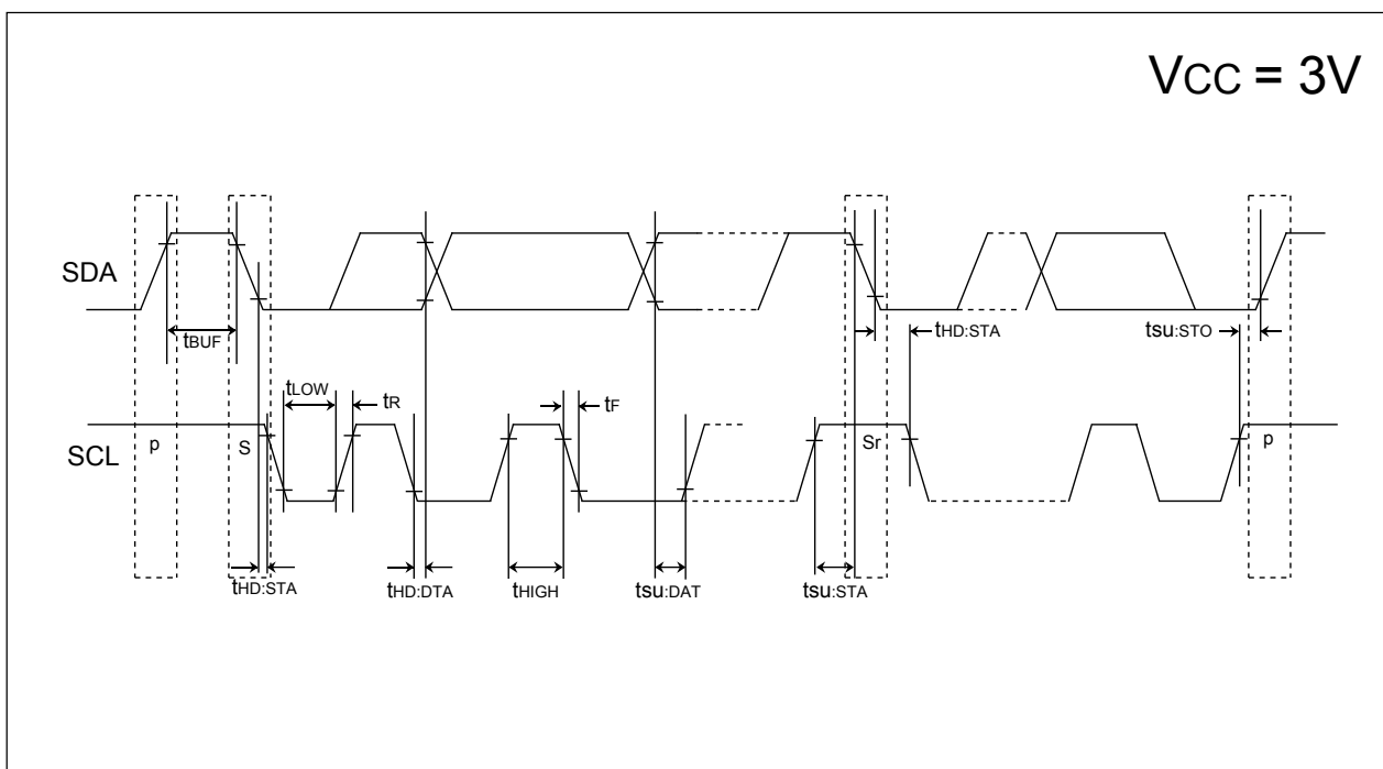
Figure 21.12 Timing Diagram (3)
