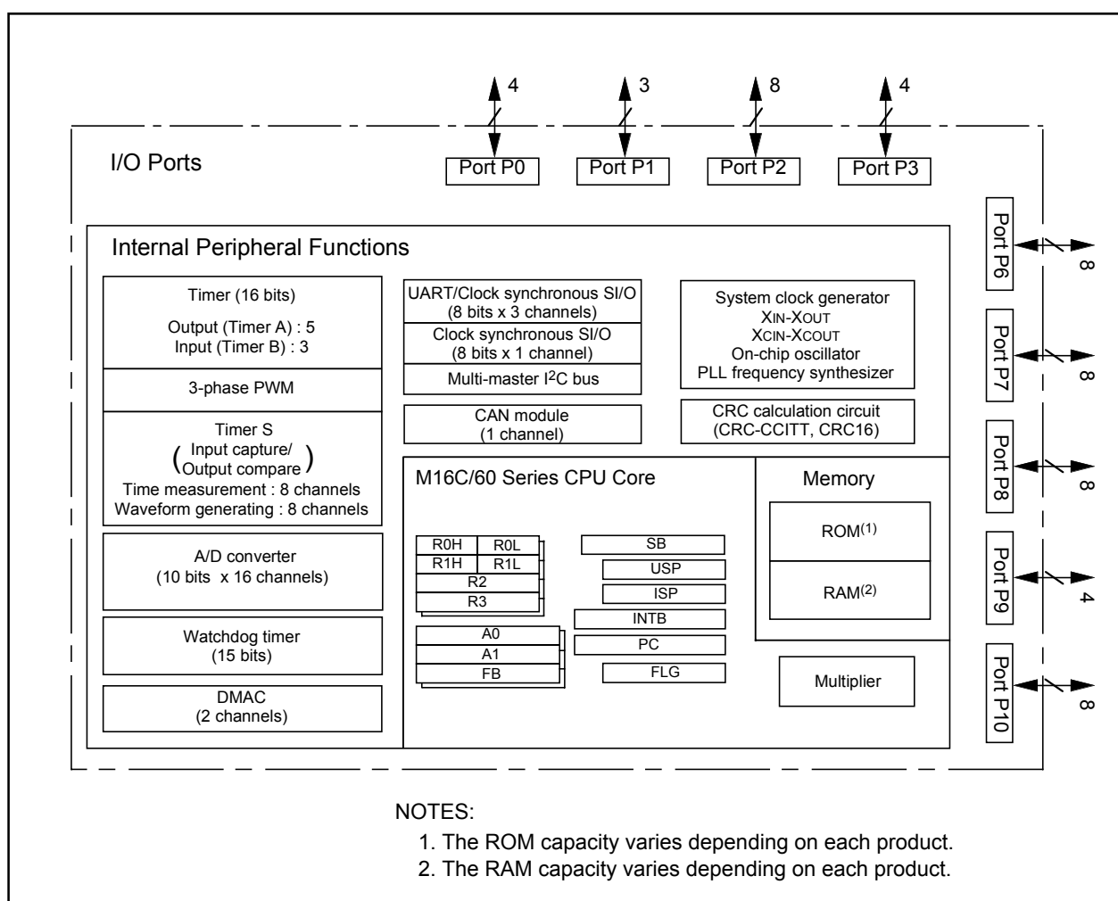
Figure 1.2 M16C/29 Group, 64-Pin Block Diagram
