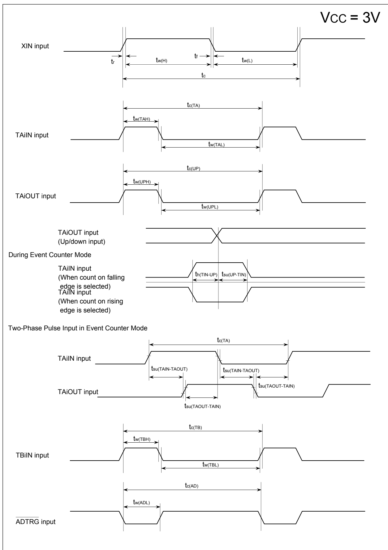
Figure 21.4 Timing Diagram (1)
