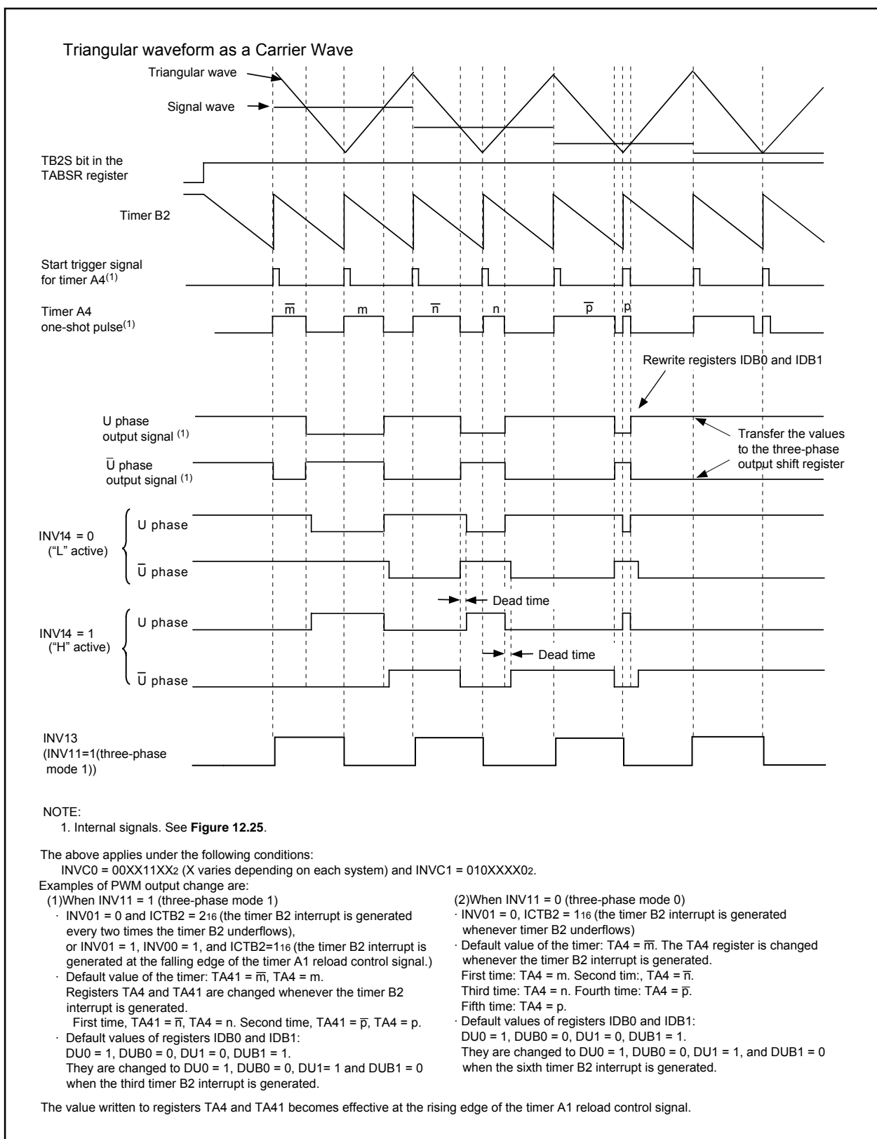
Figure 12.33 Triangular Wave Modulation Operation
