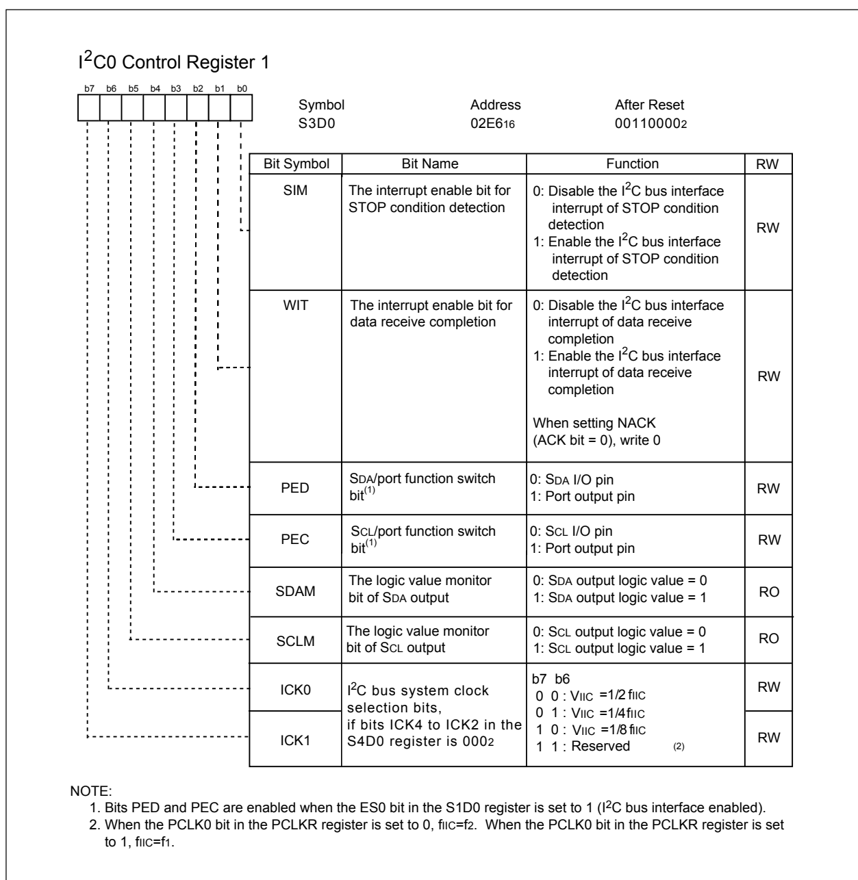
Figure 16.6 S3D0 Register
