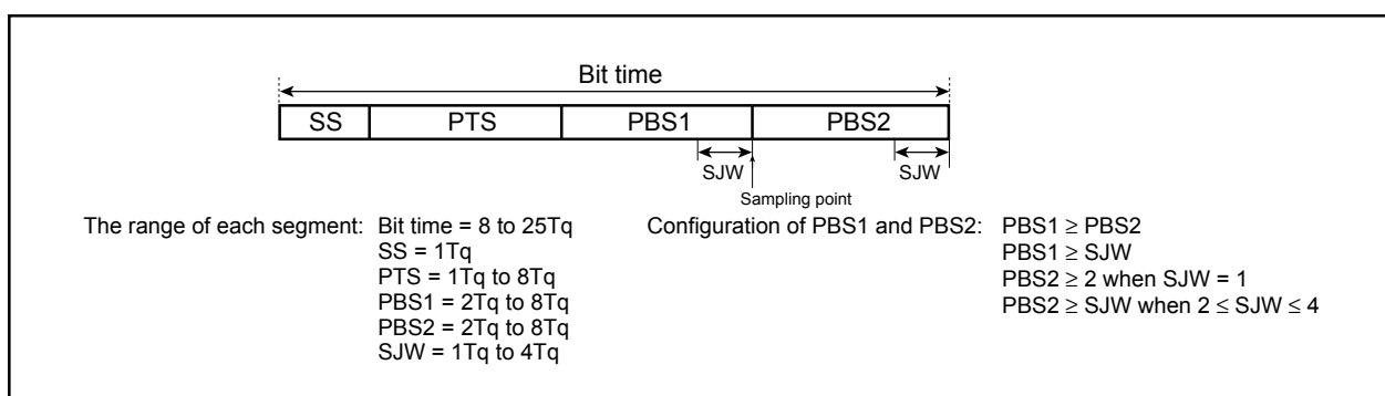
Figure 17.20 Bit Timing
