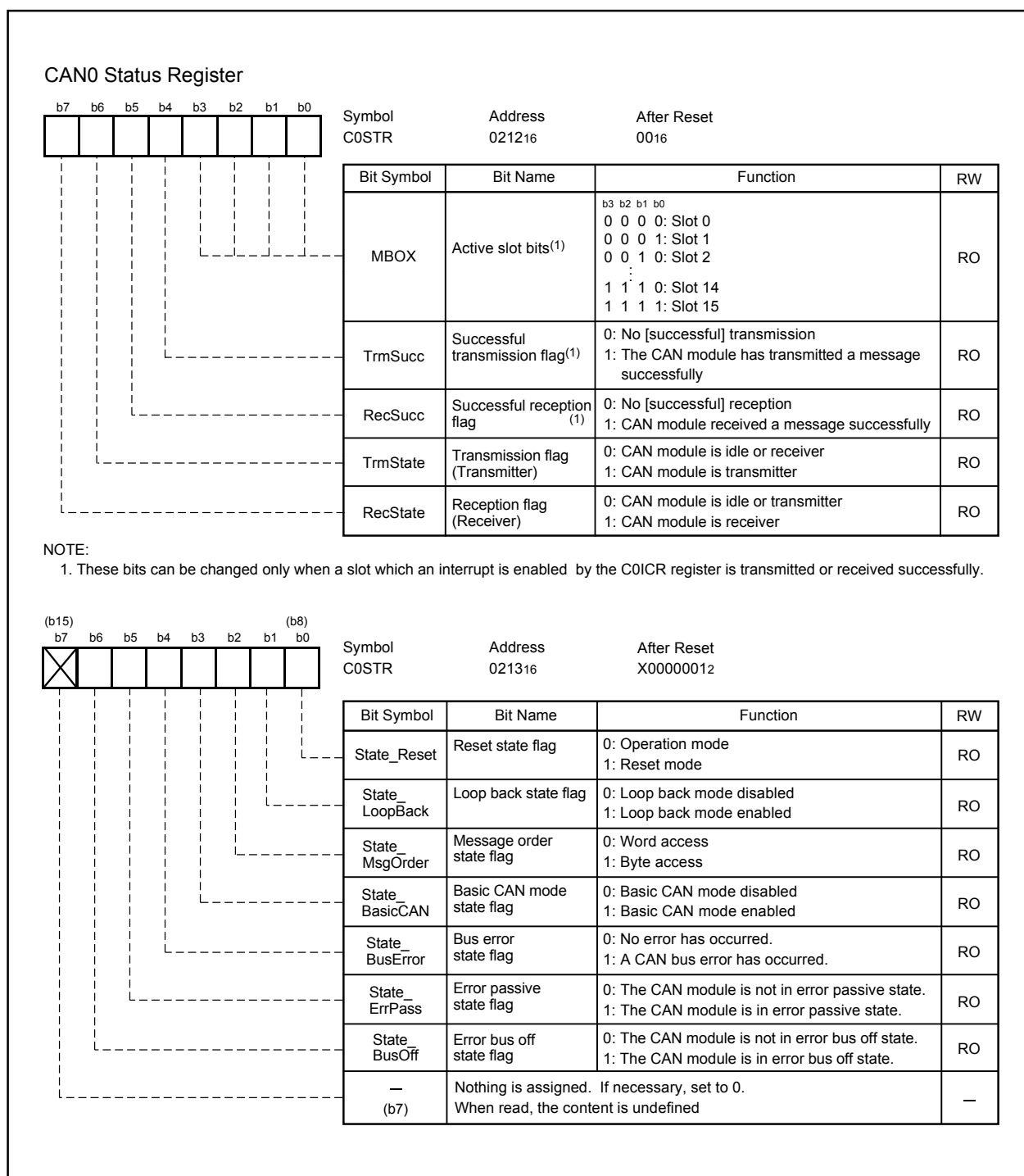
Figure 17.8 C0STR Register
