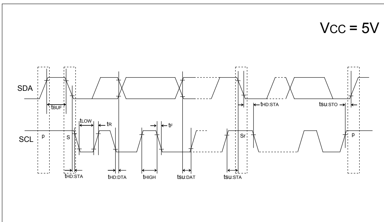
Figure 21.3 Timing Diagram (3)
