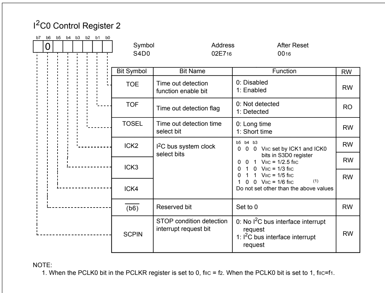
Figure 16.7 S4D0 Register
