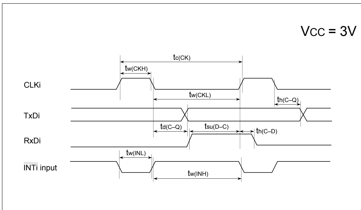
Figure 21.11 Timing Diagram (2)
