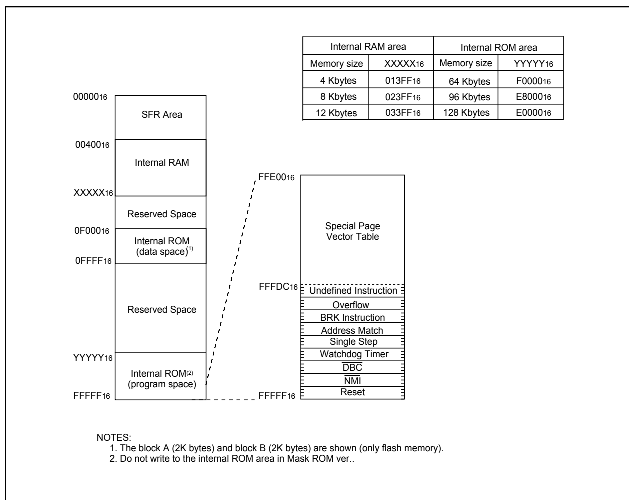
Figure 3.1 Memory Map
