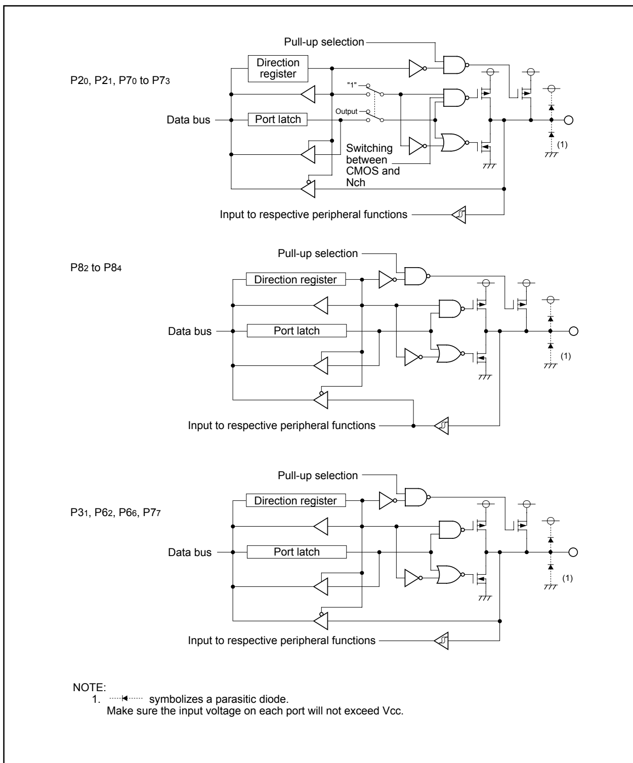
Figure 19.2 I/O Ports (2)
