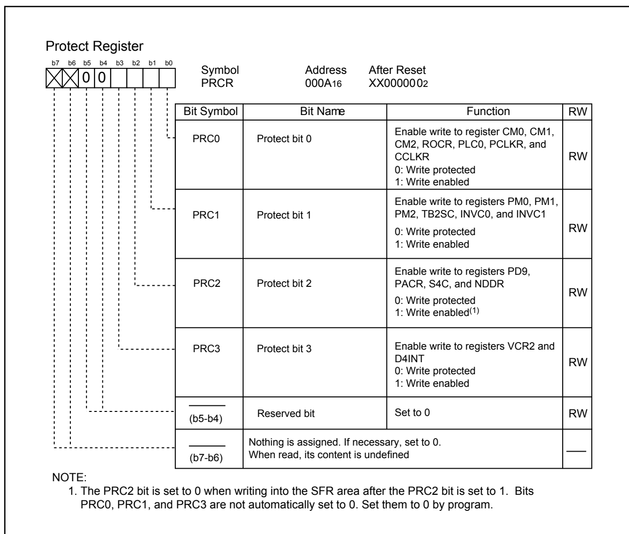
Figure 8.1 PRCR Register
