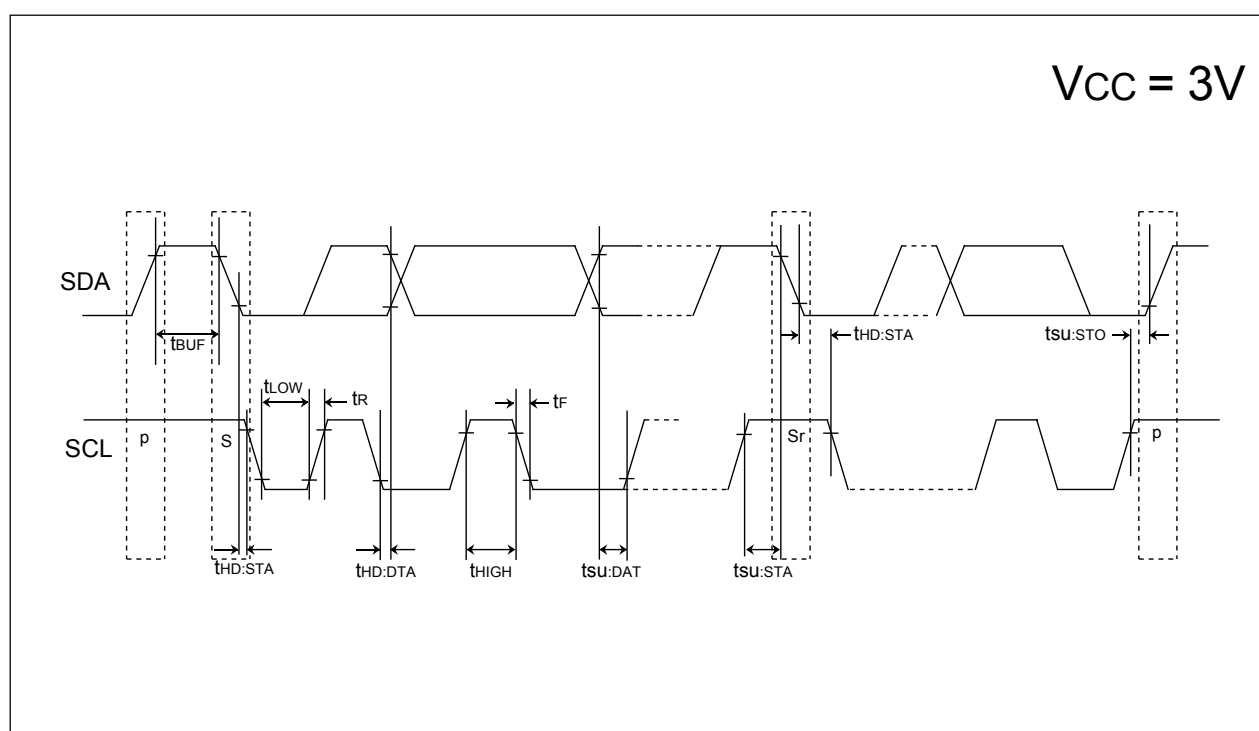
Figure 21.6 Timing Diagram (3)
