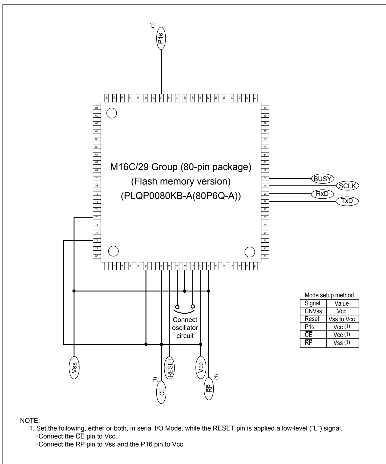
Figure 20.16 Pin Connections for Serial I/O Mode (2)
