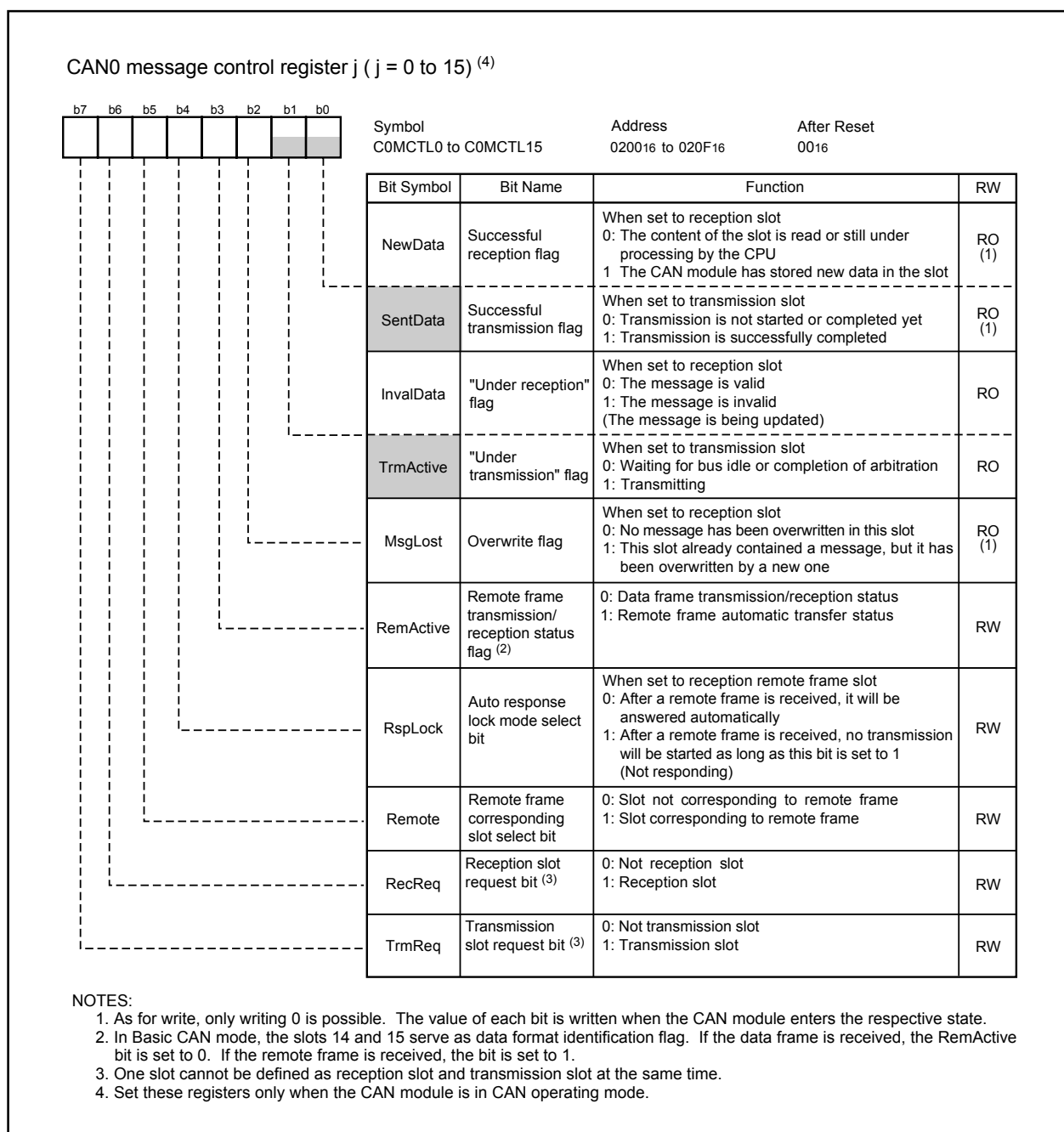
Figure 17.6 C0MCTLj Register
