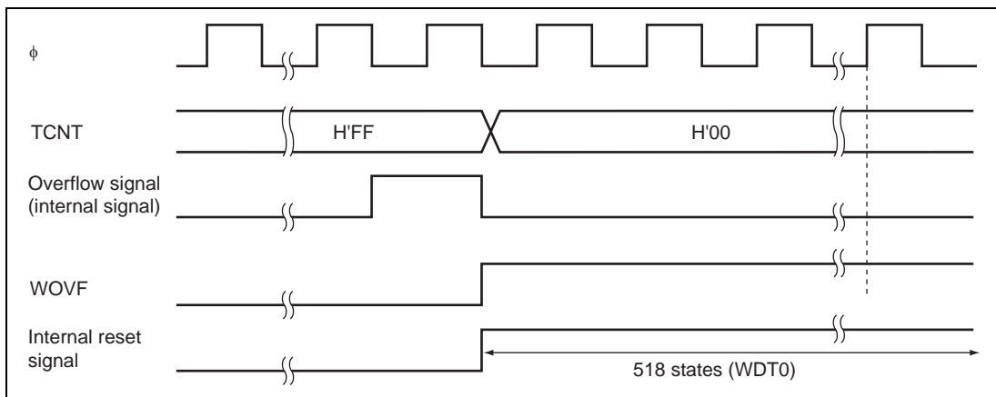
Figure 10.3 Timing of WOVSF Setting
