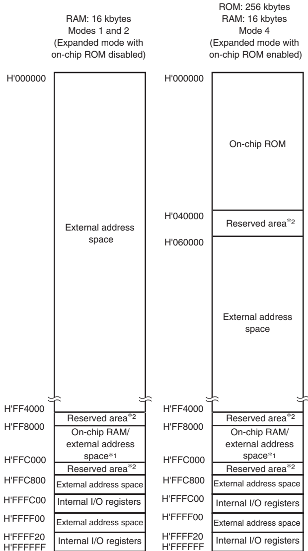
Figure 3.13 H8S/2365 Memory Map (1)
