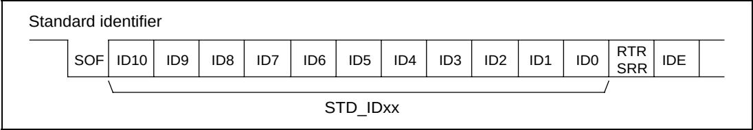
Figure 16.3 Standard Identifier
