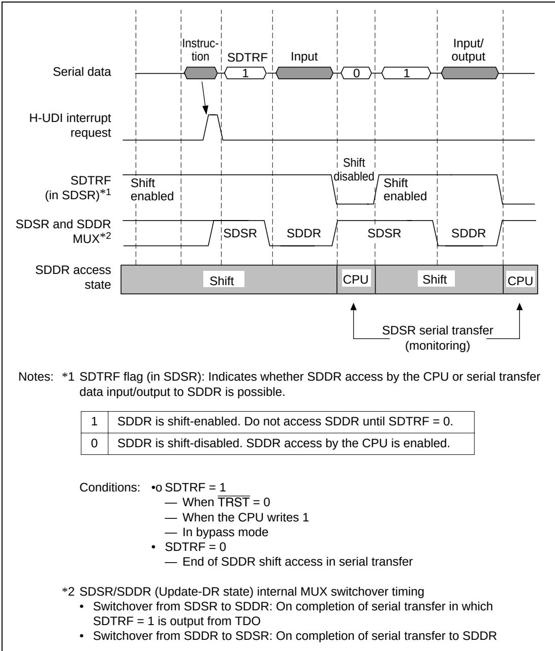
Figure 18.2 Data Input/Output Timing Chart (1)
