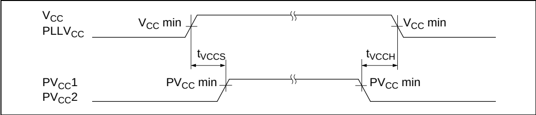
Figure 26.1 Power-On/Off Timing
