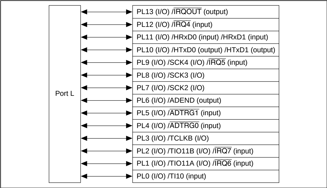
Figure 21.11 Port L
