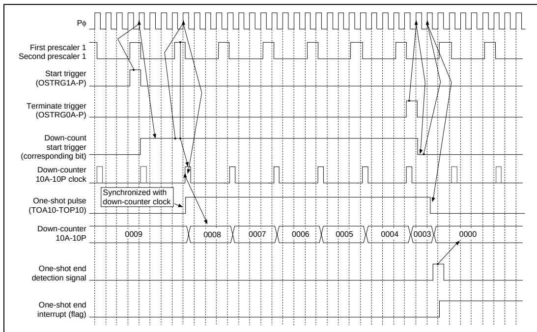
Figure 11.18 Offset One-Shot Pulse Output Function and Output Cutoff Function Operation
