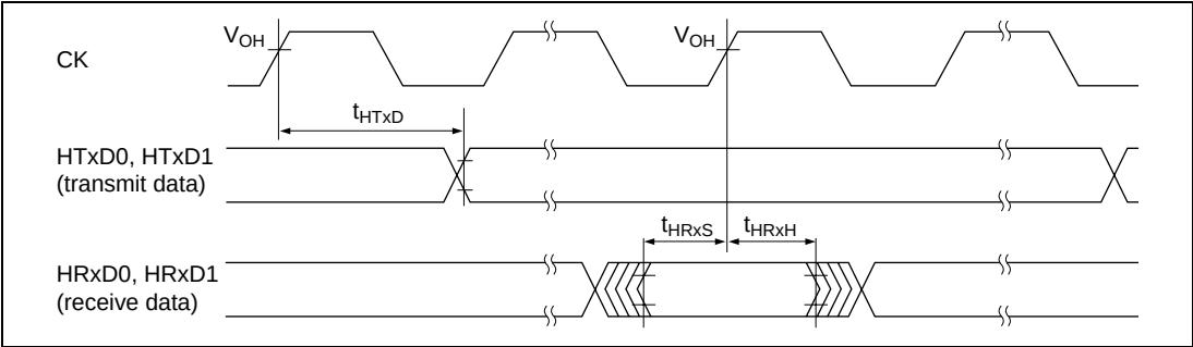
Figure 26.18 HCAN Input/Output timing
