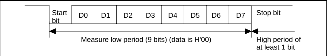
Figure 22.7 Automatic Adjustment Operation of SCI Bit Rate
