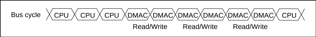
Figure 10.9 DMA Transfer Timing Example in Burst Mode
