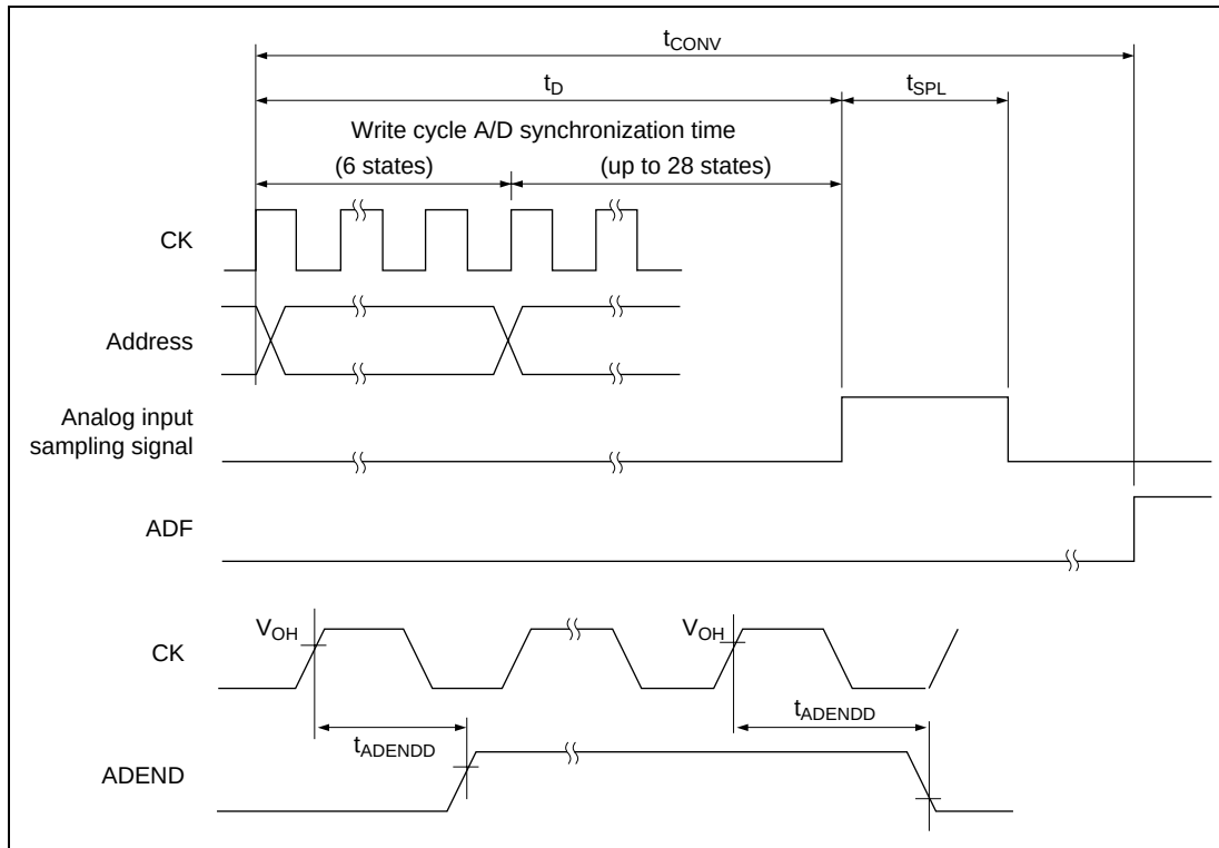
Figure 26.20 Analog Conversion Timing
