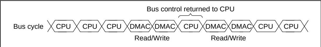
Figure 10.8 DMA Transfer Timing Example in Cycle-Steal Mode
