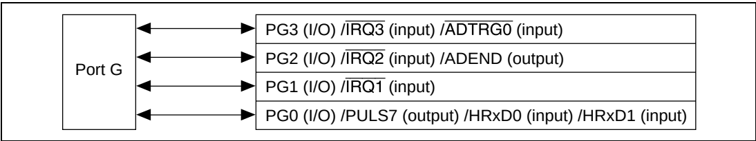
Figure 21.7 Port G
