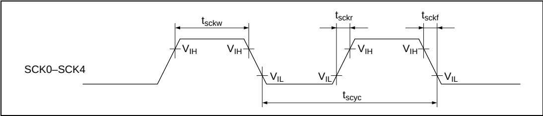
Figure 26.16 SCI Input/Output Timing
