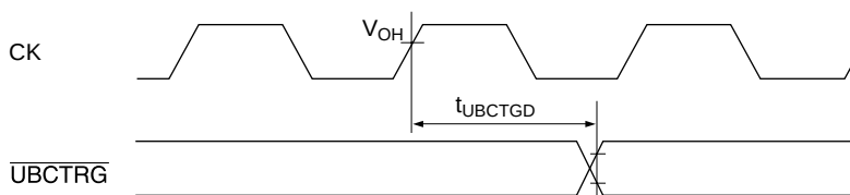
Figure 26.27 UBC Trigger Timing
