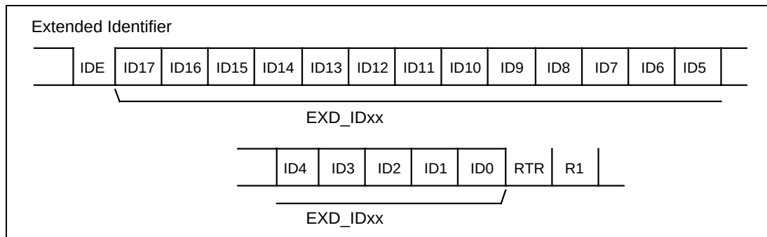
Figure 16.4 Extended Identifier
