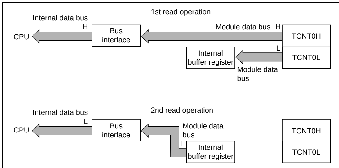
Figure 11.44 Read from TCNT0
