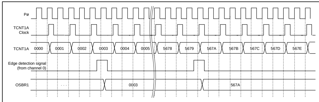
Figure 11.20 Twin-Capture Operation
