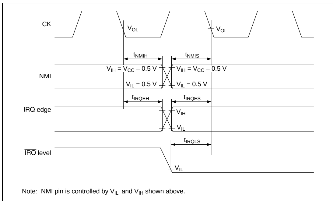
Figure 26.6 Interrupt Signal Input Timing
