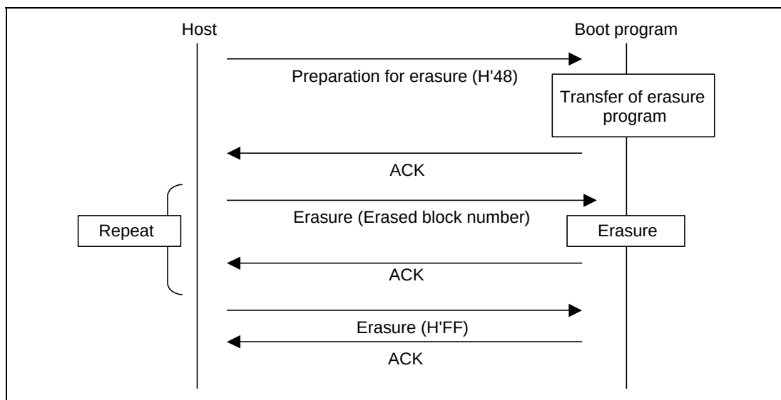
Figure 22.31 Erasing Sequence
