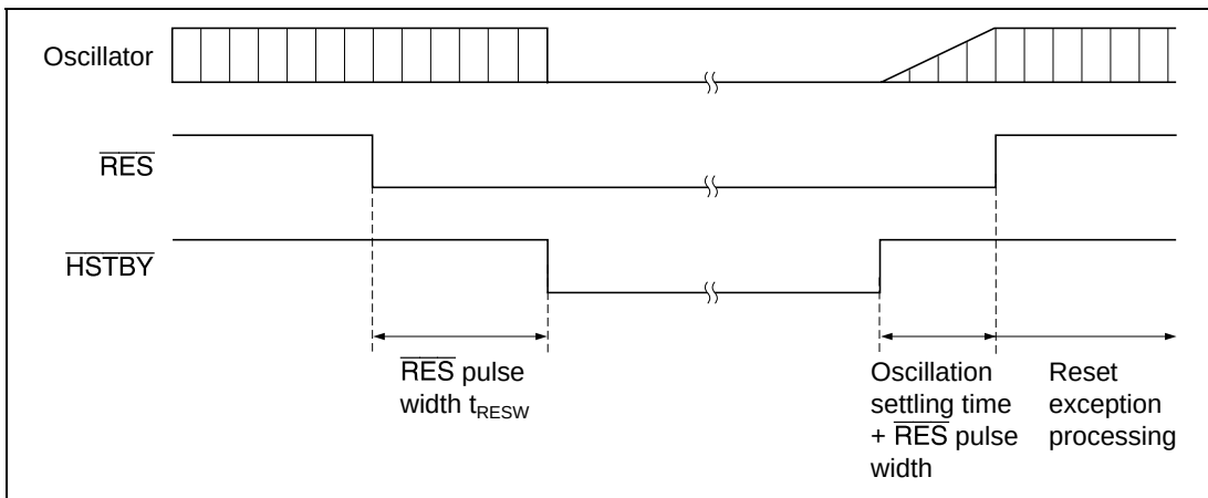
Figure 24.2 Hardware Standby Mode Timing
