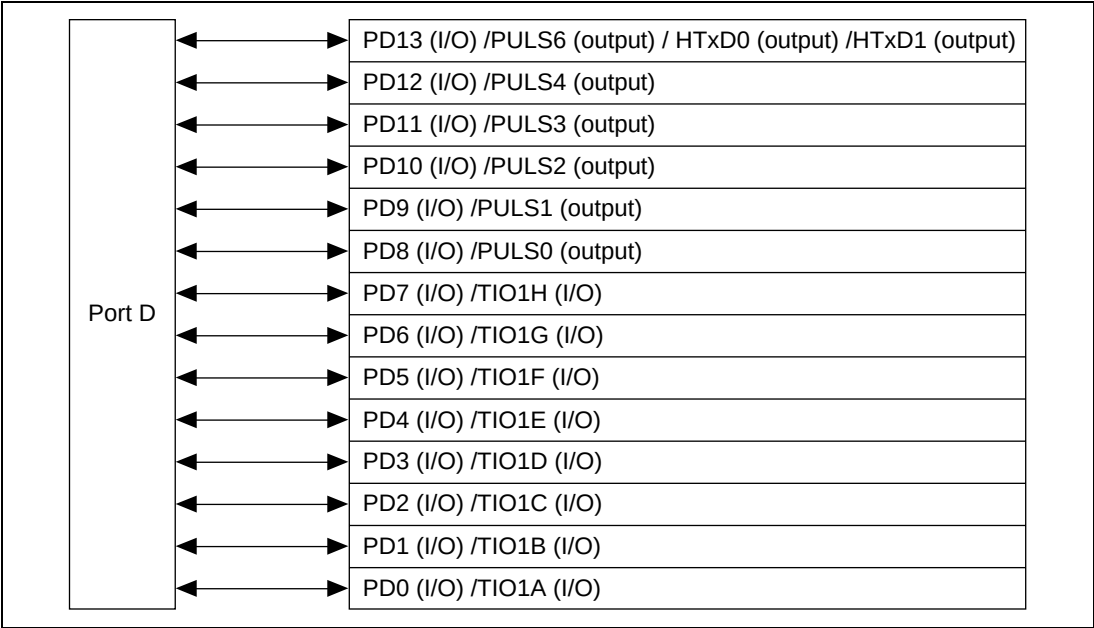
Figure 21.4 Port D
