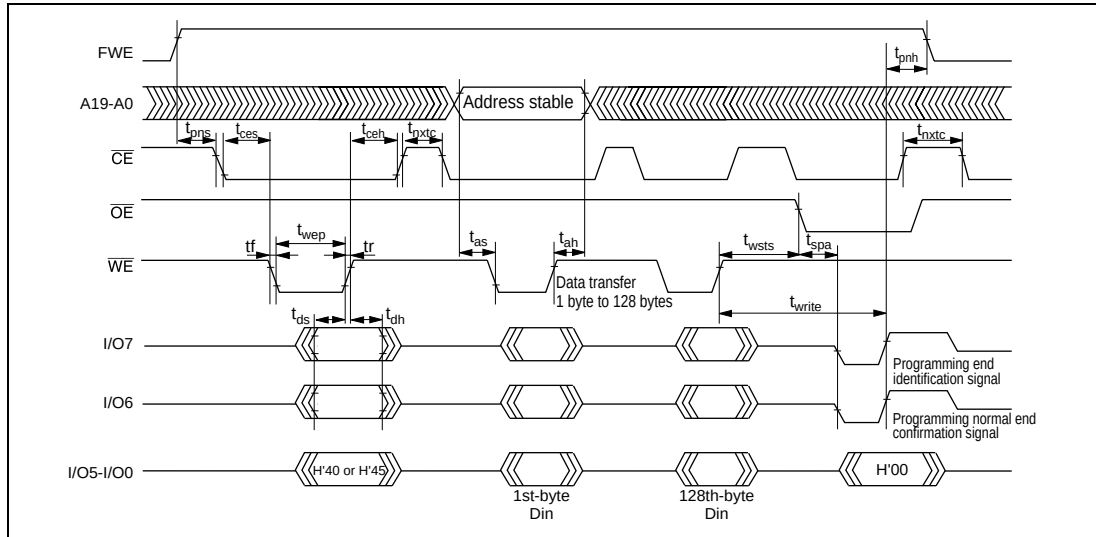
Figure 22.36 Timing in Auto-Program Mode
