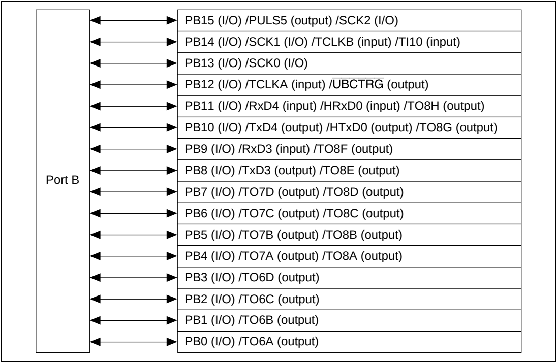
Figure 21.2 Port B
