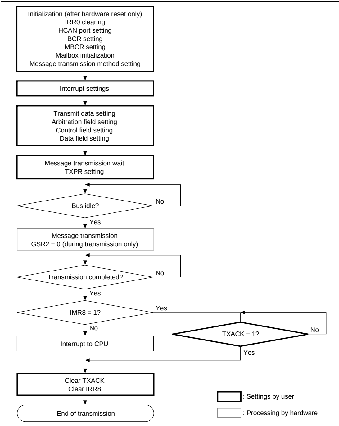
Figure 16.9 Transmission Flowchart
