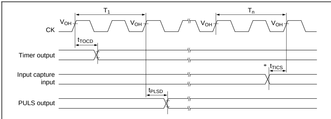
Figure 26.12 ATU Input/Output timing and APC Output timing
