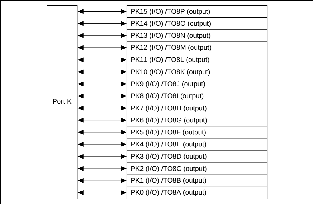
Figure 21.10 Port K
