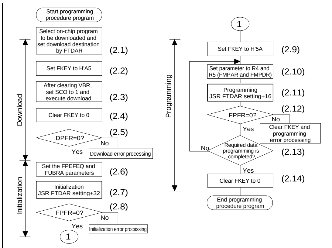
Figure 22.11 Programming Procedure
