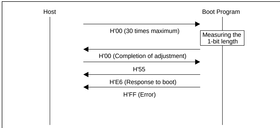
Figure 22.27 Bit-Rate-Adjustment Sequence
