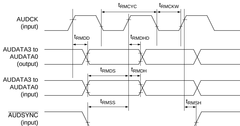
Figure 26.26 RAM Monitor Timing
