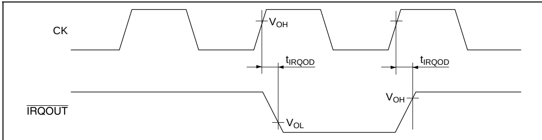
Figure 26.7 Interrupt Signal Output Timing
