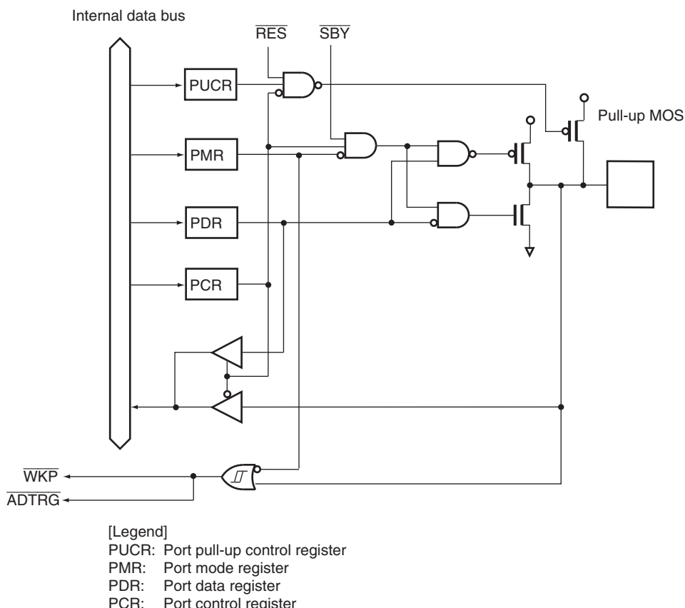
Figure B.9 Port 5 Block Diagram (P55)
