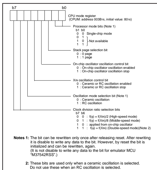
Fig. 80 Structure of CPU mode register
