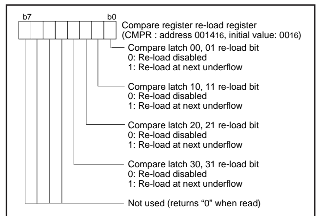
Fig. 36 Structure of compare register re-load register
