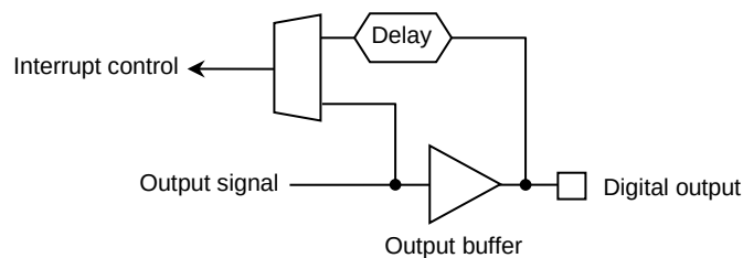
Fig.4-14-2 Diagram of digital monitoring
