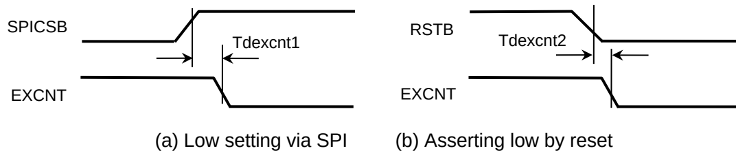
Fig. 4-10-4 EXCNT delay
