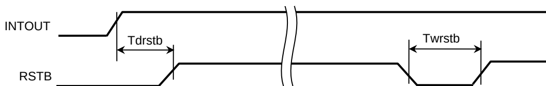
Fig. 4-9-2 RSTB timing 1
