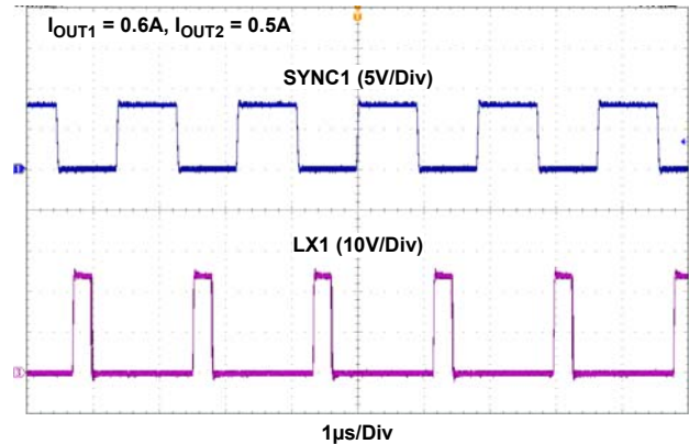
Figure 29. SYNC1 at 1.1A Load
