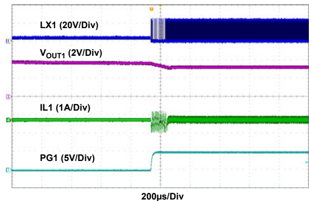
Figure 31. Negative Current Limit Recovery
