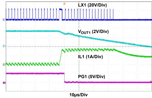
Figure 27. Overcurrent Protection
