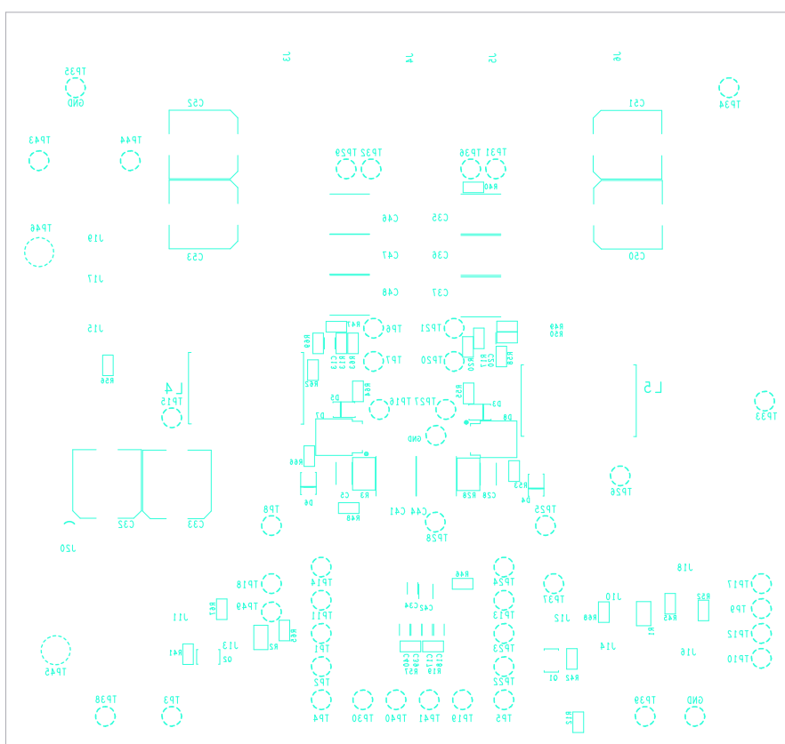
Figure 14. Silkscreen Bottom
