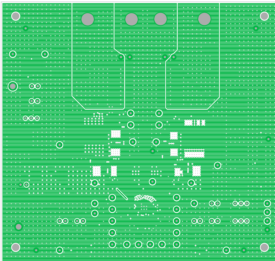
Figure 9. Layer 2
