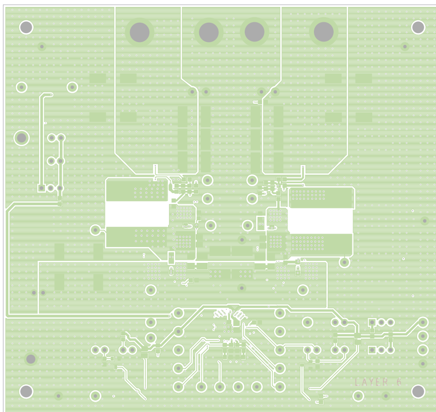
Figure 13. Layer 6
