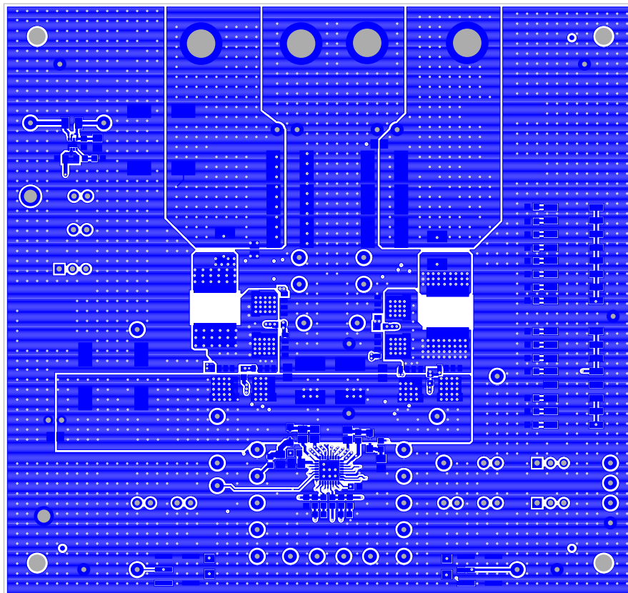
Figure 8. Layer 1
