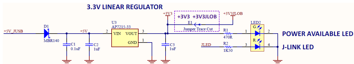
Figure 10. 3.3 V Power Regulator Circuit
