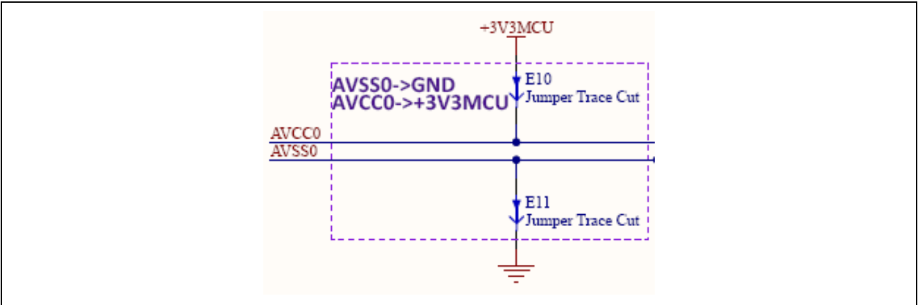
Figure 29. Analog and Reference Voltages
