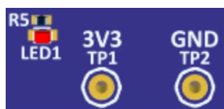
Figure 8. TP1, TP2, and LED1 on the Evaluation Kit Board
