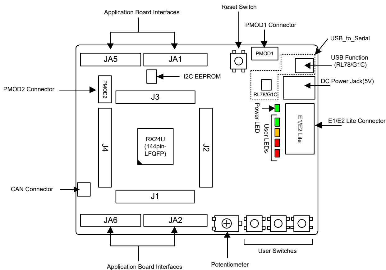
Figure 3-1: Board Layout
