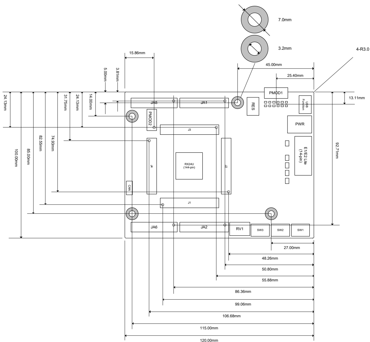
Figure 3-2: Board Dimensions
