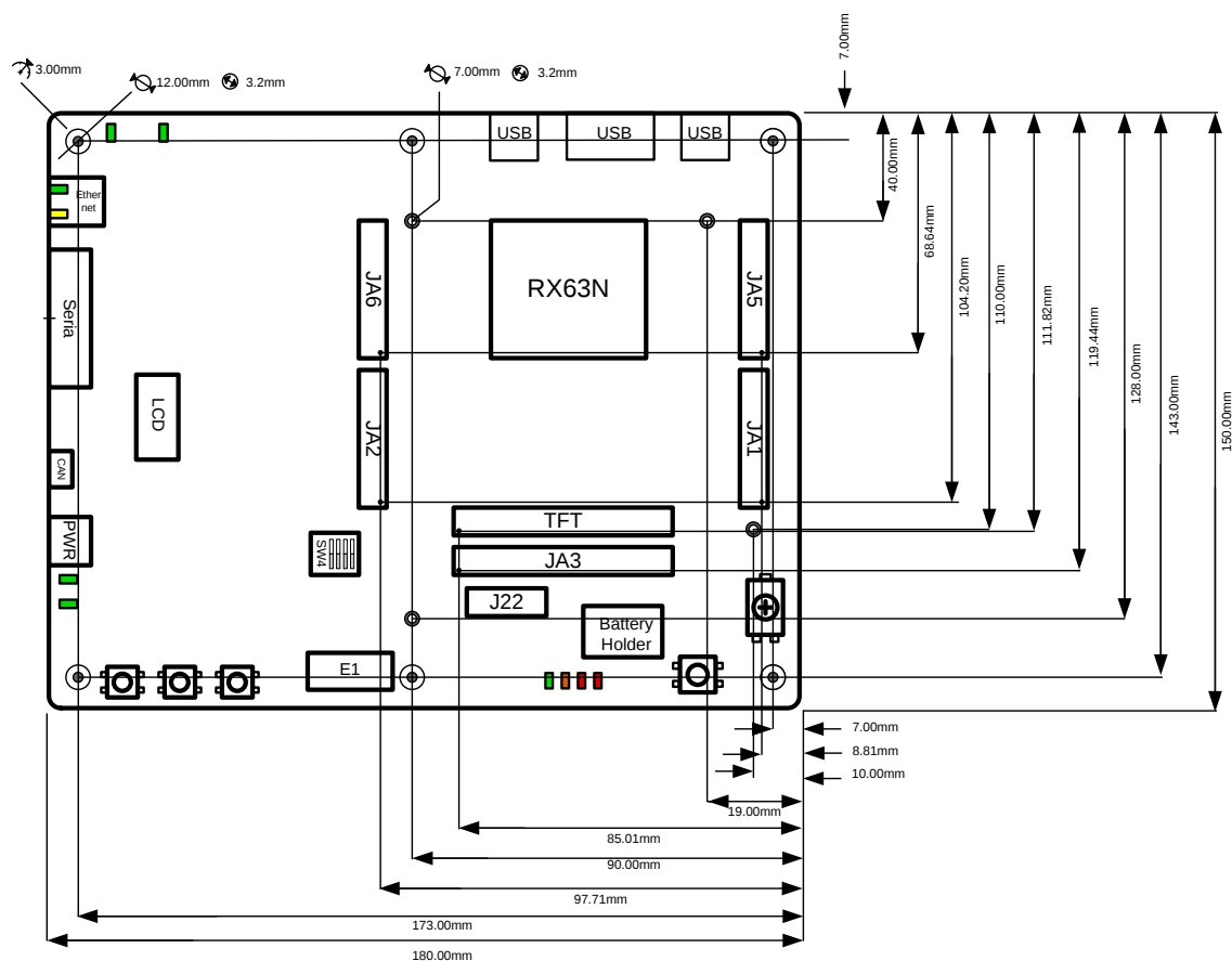
Figure 3-2: Board Dimensions
