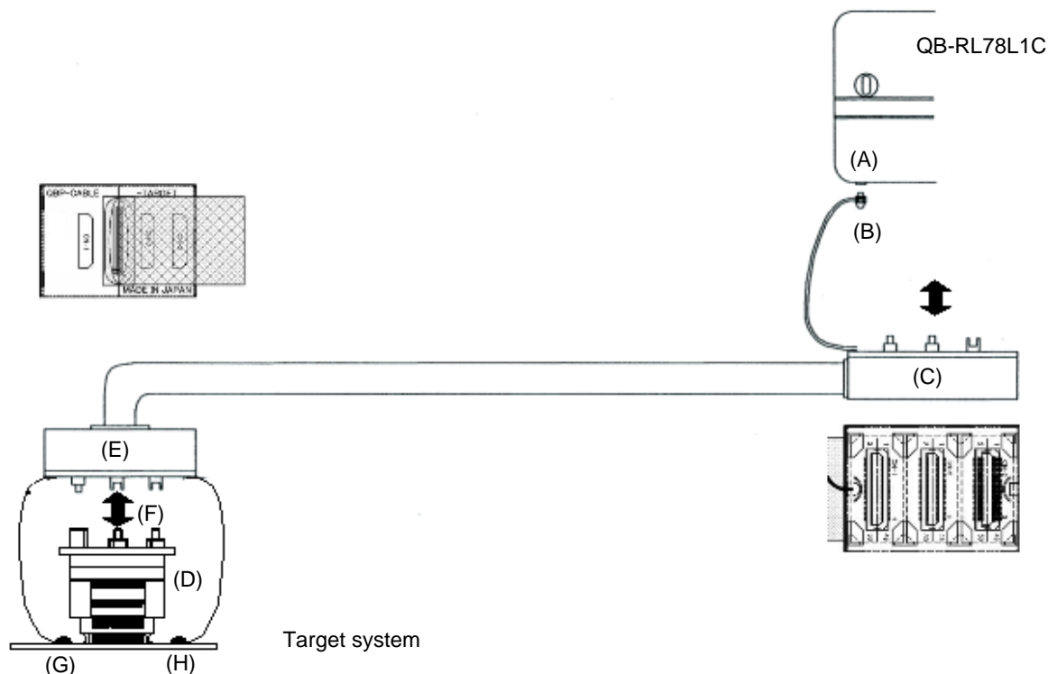
Figure 2-6. GND Wire
