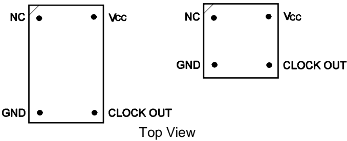
Figure 2-3. Mapping of Oscillator to Socket
