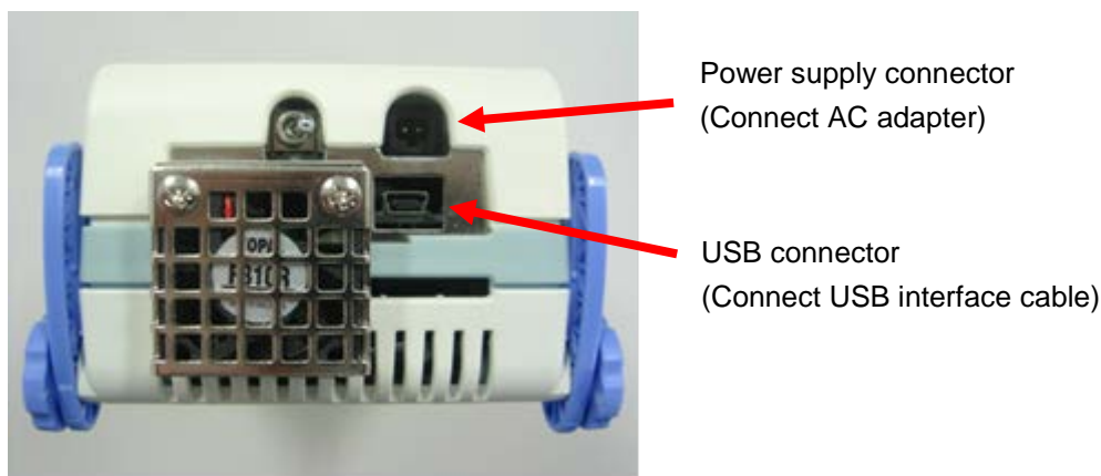
Figure 2-8. Connector Positions
