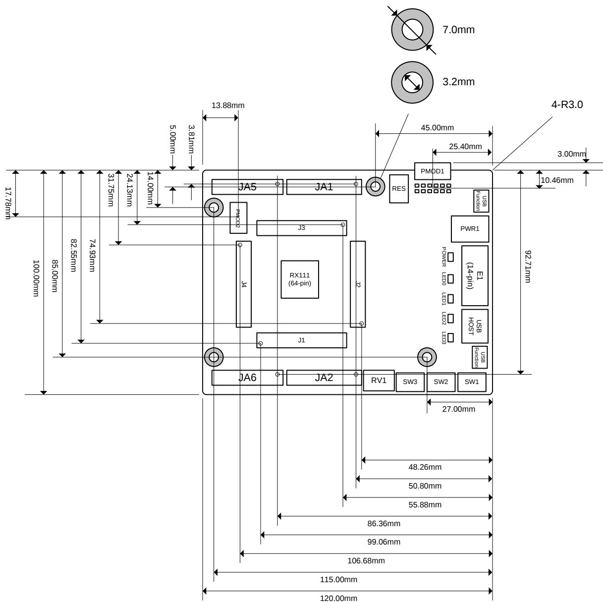
Figure 3-2: Board Dimensions
