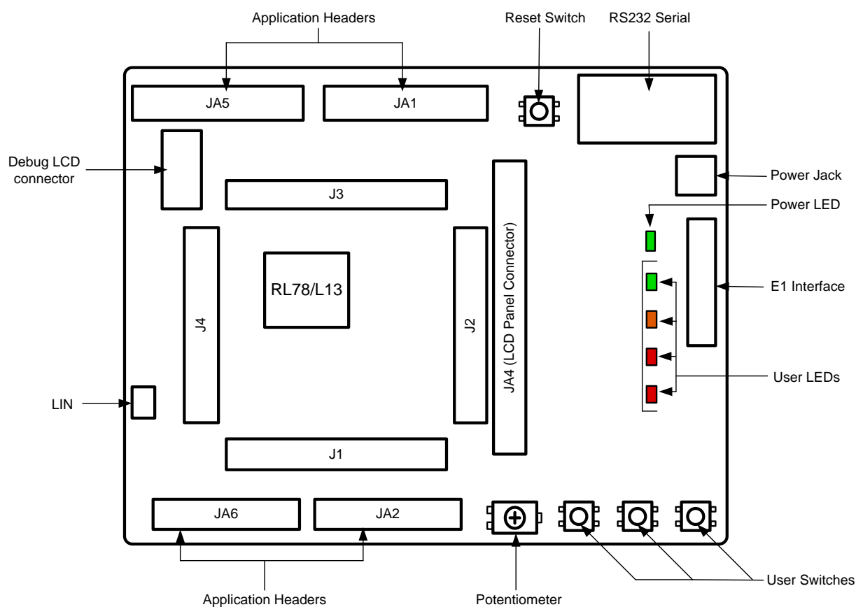
Figure 3-1: Board Layout
