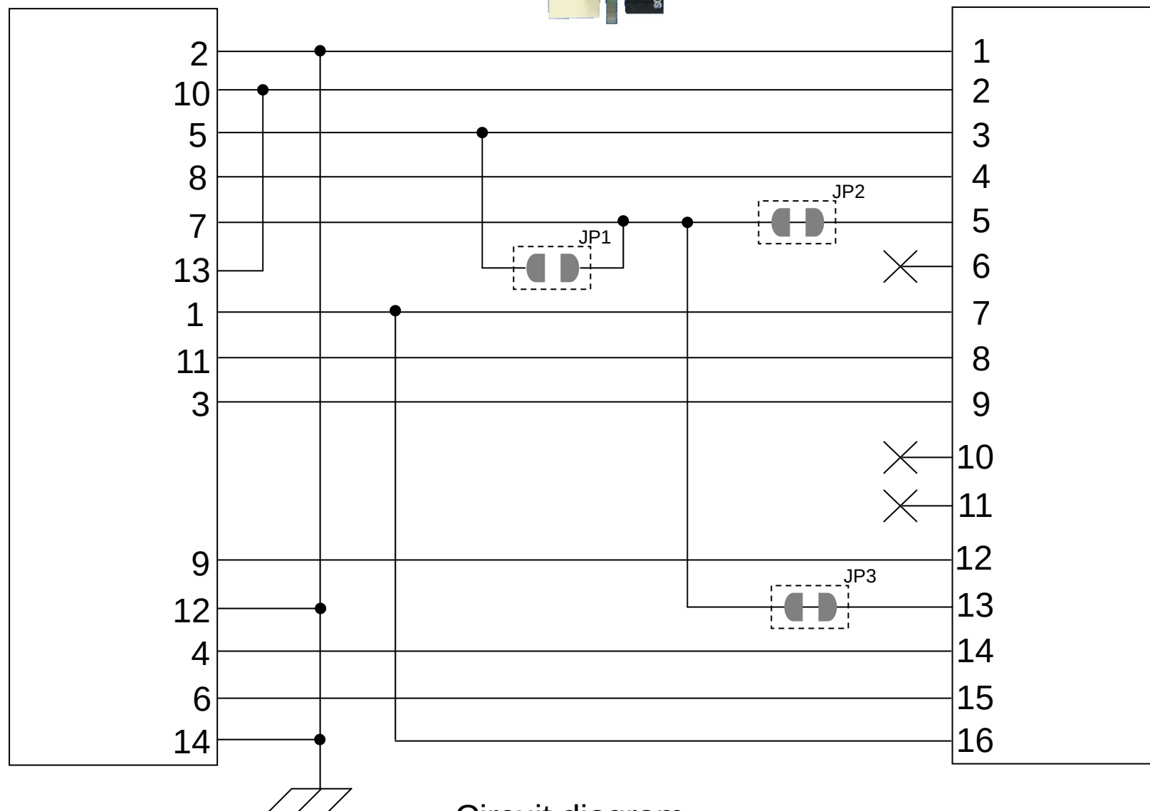
Circuit diagram
