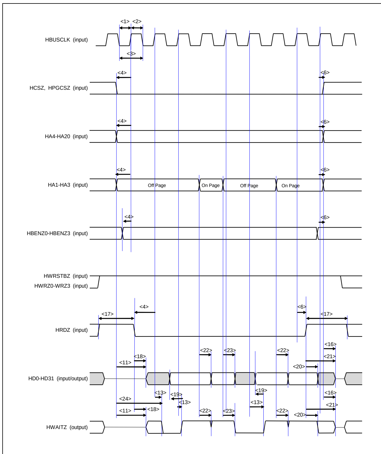
Figure 3.13 External MCU Interface Page Read Timing (MEMCSEL=L, HIFSYNC=H)
