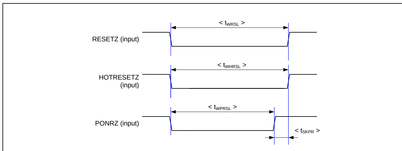
Figure 3.6 Reset Timing
