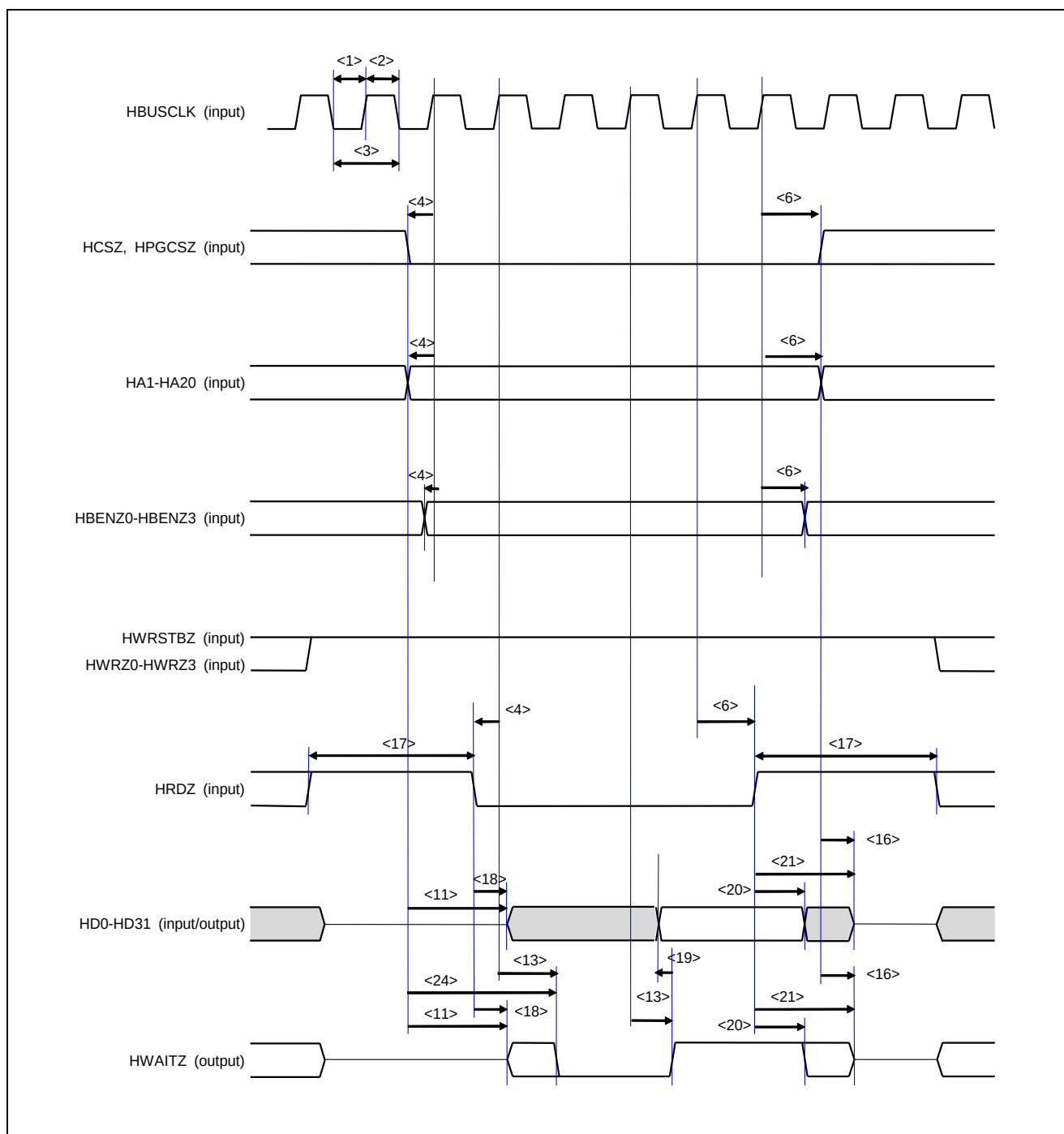
Figure 3.12 External MCU Interface Read Timing (MEMCSEL=L, HIFSYNC=H)
