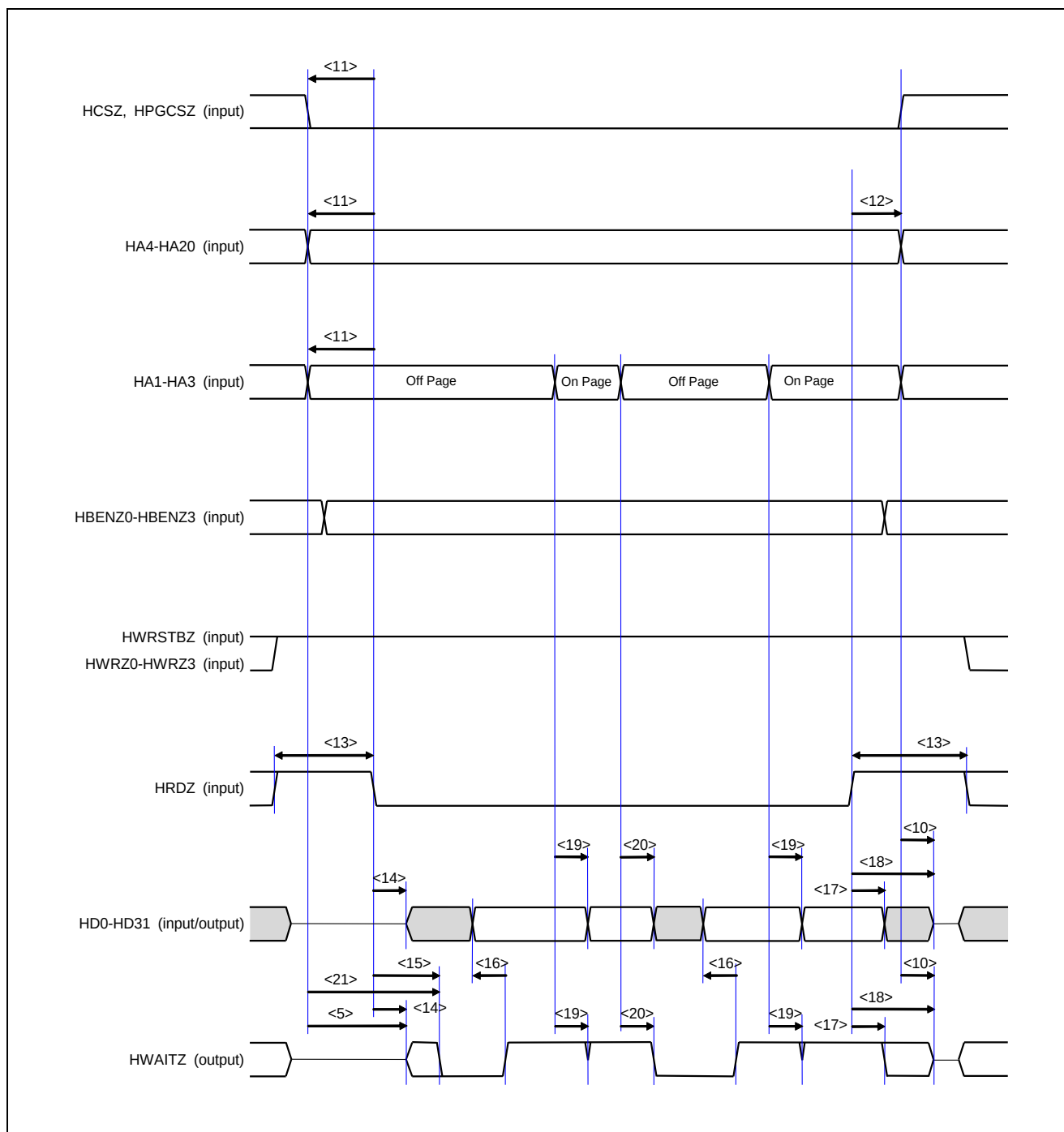
Figure 3.16 External MCU Interface Page Read Timing (MEMCSEL=L, HIFSINC=L)
