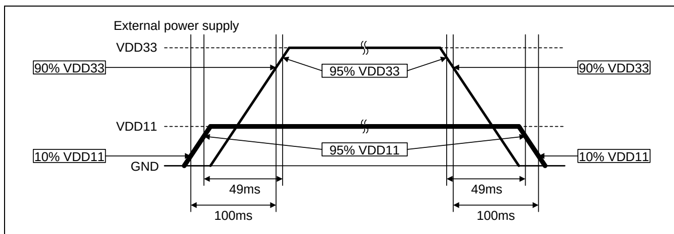
Figure 3.3 Power-On/Off Sequence (with 2.5-V built-in Regulator)
