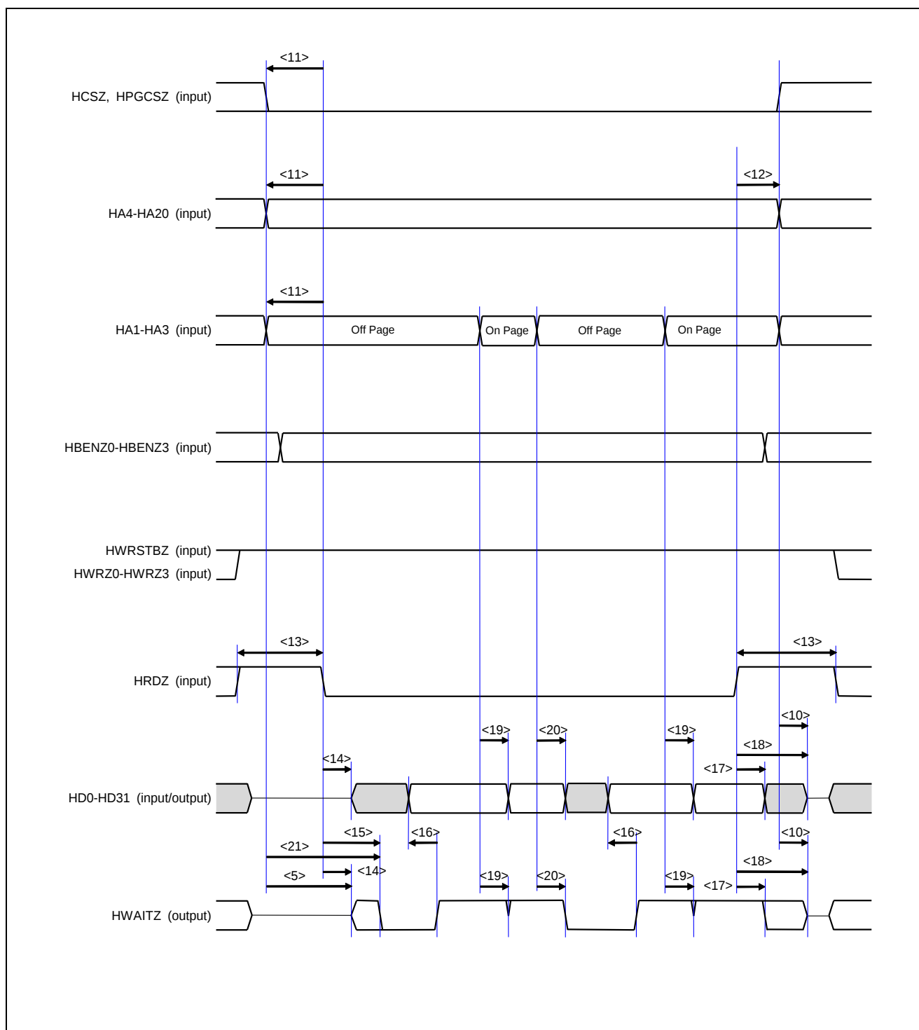
Figure 4.15 External MCU Page-Read Timing (MEMCSEL = L, HIFSUNC = L)
