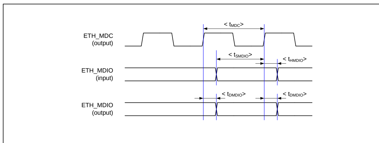
Figure 4.29 Ethernet Access Timing Diagram (Serial Management)
