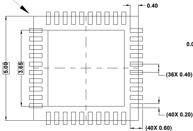
PACKAGE OUTLINE
