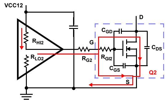
Figure 9. Typical Lower-Gate Drive Turn-On Path
