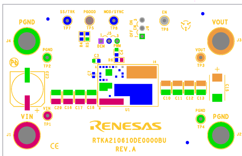
Figure 8. Silkscreen Top
