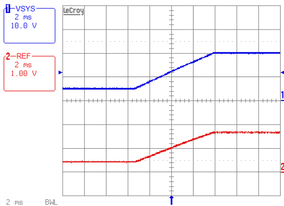
Figure 18. Forward Mode, 5VSY to 20VSY
