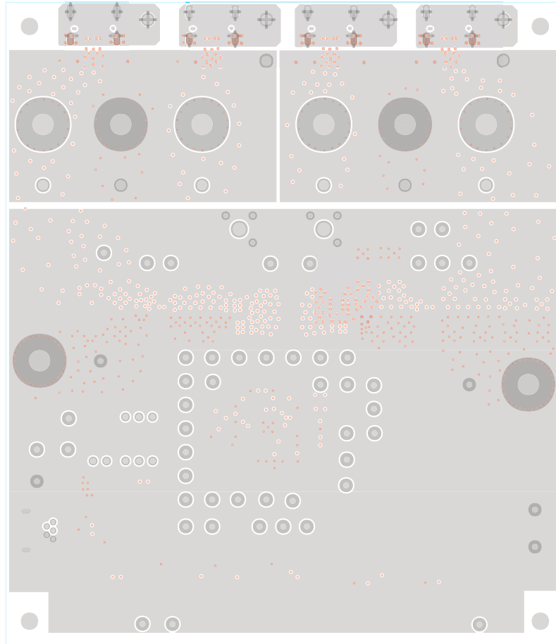
Figure 9. Inner Layer 1
