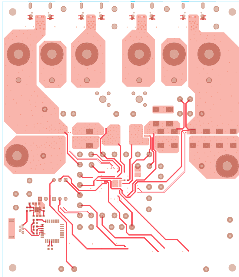
Figure 11. Bottom Layer
