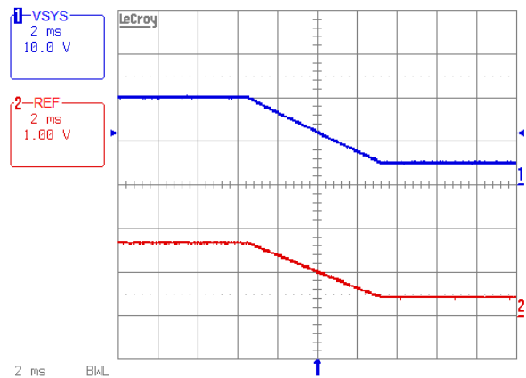
Figure 19. Forward Mode, 20VSY to 5VSY
