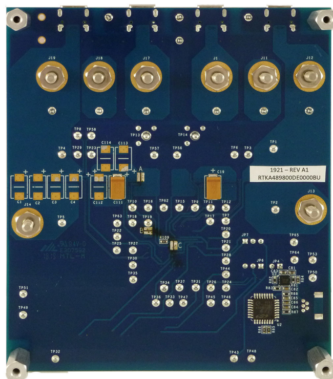
Figure 5. Evaluation Board Bottom
