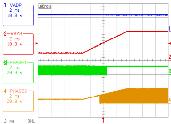
Figure 14. VSYS Voltage Ramps Up in Forward Mode, Buck -&gt; Buck-Boost -&gt; Boost Operation Mode Transition
