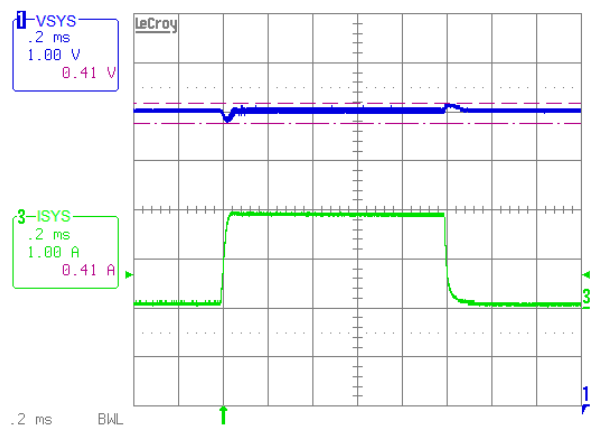
Figure 24. Forward Mode, 5VADP, 12VSYN, 0-2A Transient Load
