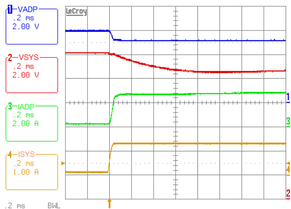
Figure 21. Forward Mode, Output Voltage Loop to Adapter Voltage Loop Transition. 6VADP, Input Voltage Limit = 5.12V, 12VSY, System Load 0A to 1.3A Step, System Current Limit = 5A, Input Current Limit = 5A
