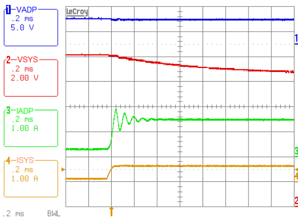
Figure 20. Forward Mode, Output Voltage Loop to ADP Current Loop Transition. 5VADP, 12VSY, System Load 0A to 0.65A Step, ADP Current Limit = 1.5A
