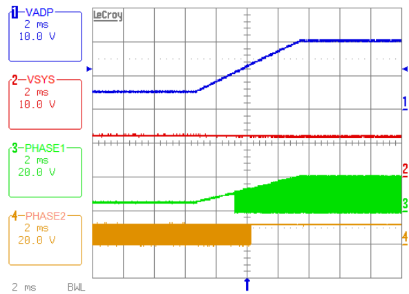
Figure 15. ADP Voltage Ramps Up in Reverse Mode, Buck -&gt; Buck-Boost -&gt; Boost Operation Mode Transition
