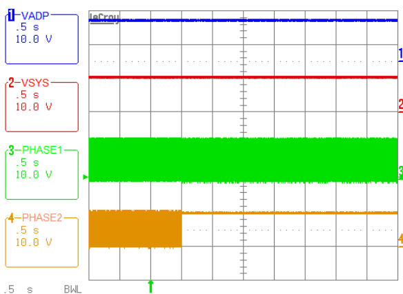
Figure 22. Forward Mode, Force Buck-Boost Mode to Buck Mode. 12VADP, 10.1VSY
