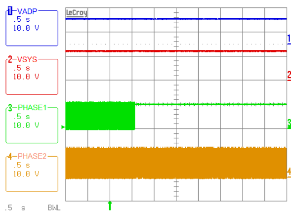
Figure 23. Reverse Mode, Force Buck-Boost Mode to Buck Mode. 10.1VADP, 12VSY
