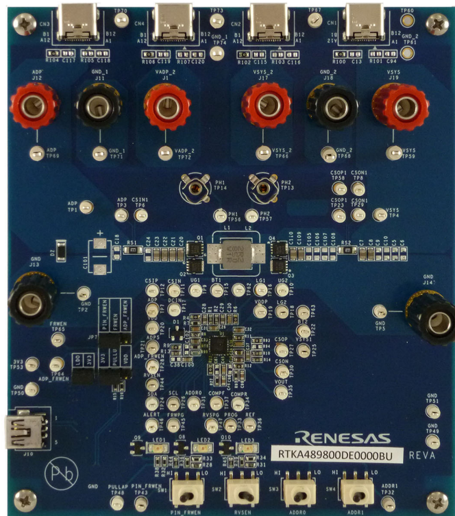
Figure 4. Evaluation Board Top
