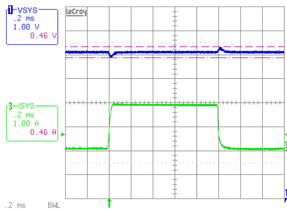
Figure 25. Reverse Mode, 20VADP, 12VSYN, 0-2A Transient Load
