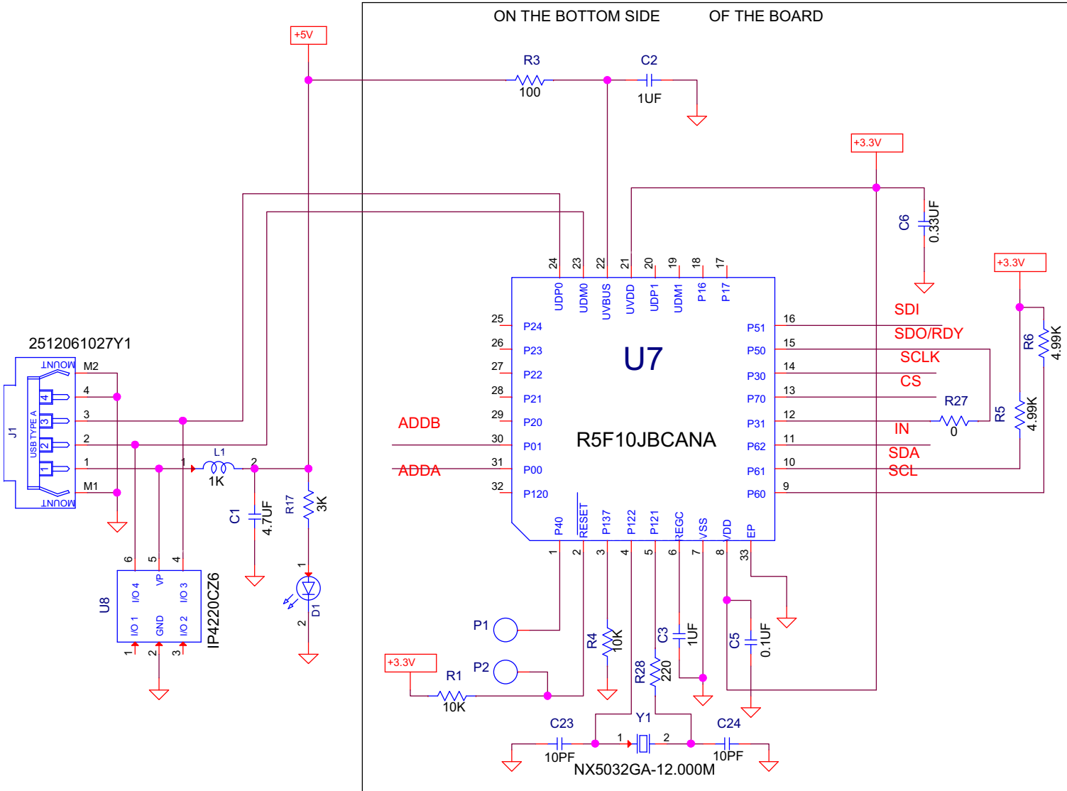
Figure 20. RTKA-BDGSTKEV2Z MCU Schematic
