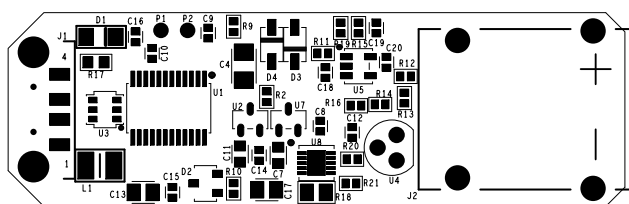
Figure 17. Top Assembly Drawing
