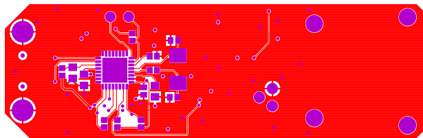
Figure 16. Bottom Layer
