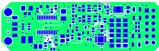
Figure 7. Top Layer
