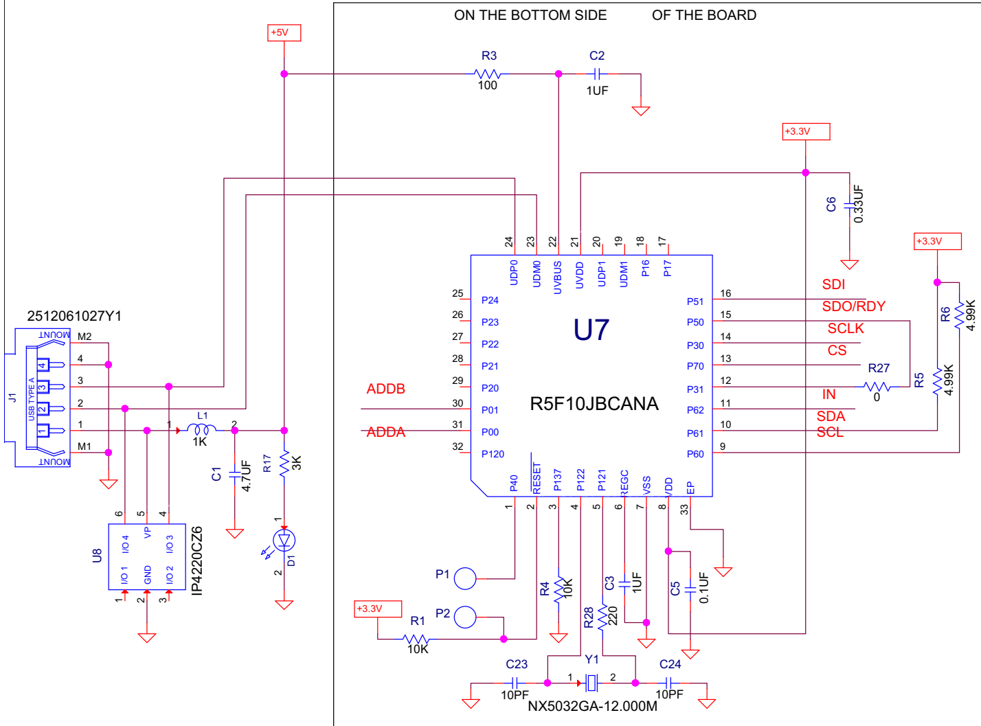
Figure 12. RTKA-BDGSTKEV2Z MCU Schematic
