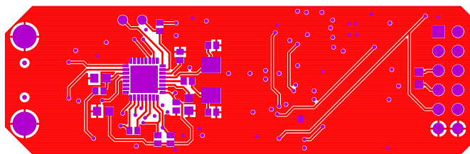
Figure 8. Bottom Layer
