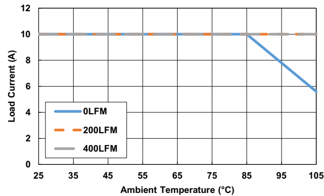
Figure 25. Derating Curve, V_{OUT} = 1V
