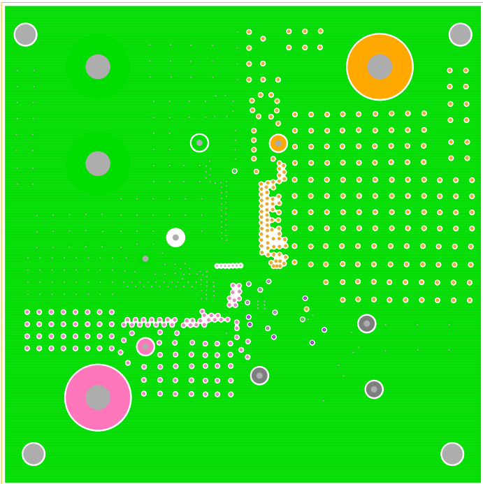
Figure 12. Inner Layer 5
