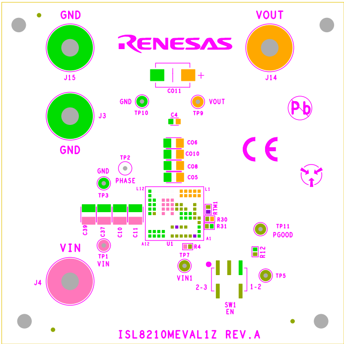
Figure 7. Silkscreen Top
