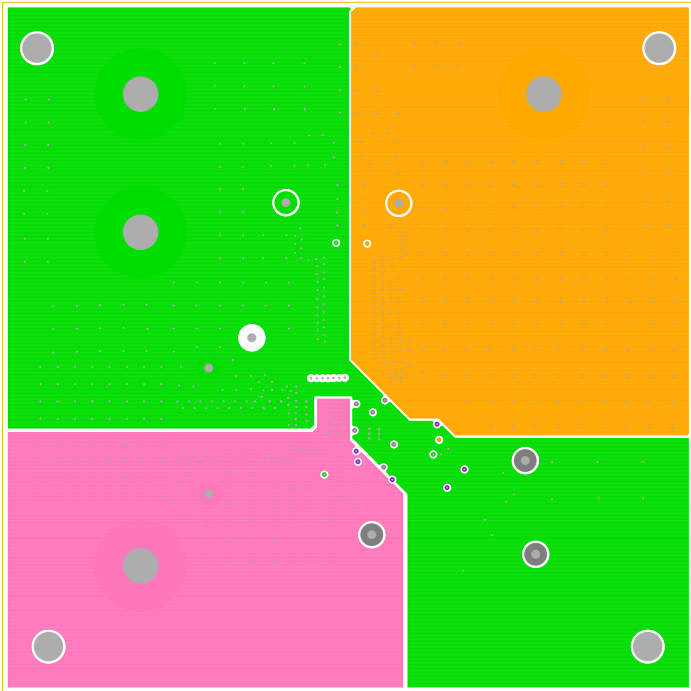
Figure 11. Inner Layer 4
