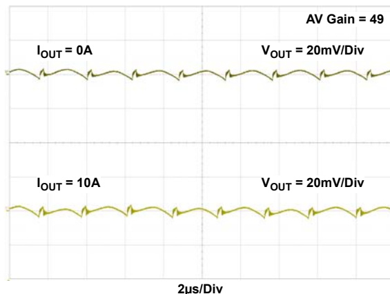
Figure 20. Output Ripple at 12V IN and 1V OUT , 400kHz
