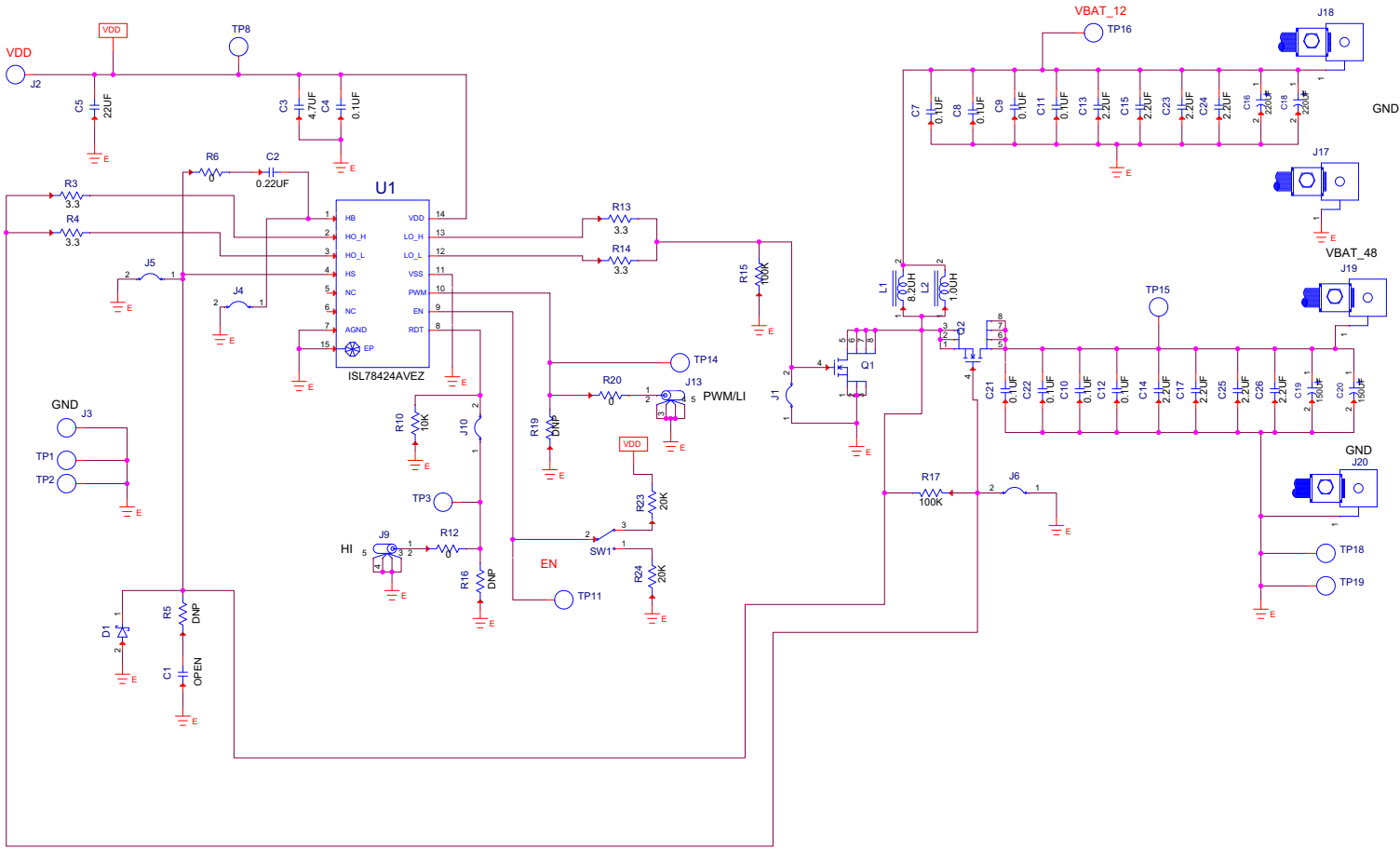
Figure 5. ISL78424EVAL3Z Schematic
