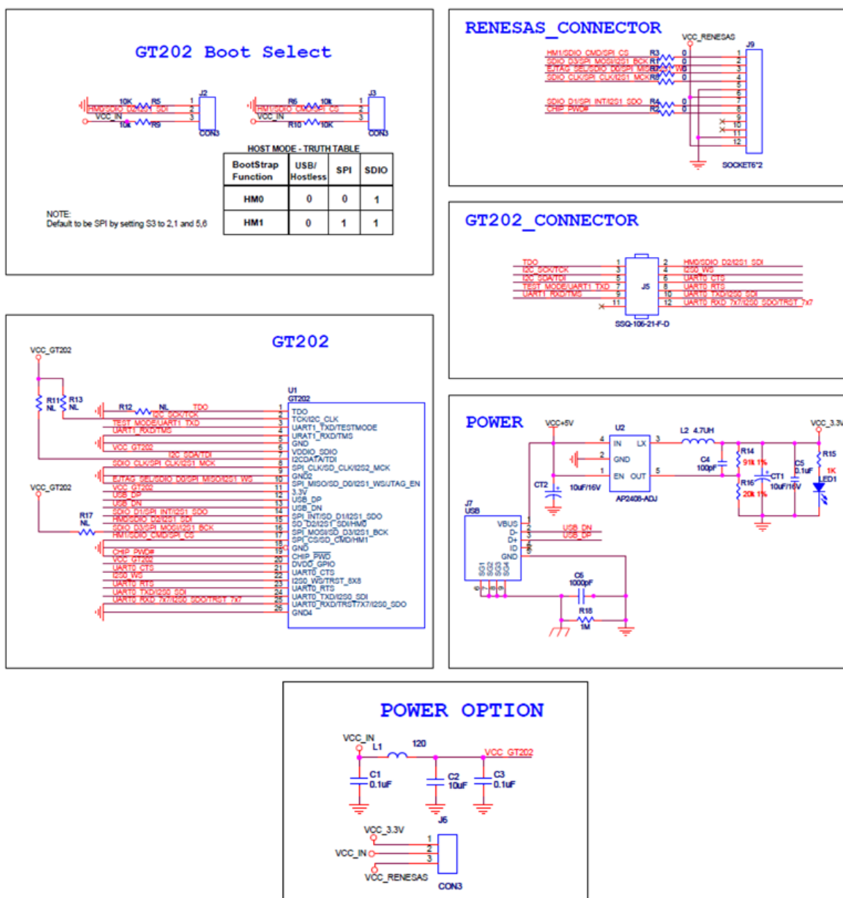
Figure 18 Wi-Fi Board Schematic
