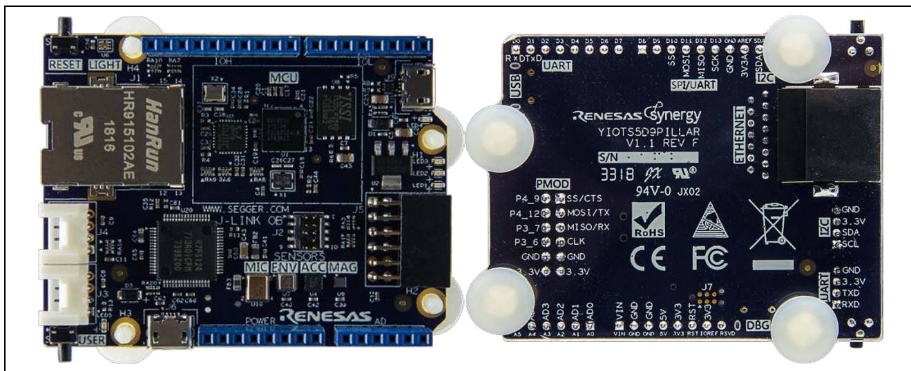
Figure 7 MCU Board
