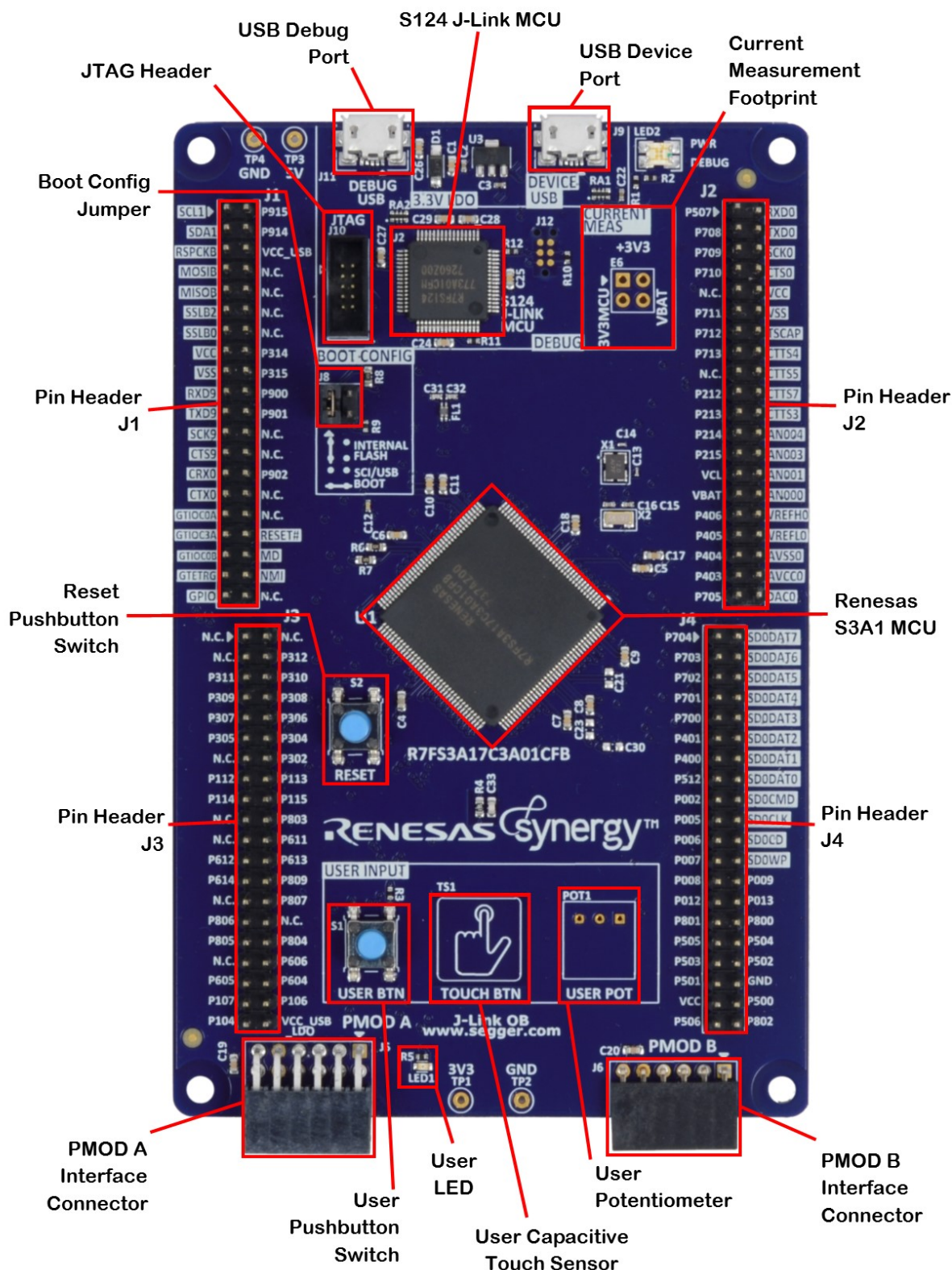
Figure 1. TB-S3A1 Top Side
