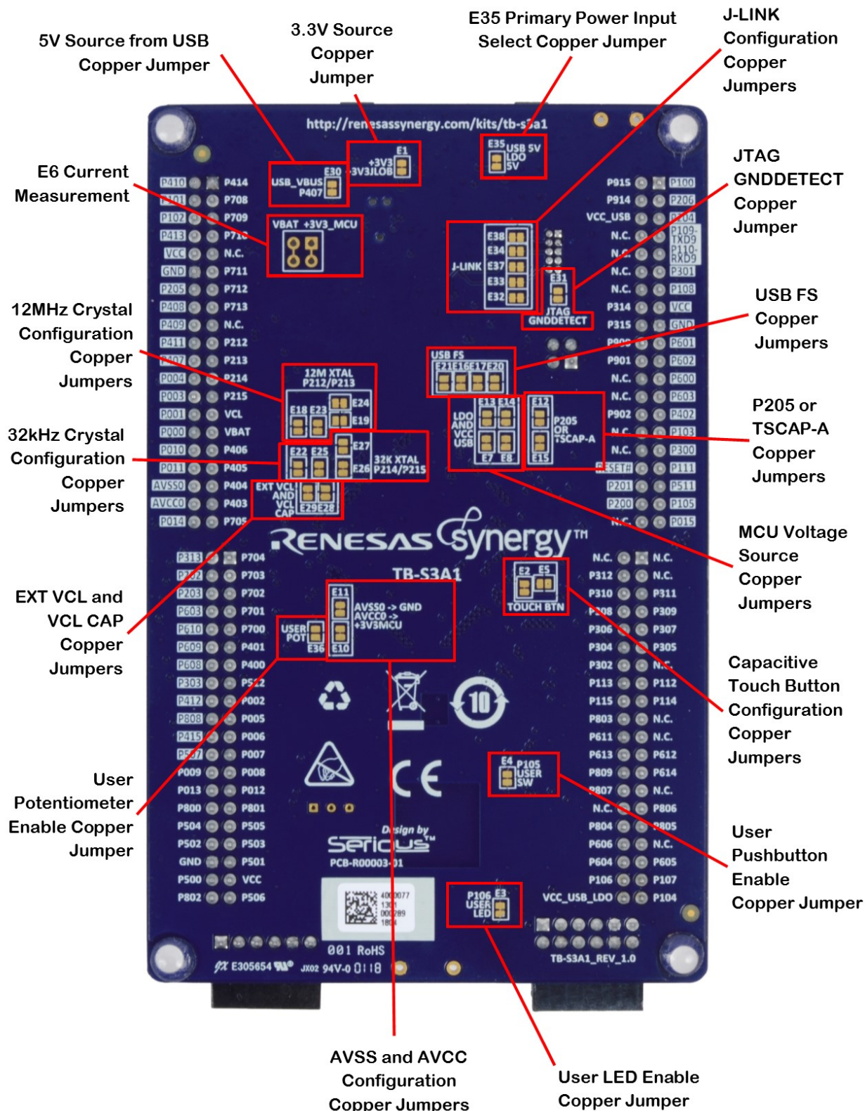
Figure 2. TB-S3A1 Bottom Side
