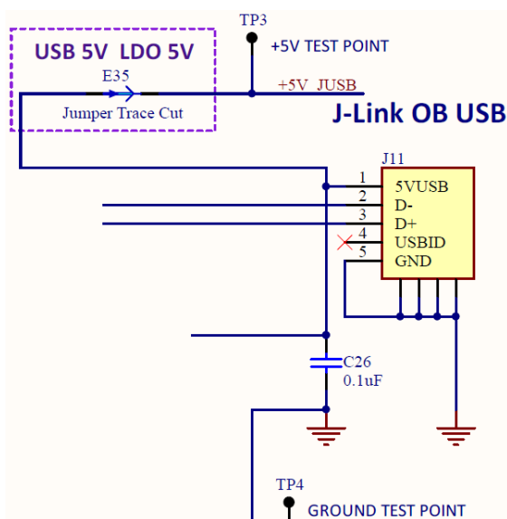
Figure 8. 5 V Power Input Circuit
