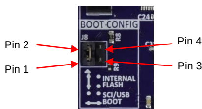
Figure 31. Boot Config Jumper J8
