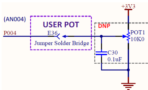
Figure 29. User Potentiometer Circuit
