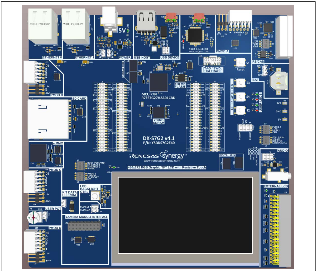
Figure 1 DK-S7G2 Board
