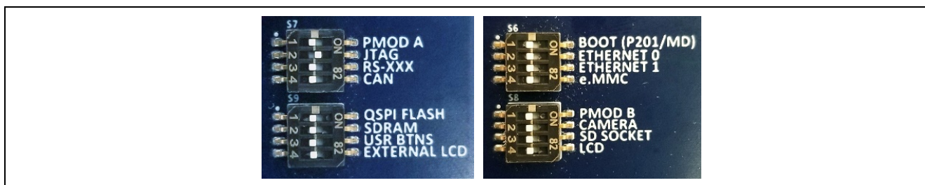
Figure 2 DIP Switch Settings
