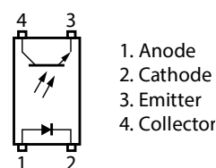
PIN CONNECTION (Top View)
