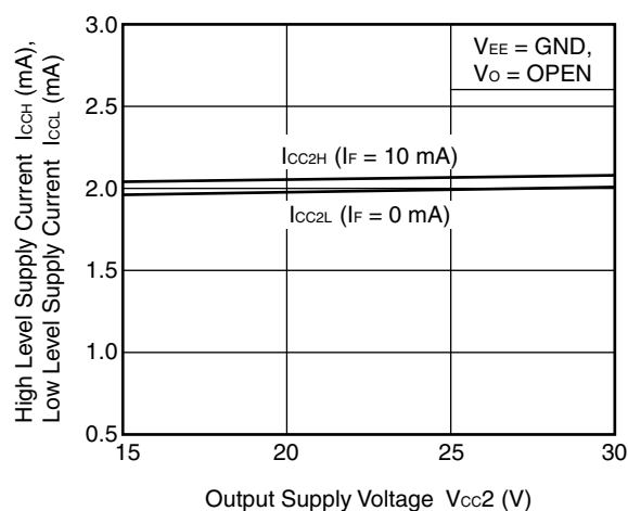
HIGH LEVEL SUPPLY CURRENT, LOW LEVEL SUPPLY CURRENT vs. OUTPUT SUPPLY VOLTAGE
