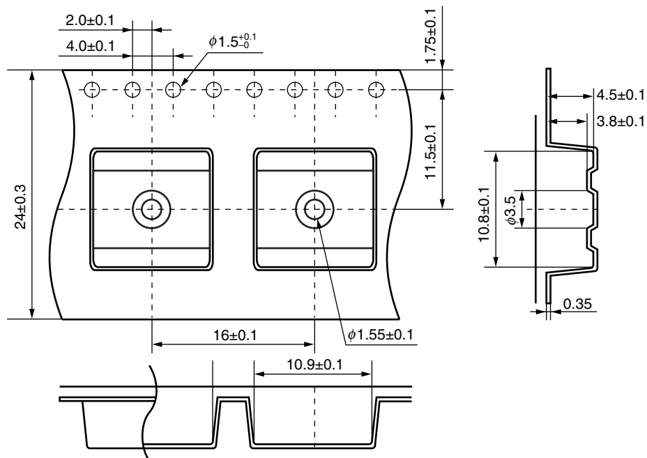
Outline and Dimensions (Tape)
