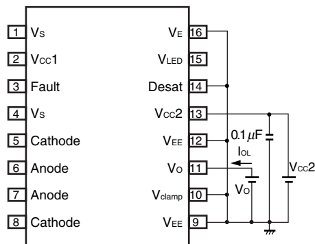
Fig. 4 I_{OL} Test Circuit
