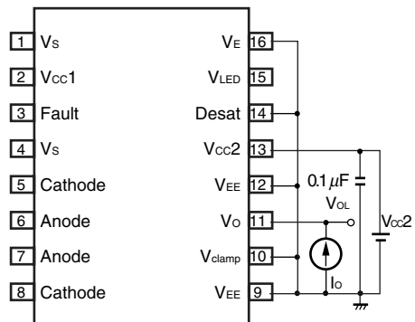
Fig. 6 V_{OL} Test Circuit
