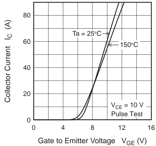
Transfer Characteristics (Typical)
