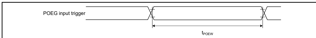
Figure 51.48 POEG input trigger timing
