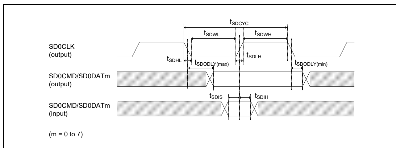
Figure 51.75 SD/MMC host interface signal timing
