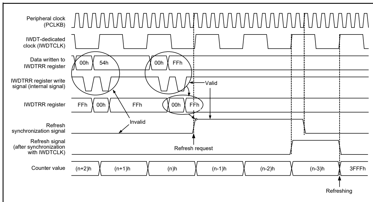
Figure 27.4 IWDTC refresh operation waveforms when OFS0.IWDTCCKS[3:0] = 0000b, OFS0.IWDTTOPS[1:0] = 11b
