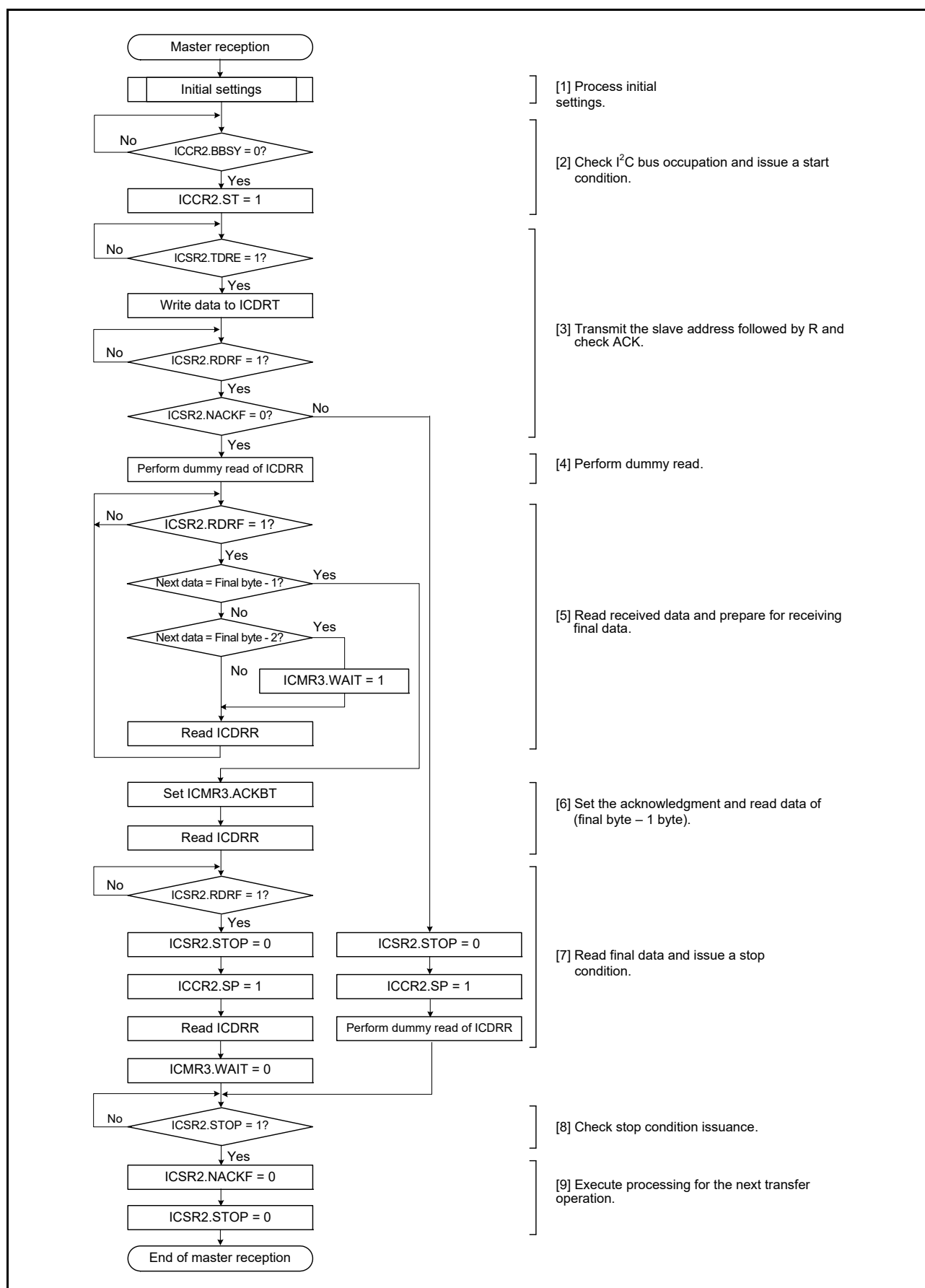
Figure 30.11 Example master reception flow with 7-bit address format and 3 or more bytes
