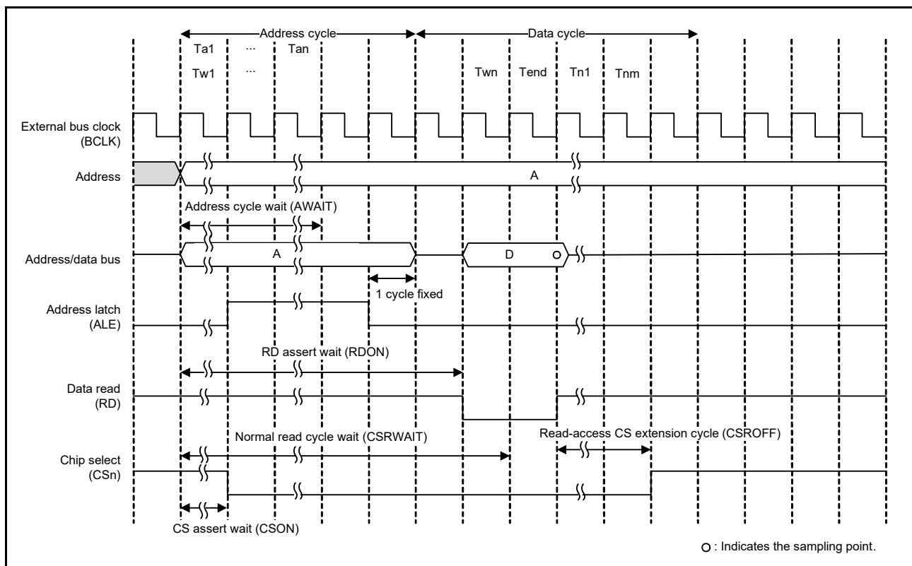
Figure 15.23 Example of read access operation with address/data multiplexed I/O interface (n = 0 to 3)
