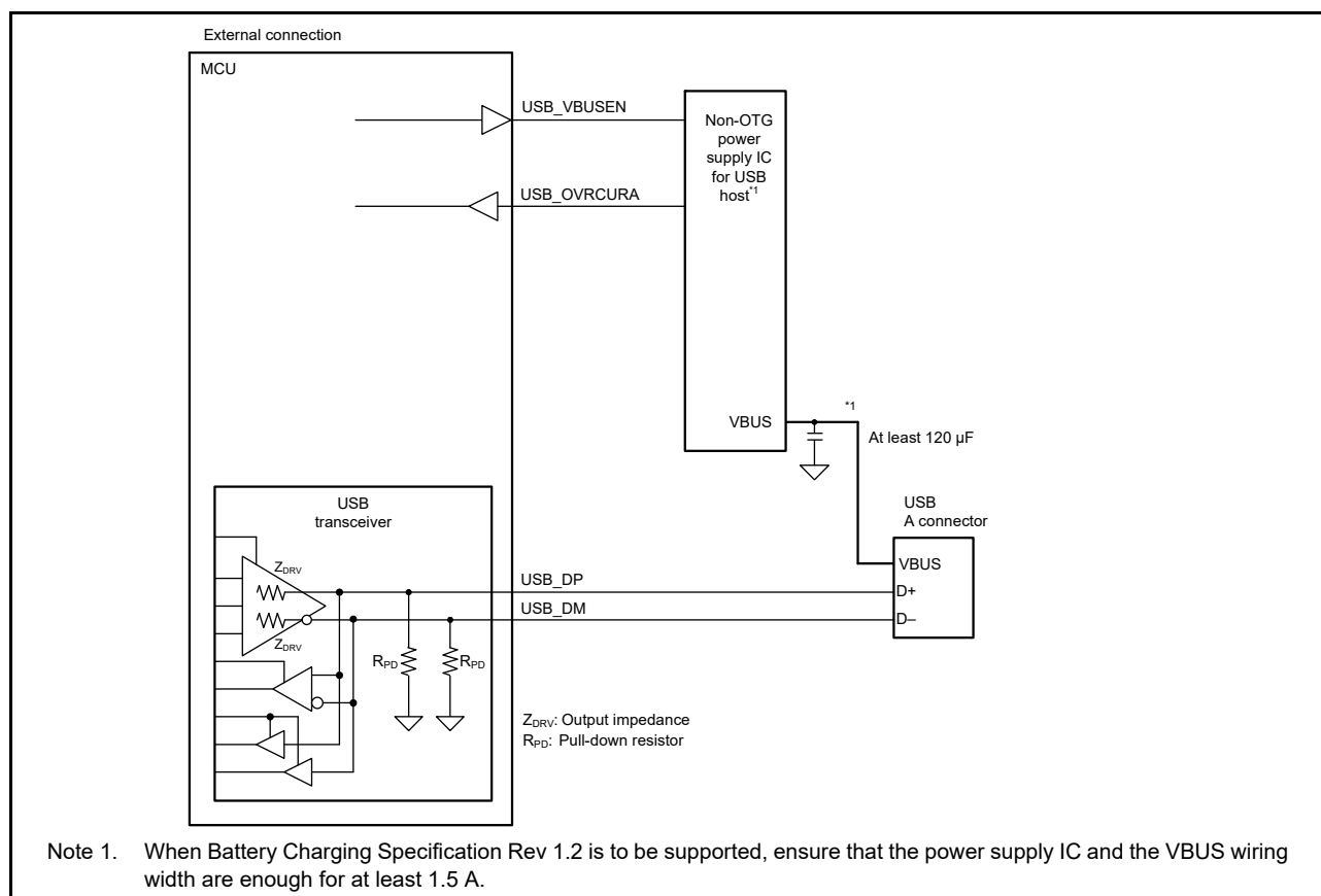
Figure 28.7 Example host connection
