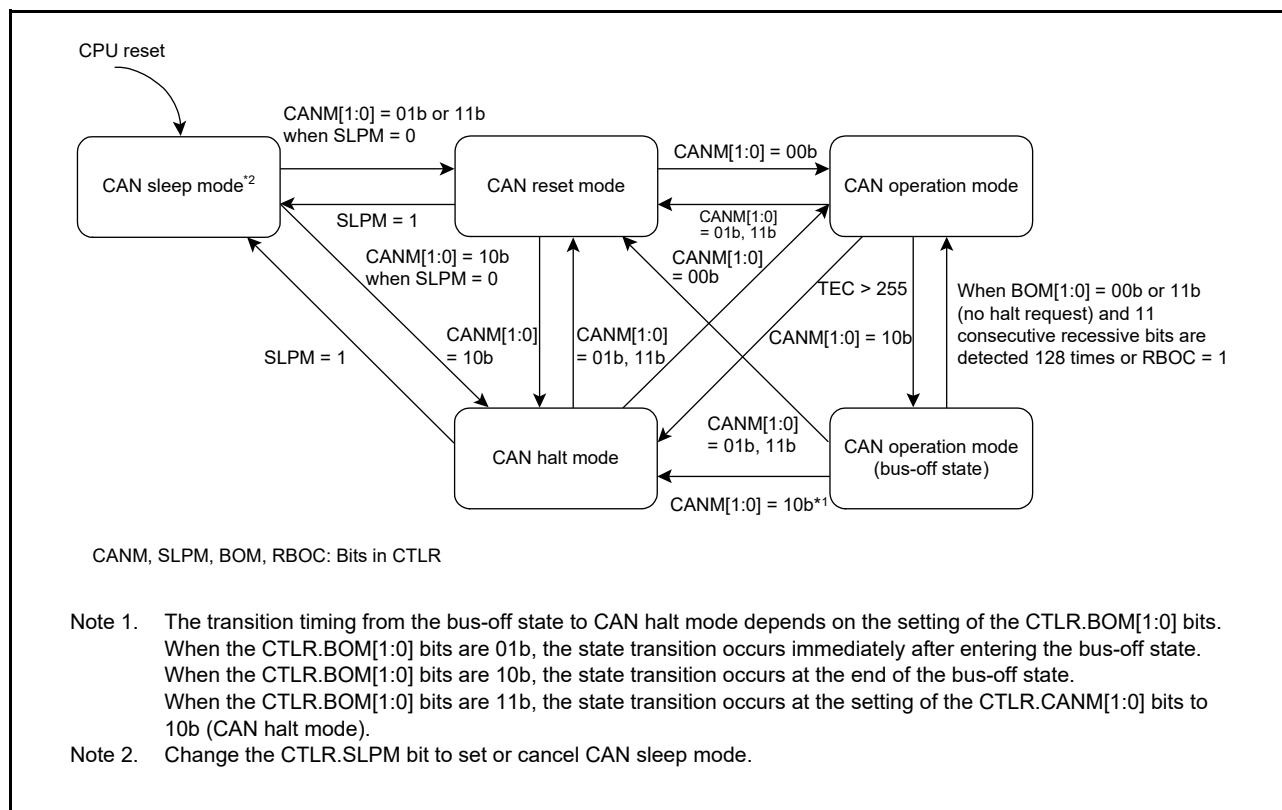
Figure 31.9 Transition between different operation modes
