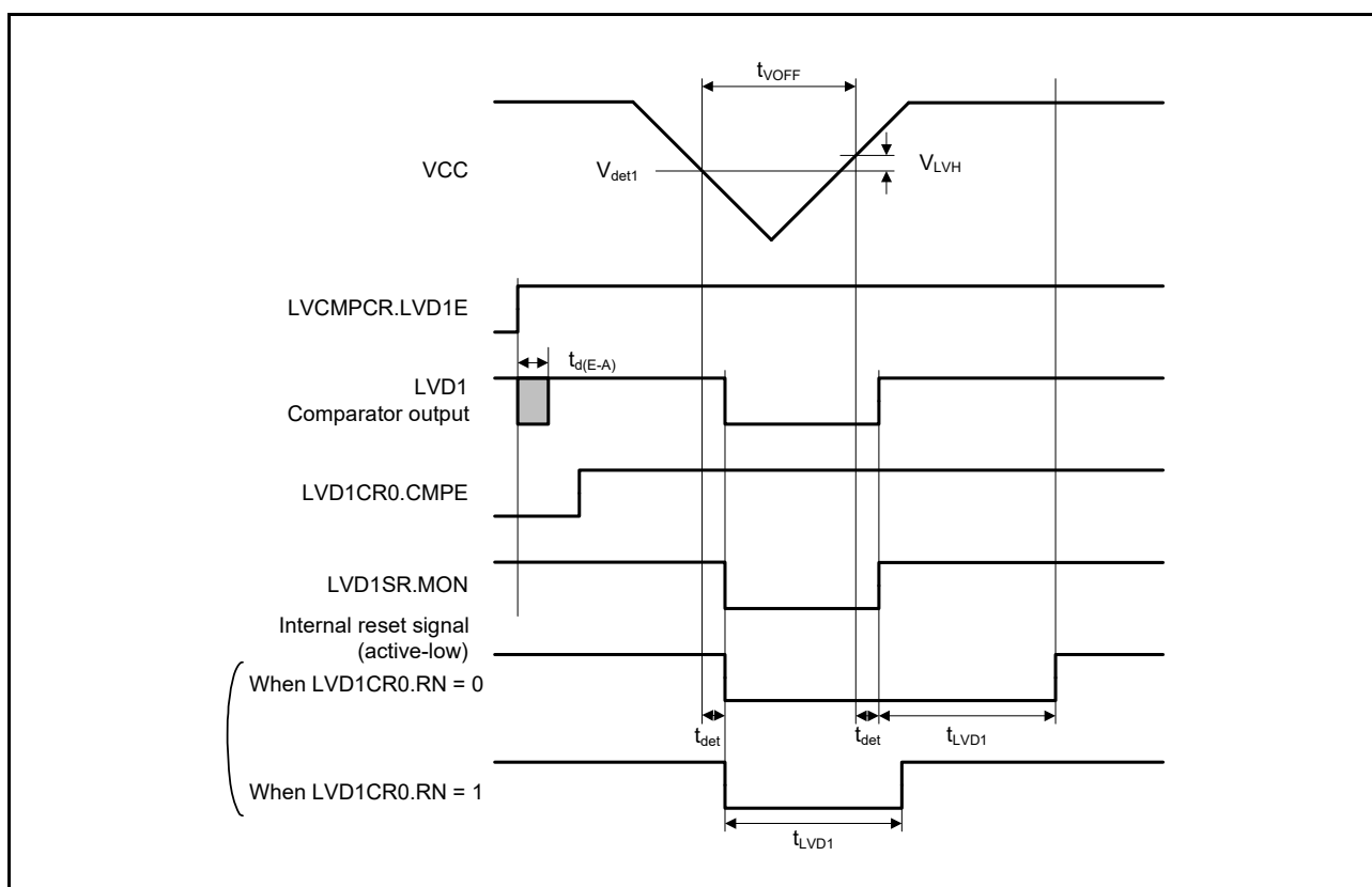
Figure 51.88 Voltage detection circuit timing (V det1 )
