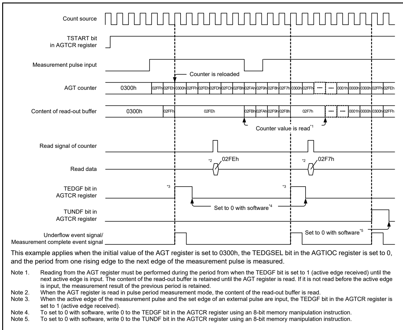
Figure 24.10 Operation example in pulse period measurement mode
