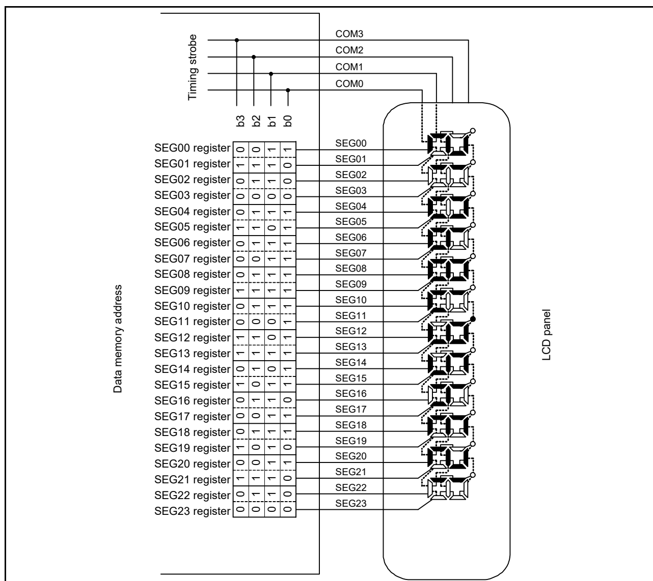
Figure 48.29 Example for connecting four-time-slice LCD panel
