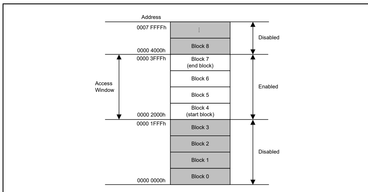
Figure 47.8 Flash area protection overview
