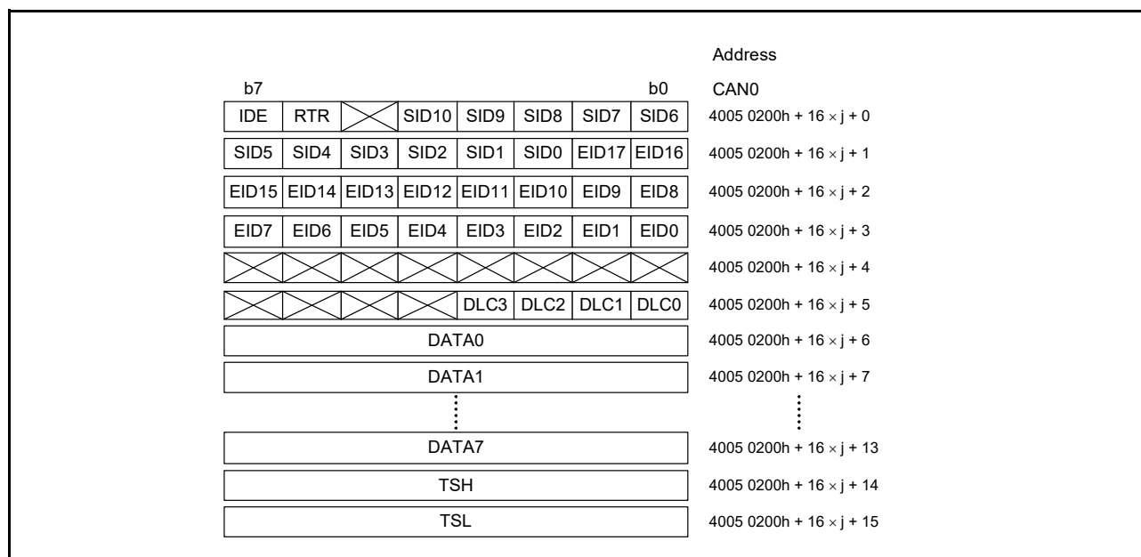
Figure 31.13 Structure of the mailbox registers (j = 0 to 31)
