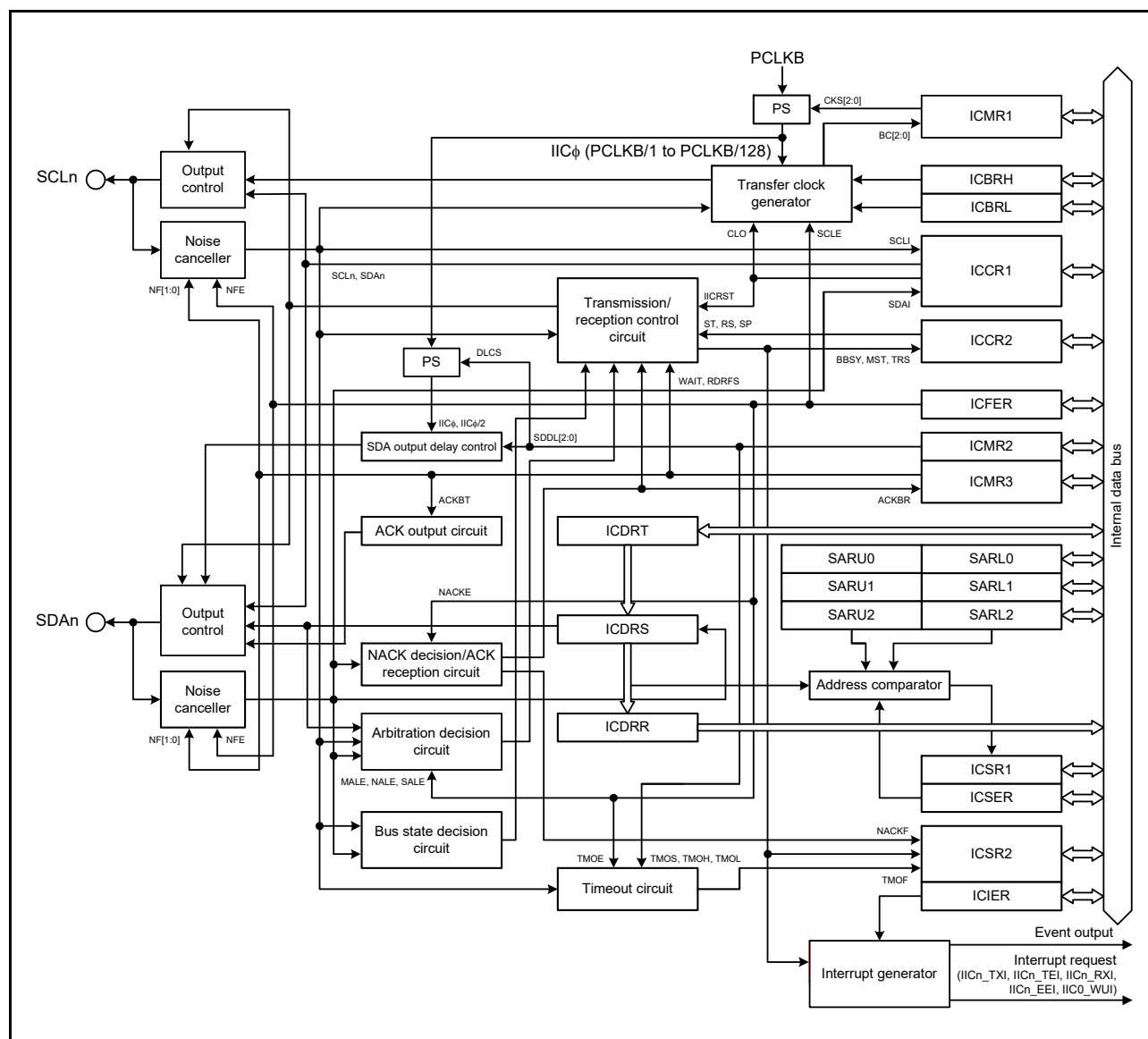
Figure 30.1 IIC block diagram
