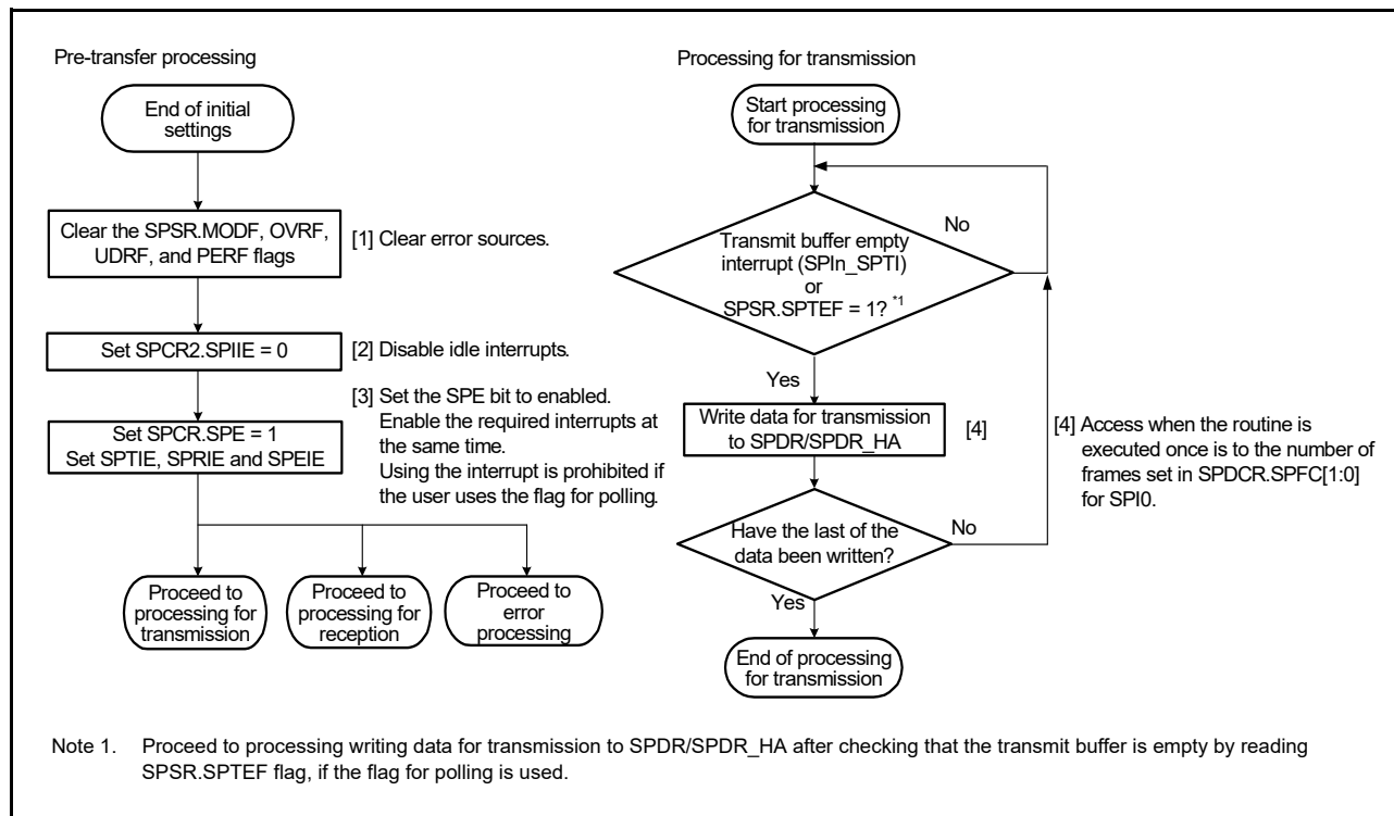
Figure 32.48 Transmission flow in slave mode
