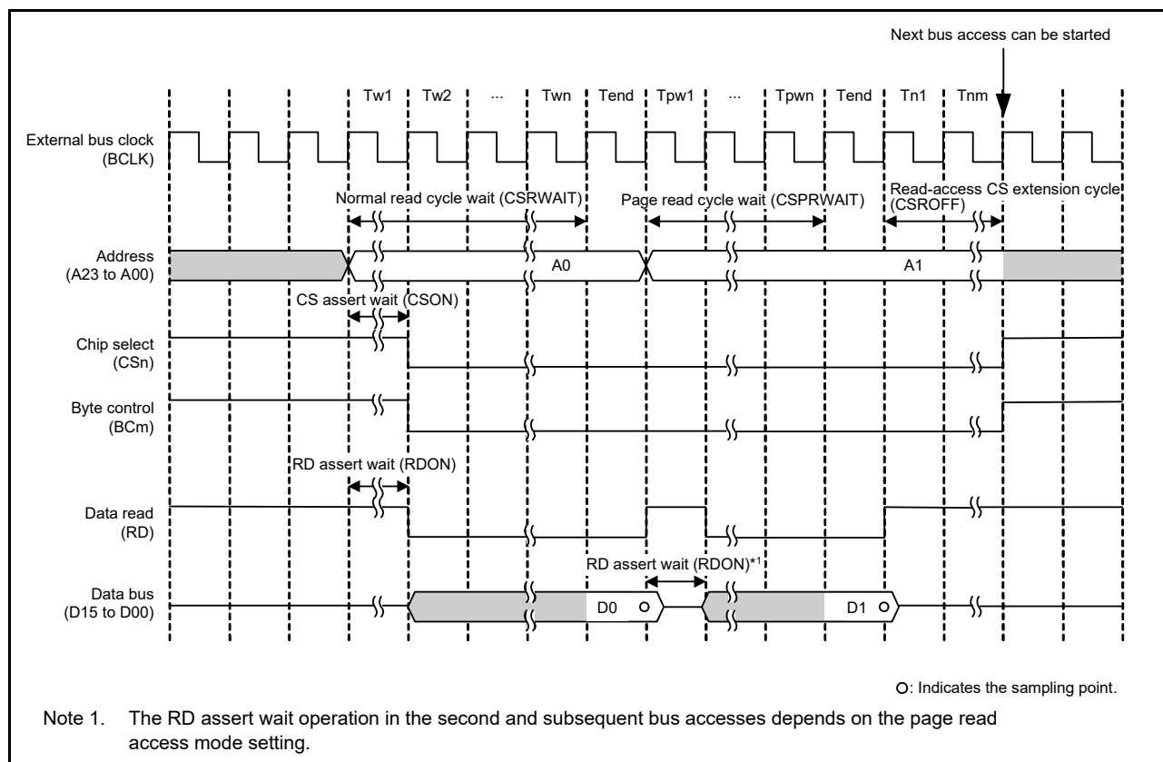
Figure 15.17 Page read access timing (n = 0 to 3; m = 0, 1)
