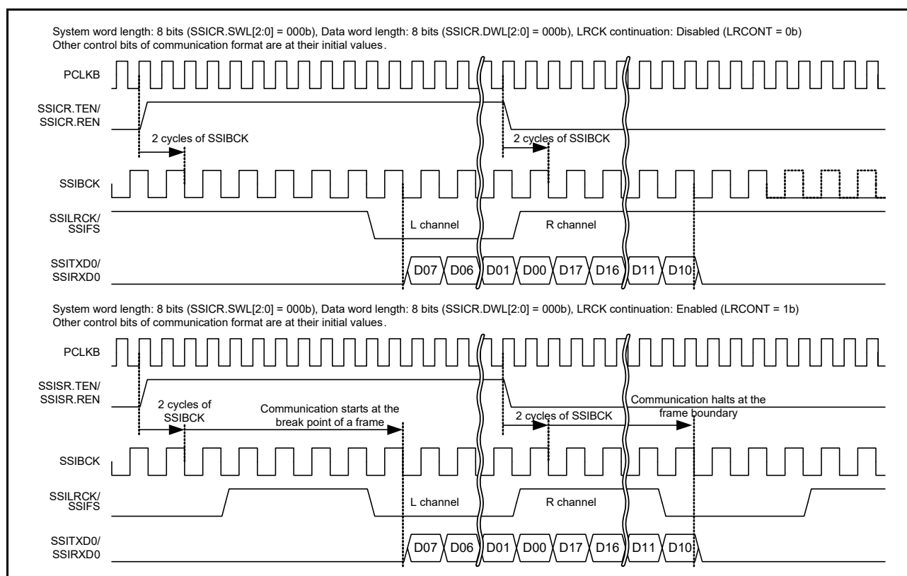
Figure 35.31 Example of LR clock/frame synchronization continuation operation
