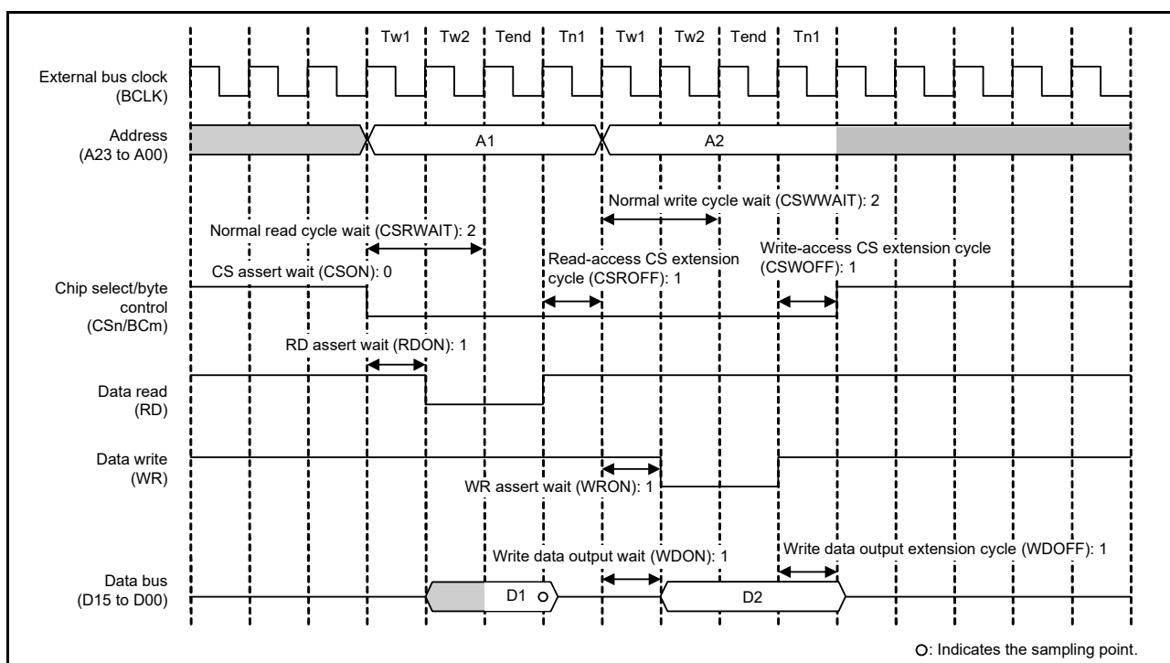
Figure 15.9 Example of normal access operation for read and write ( n = 0 to 3; m = 0, 1 )
