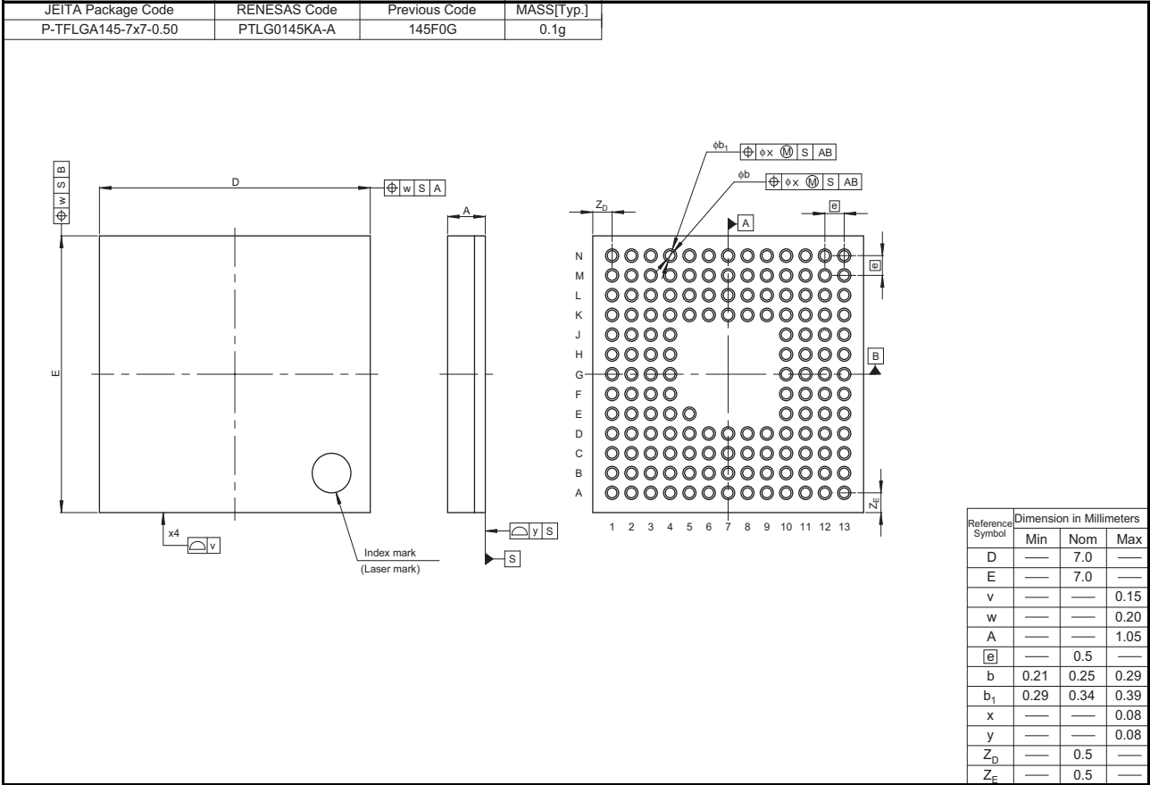
Figure 2.1 LGA 145-pin
