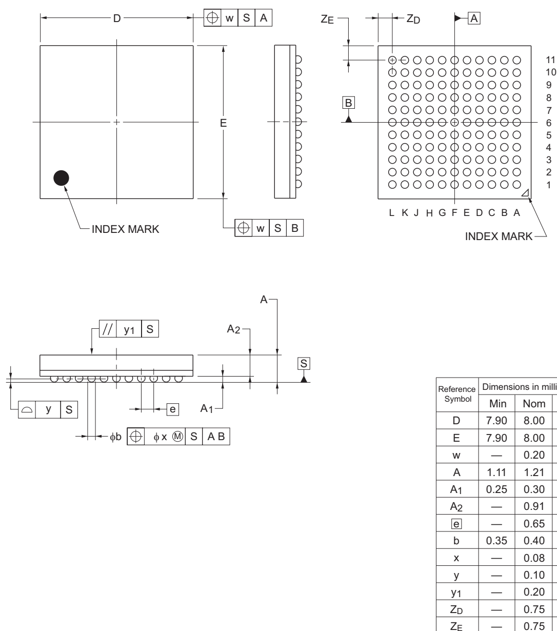
Figure 2.3 BGA 121-pin
