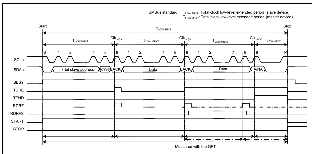
Figure 30.50 SMBus timeout measurement
