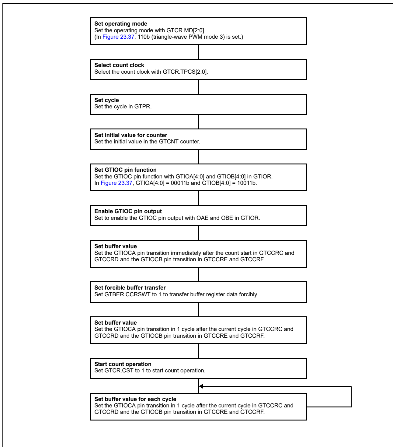
Figure 23.38 Example for setting triangle-wave PWM mode 3
