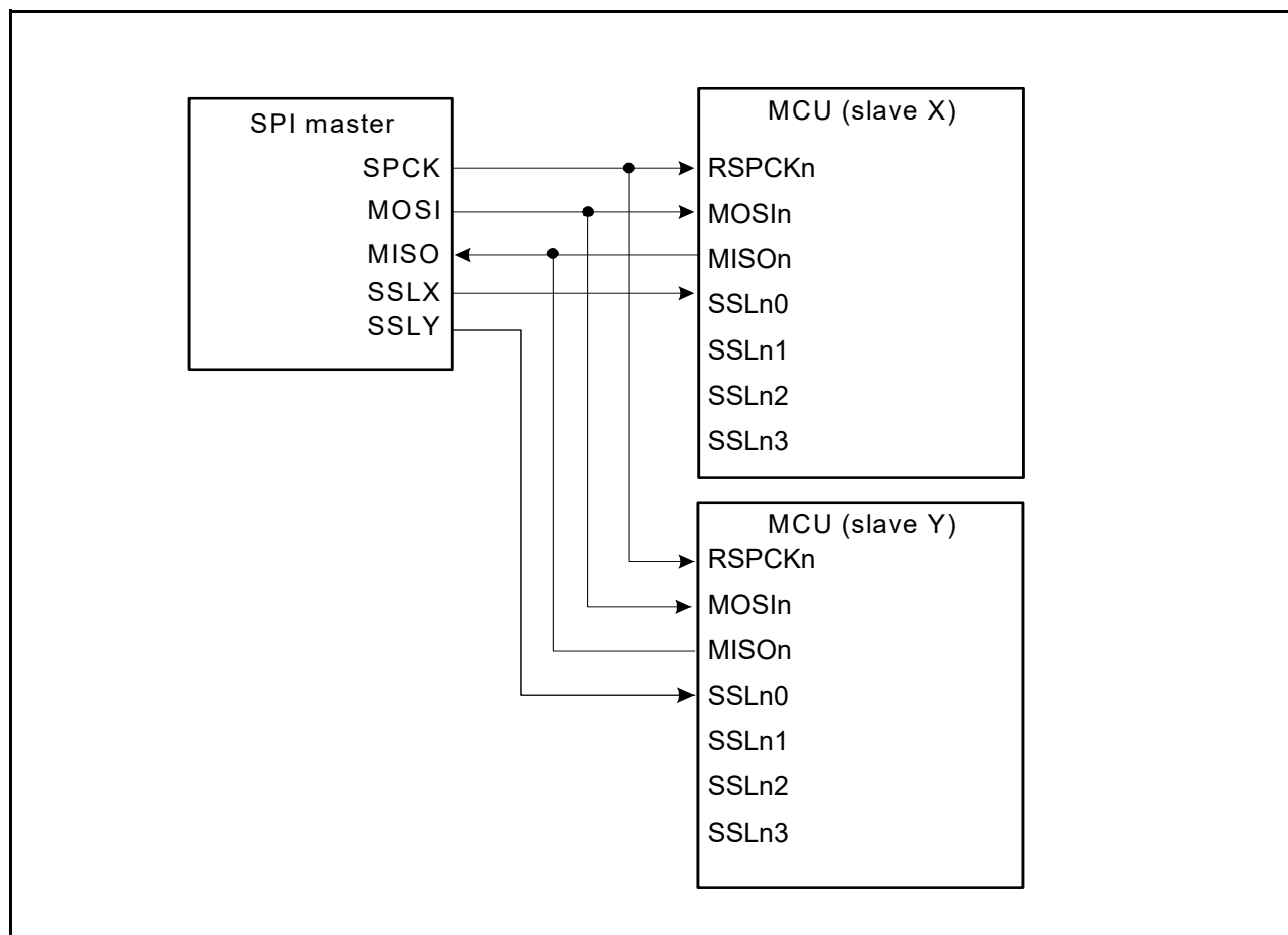
Figure 32.12 Single-master/multi-slave configuration example with the MCU as slave
