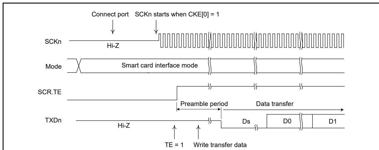
Figure 29.51 Example timing of data transmission in smart card interface mode
