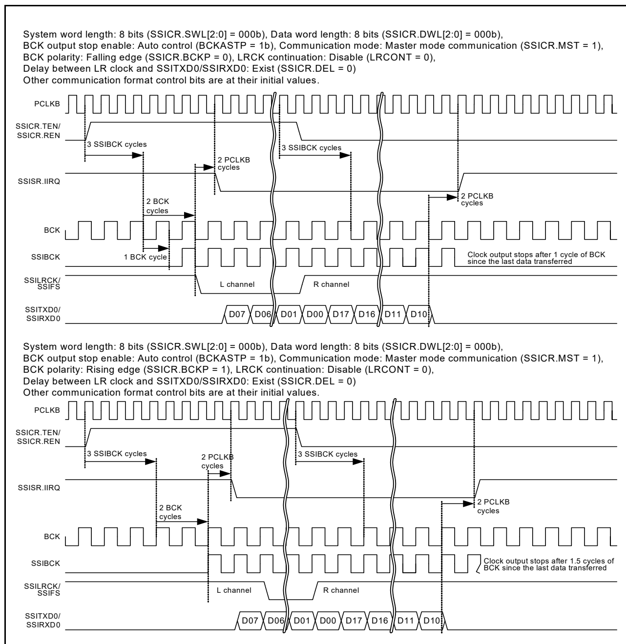
Figure 35.33 Example operation of the BCKASTP bit communication with BCKASTP = 1
