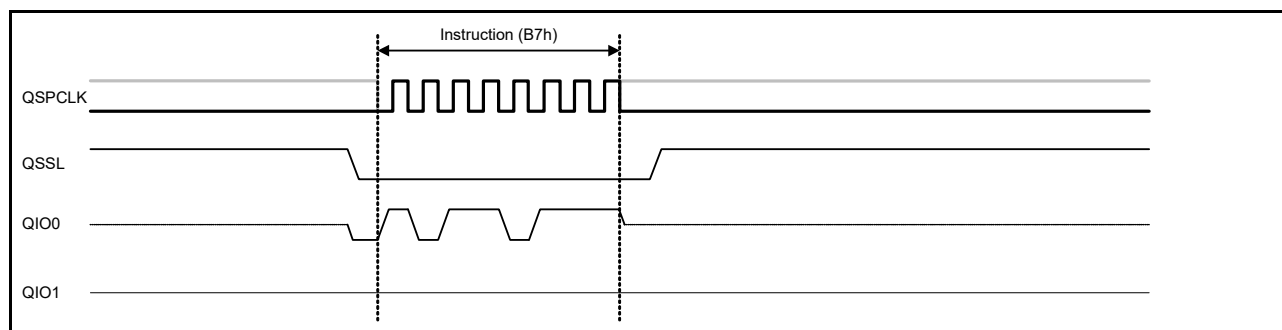
Figure 33.27 Bus cycle for enter 4-byte mode instruction
