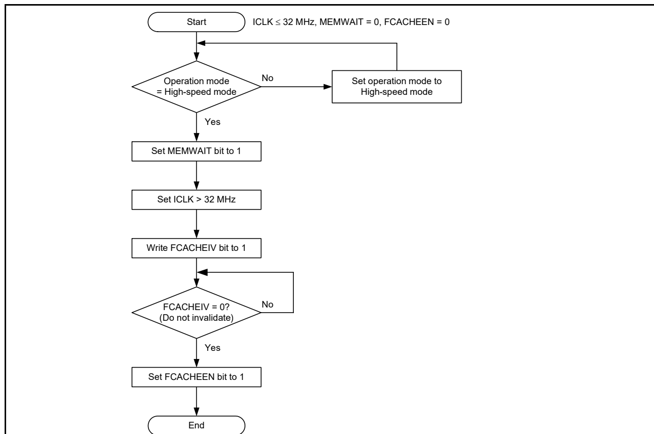
Figure 9.2 When setting the ICLK > 32 MHz
