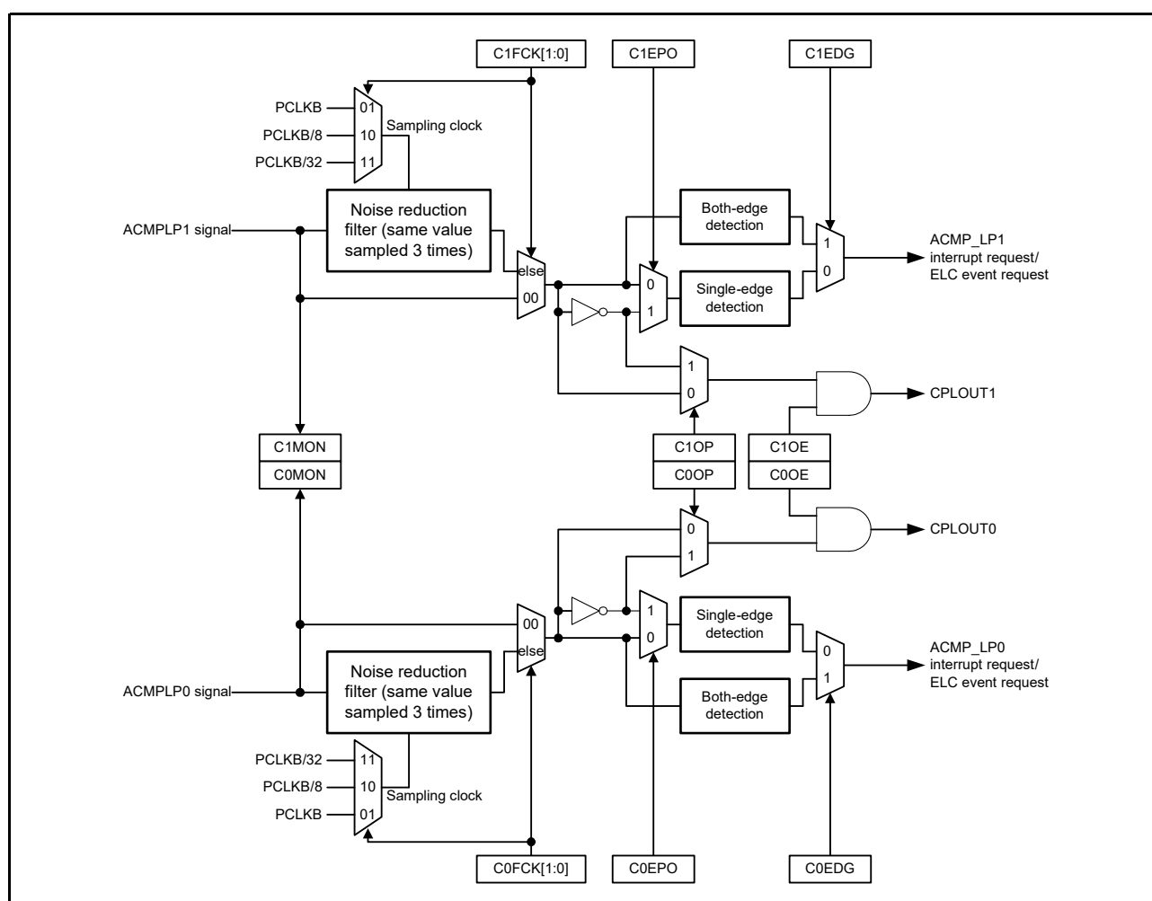
Figure 42.5 Noise filter and edge detection configuration
