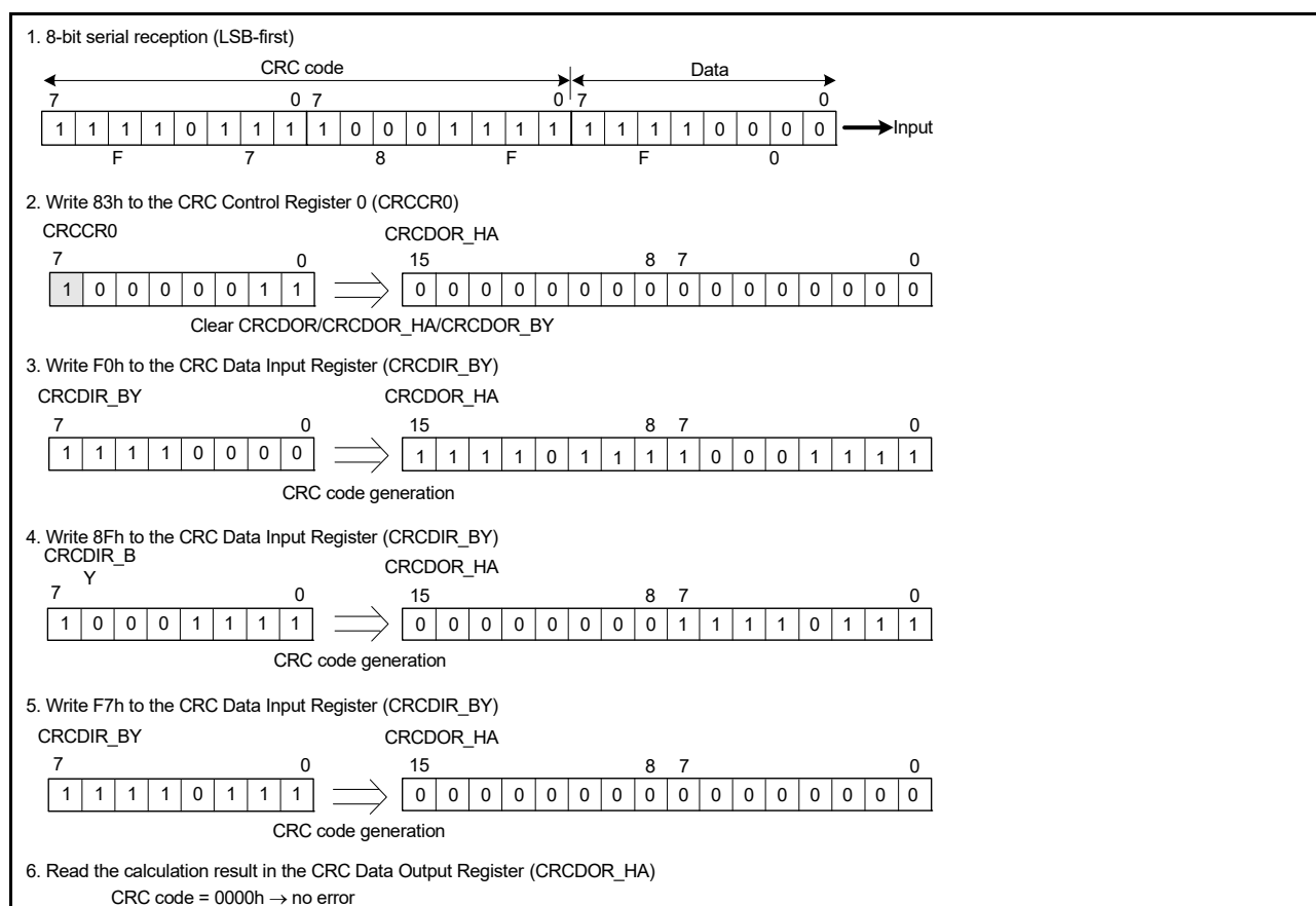
Figure 34.4 LSB-first data reception
