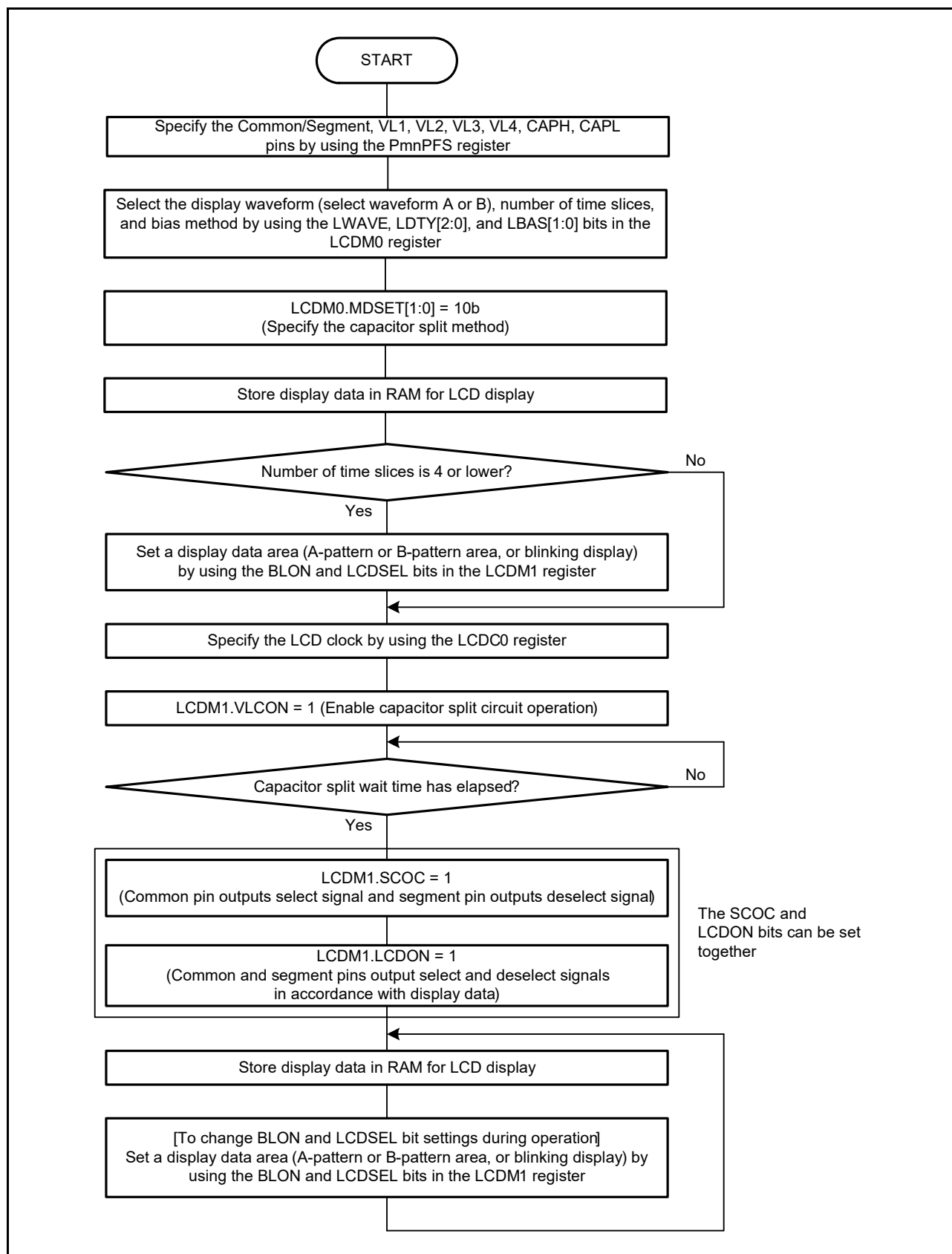
Figure 48.7 Setting procedure for capacitor split method during normal liquid crystal waveform display
