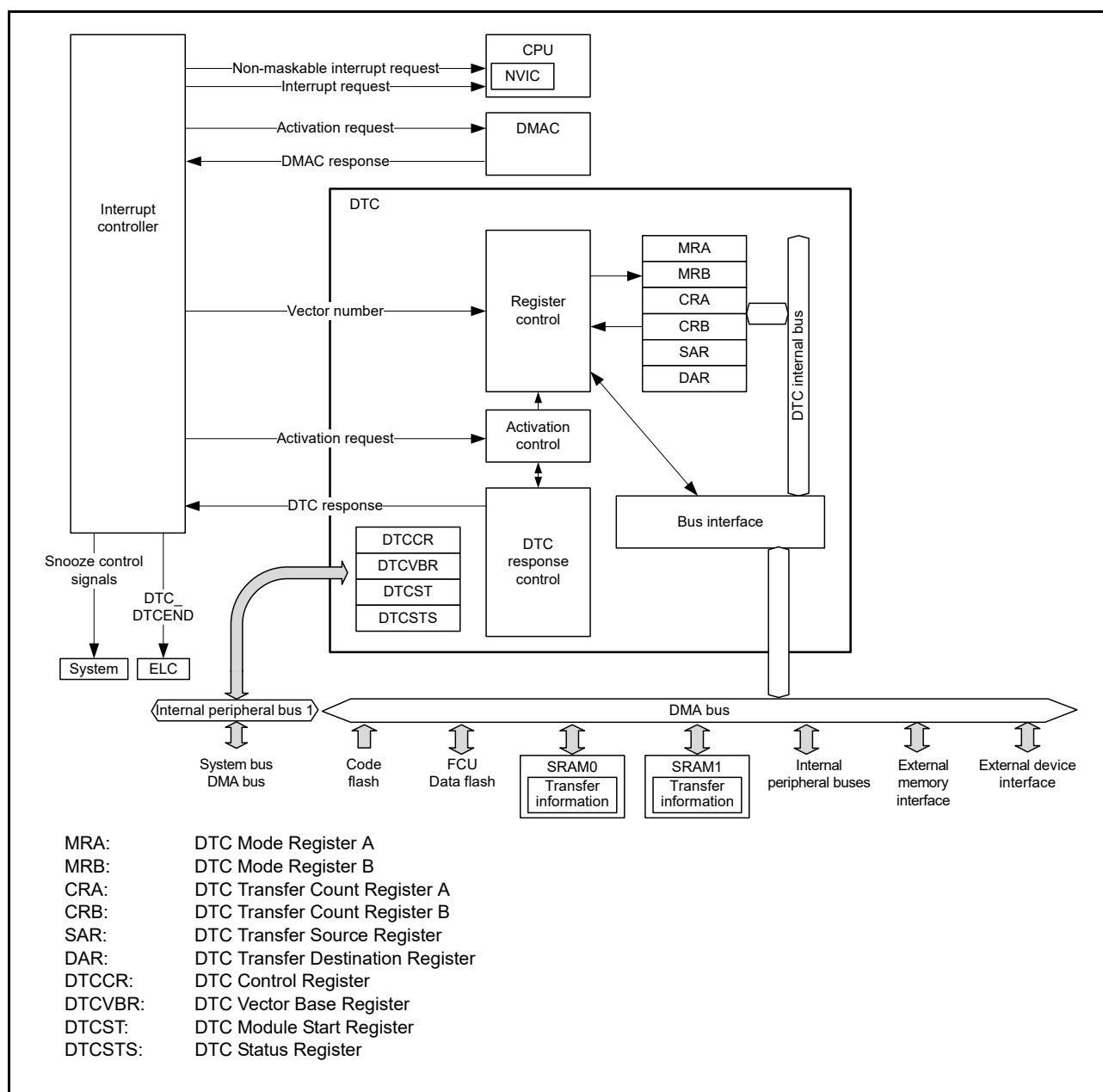
Figure 18.1 DTC block diagram
