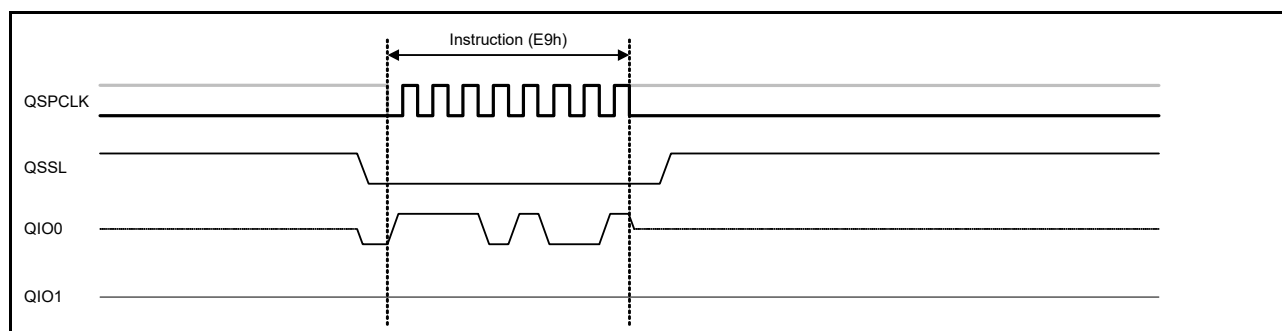
Figure 33.28 Bus cycle for exit 4-byte mode instruction
