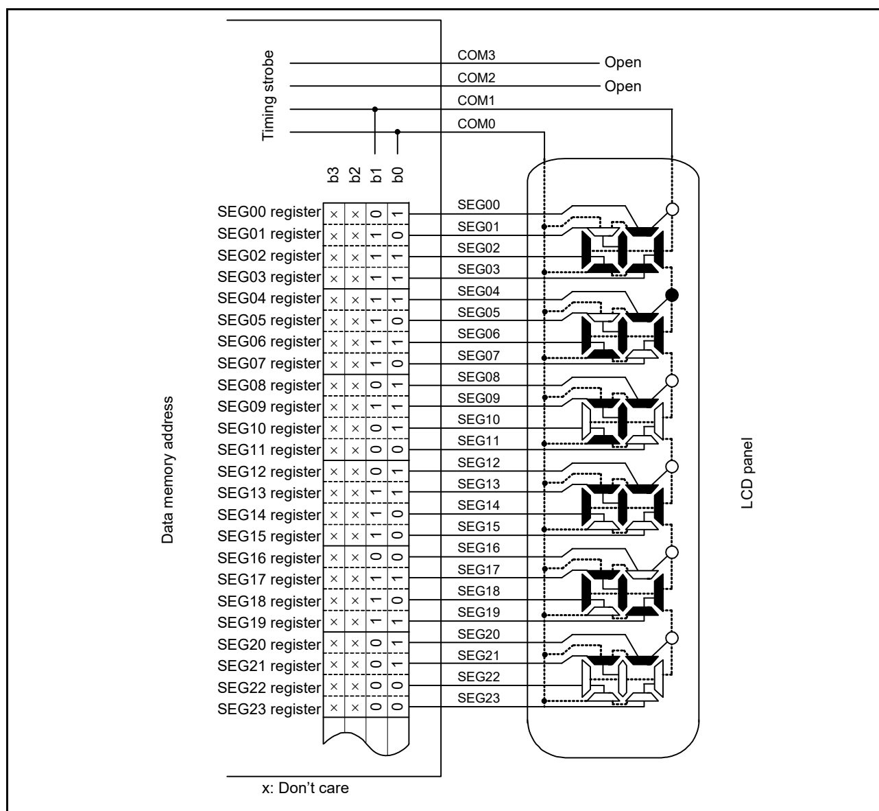
Figure 48.22 Example of connecting two-time-slice LCD panel
