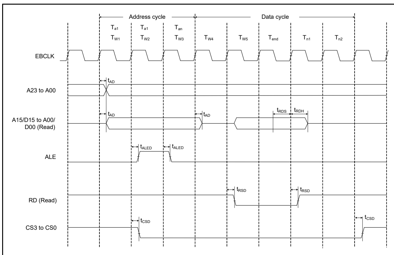
Figure 51.40 Address/data multiplexed bus read access timing
