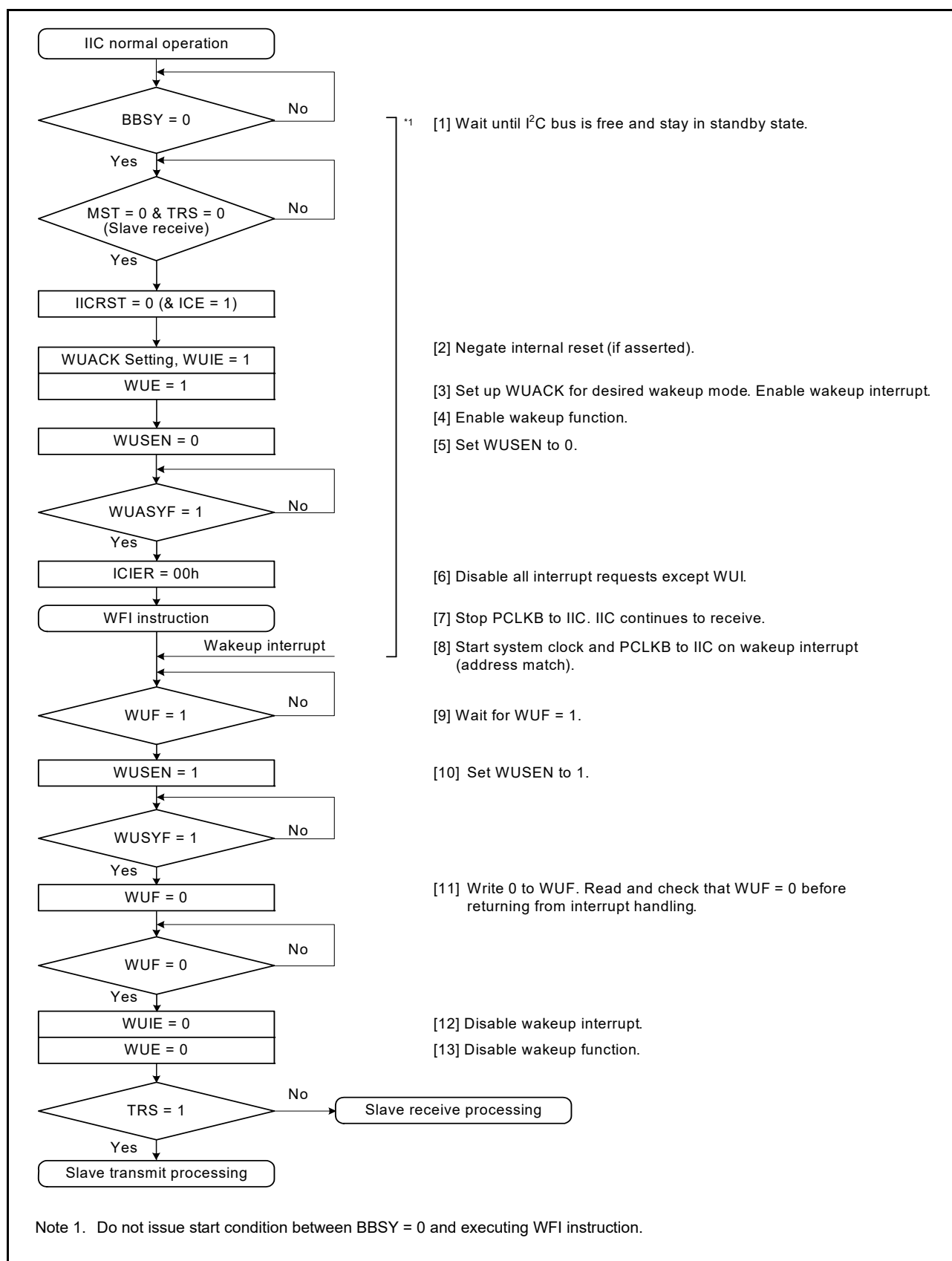
Figure 30.30 Example operation of normal wakeup mode 1 when wakeup is triggered by a wakeup interrupt on match of the slave address
