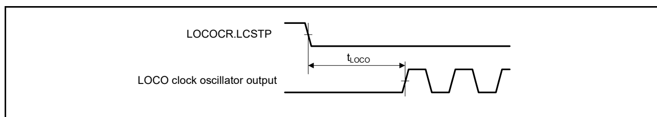
Figure 51.28 LOCO clock oscillator start timing
