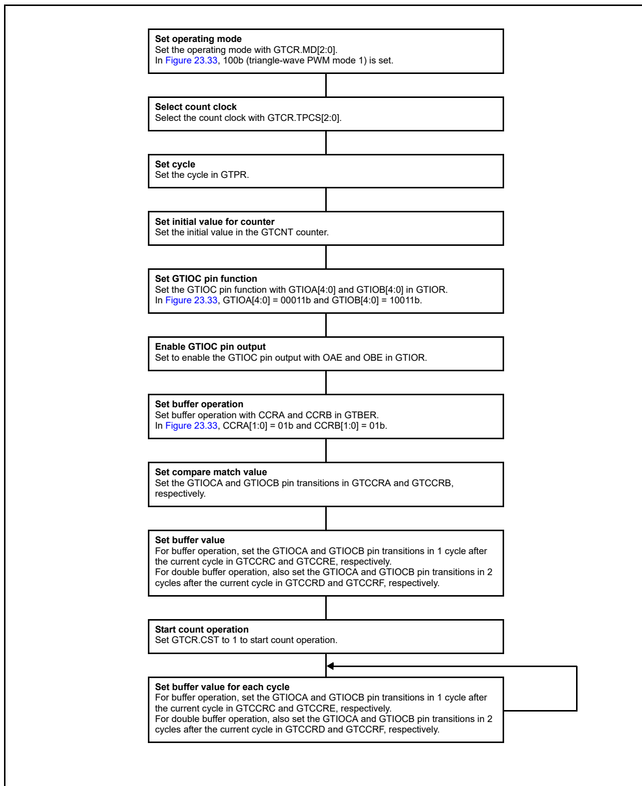
Figure 23.34 Example for setting triangle-wave PWM mode 1
