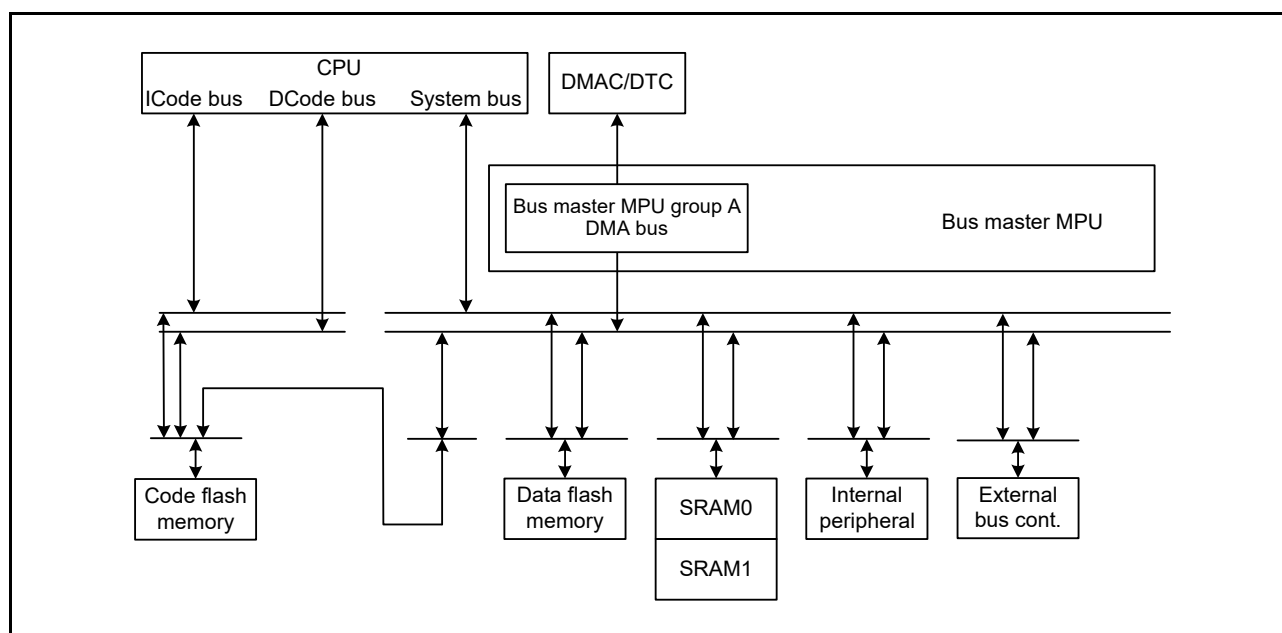
Figure 16.3 Bus master MPU block diagram
