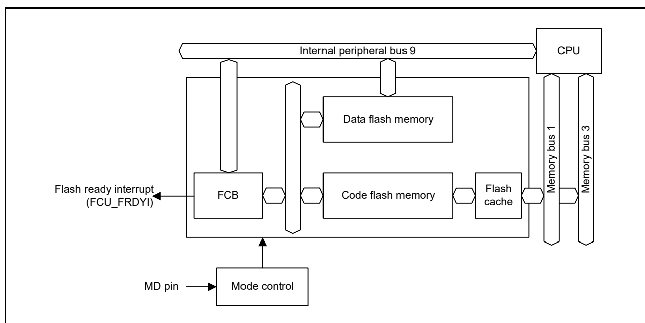
Figure 47.1 Flash memory-related modules block diagram
