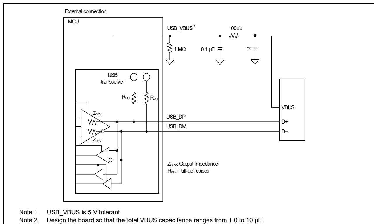
Figure 28.6 Example device connection in self-powered state
