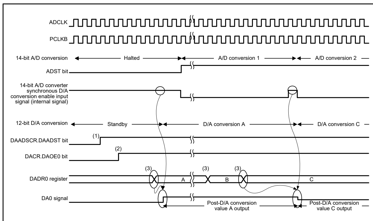
Figure 39.3 Example of conversion when DAC12 is synchronized with ADC14
