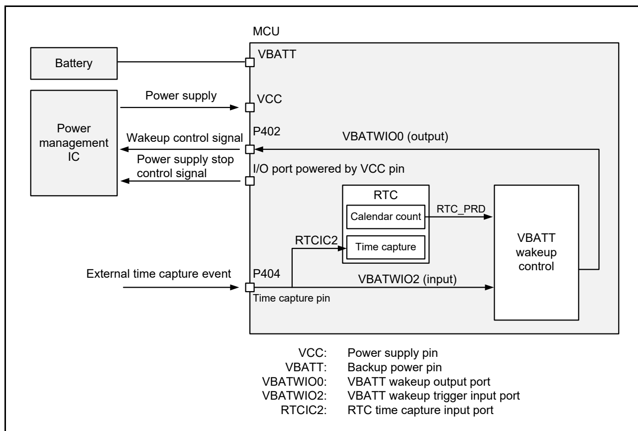
Figure 12.5 VBATT wakeup control function example application
