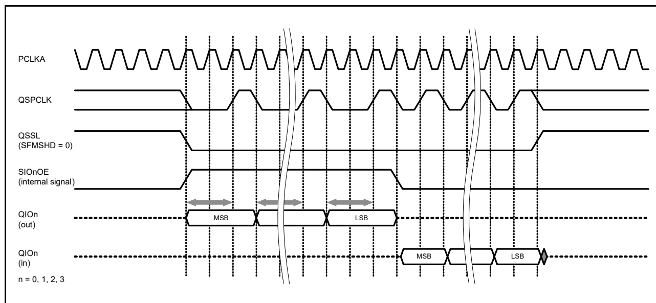
Figure 33.13 Setup time adjustment of serial data output using the SFMOSW bit
