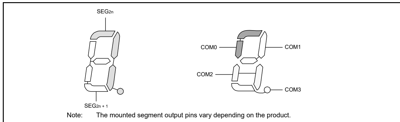
Figure 48.28 Four-time-slice LCD display pattern and electrode connections
