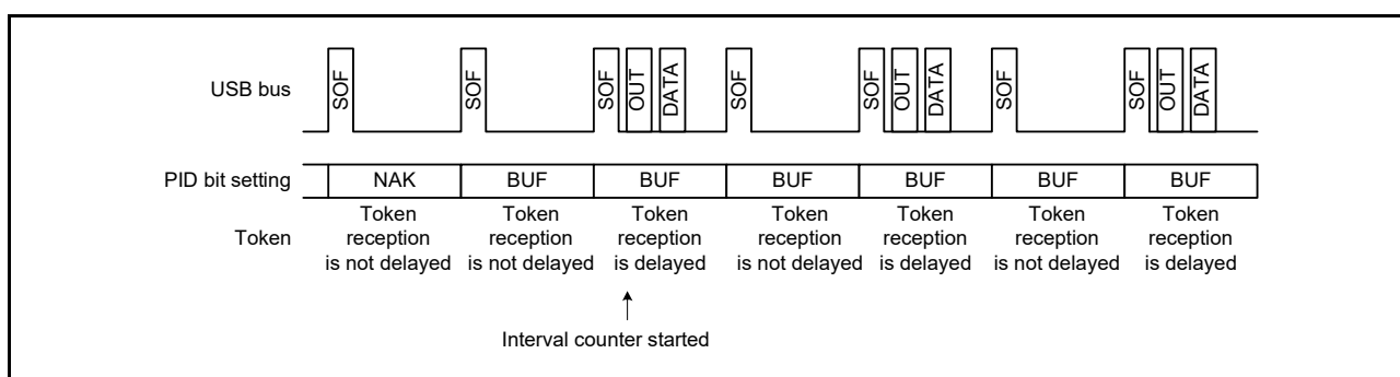
Figure 28.20 Relationship between frames and expected token reception when IITV[2:0] \neq 0
