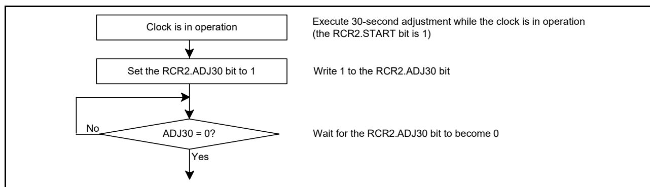
Figure 25.5 30-second adjustment
