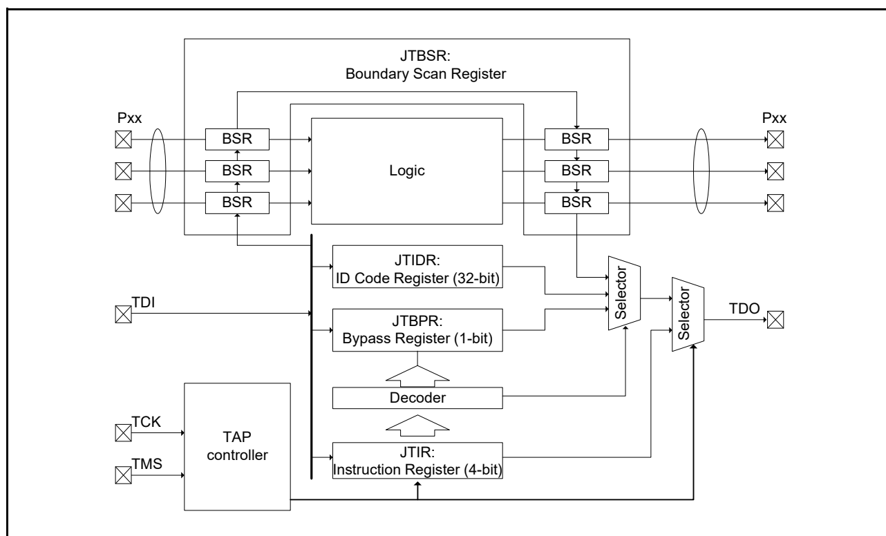
Figure 37.1 Boundary scan function block diagram
