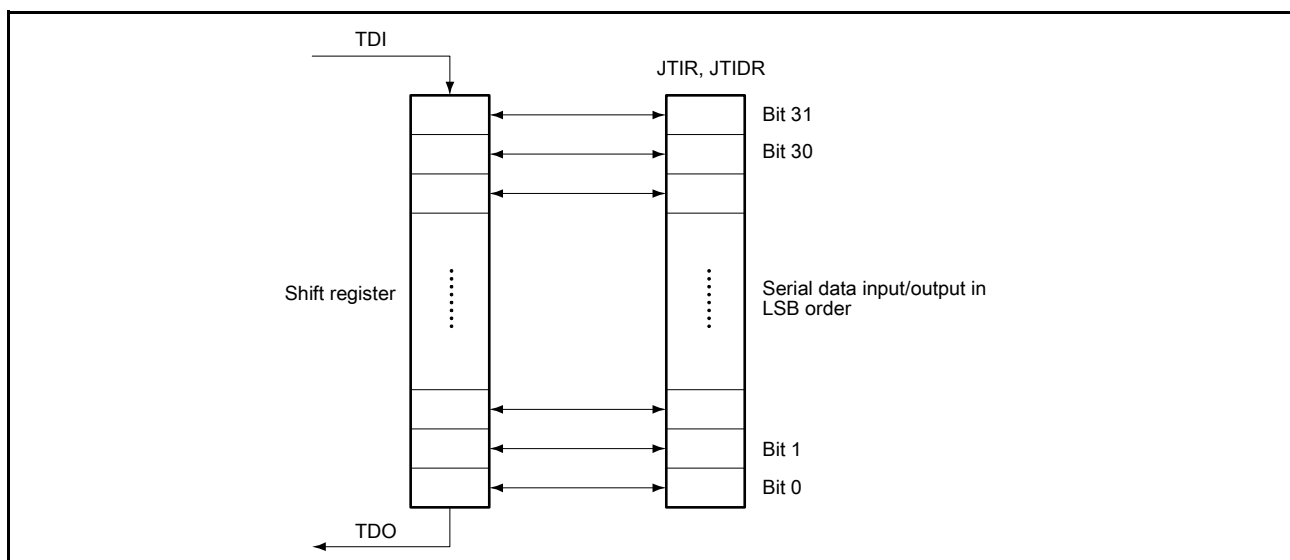
Figure 37.3 Serial data input/output
