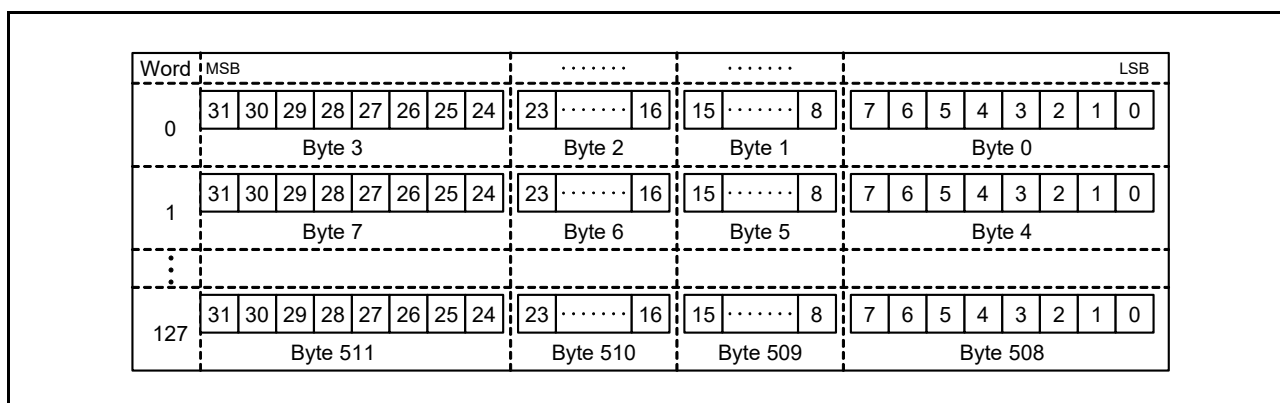
Figure 36.5 SD_BUF data storage
