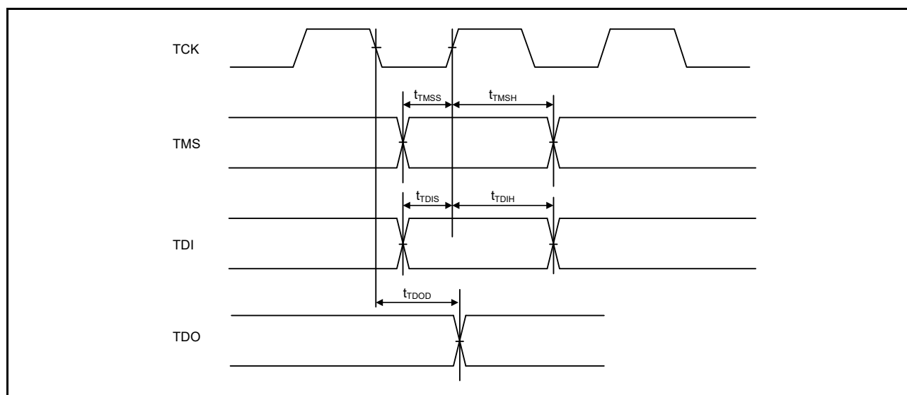
Figure 51.98 JTAG input/output timing
