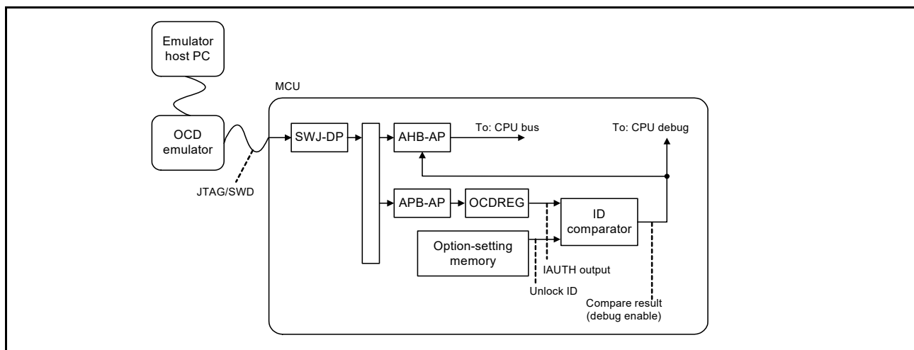
Figure 2.4 Authentication mechanism block diagram
