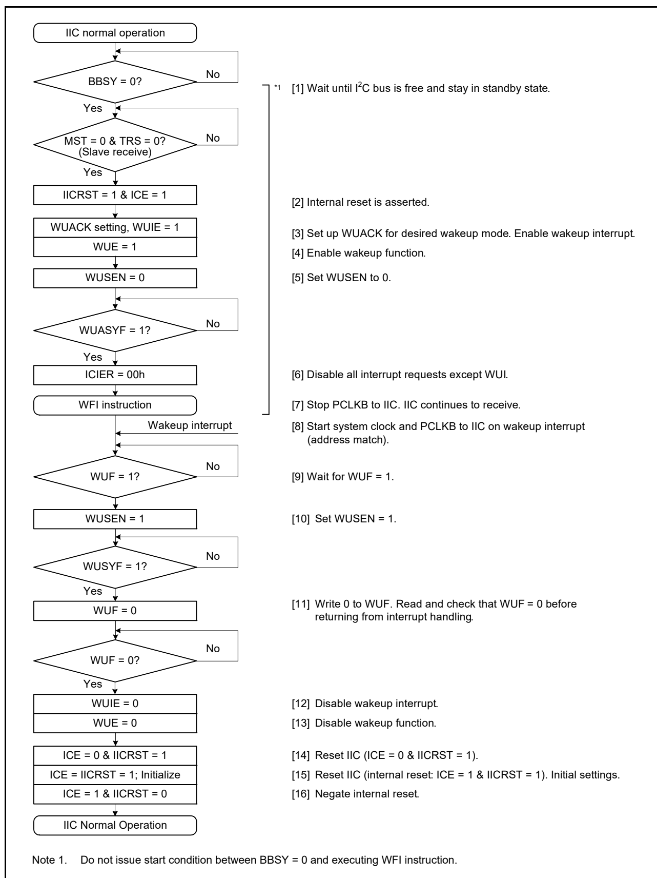
Figure 30.35 Example operation of command recovery and EEPROM response modes when wakeup is triggered by a wakeup interrupt on a match of the slave address
