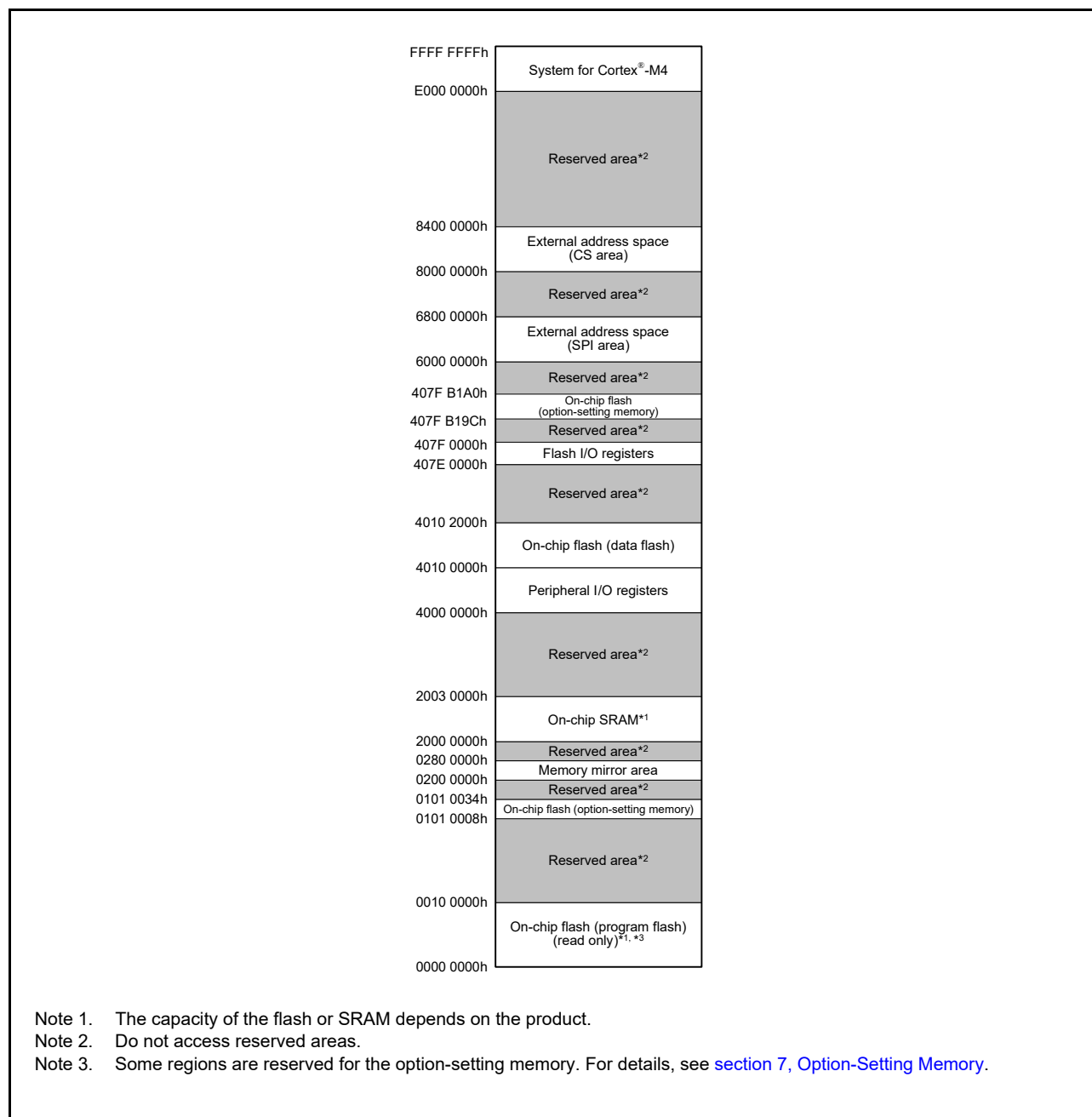
Figure 4.1 Memory map
