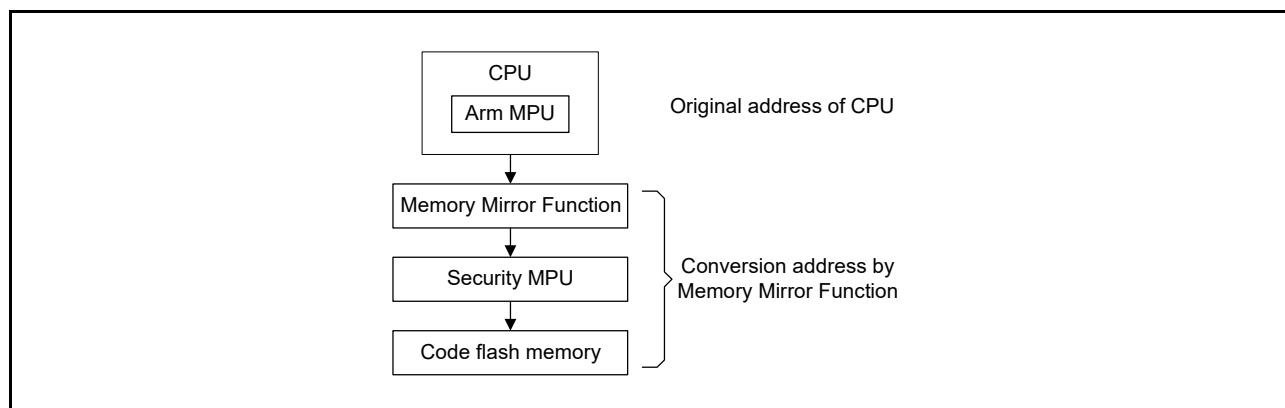
Figure 5.3 MMF address handling
