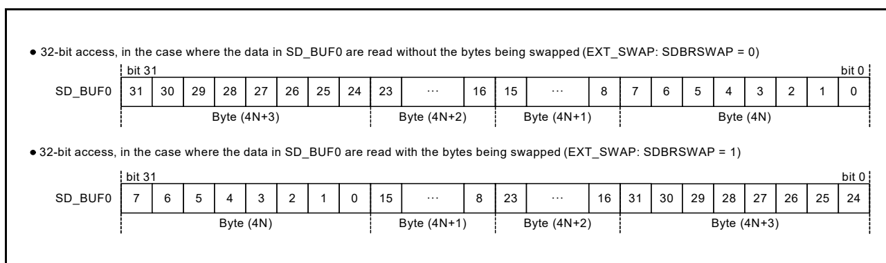
Figure 36.6 Reading from the SD_BUF0 register
