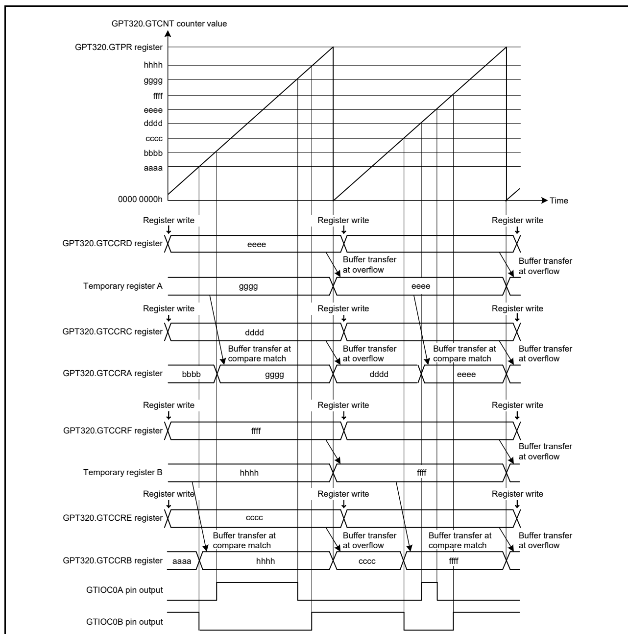
Figure 23.31 Example of saw-wave one-shot pulse mode operation with up-counting, low output from the GTIOC0A pin and high output from the GTIOC0B pin at count start, output toggled at GTCCRA/ GTCCRB compare match, and output retained at cycle end
