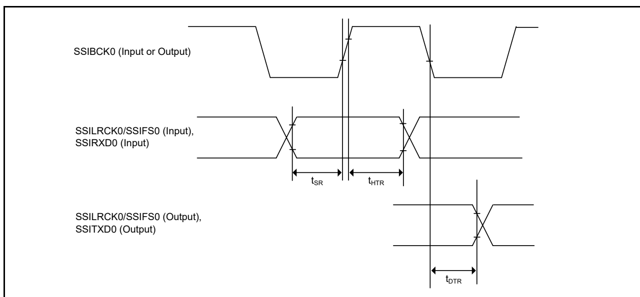
Figure 51.72 SSIE data transmit/receive timing (SSICR.BCKP = 0)
