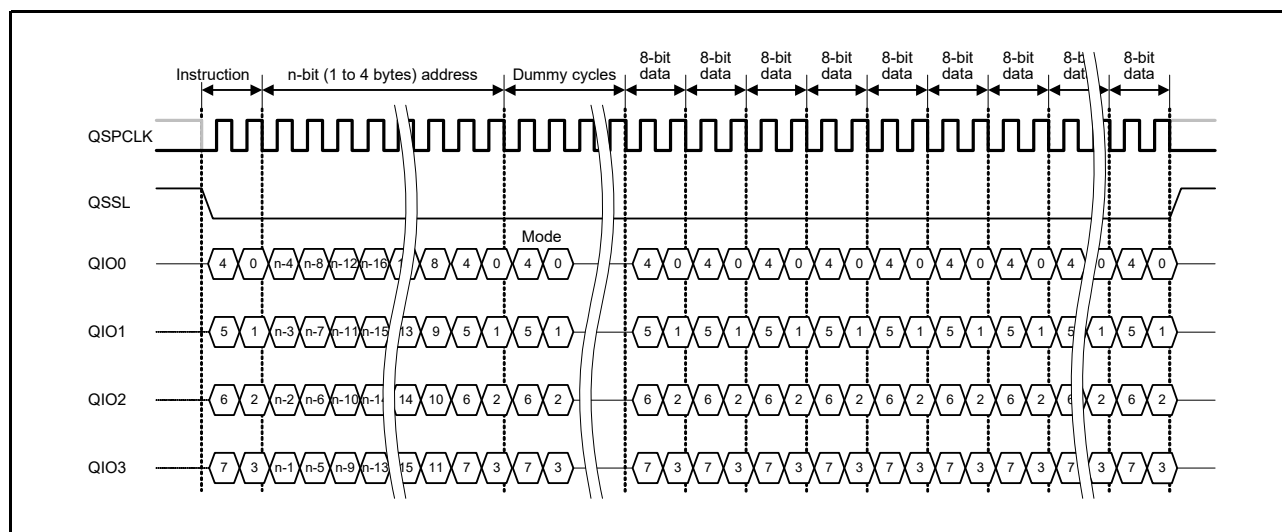
Figure 33.7 Quad SPI protocol example for Fast Read
