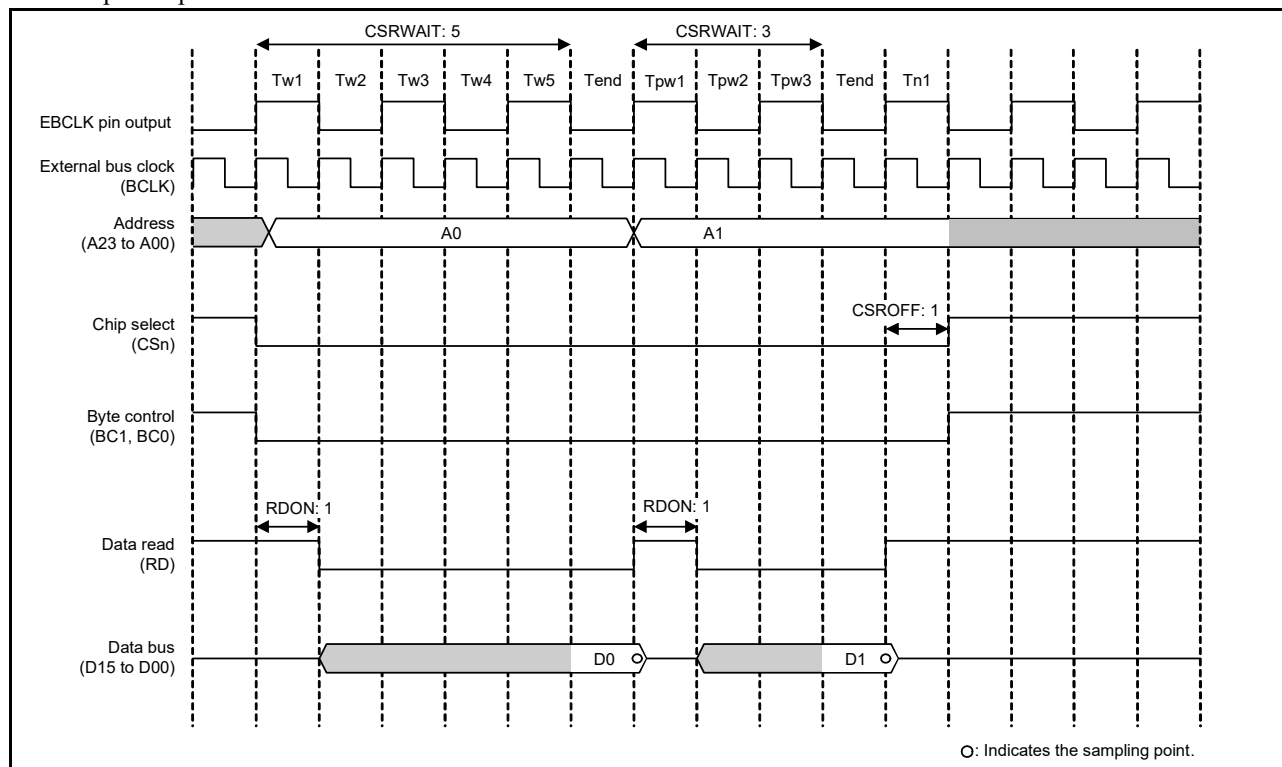
Figure 15.21 Example of page read access operation when BCLK/2 is selected with EBCLK pin output select bit, two rounds of bus access are generated in response to a single transfer request ( n = 0 to 3)
