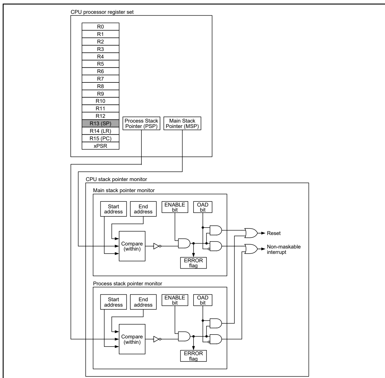
Figure 16.1 CPU stack pointer monitor block diagram
