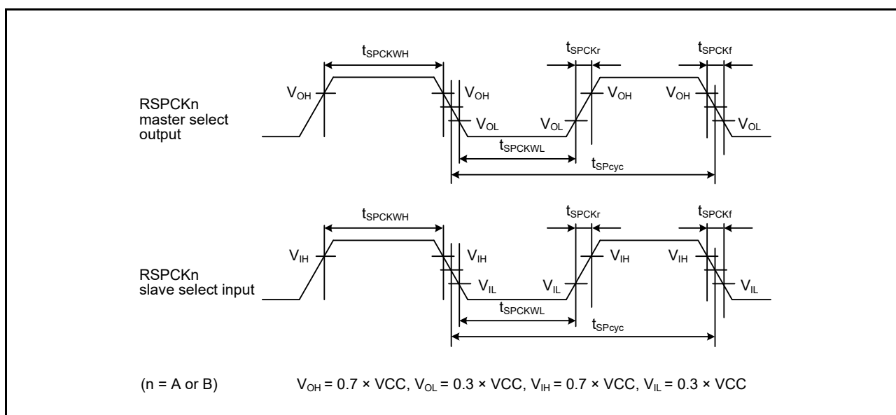
Figure 51.61 SPI clock timing
