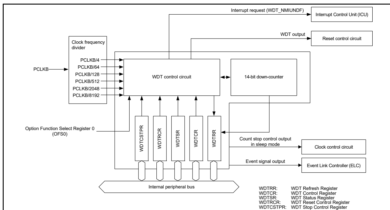
Figure 26.1 WDT block diagram
