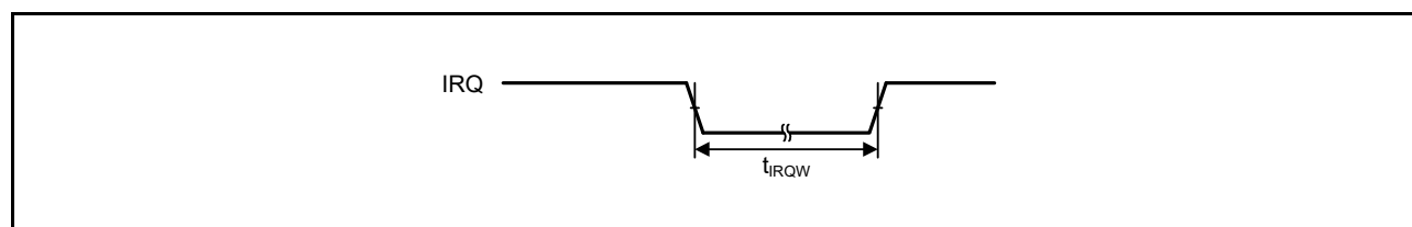
Figure 51.39 IRQ interrupt input timing
