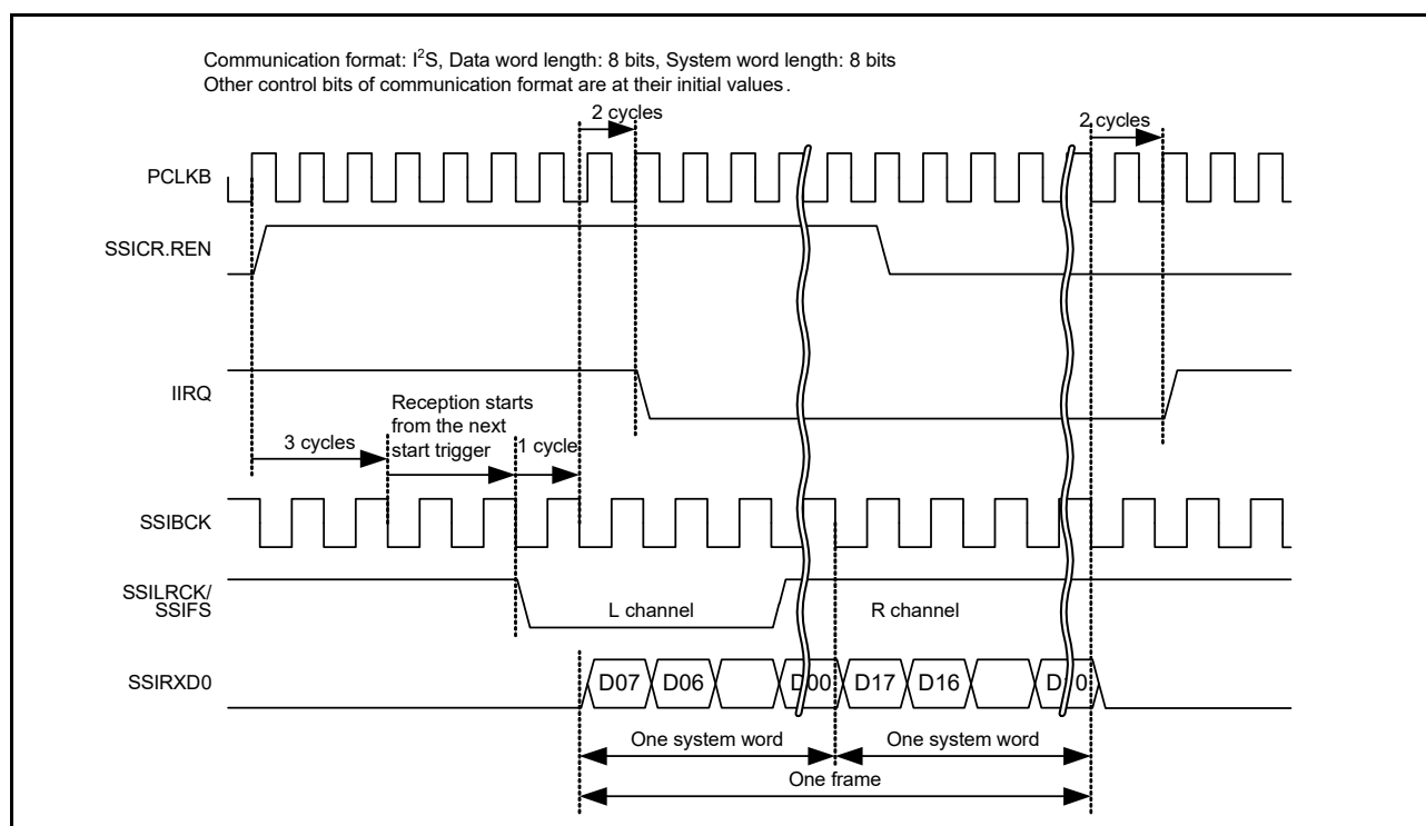
Figure 35.13 IIRQ setting timing (reception)
