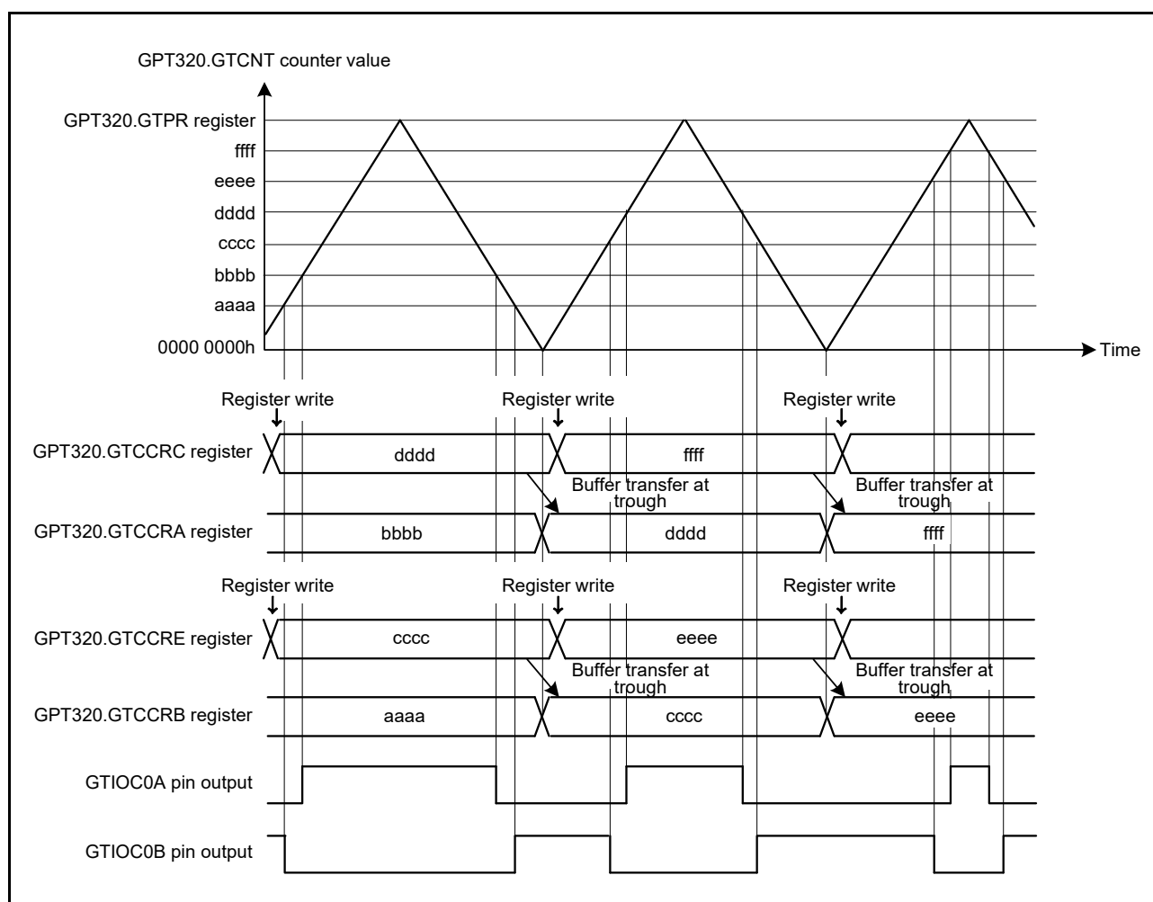
Figure 23.33 Example of triangle-wave PWM mode 1 operation with buffer operation, low output from the GTIOCA pin and high output from the GTIOCB pin at count start, output toggled at GTCCRA/ GTCCRB register compare match, and output retained at cycle end
