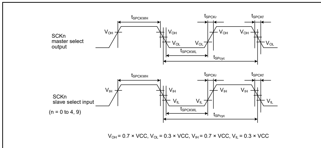
Figure 51.55 SCI simple SPI mode clock timing
