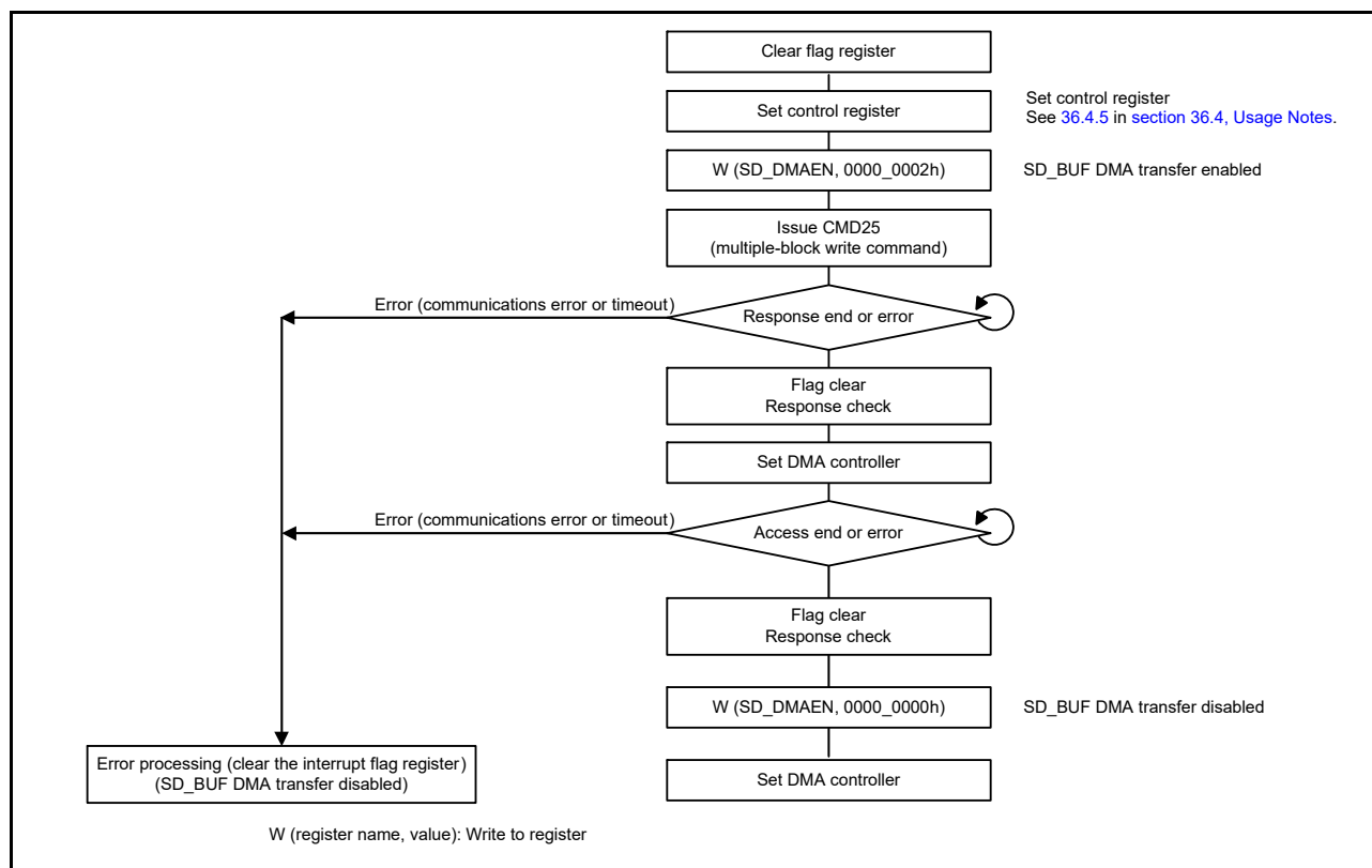
Figure 36.24 Example of SD_BUF DMA write operation
