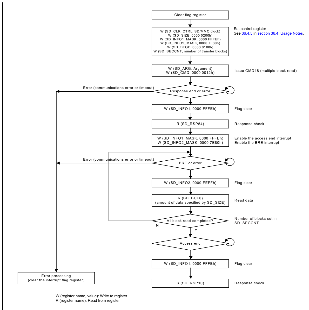
Figure 36.13 Example flow of multiple block read operation
