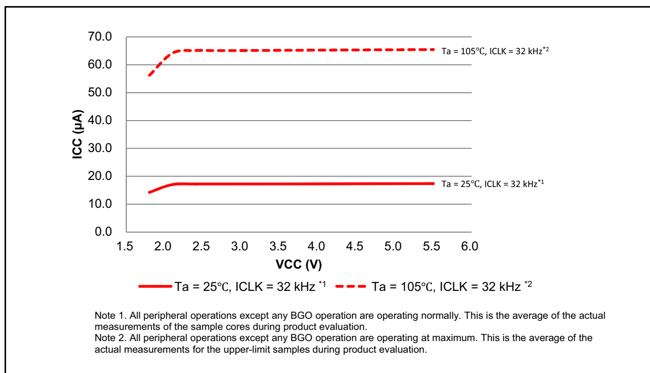
Figure 51.21 Voltage dependency in Subosc-speed mode (reference data)
