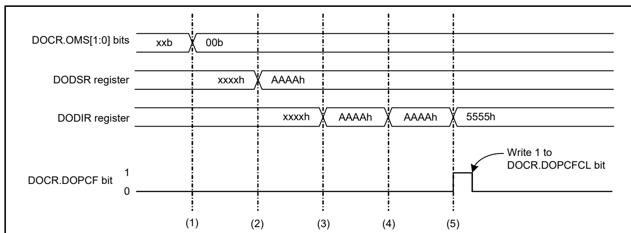
Figure 45.2 Example operation in data comparison mode
