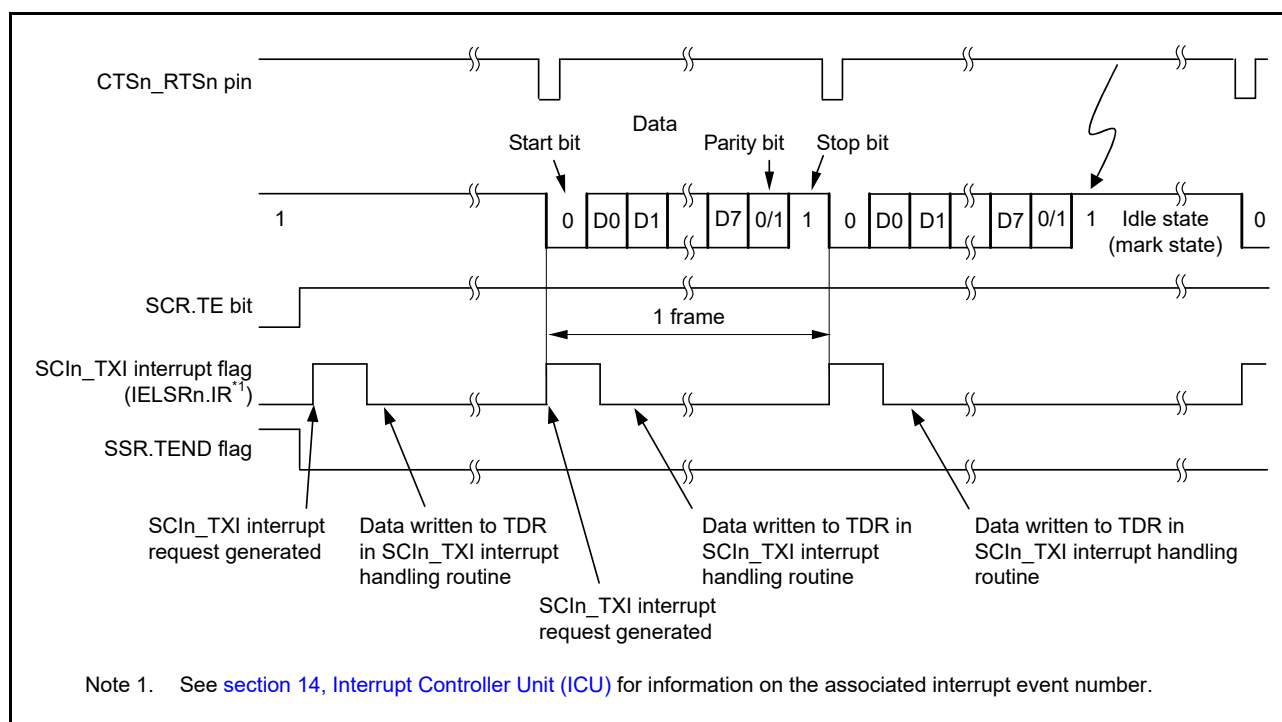
Figure 29.10 Example operation for serial transmission in asynchronous mode (2) with 8-bit data, parity bit, 1 stop bit, CTS function used, and at the beginning of transmission
