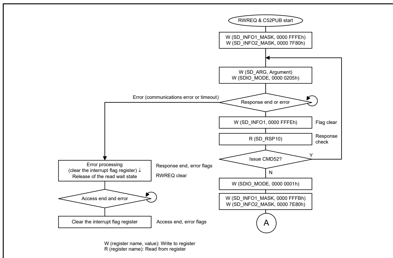
Figure 36.19 Flow when CMD52 (SDIO none abort) is issued at CMD53 multiple block read while the SD host interface is in read wait state
