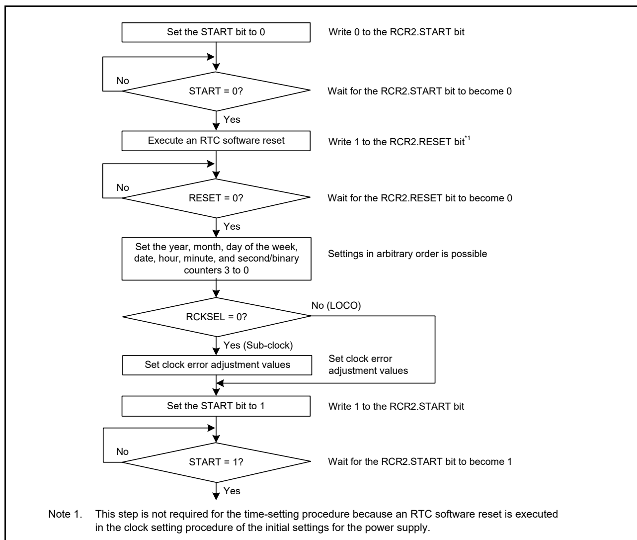
Figure 25.4 Setting the time
