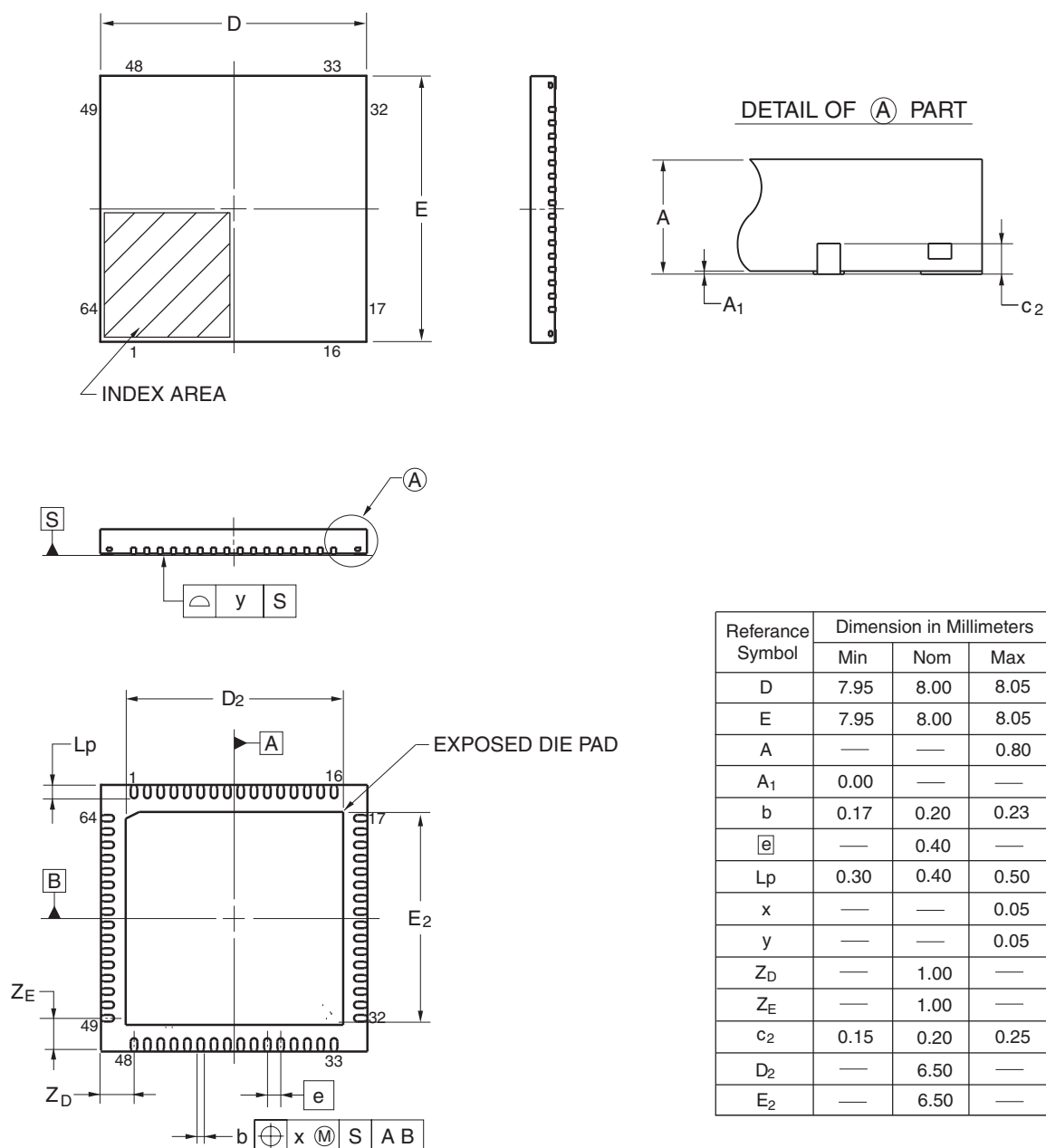
Figure 2.7 QFN 64-pin
