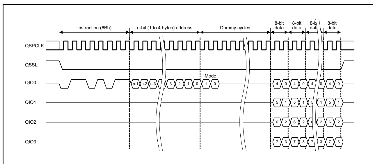
Figure 33.23 Fast Read Quad Output bus cycle
