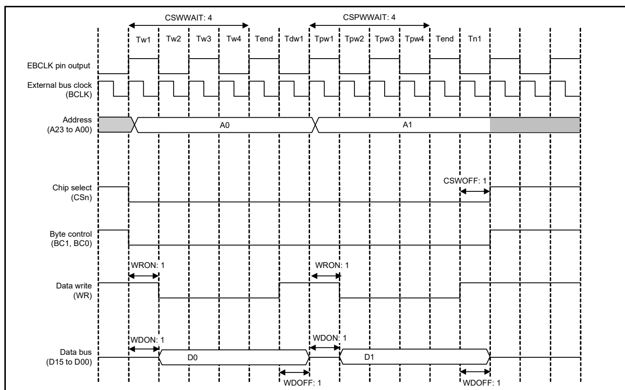
Figure 15.22 Example of page write access operation when BCLK/2 is selected with the EBCLK pin output select bit, two rounds of bus access are generated in response to a single transfer request, in single write strobe mode ( n = 0 to 3)
