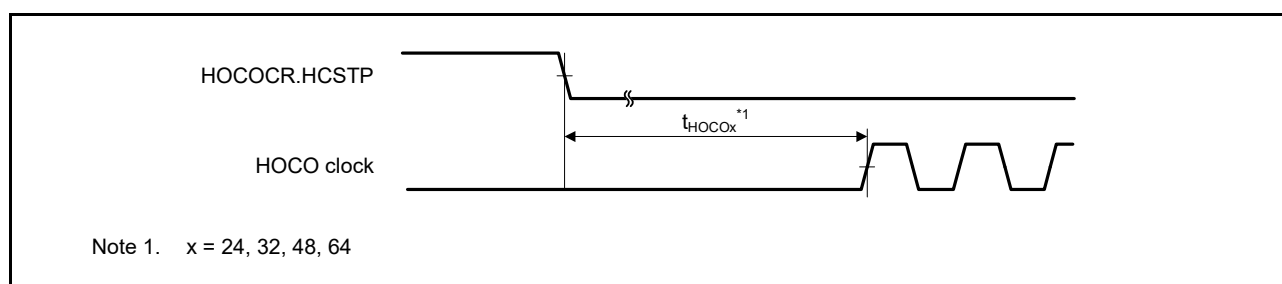
Figure 51.29 HOCO clock oscillator start timing (started by setting HOCOCR.HCSTP bit)
