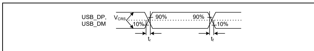
Figure 51.77 USB_DP and USB_DM output timing
