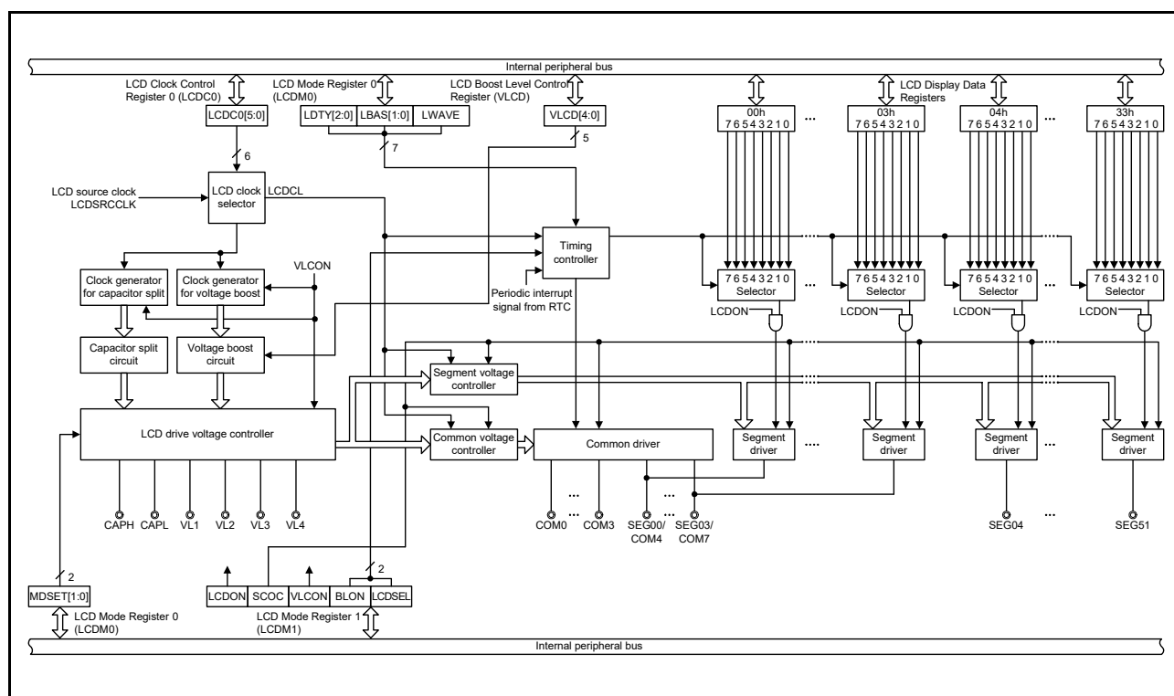
Figure 48.1 SLCDC block diagram
