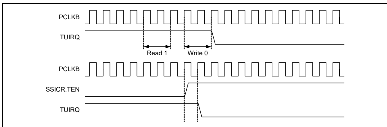
Figure 35.17 TUIRQ clearing timing
