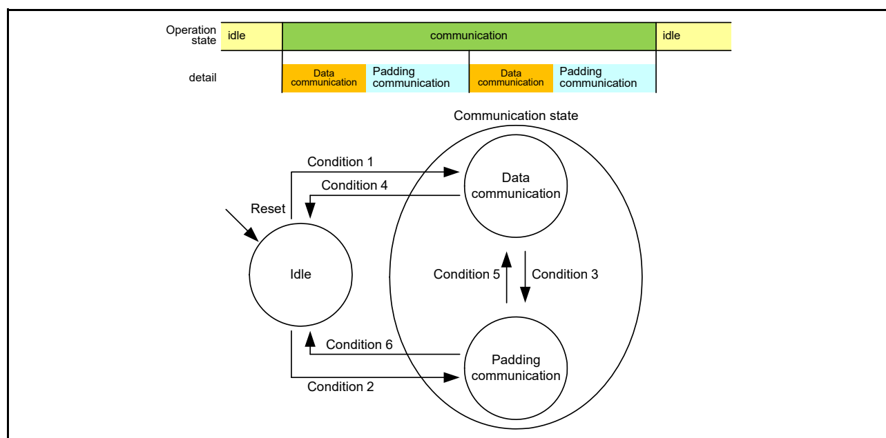
Figure 35.42 Communication state transition
