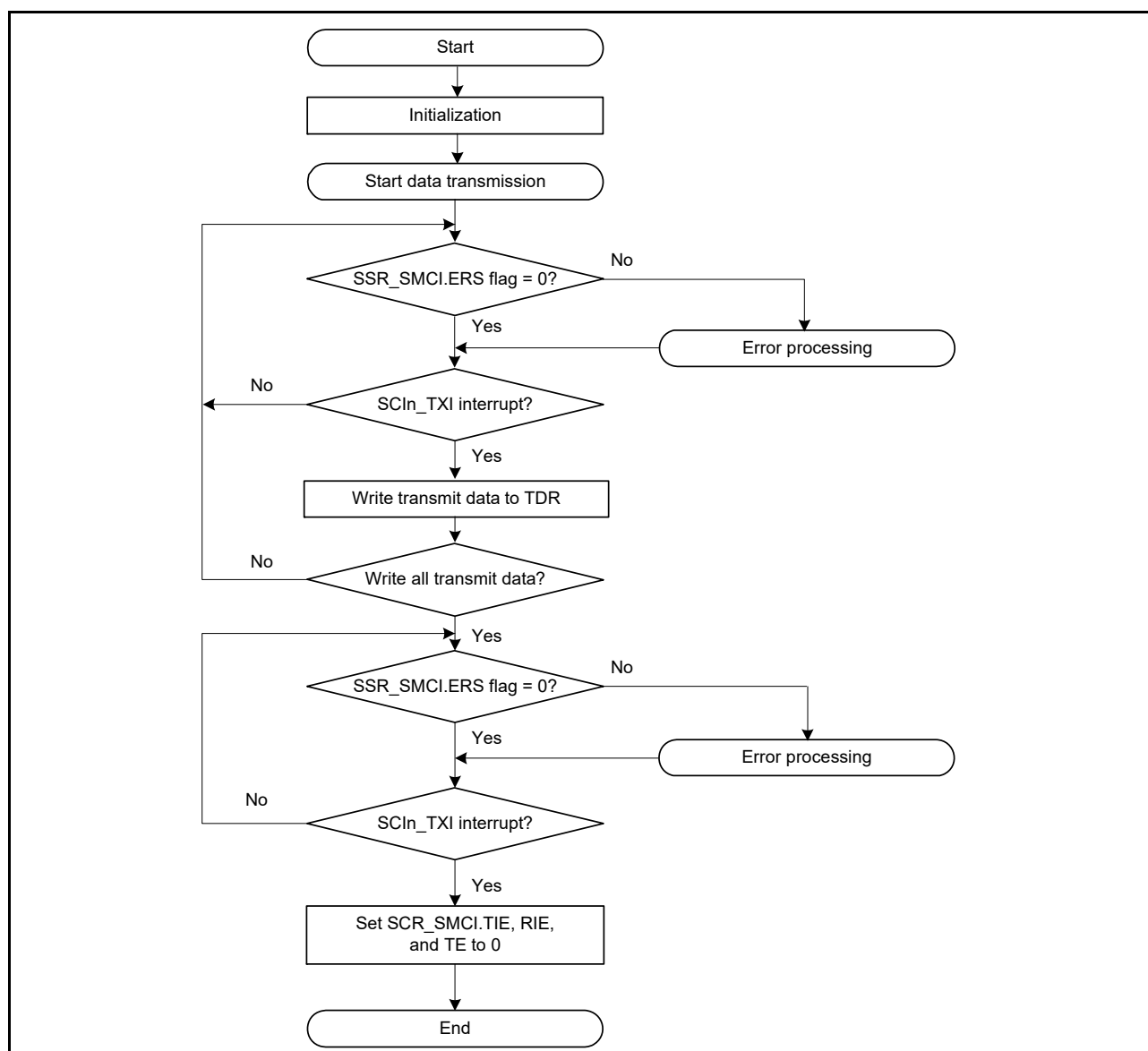
Figure 29.54 Example flow of smart card interface transmission
