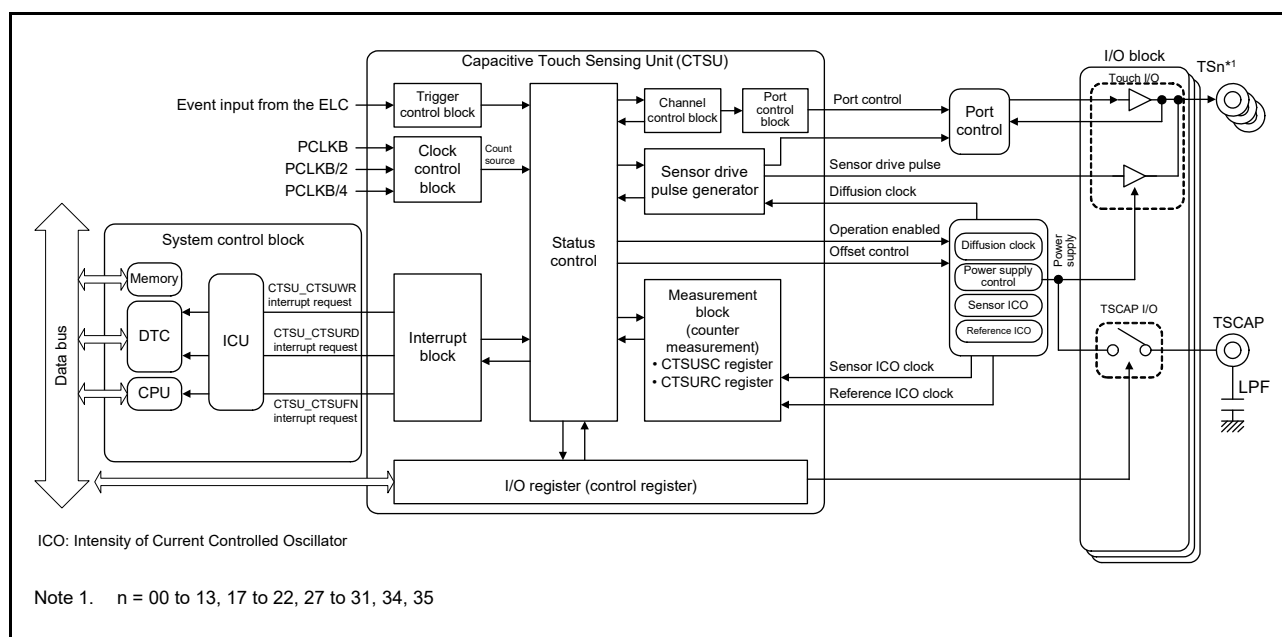
Figure 44.3 CTSU block diagram
