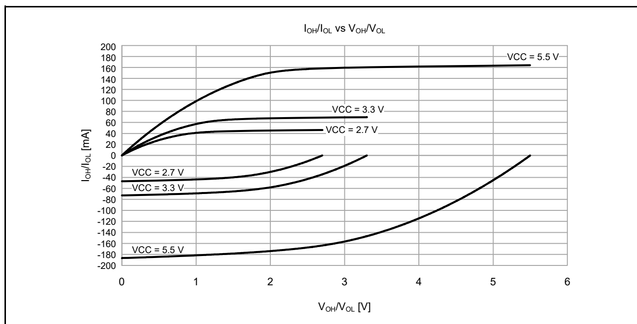
Figure 51.12 V_{OH}/V_{OL} and I_{OH}/I_{OL} voltage characteristics at T_a = 25^\circ\text{C} when middle drive output is selected (reference data)
