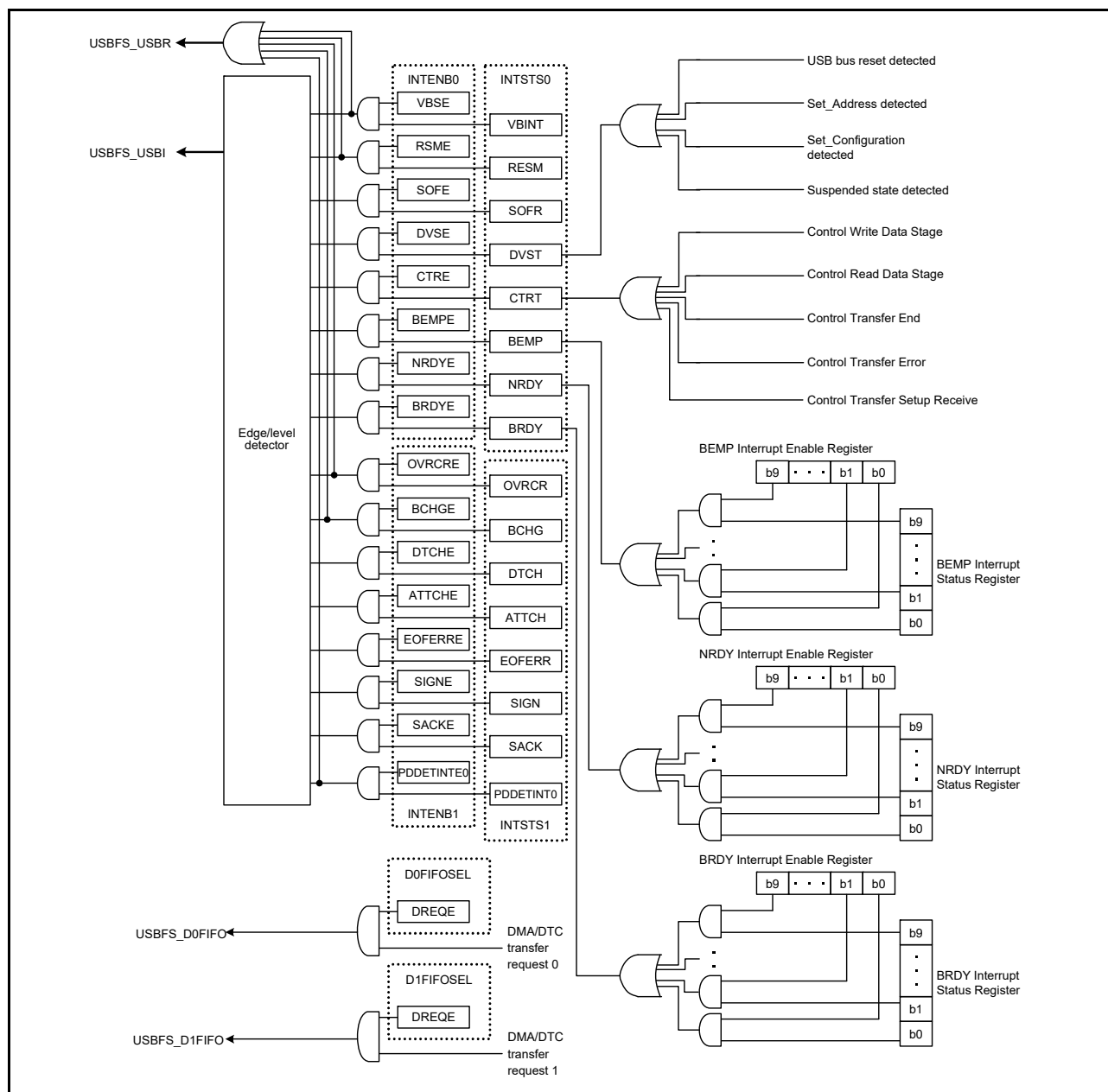
Figure 28.11 USBFS interrupt-related circuits
