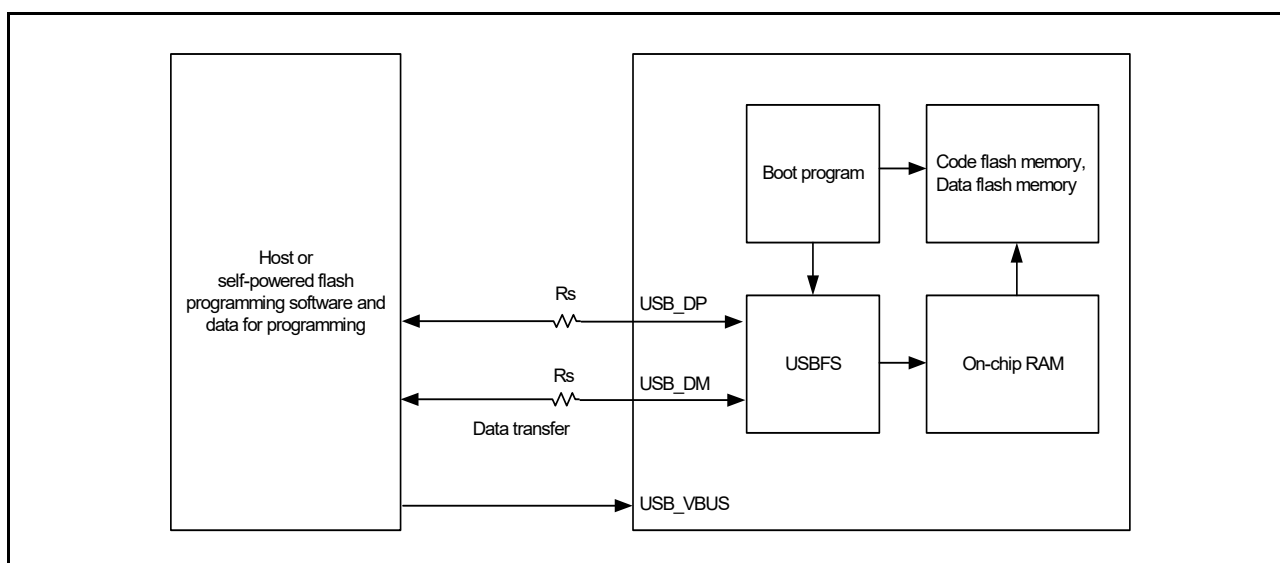
Figure 47.10 System configuration in USB boot mode
