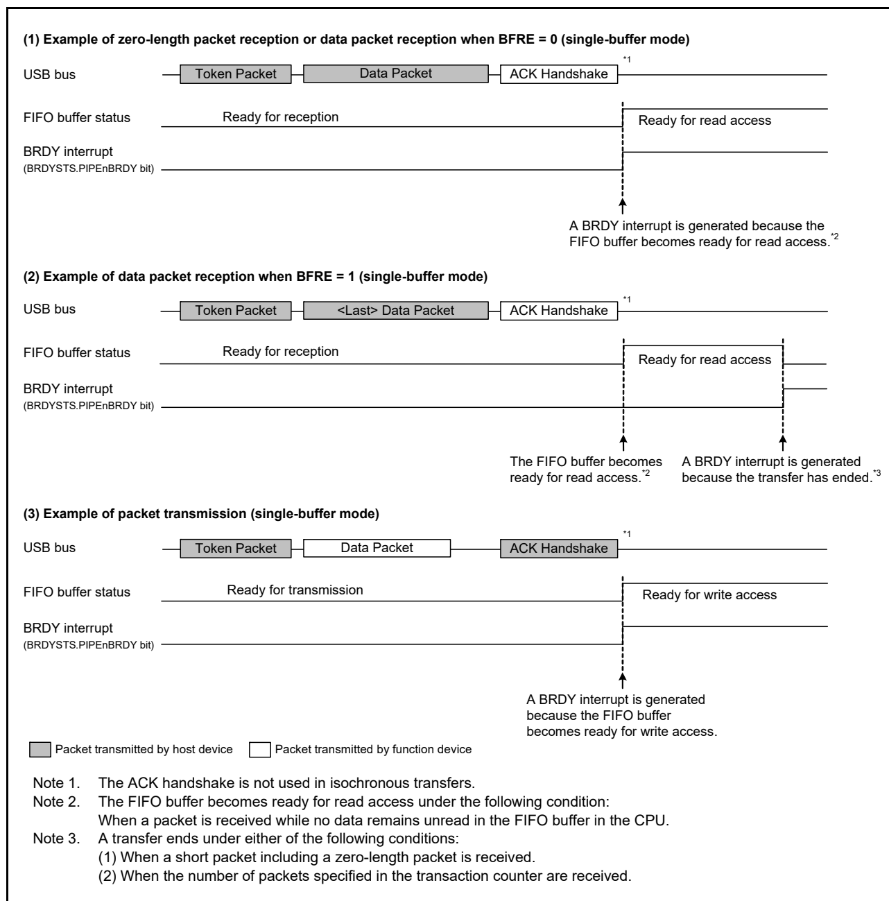
Figure 28.12 Timing of BRDY interrupt generation
