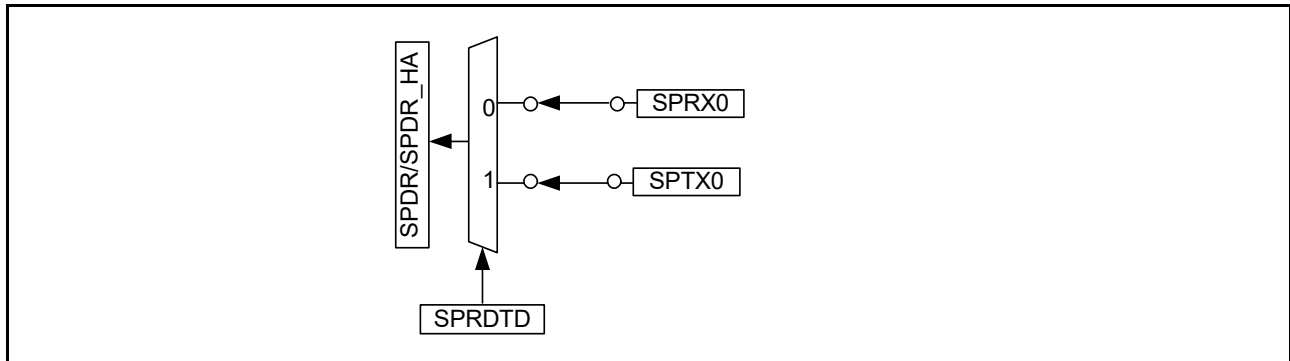
Figure 32.7 Configuration of SPDR/SPDR_HA for read access (SPI1)
