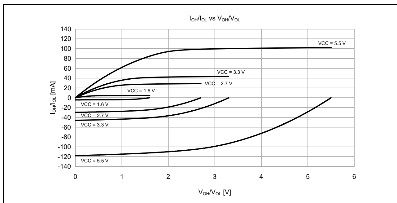
Figure 51.7 V_{OH}/V_{OL} and I_{OH}/I_{OL} voltage characteristics at T_a = 25^\circ\text{C} when middle drive output is selected (reference data)
