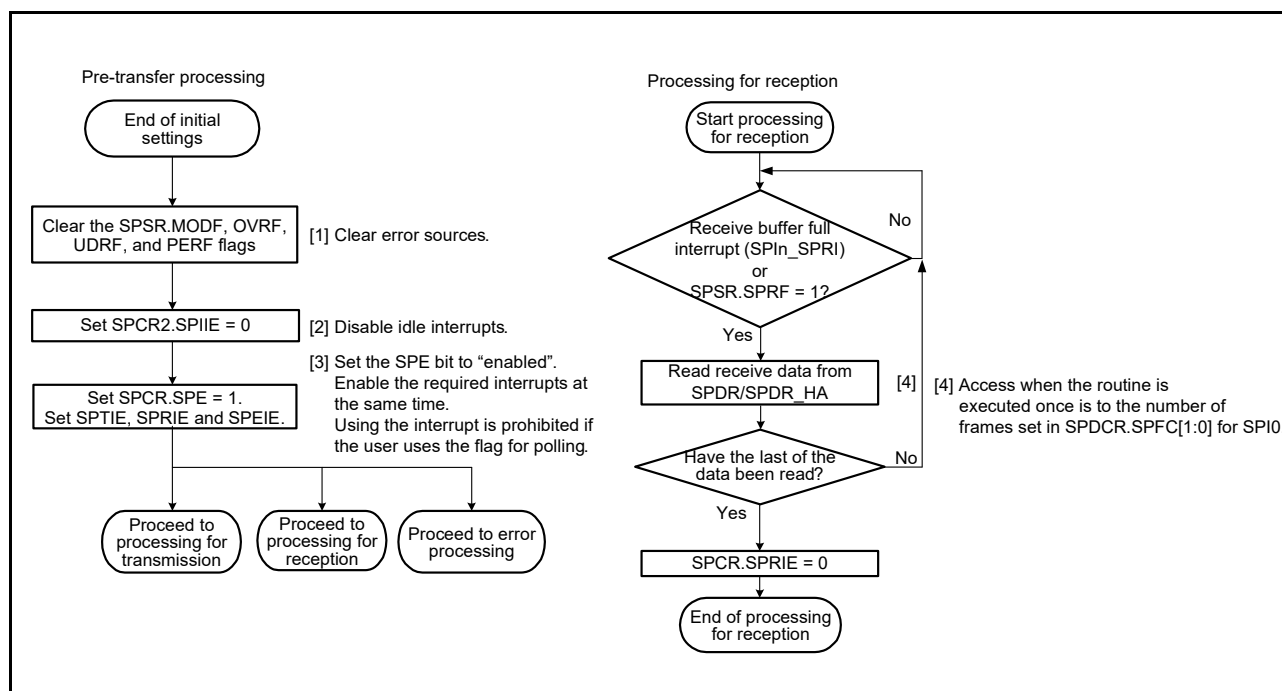
Figure 32.49 Reception flow in slave mode
