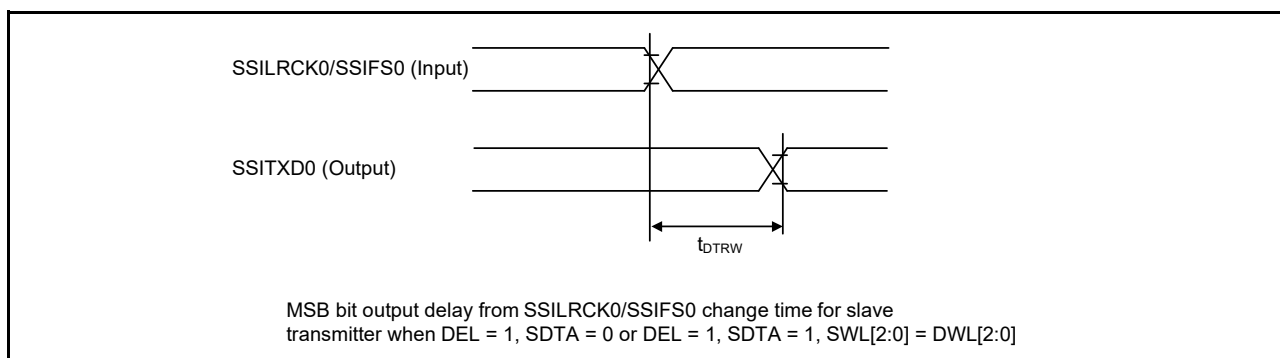
Figure 51.74 SSIE data output delay from SSILRCK0/SSIFS0 change time
