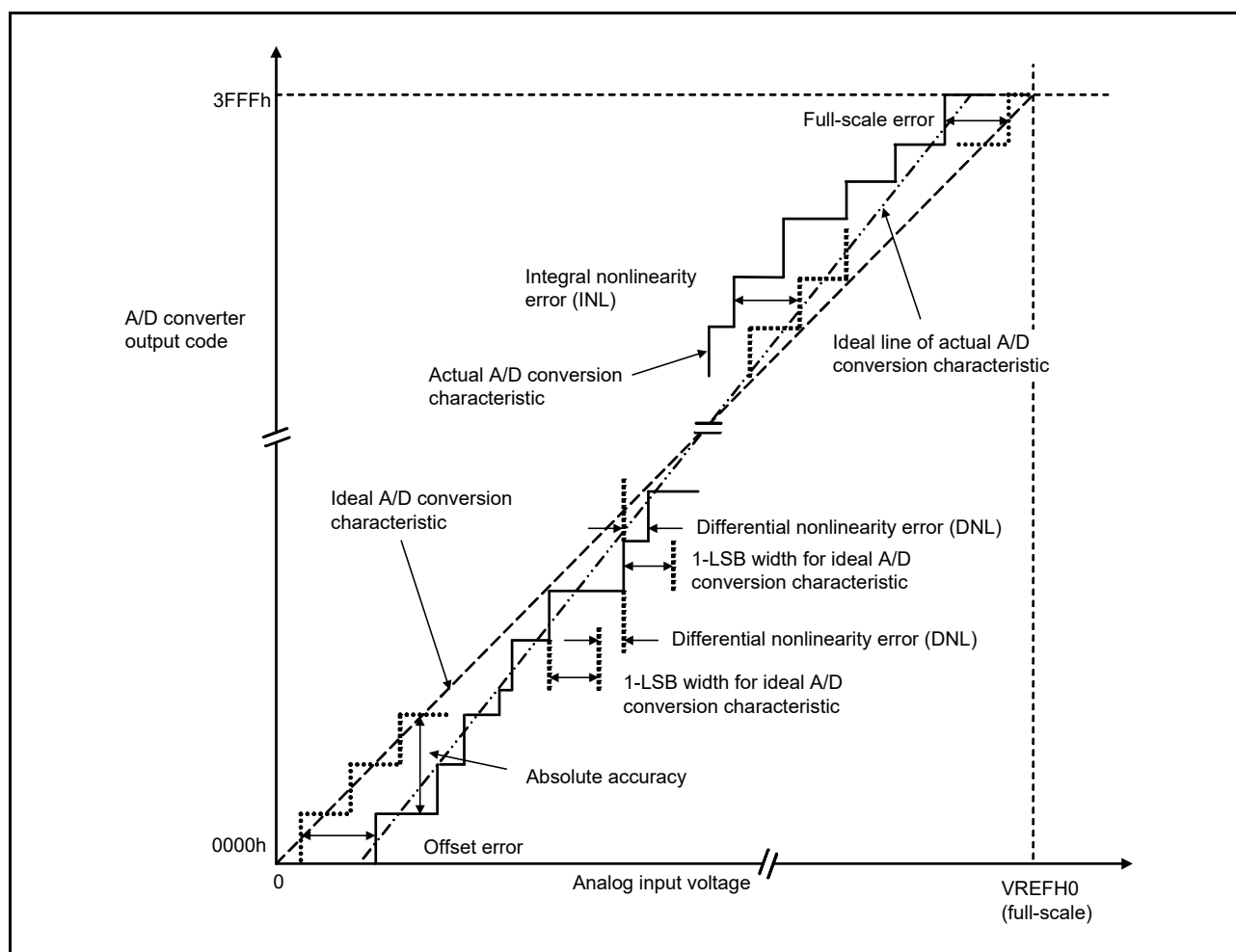
Figure 51.82 Illustration of 14-bit A/D converter characteristic terms
