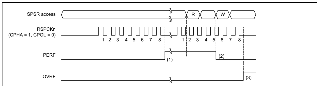
Figure 32.35 Operation example of the PERF flag
