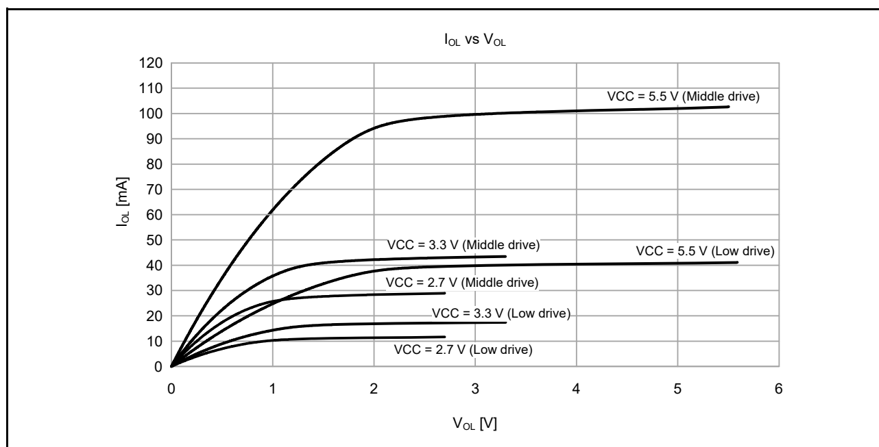
Figure 51.16 V_{OH}/V_{OL} and I_{OH}/I_{OL} voltage characteristics at T_a = 25^\circ\text{C}
