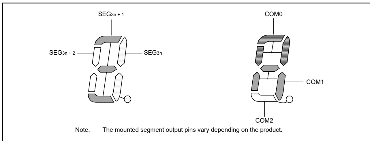
Figure 48.24 Three-time-slice LCD display pattern and electrode connections
