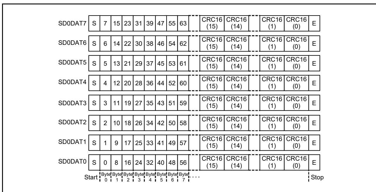
Figure 36.4 SD0DAT in 8-bit width mode
