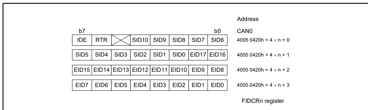
Figure 31.15 Structure of the FIDCRn registers (n = 0, 1)
