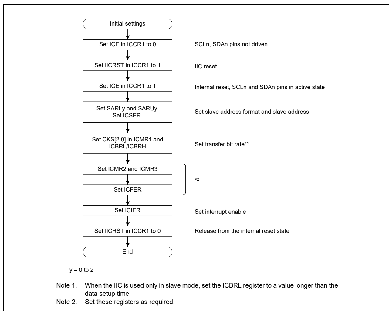
Figure 30.5 Example IIC initialization flow
