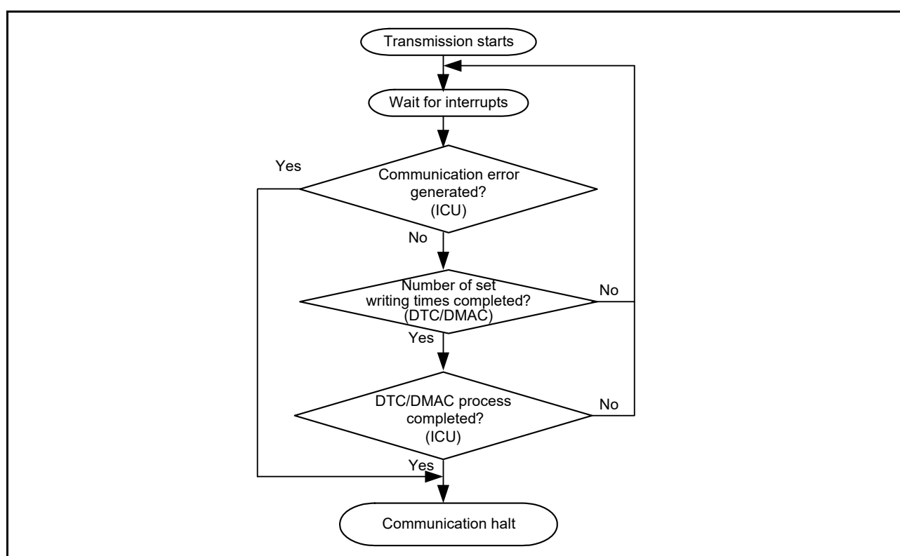
Figure 35.50 Transmission procedure
