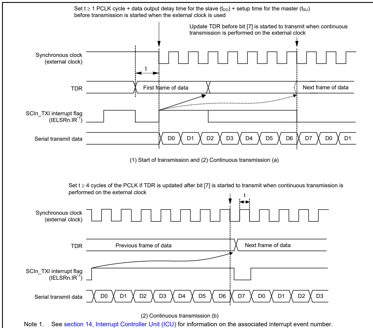
Figure 29.78 Restrictions on the use of external clock in clock synchronous transmission
