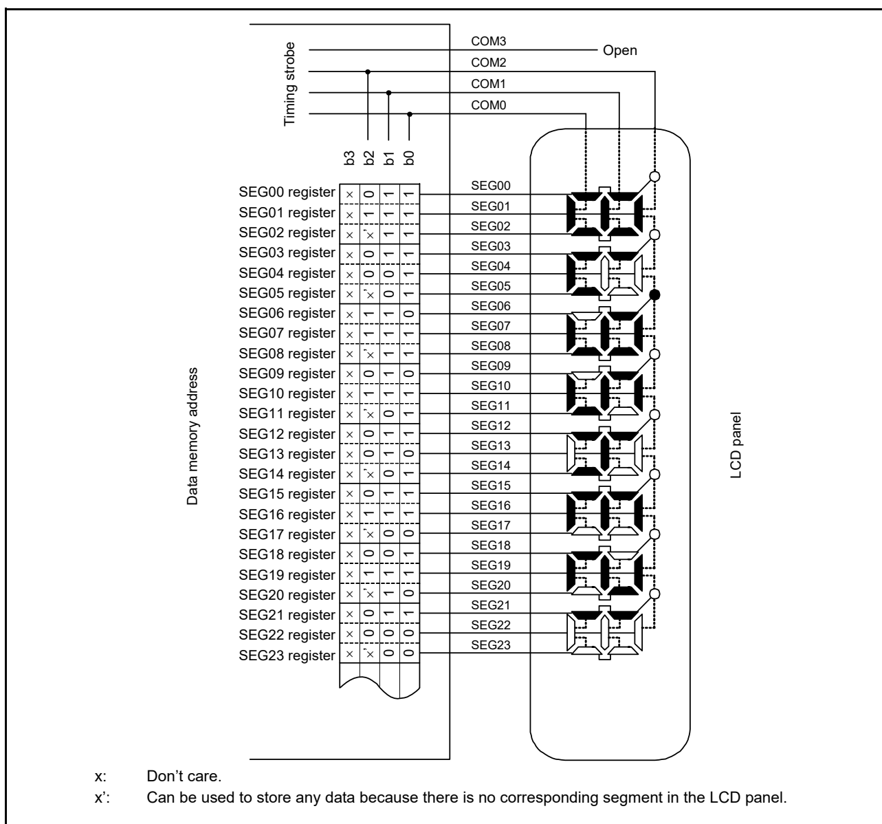
Figure 48.25 Example of connecting three-time-slice LCD panel
