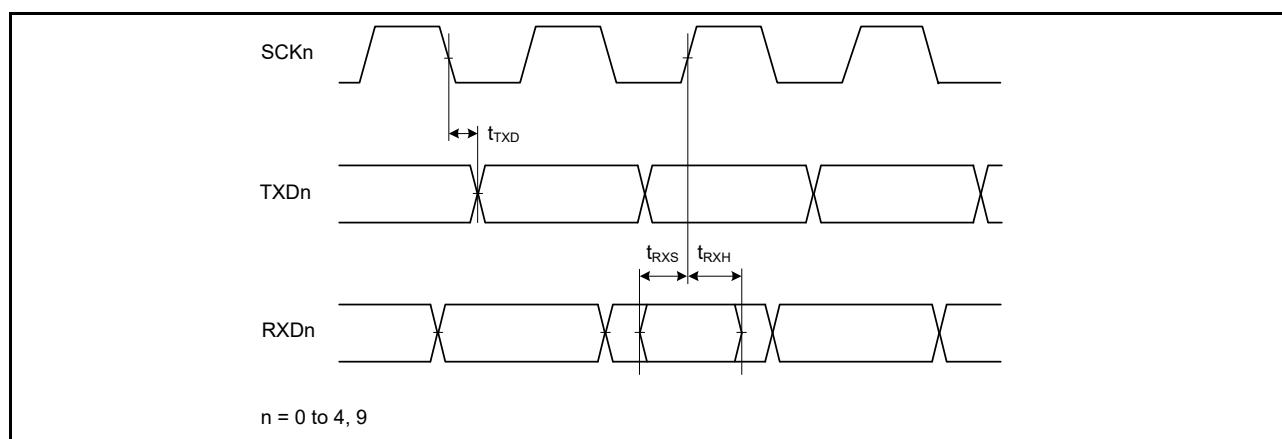
Figure 51.54 SCI input/output timing in clock synchronous mode
