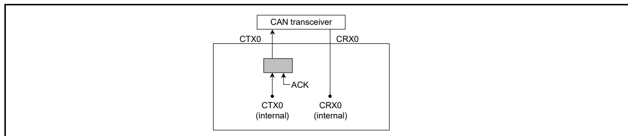
Figure 31.7 Connection when self-test mode 0 is selected
