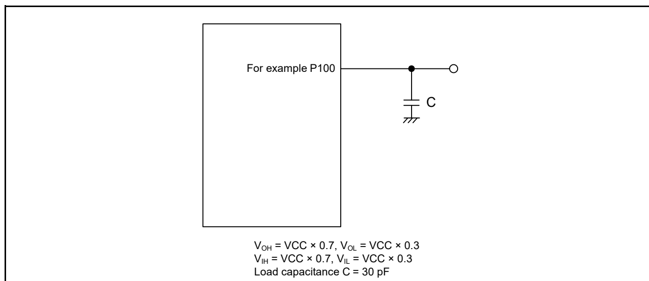
Figure 51.1 Input or output timing measurement conditions
