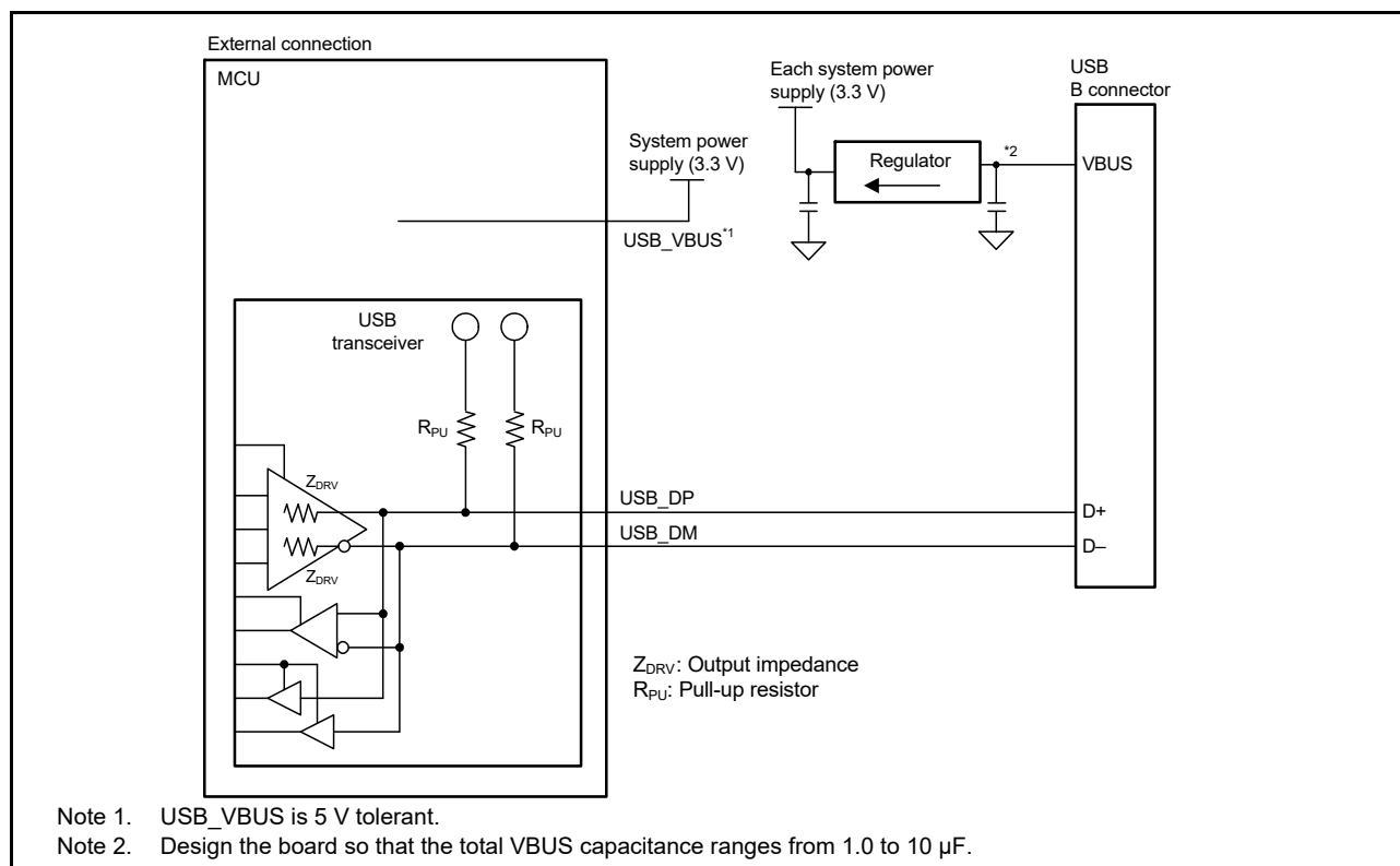
Figure 28.8 Example device connection in bus-powered state 1
