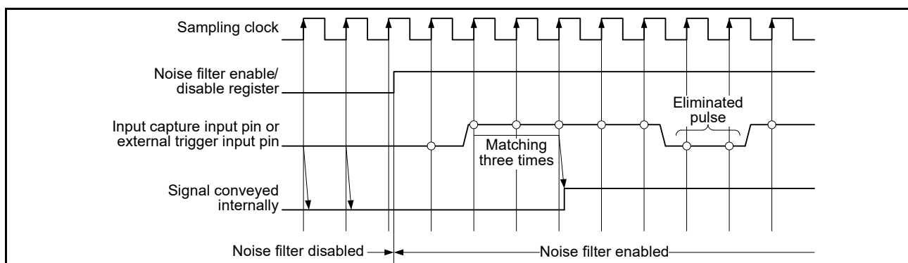
Figure 23.82 Timing of noise filtering
