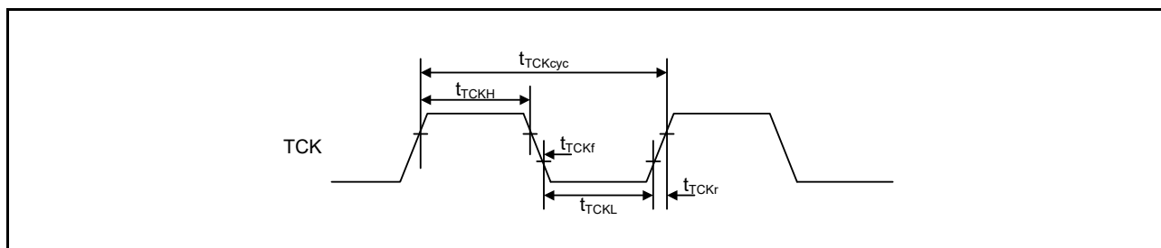
Figure 51.94 Boundary scan TCK timing
