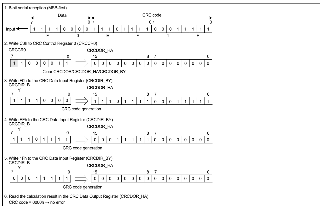
Figure 34.5 MSB-first data reception
