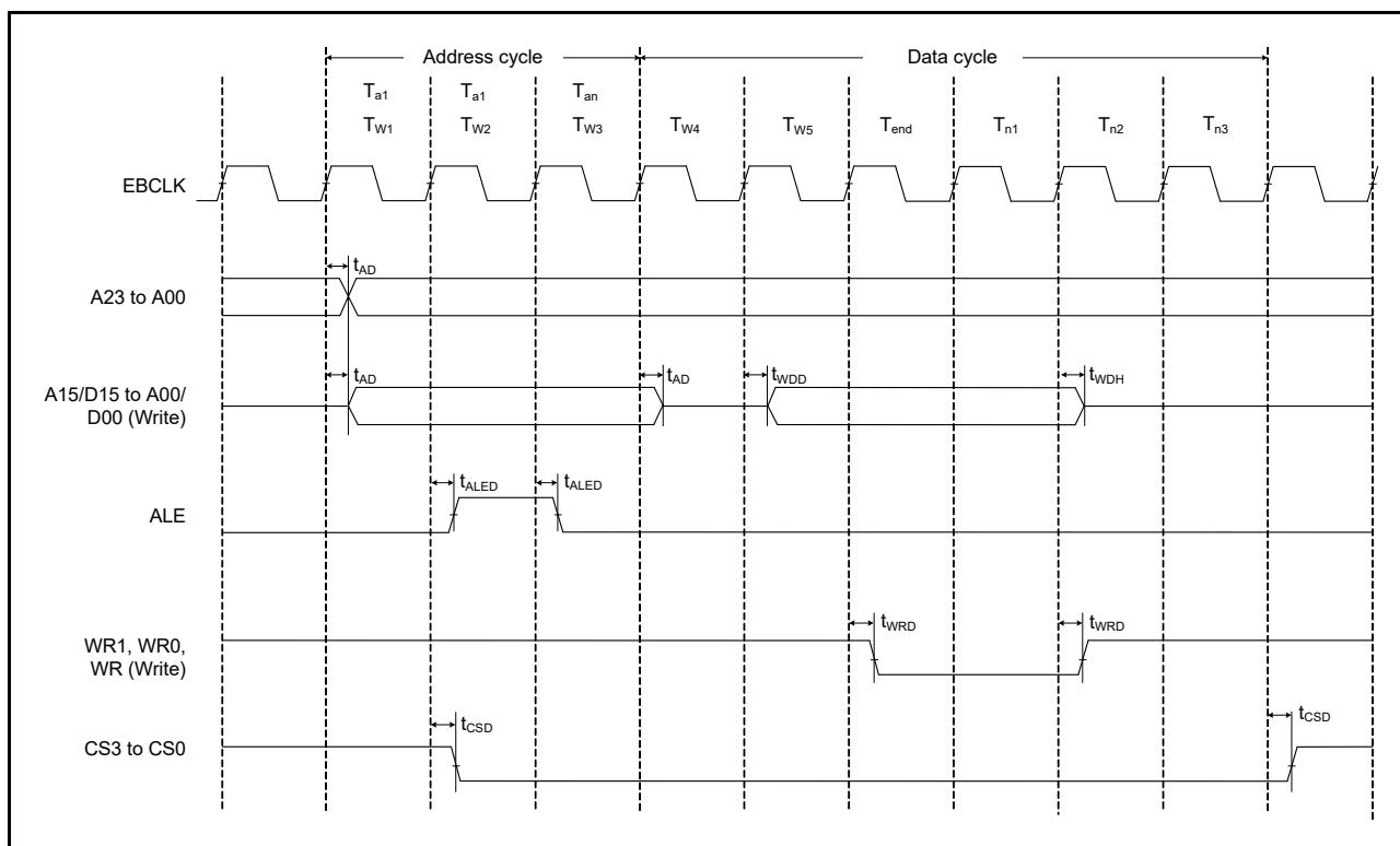
Figure 51.41 Address/data multiplexed bus write access timing
