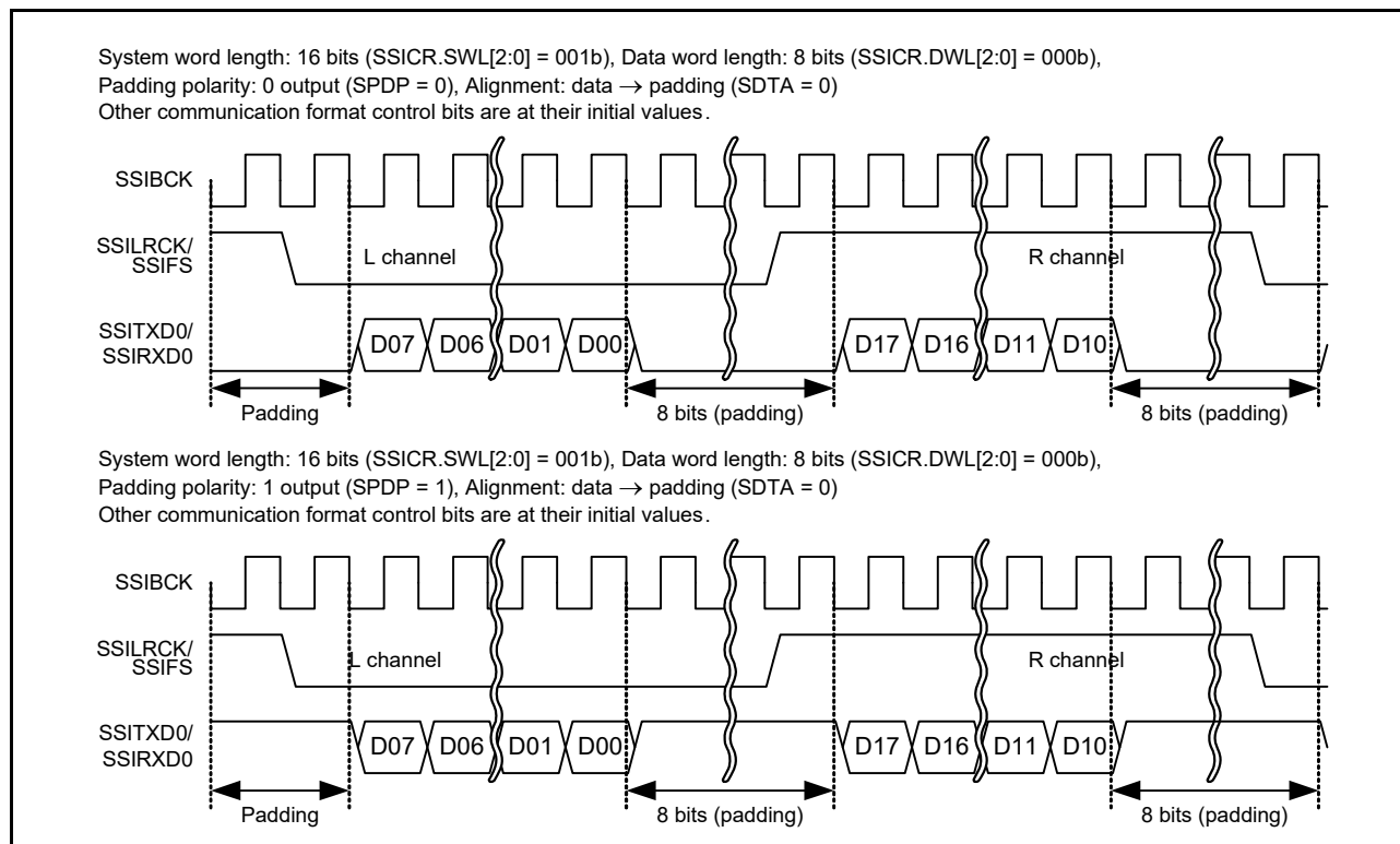
Figure 35.10 Padding bit polarity
