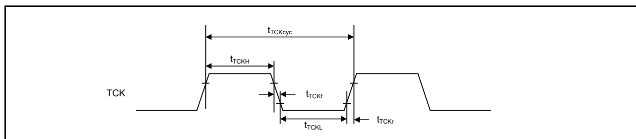
Figure 51.97 JTAG TCK timing
