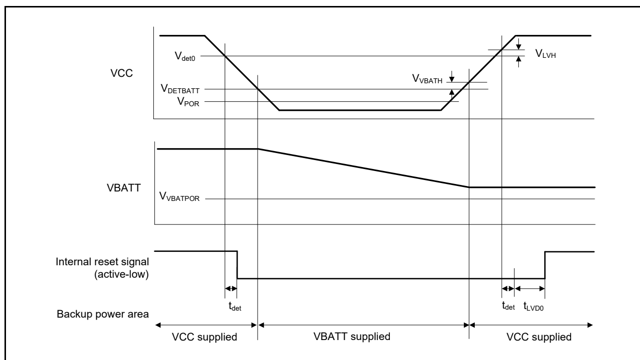
Figure 51.90 Power supply switching and LVD0 reset timing
