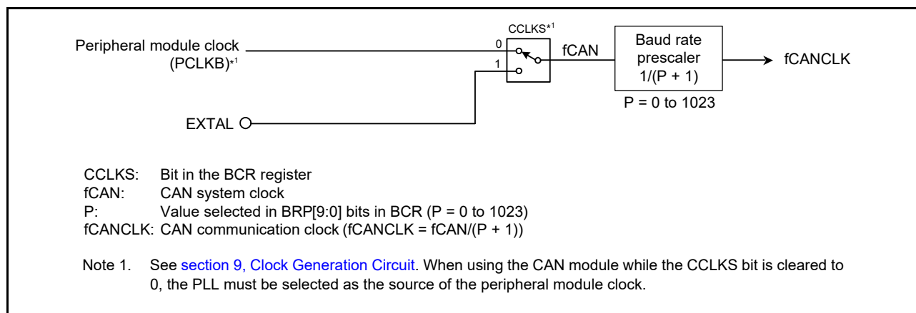
Figure 31.11 CAN clock generator block diagram
