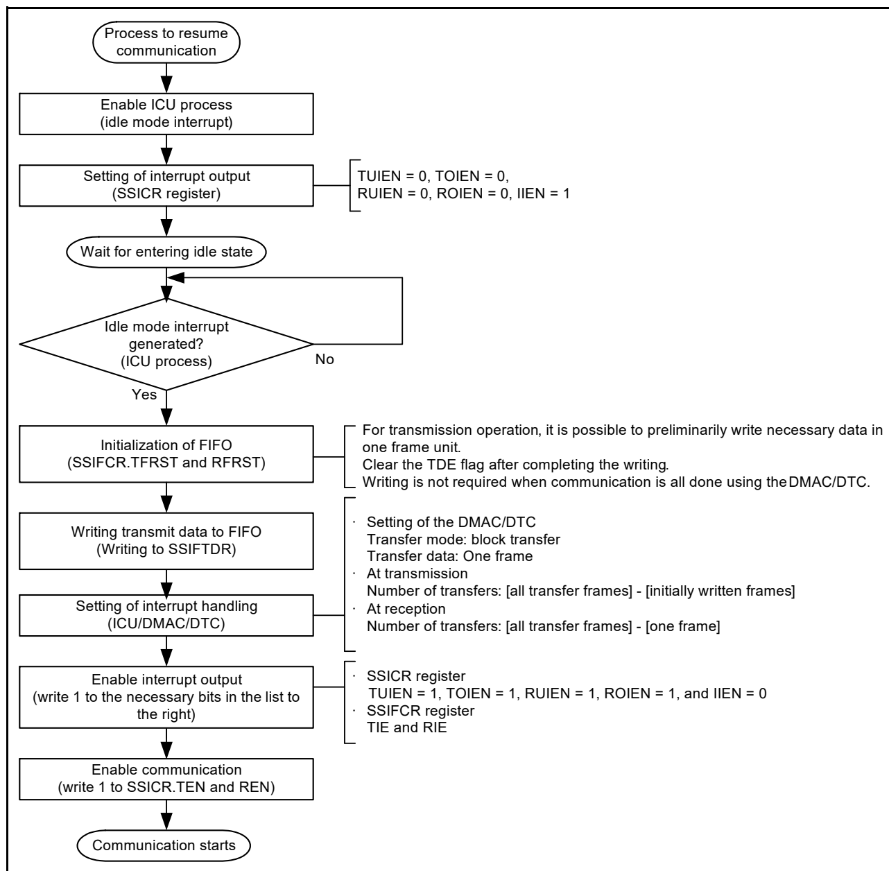
Figure 35.54 Procedure to resume communication (CPU operation)
