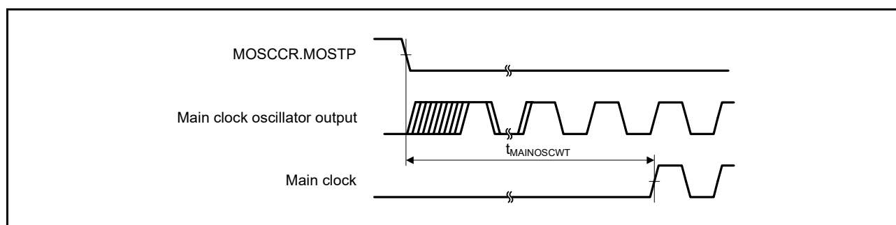
Figure 51.30 Main clock oscillation start timing
