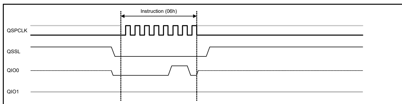
Figure 33.29 Write enable bus cycle
