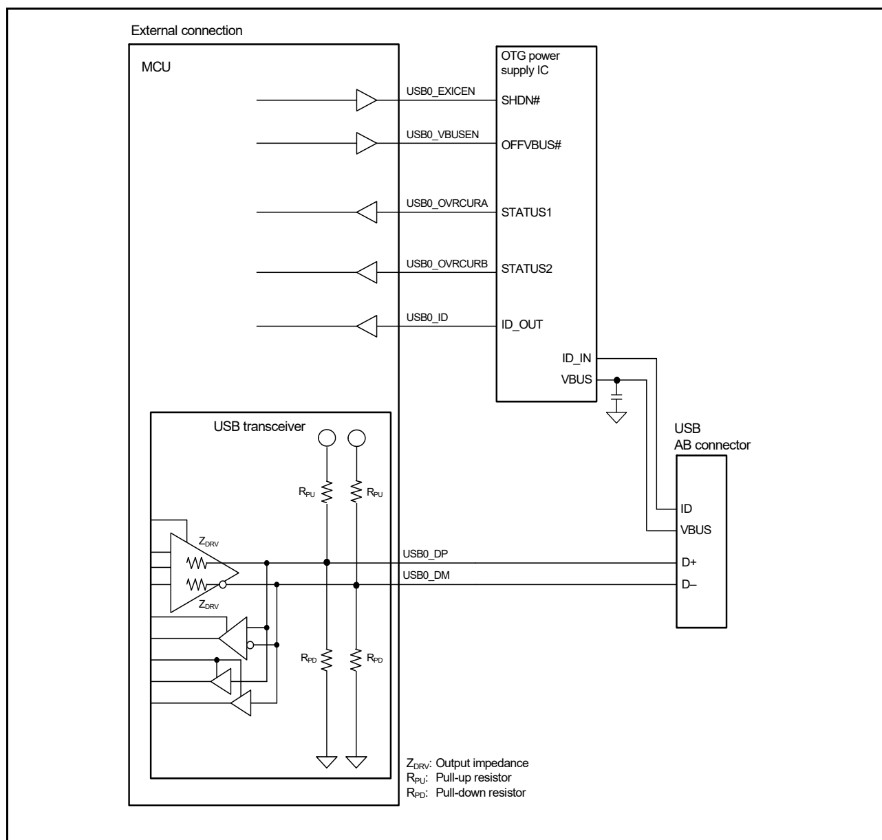
Figure 28.5 Example OTG connection in self-powered state
