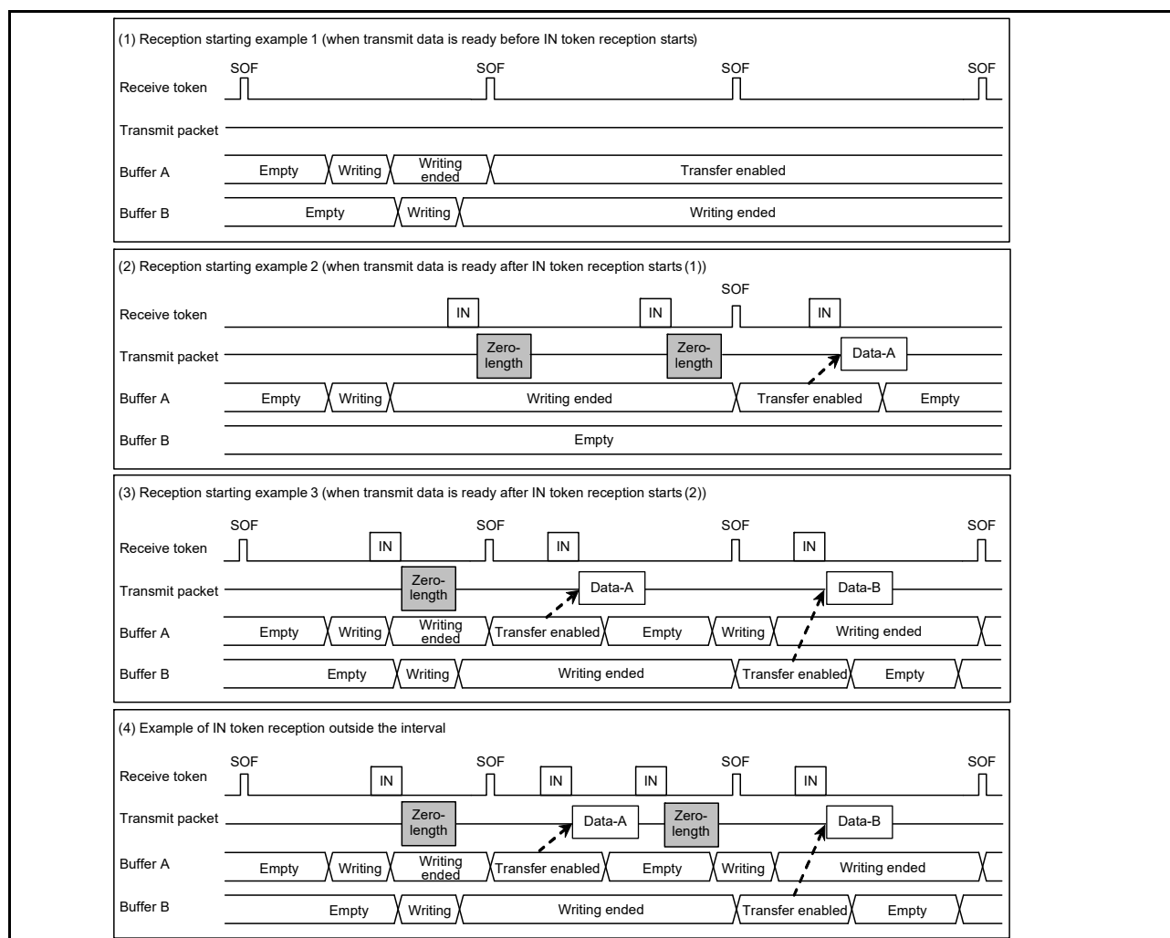
Figure 28.21 Example data setup operation
