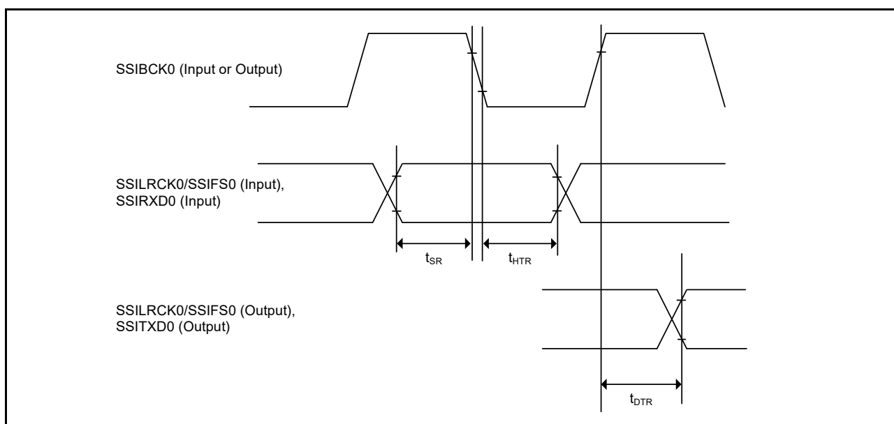
Figure 51.73 SSIE data transmit/receive timing (SSICR.BCKP = 1)
