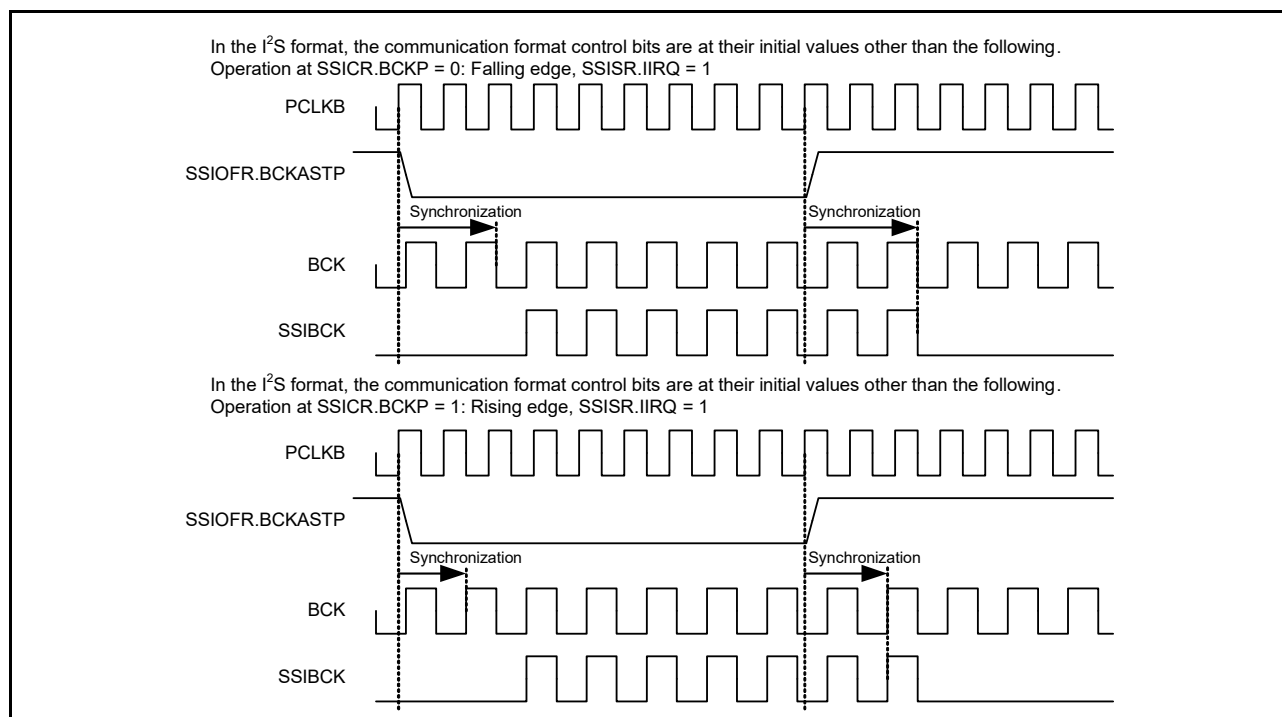
Figure 35.41 Example of stopping SSIBCK with SSIOFR.BCKASTP
