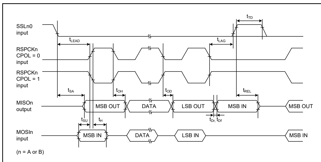
Figure 51.66 SPI timing (slave, CPHA = 0)
