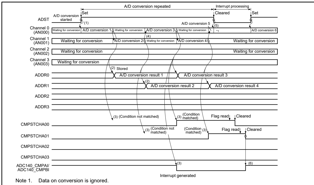
Figure 38.21 Example of compare function operation, when AN000 to AN003 are compared
