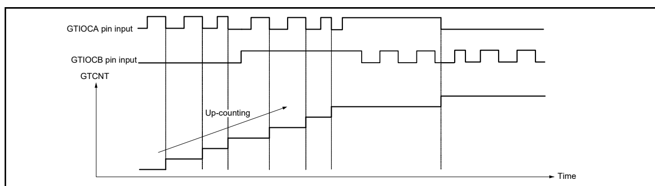
Figure 23.75 Example of phase counting mode 5 (A)
