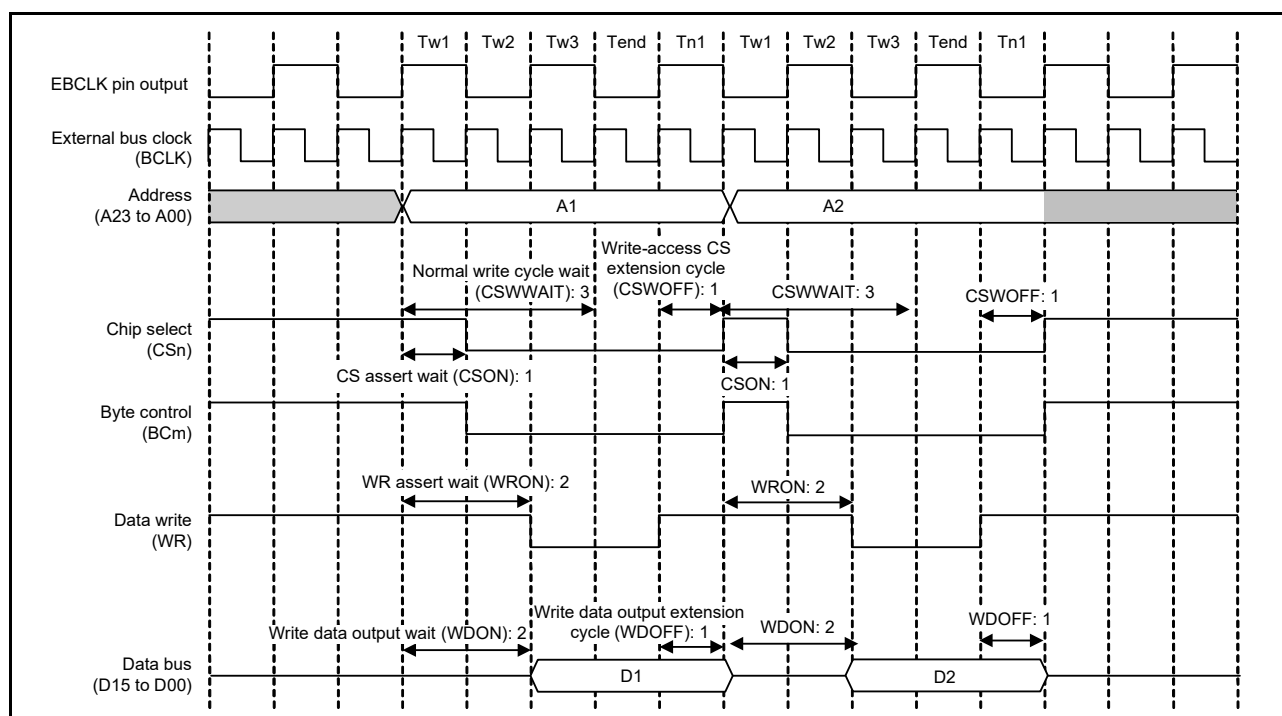
Figure 15.16 Example of normal-write operation when BCLK/2 is selected with the EBCLK pin output select bit and two rounds of bus access are generated in response to a single transfer request ( n = 0 to 3 ; m = 0, 1 )
