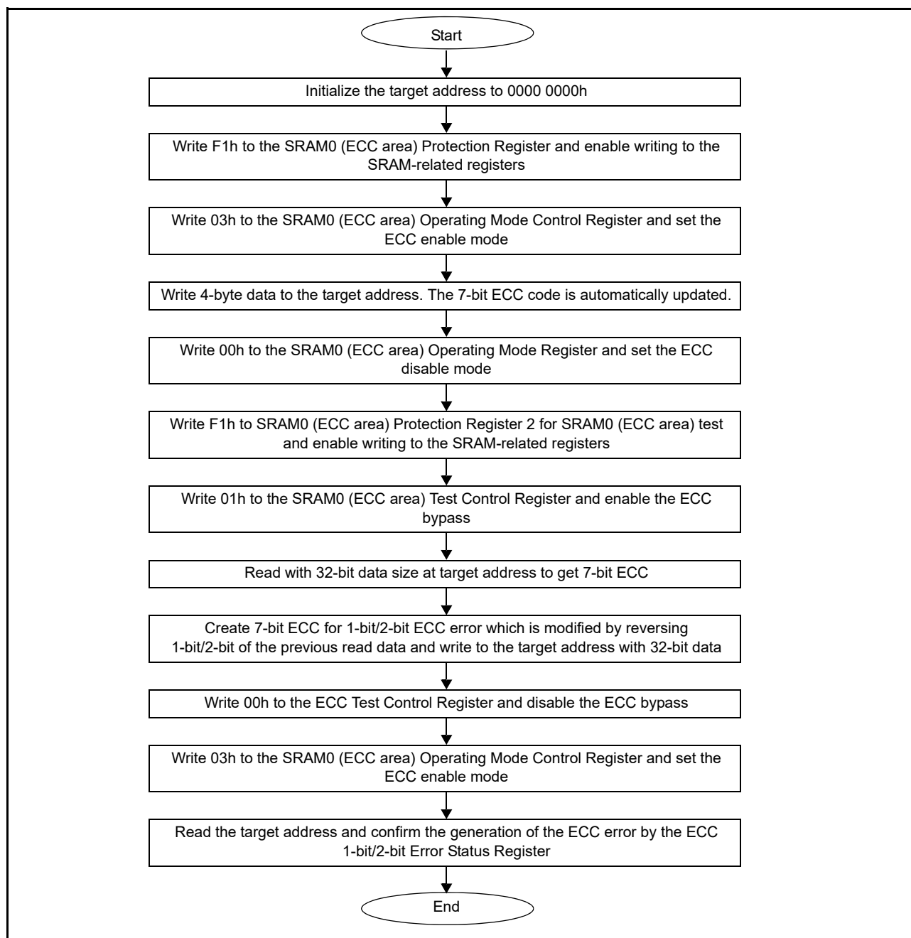
Figure 46.1 ECC decoder testing
