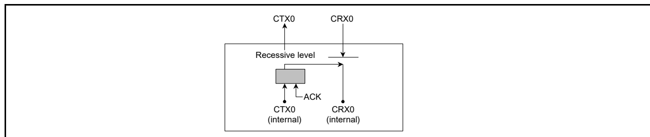
Figure 31.8 Connection when self-test mode 1 is selected
