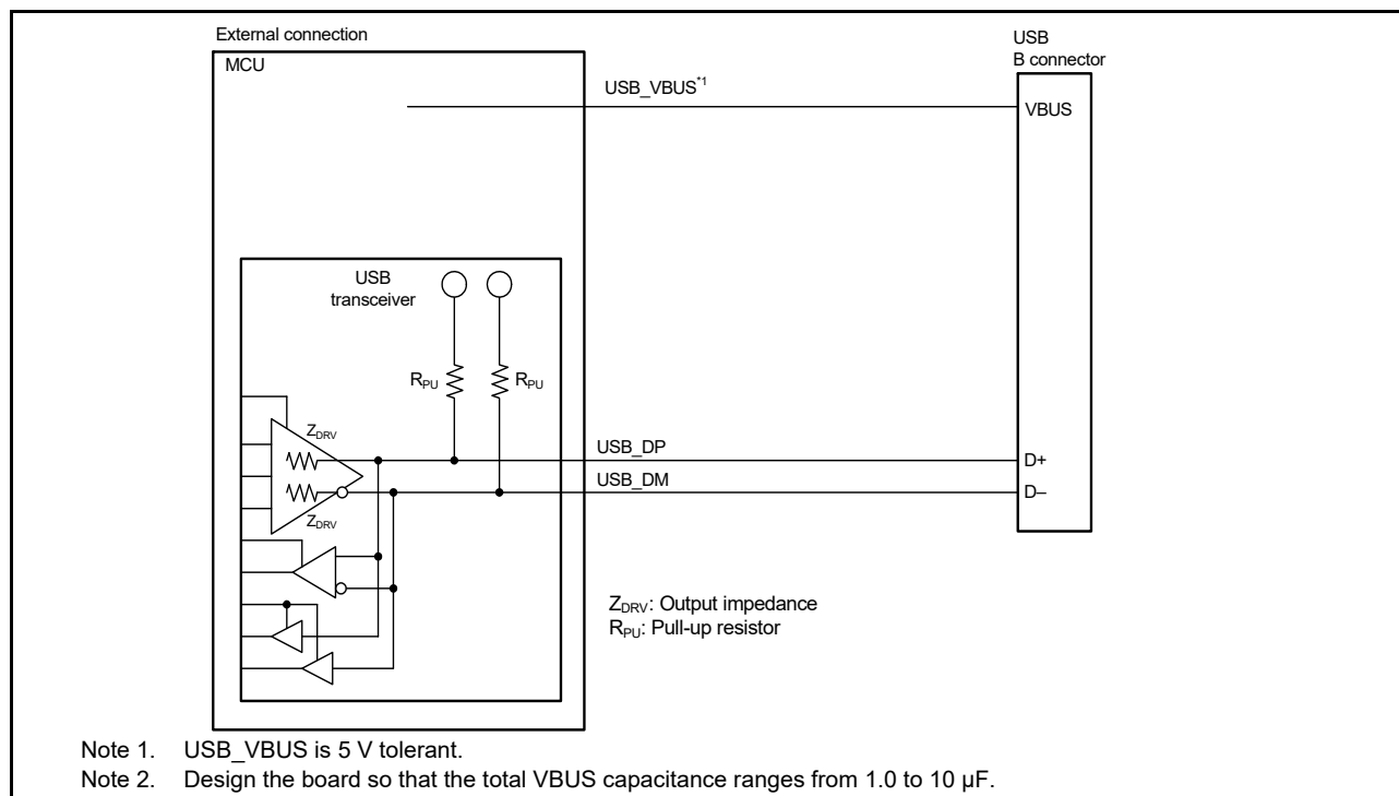
Figure 28.9 Example device connection in bus-powered state 2
