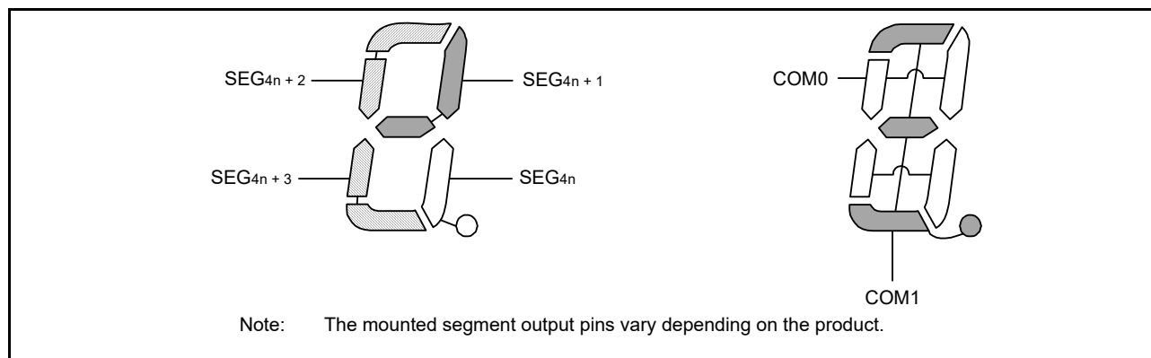
Figure 48.21 Two-time-slice LCD display pattern and electrode connections
