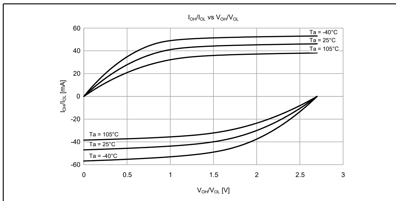
Figure 51.13 V_{OH}/V_{OL} and I_{OH}/I_{OL} temperature characteristics at V_{CC} = 2.7\text{ V} when middle drive output is selected (reference data)
