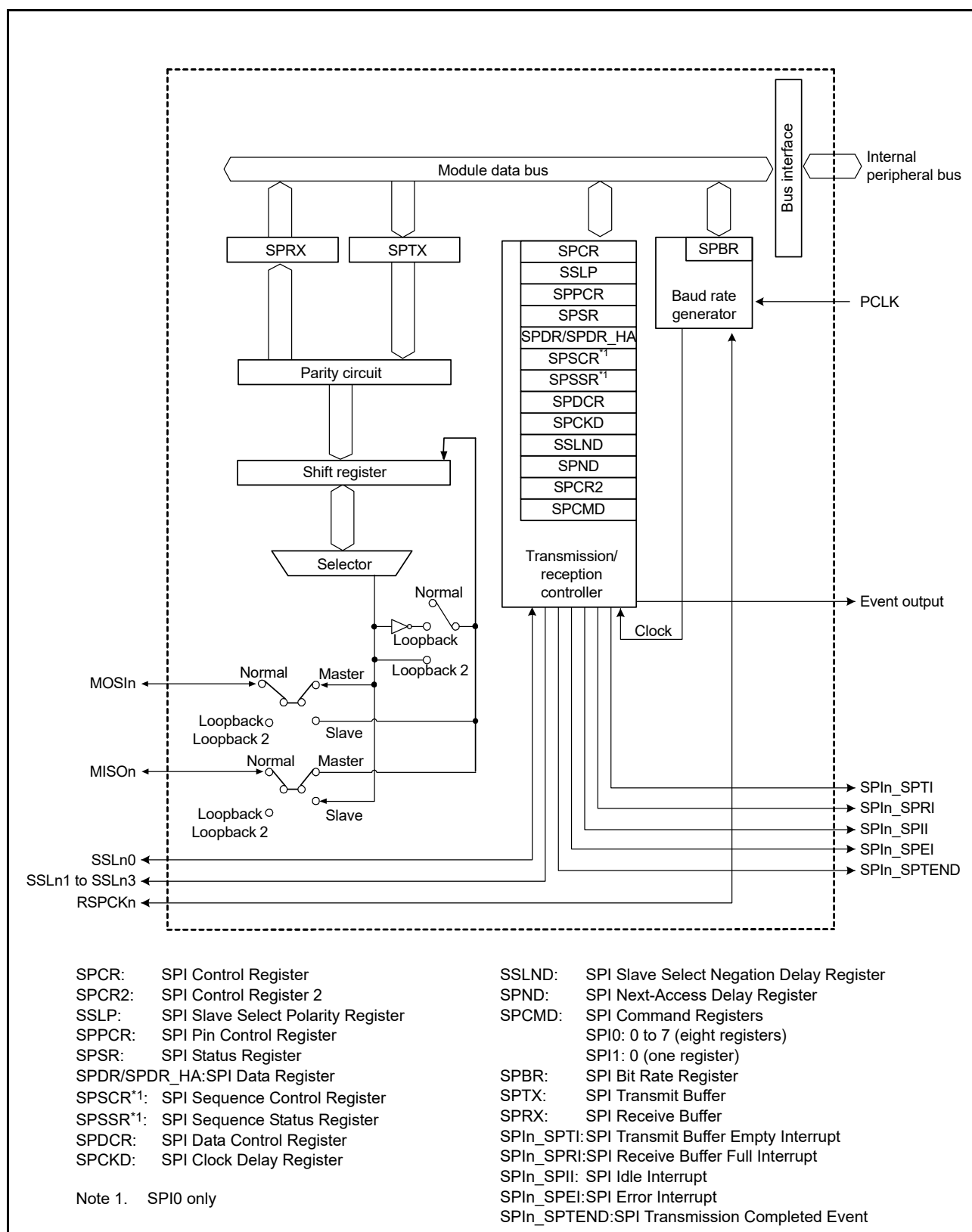
Figure 32.1 SPI block diagram
