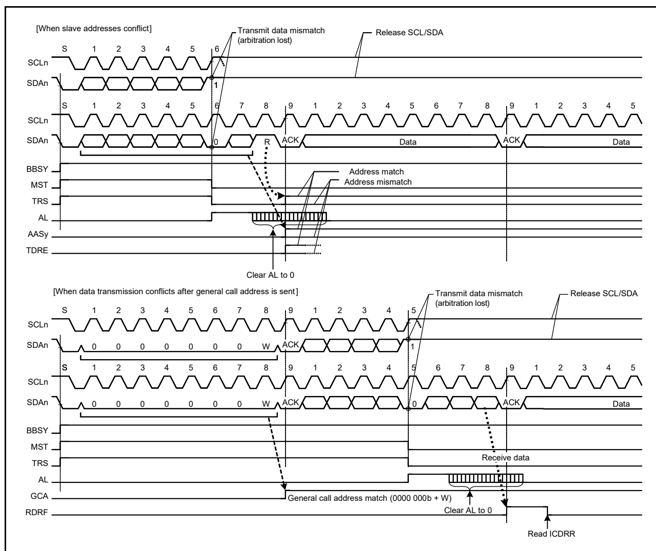
Figure 30.41 Examples of master arbitration-lost detection when MALE = 1
