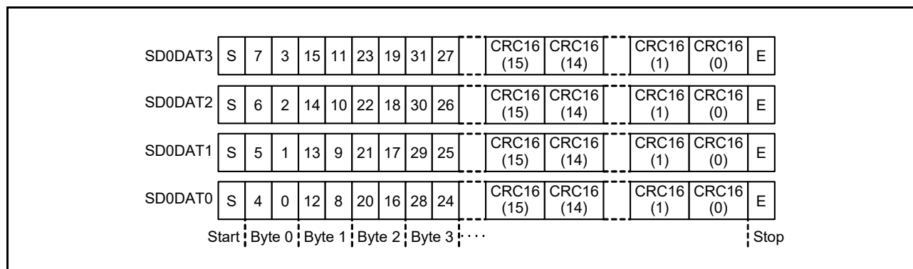
Figure 36.3 SD0DAT in 4-bit width mode
