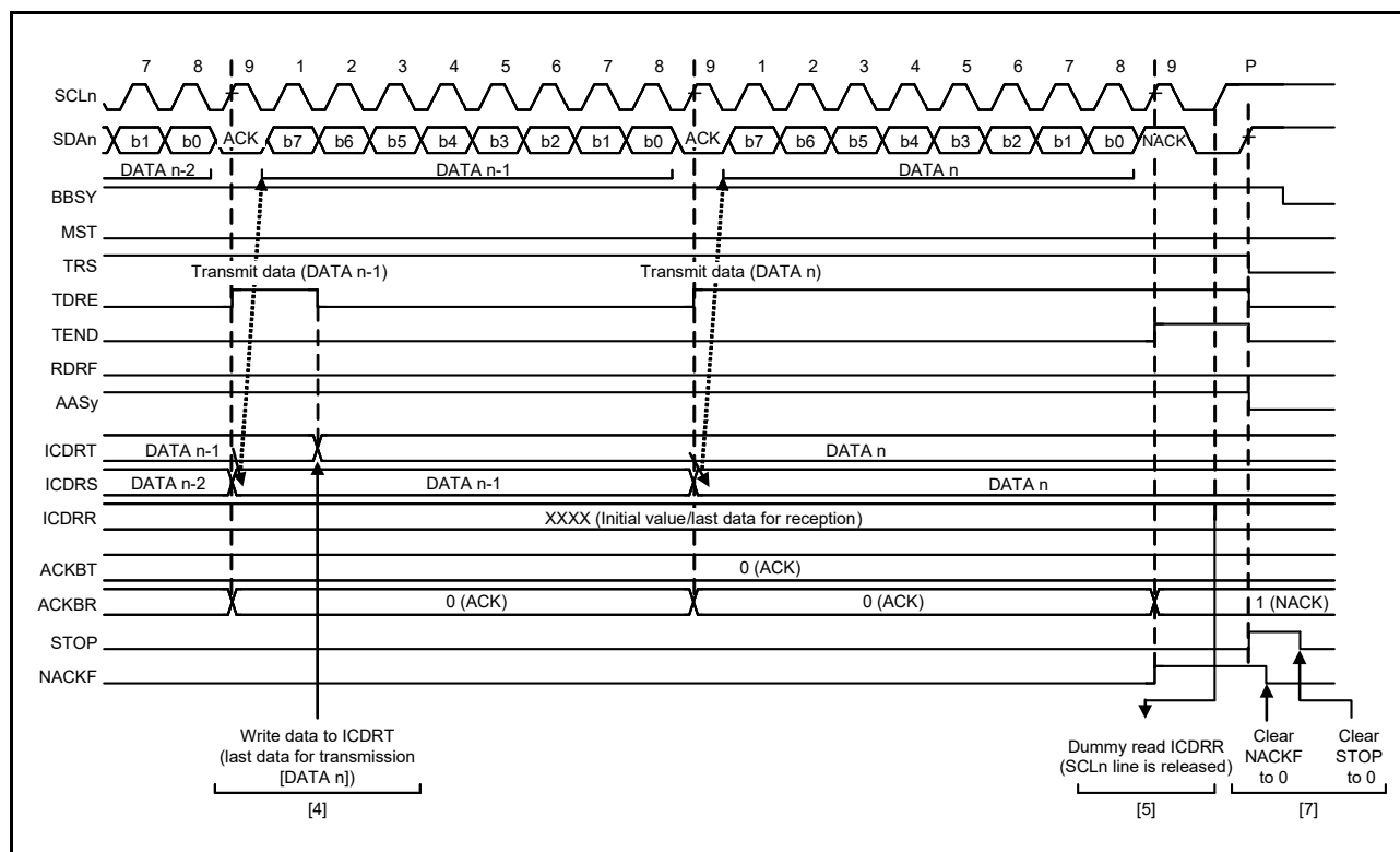
Figure 30.17 Slave transmit operation timing (2)
