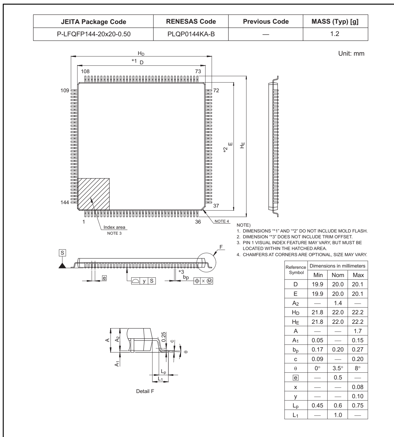
Figure 2.2 LQFP 144-pin
