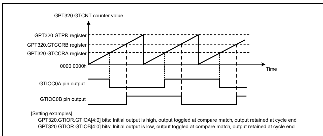
Figure 23.13 Example of toggled output operation (1)
