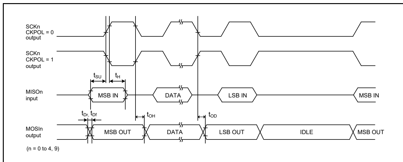
Figure 51.56 SCI simple SPI mode timing (master, CKPH = 1)
