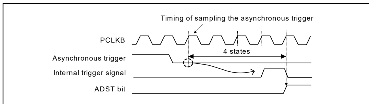
Figure 38.29 Asynchronous trigger input timing
