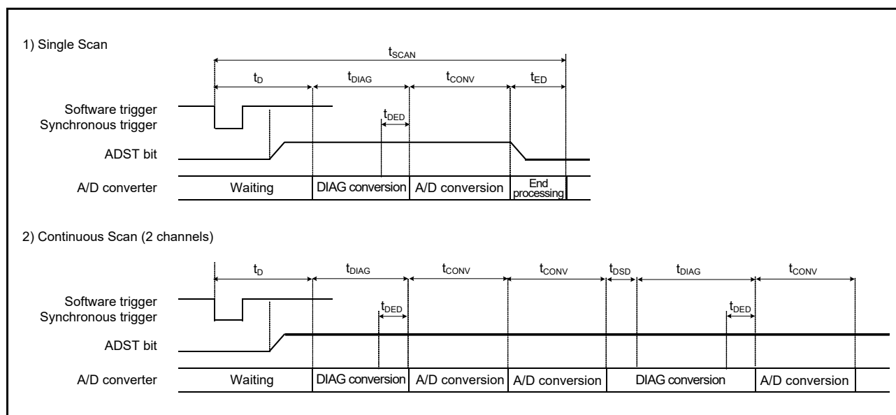
Figure 38.24 Scan conversion timing activated by software or synchronous trigger ELC input
