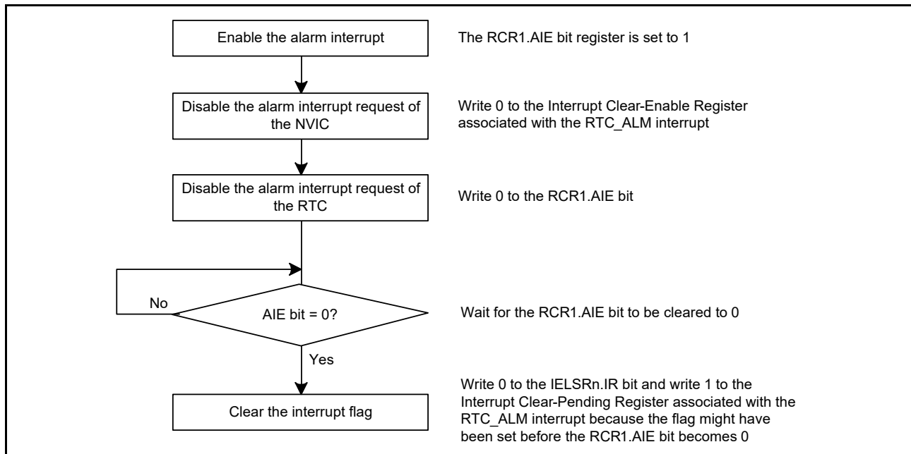
Figure 25.8 Procedure for disabling alarm interrupt request
