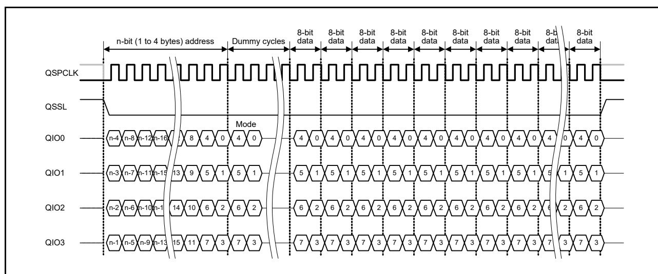
Figure 33.26 Fast Read Quad I/O bus cycle in XIP mode
