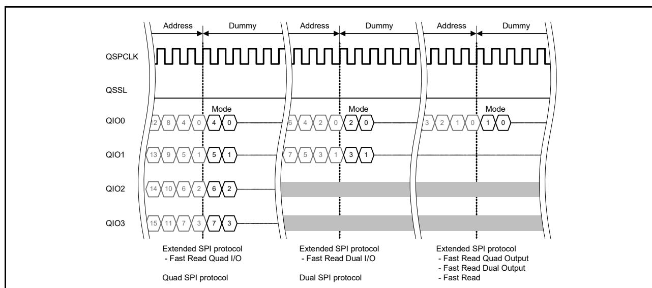
Figure 33.33 XIP mode control data
