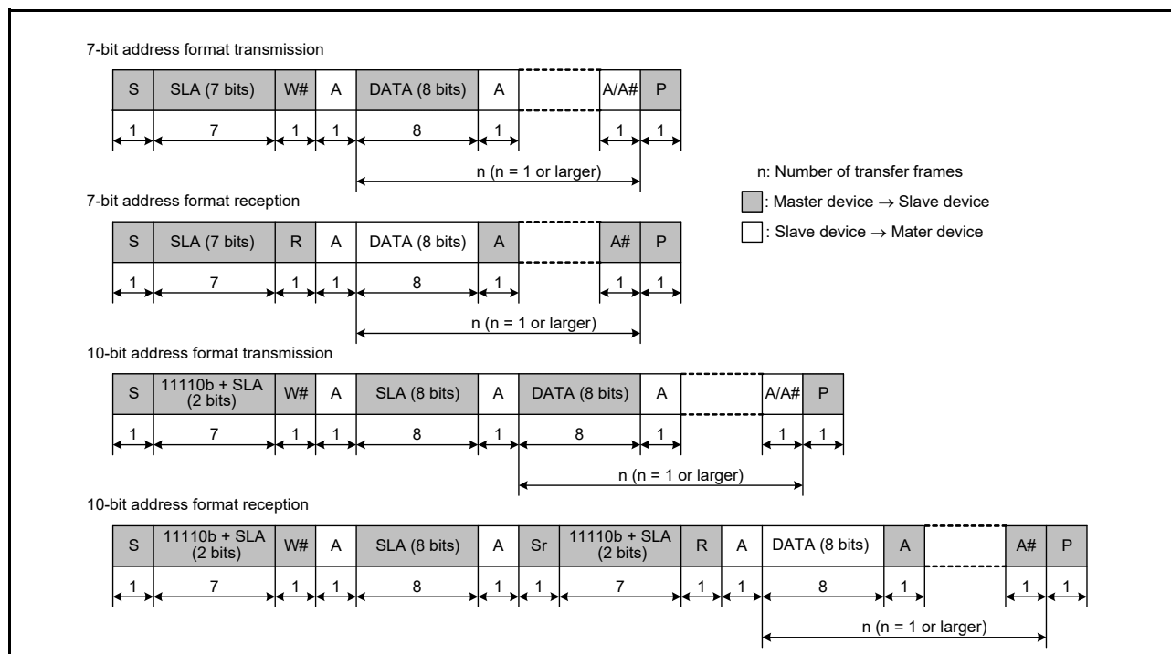
Figure 29.58 I 2 C bus format
