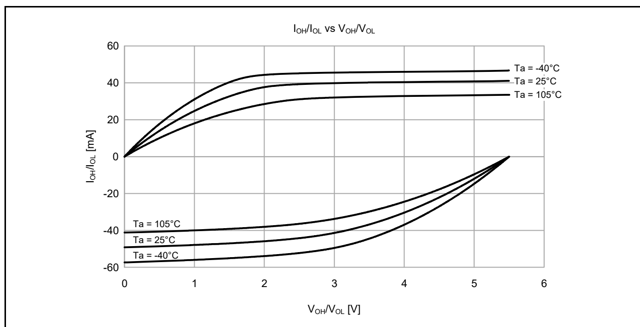
Figure 51.6 V_{OH}/V_{OL} and I_{OH}/I_{OL} temperature characteristics at V_{CC} = 5.5 V when low drive output is selected (reference data)
