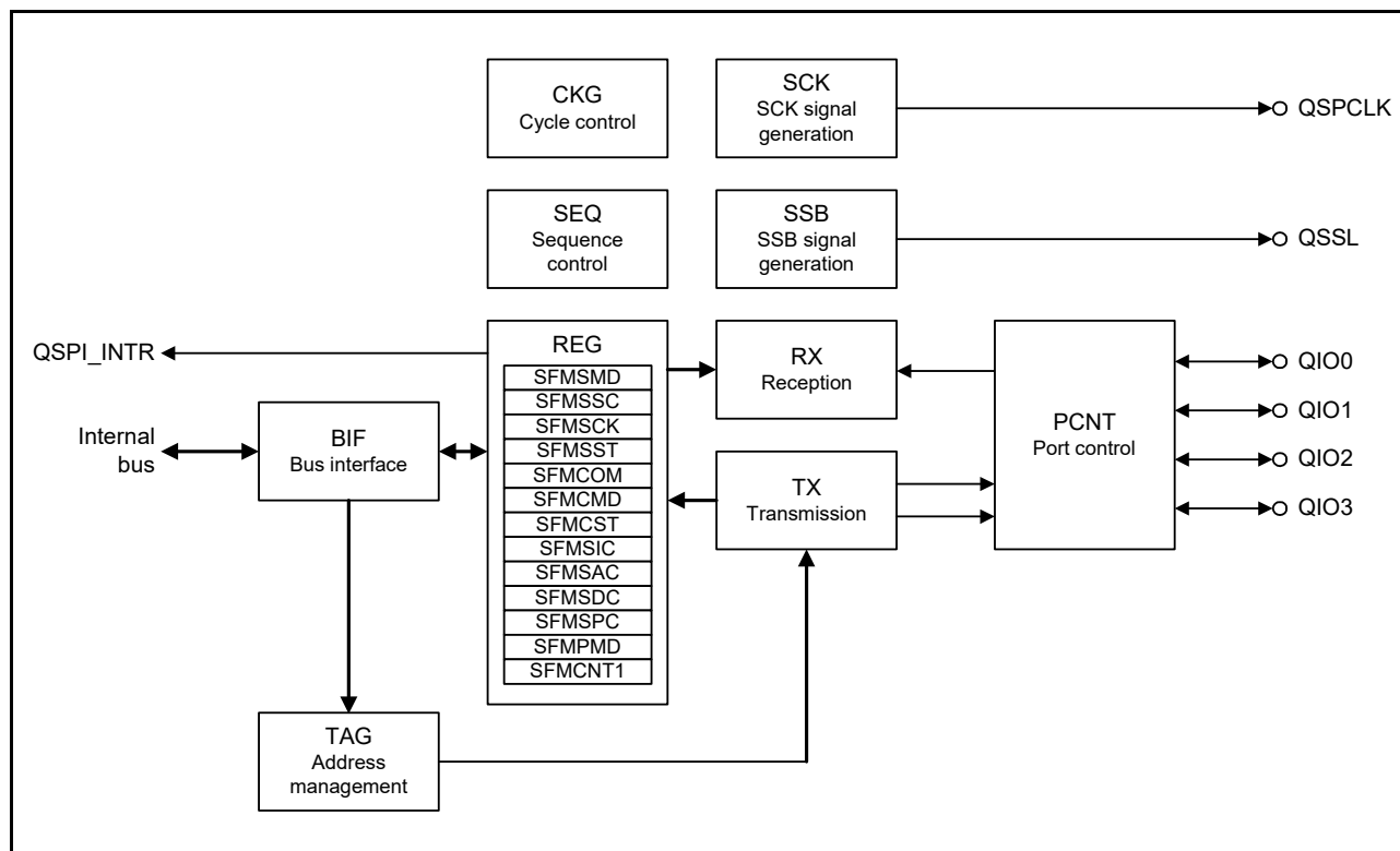
Figure 33.1 QSPI block diagram
