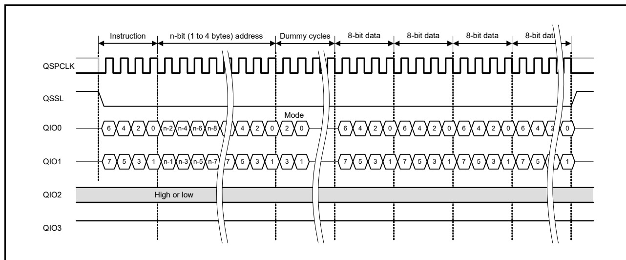
Figure 33.6 Dual SPI protocol example for Fast Read
