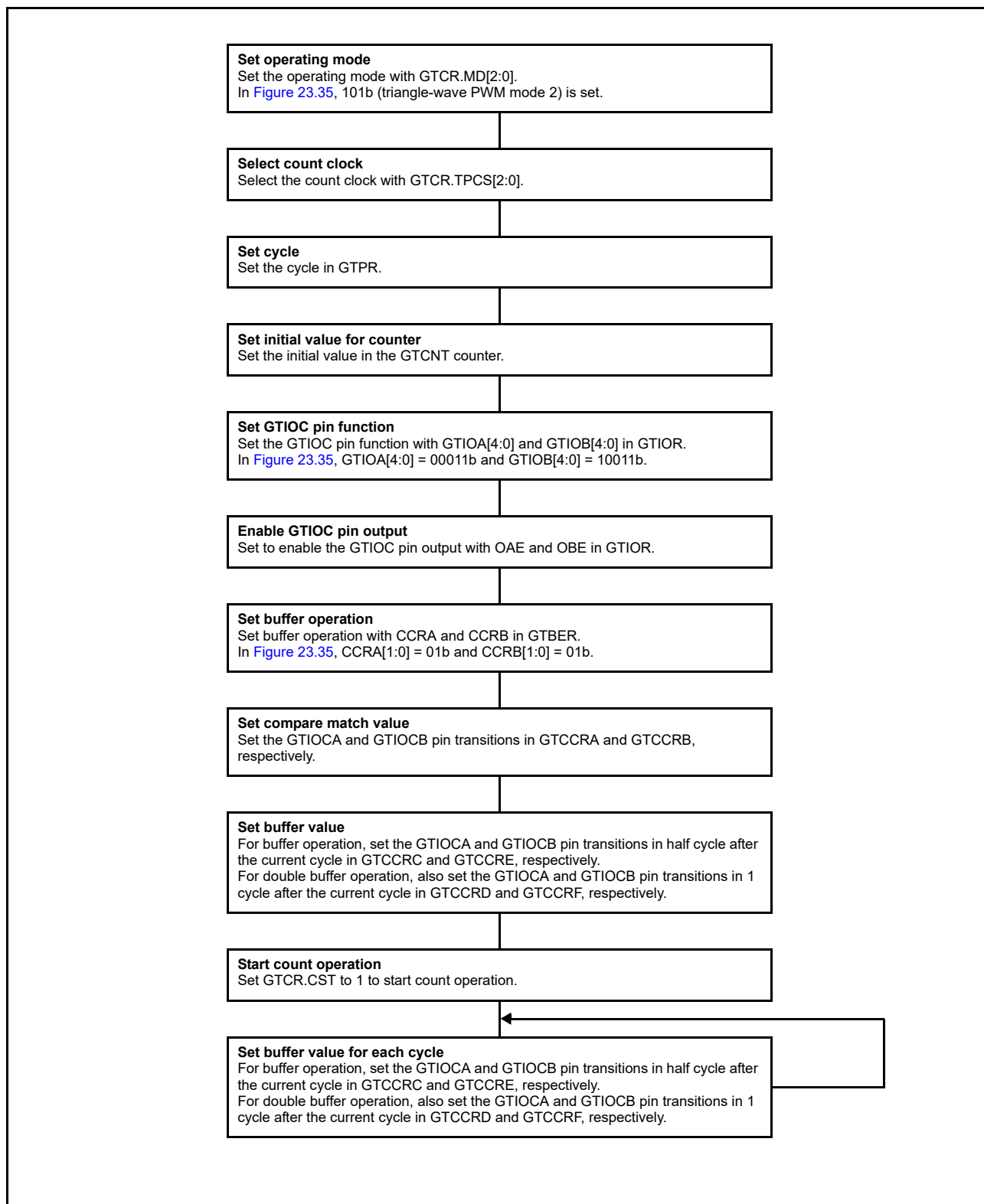
Figure 23.36 Example for setting triangle-wave PWM mode 2
