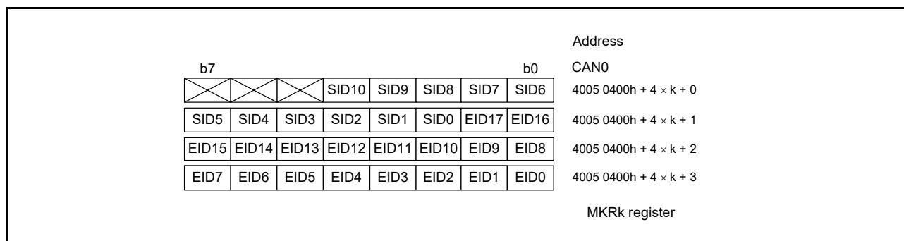
Figure 31.14 Structure of the MKRk registers (k = 0 to 7)
