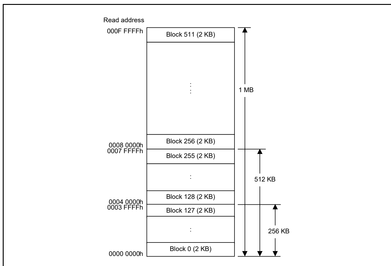
Figure 47.2 Mapping of the code flash memory
