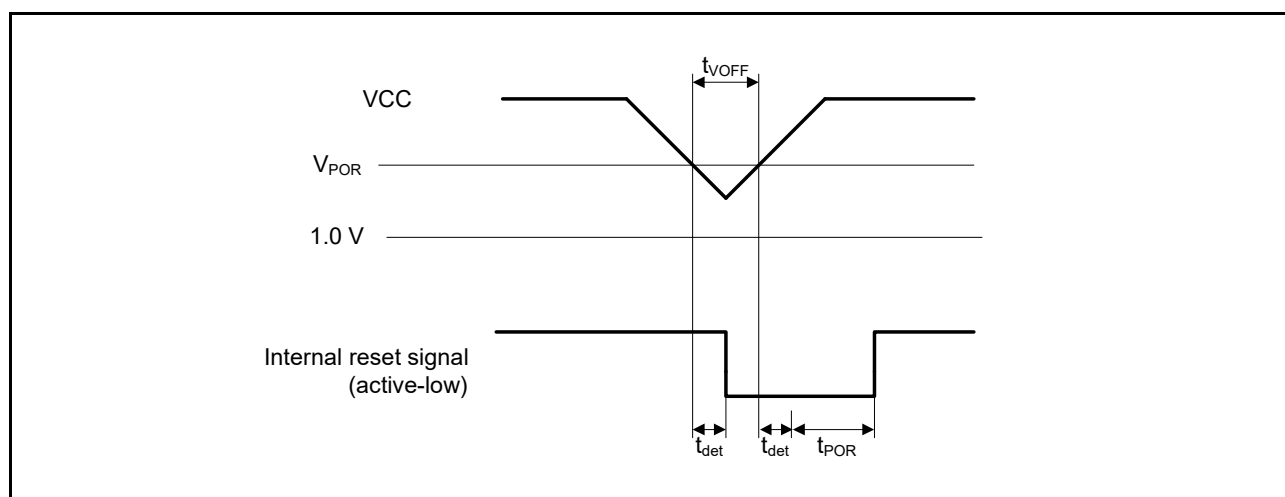
Figure 51.85 Voltage detection reset timing
