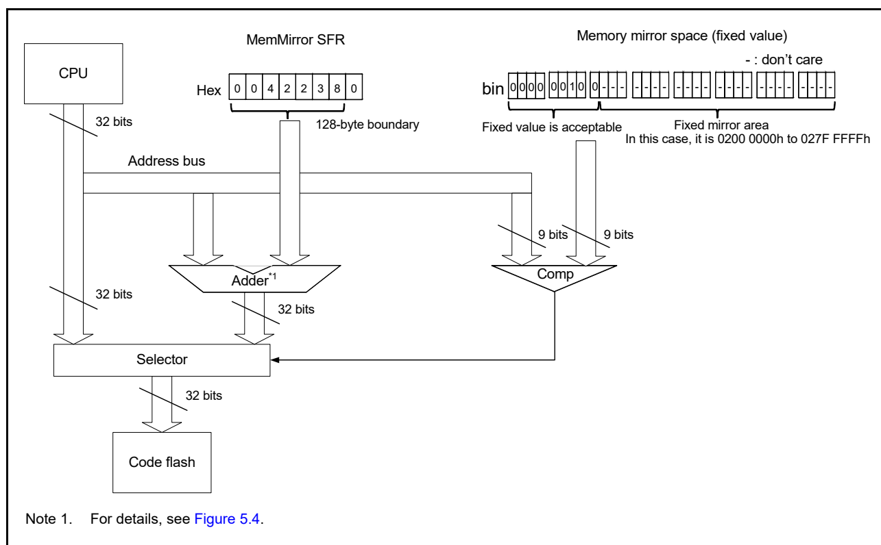
Figure 5.2 MMF block diagram
