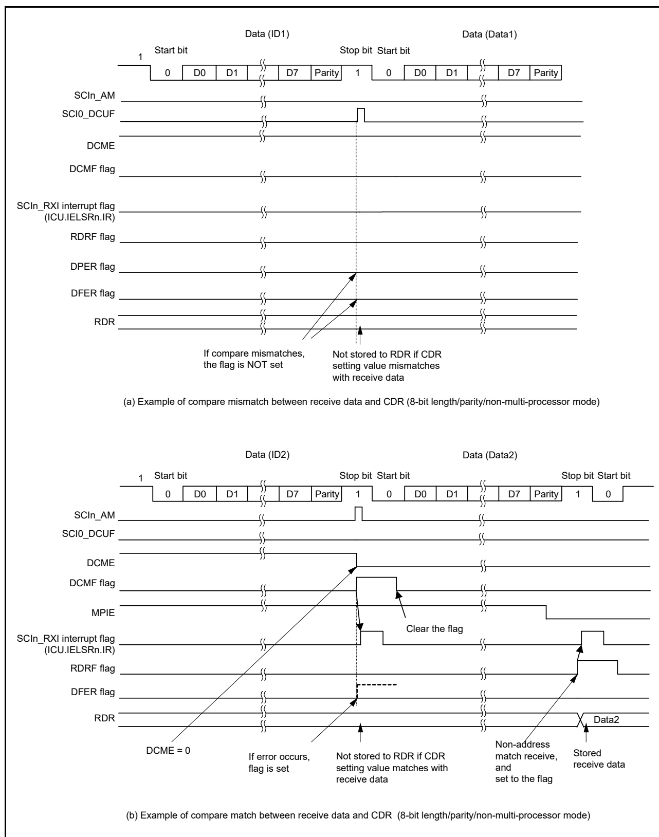
Figure 29.5 Example of address match (1) in non-multi-processor mode
