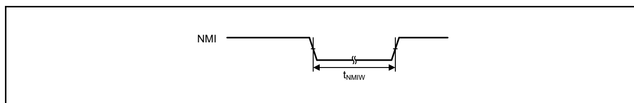
Figure 51.38 NMI interrupt input timing
