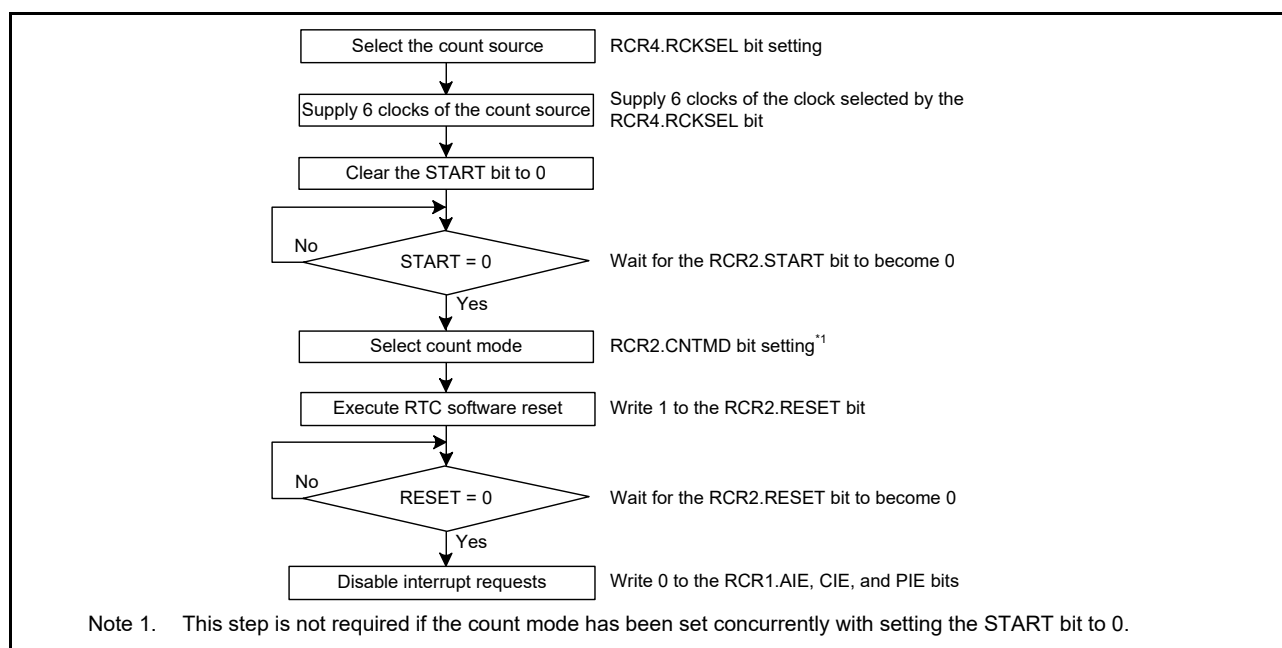
Figure 25.14 Initialization procedure
