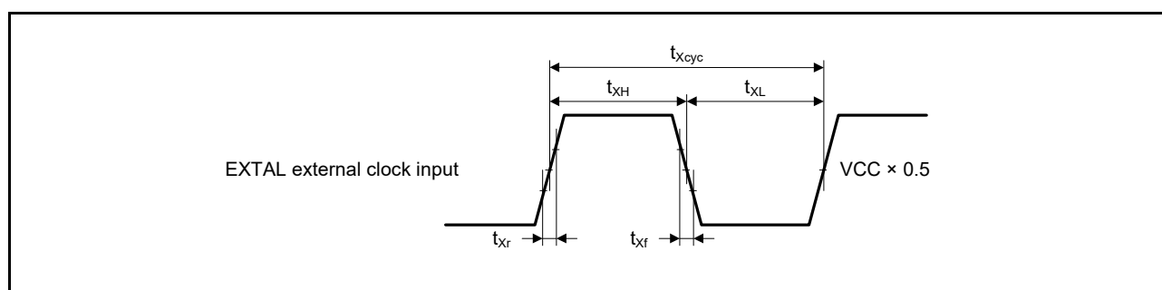
Figure 51.27 EXTERNAL external clock input timing
