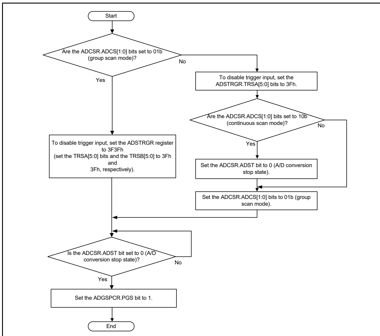
Figure 38.15 Flow for ADGSPCR.PGS bit setting
