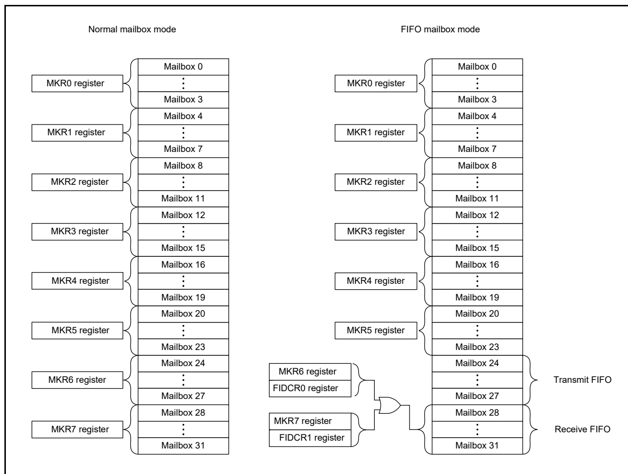
Figure 31.16 Association between mask registers and mailboxes
