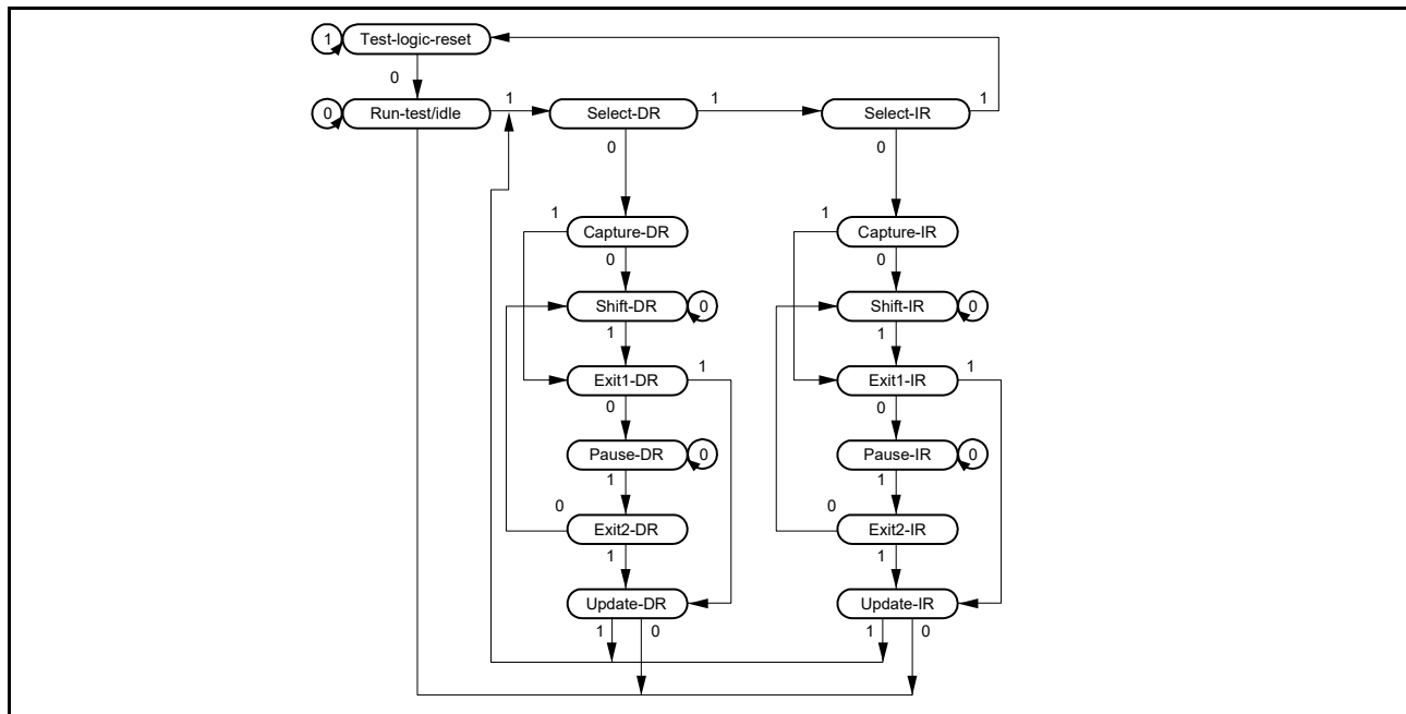
Figure 37.2 State transition diagram of TAP controller
