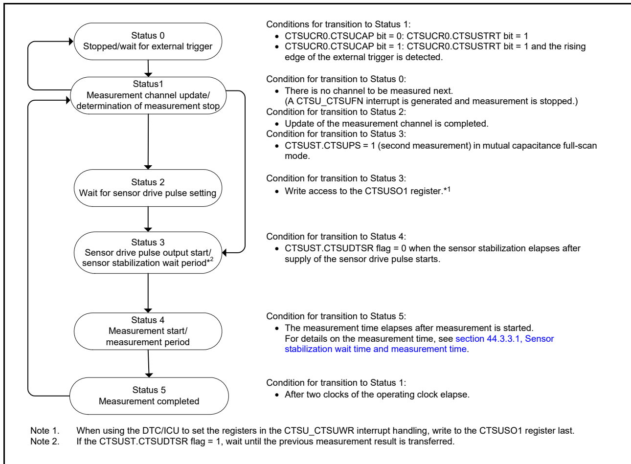
Figure 44.11 Status operation transitions
