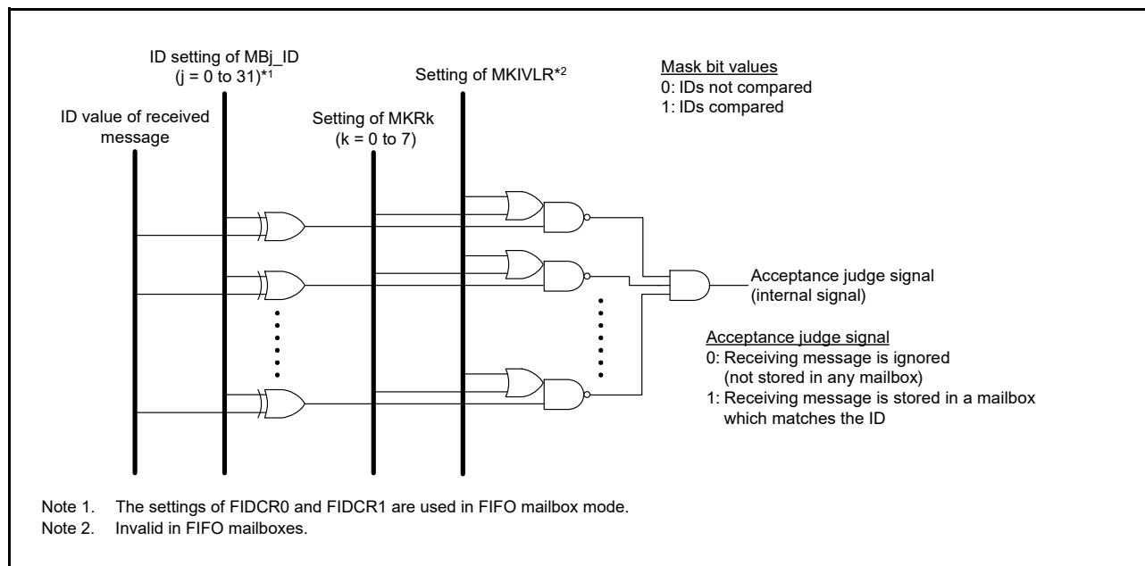
Figure 31.17 Acceptance filtering
