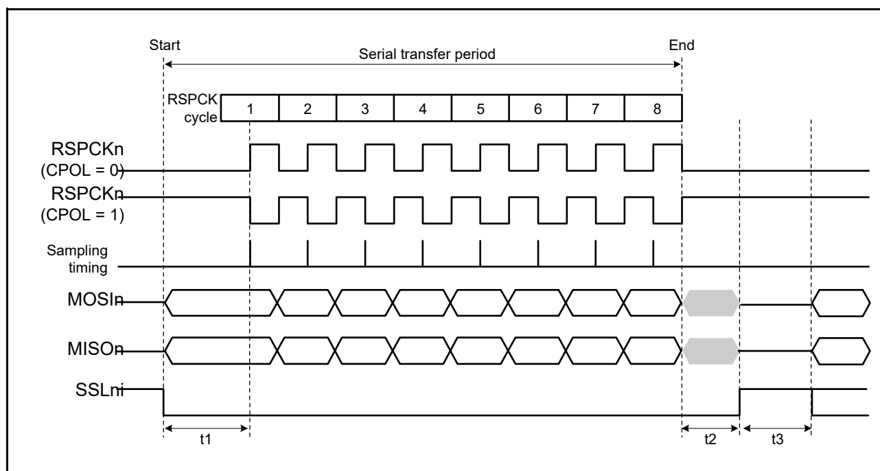
Figure 32.26 SPI transfer format when CPHA = 0
