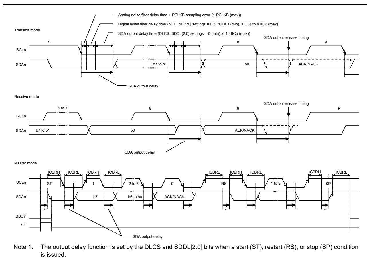
Figure 30.22 SDA output delay function
