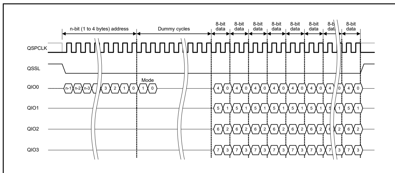
Figure 33.24 Fast Read Quad Output bus cycle in XIP mode
