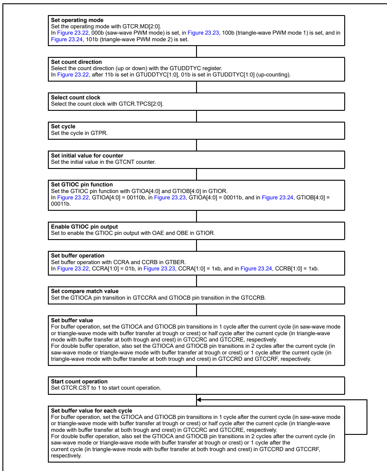
Figure 23.25 Example for setting GTCCRA and GTCCRB buffer operation with output compare
