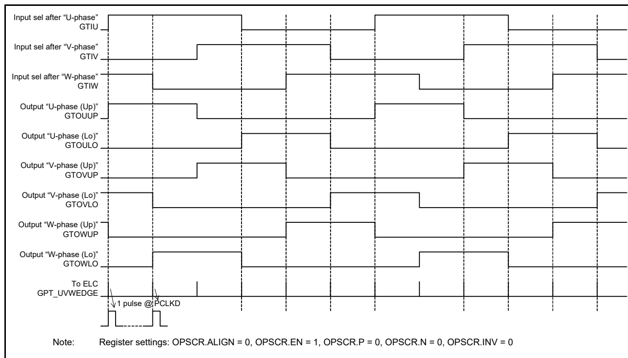
Figure 23.78 6-phase level output operation example
