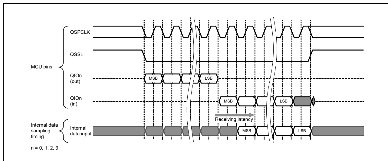
Figure 33.15 Receiving latency
