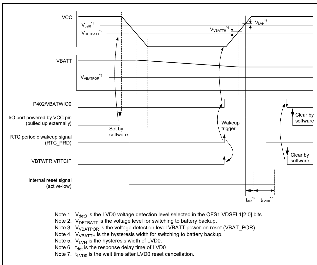
Figure 12.6 VBATT wakeup function timing diagram
