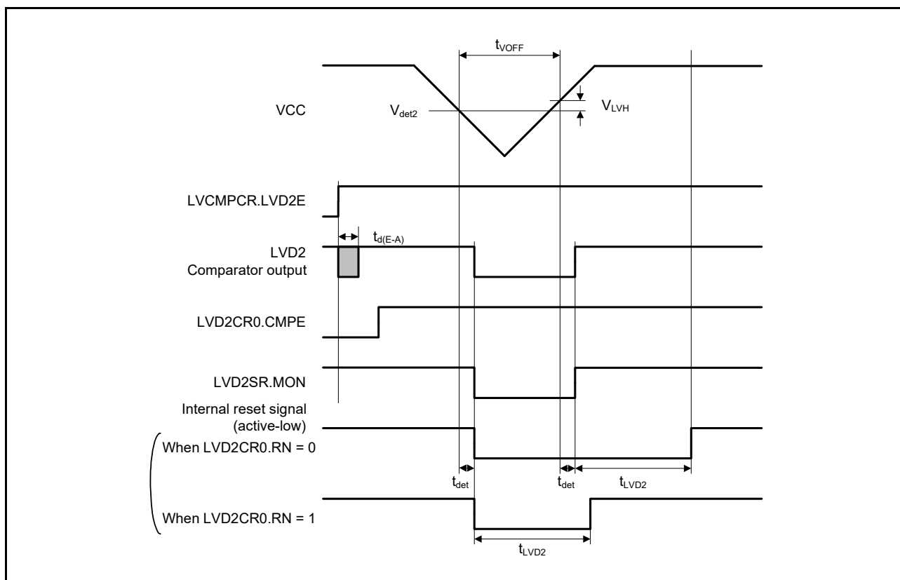
Figure 51.89 Voltage detection circuit timing (V det2 )
