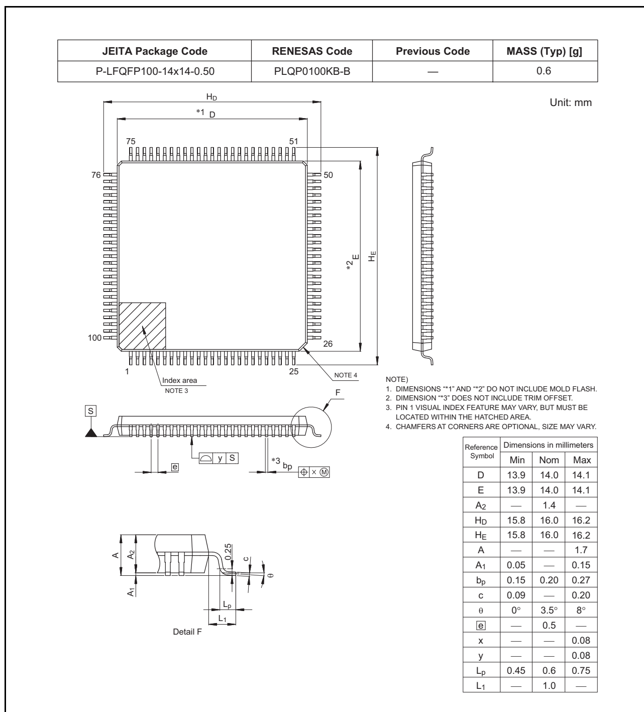
Figure 2.5 LQFP 100-pin
