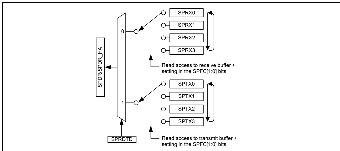
Figure 32.6 Configuration of SPDR/SPDR_HA for read access (SPI0)
