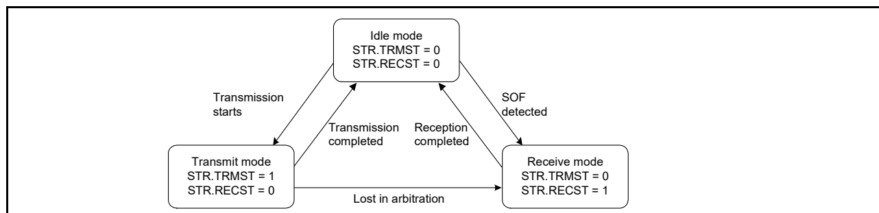
Figure 31.10 Sub-modes of CAN operation mode
