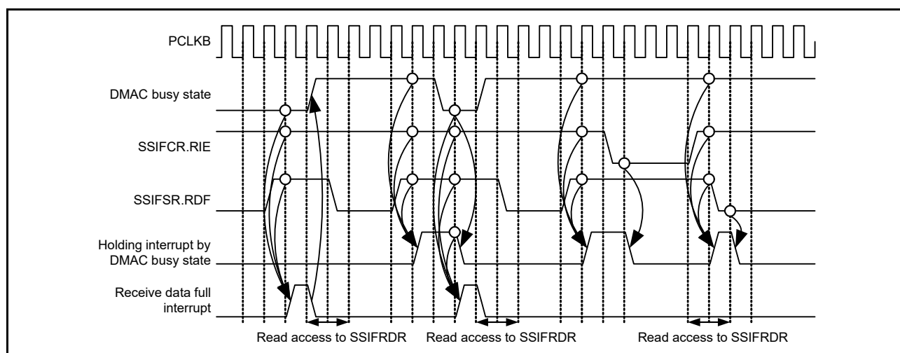
Figure 35.20 Timing of receive data full interrupt
