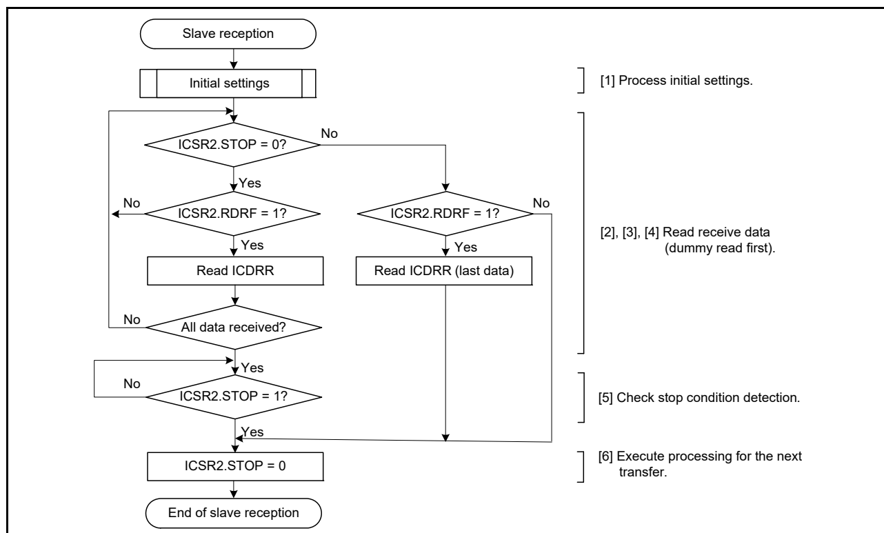
Figure 28.18 Example slave reception flow
