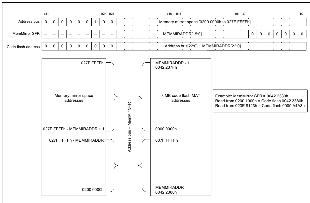
Figure 5.1 MMF operation
