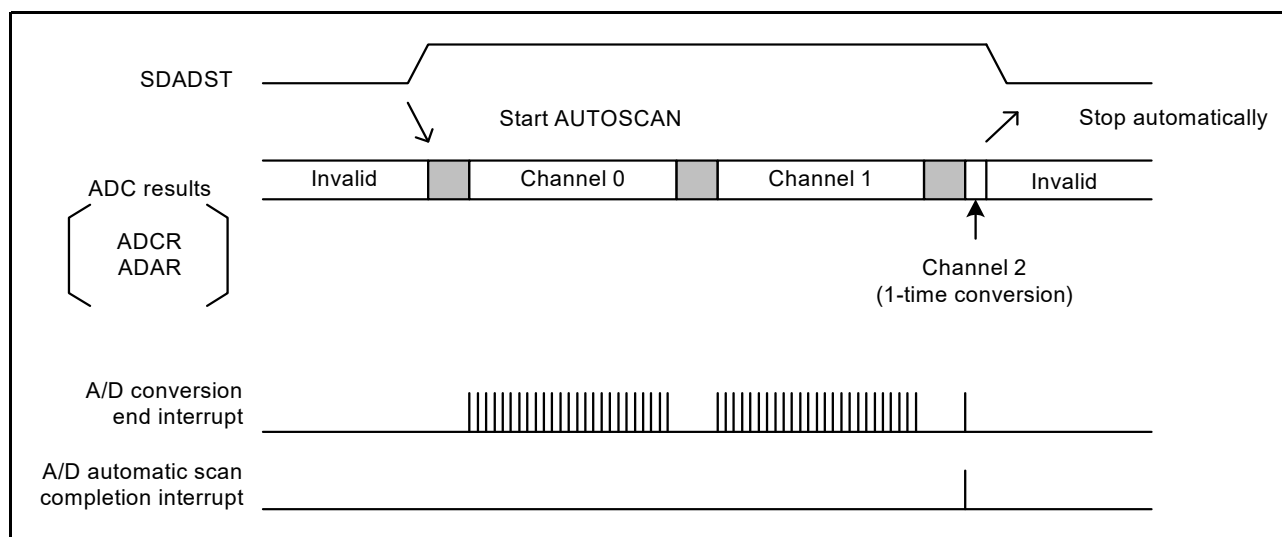
Figure 33.14 Example for one-shot operation
