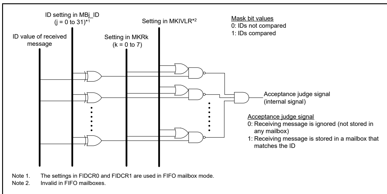
Figure 29.17 Acceptance filtering
