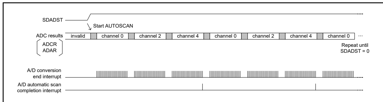
Figure 33.13 Example for skipping the conversion channels
