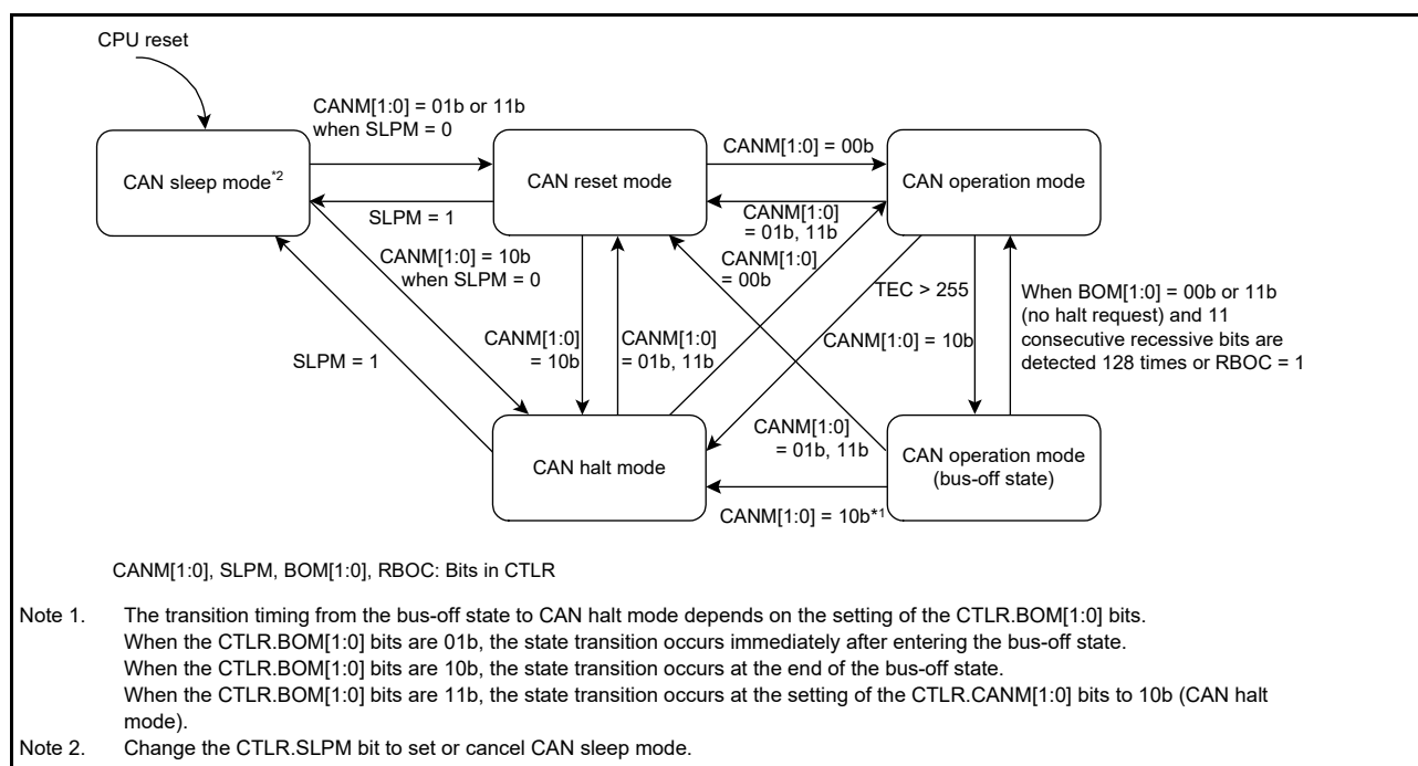
Figure 29.9 Transition between different operation modes
