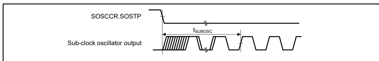
Figure 47.28 Sub-clock oscillation start timing
