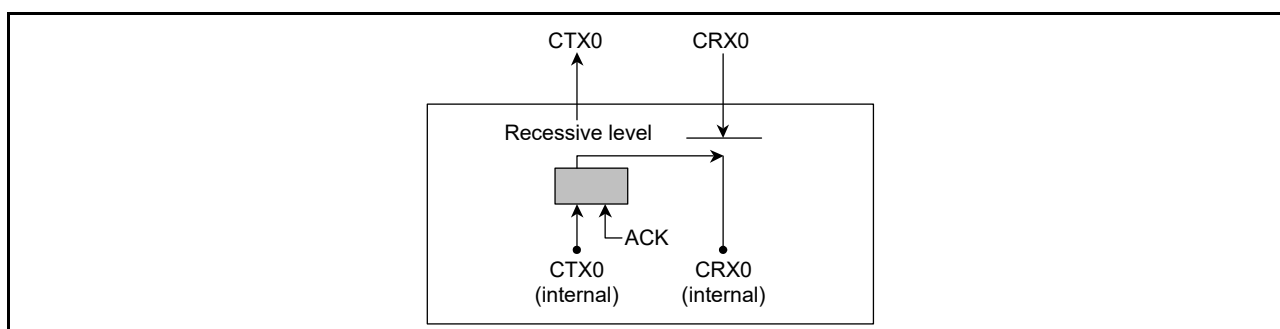
Figure 29.8 Connection when self-test mode 1 is selected
