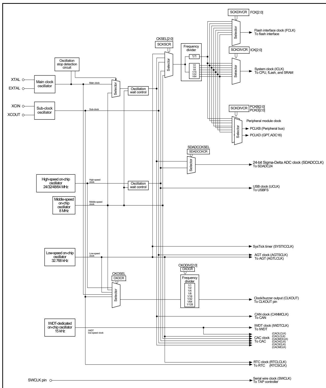
Figure 9.1 Clock generation circuit block diagram
