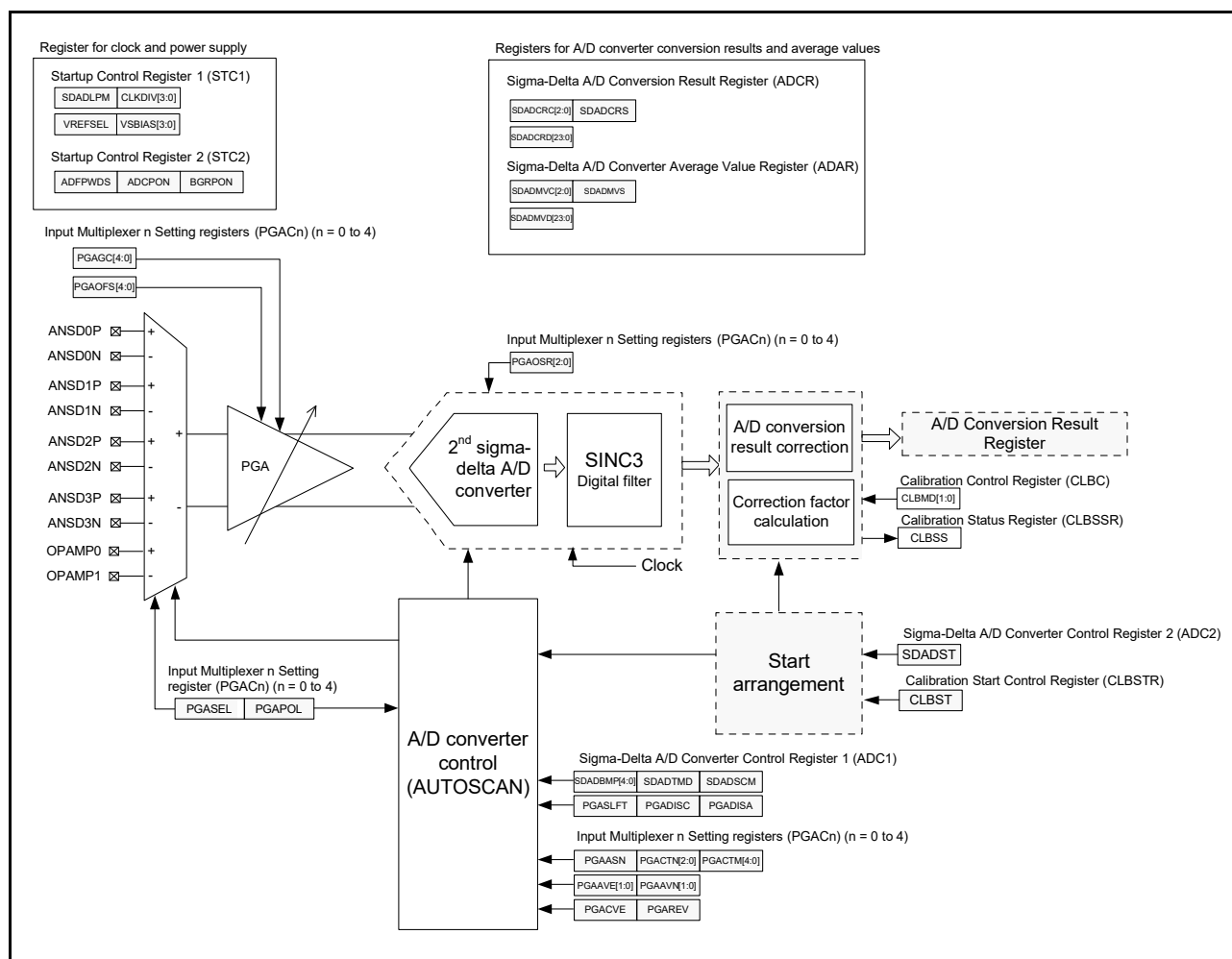
Figure 33.3 SDADC24 block diagram
