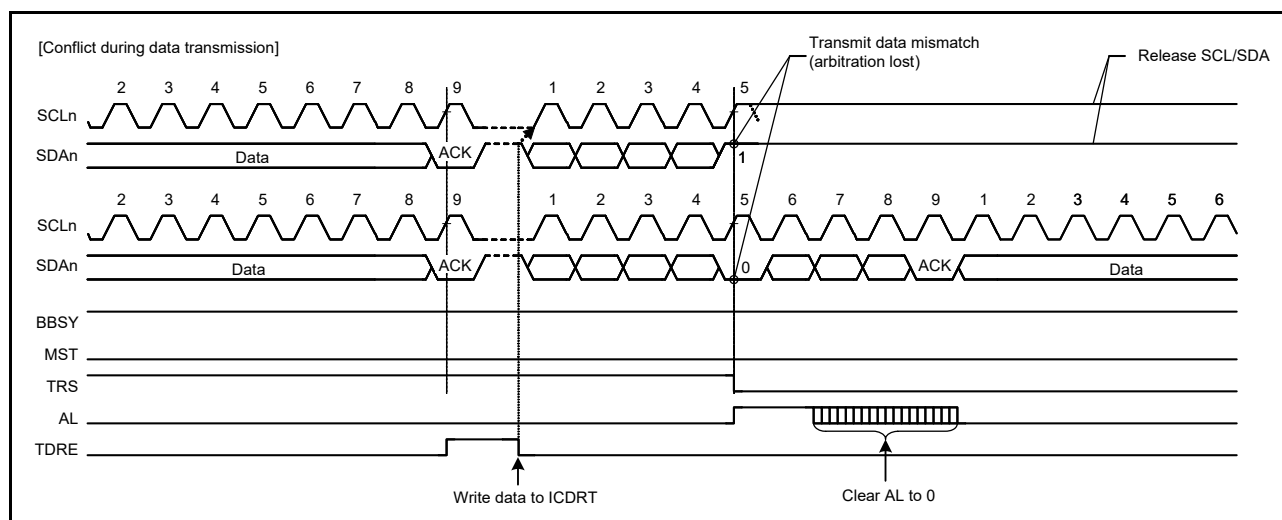
Figure 28.44 Example of slave arbitration-lost detection (SALE = 1)
