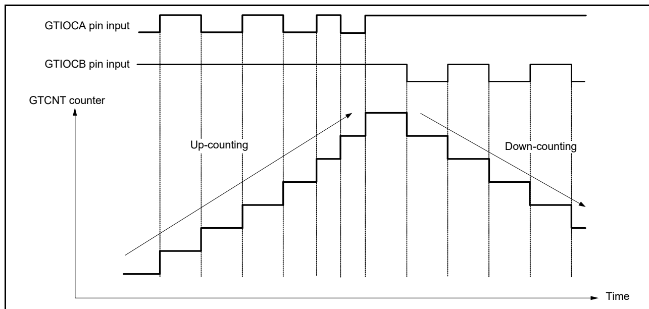
Figure 21.73 Example of phase counting mode 3 (C)
