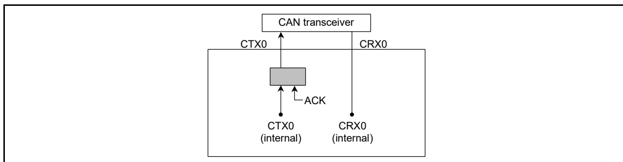
Figure 29.7 Connection when self-test mode 0 is selected
