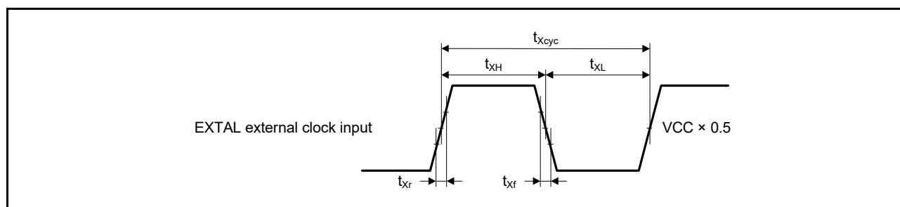
Figure 47.25 EXTAL external clock input timing
