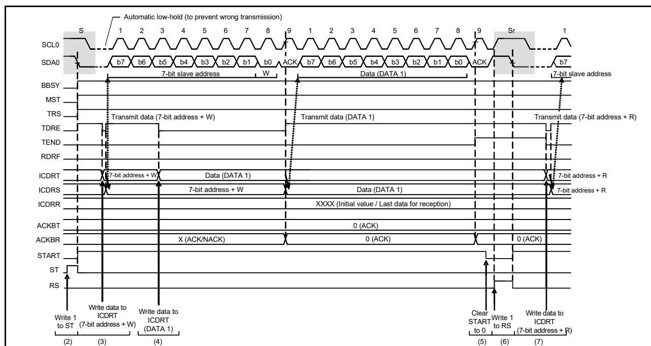
Figure 28.46 Restart condition issue timing after master transmission
