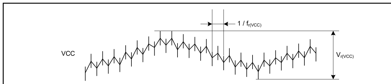
Figure 47.24 Ripple waveform
