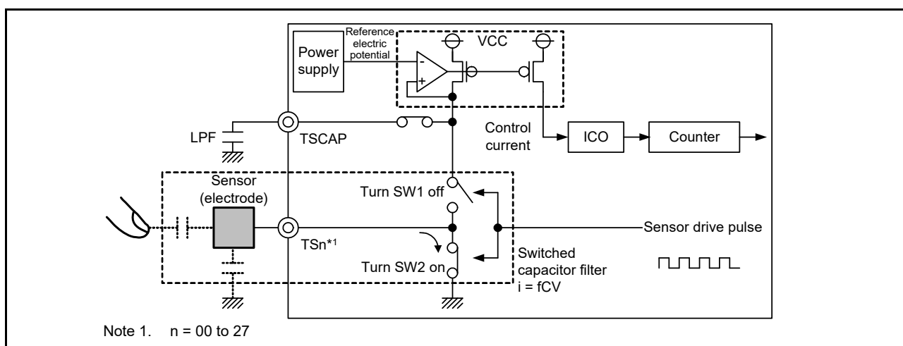
Figure 40.6 Discharging operation
