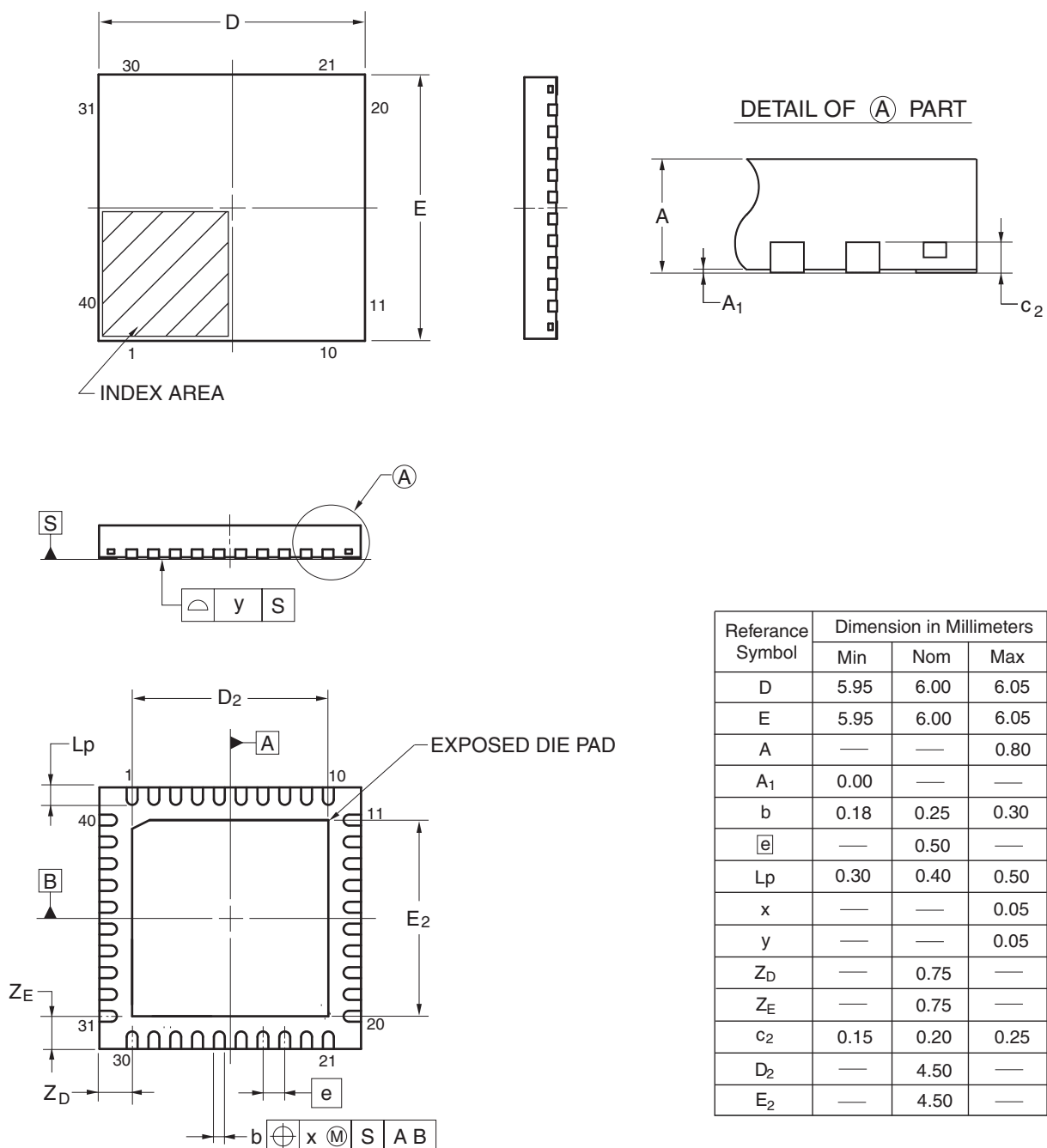
Figure 2.5 QFN 40-pin
