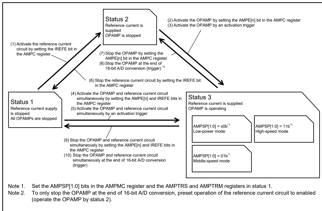
Figure 37.5 OPAMP state transitions
