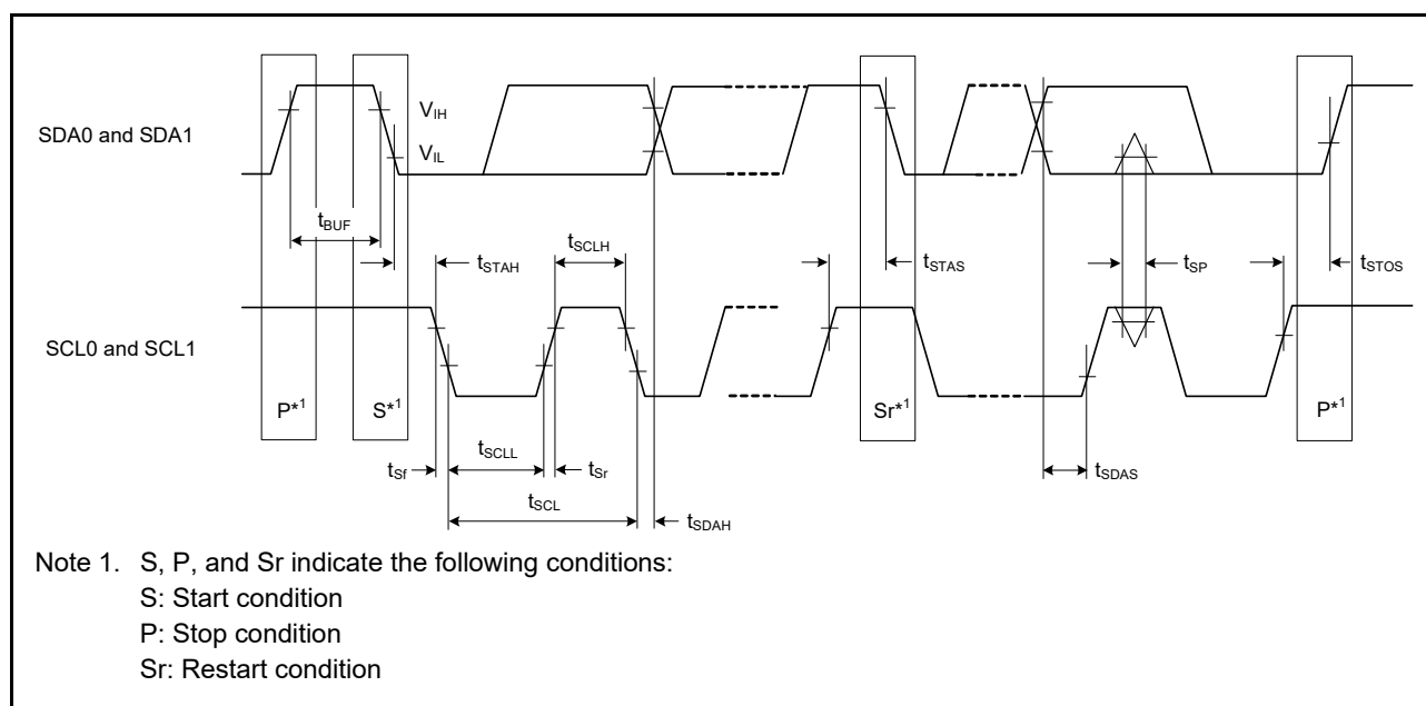
Figure 47.57 I2C bus interface input/output timing
