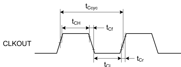
Figure 47.58 CLKOUT output timing
