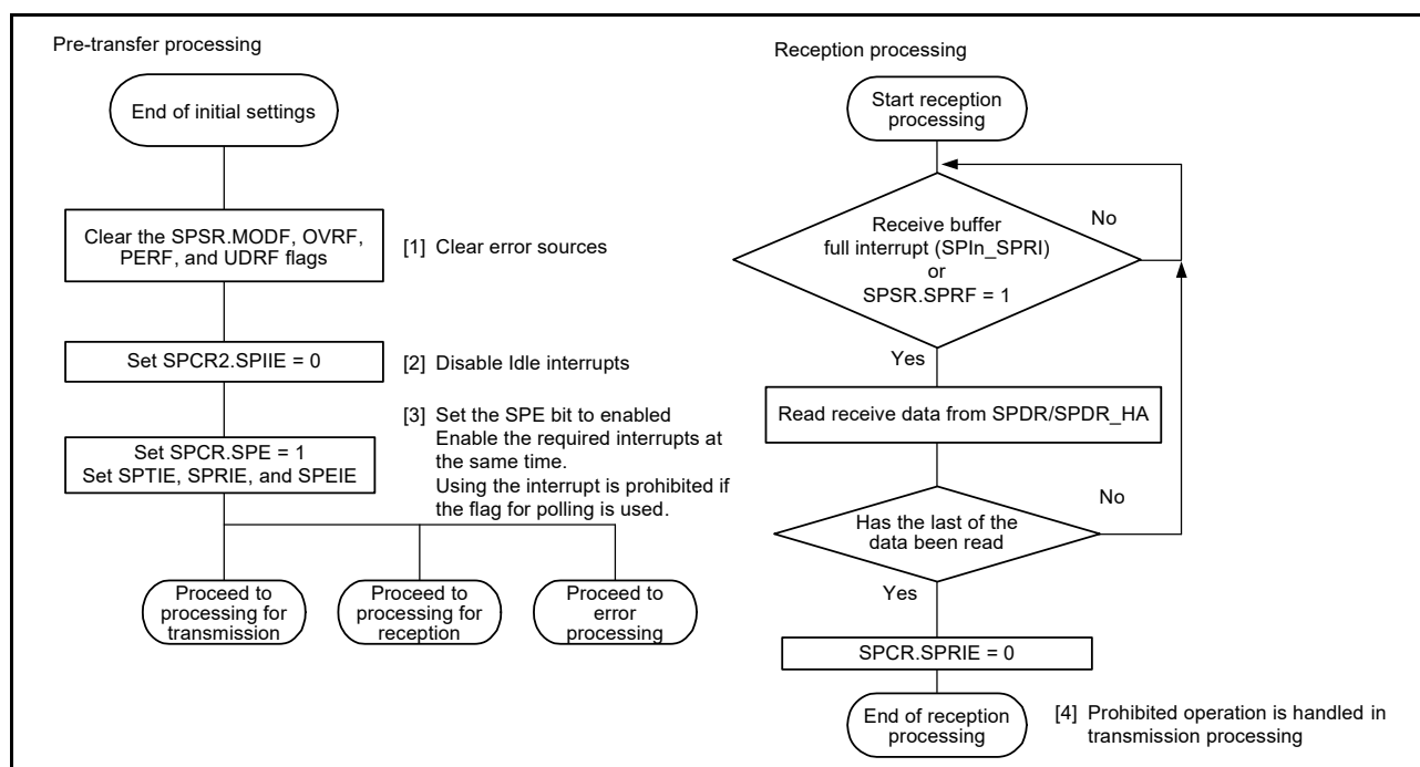
Figure 30.34 Reception flow in master mode
