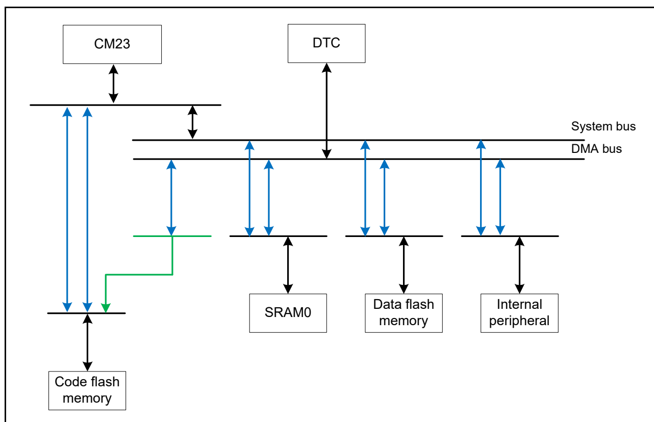
Figure 14.1 Bus configuration
