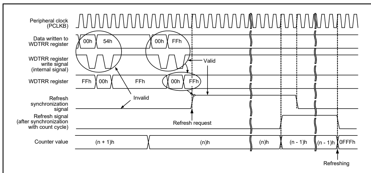
Figure 24.6 WDT refresh operation waveforms when \text{WDTCR.CKS}[3:0] = 0100\text{b} , \text{WDTCR.TOPS}[1:0] = 01\text{b}
