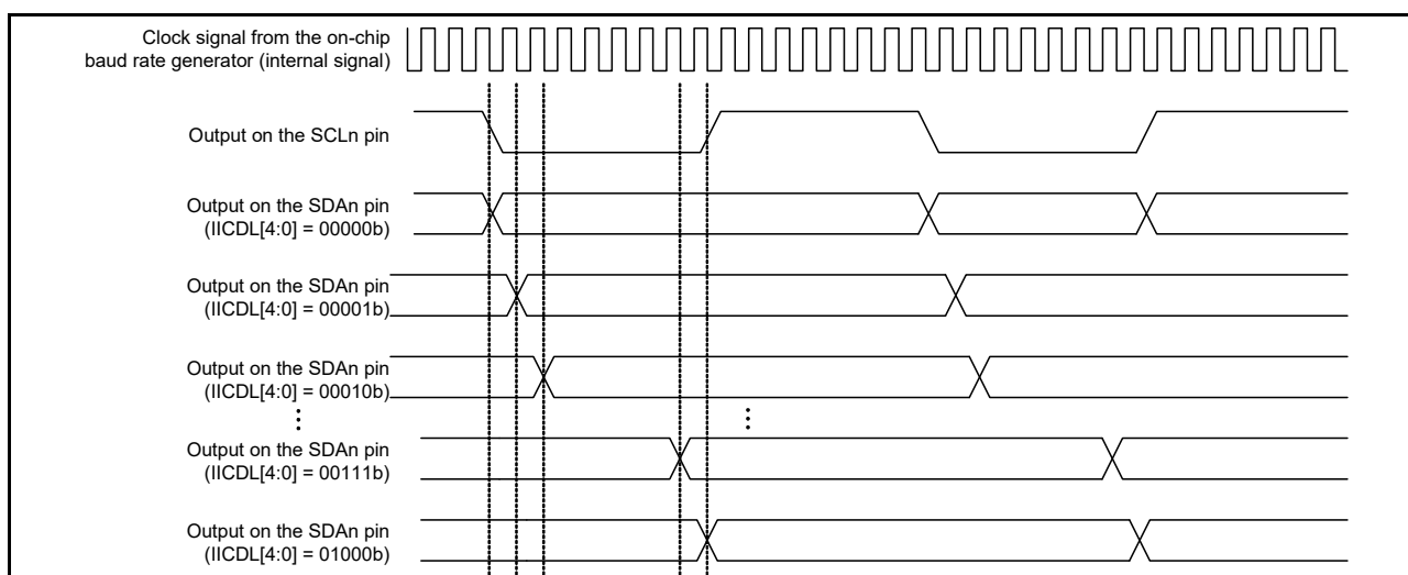
Figure 27.62 Timing of delays in SDAn output
