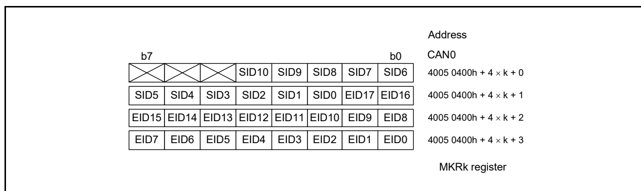
Figure 30.14 Structure of MKRk (k = 0 to 7)
