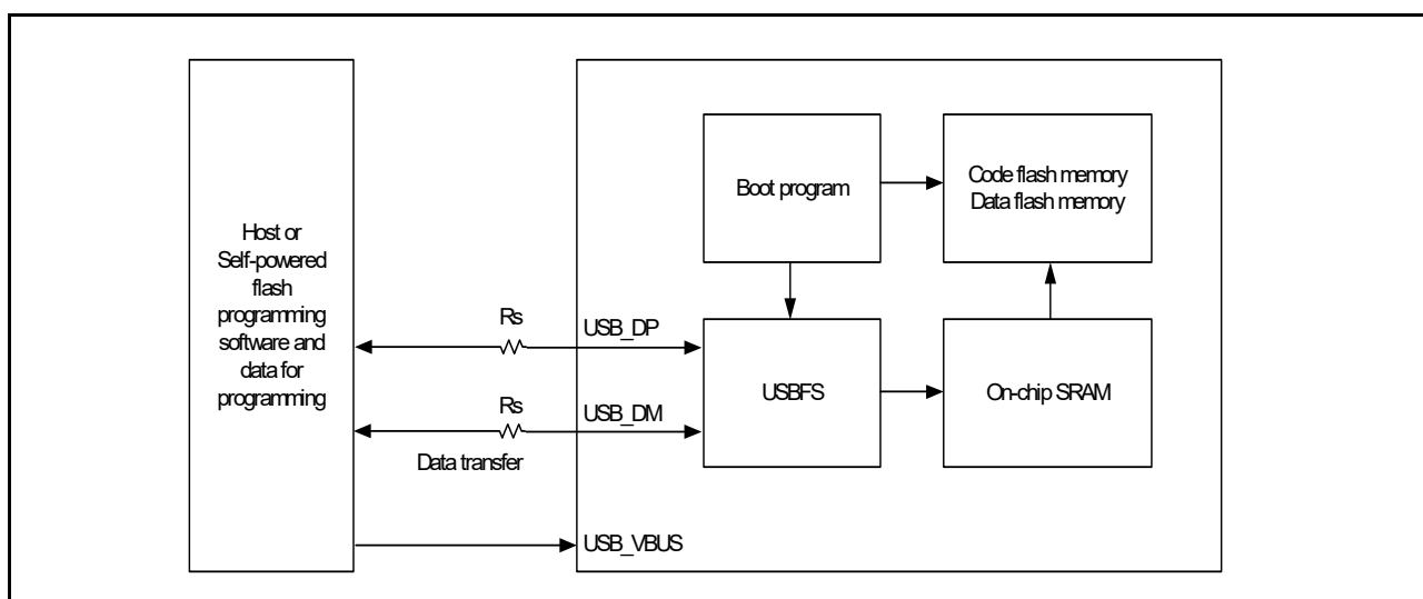
Figure 44.10 System configuration in USB boot mode
