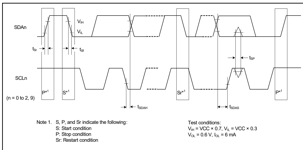
Figure 48.51 SCI simple IIC mode timing
