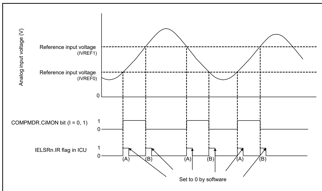
Figure 39.4 Operating example of ACMPLPi (i = 0, 1) when window function is enabled
