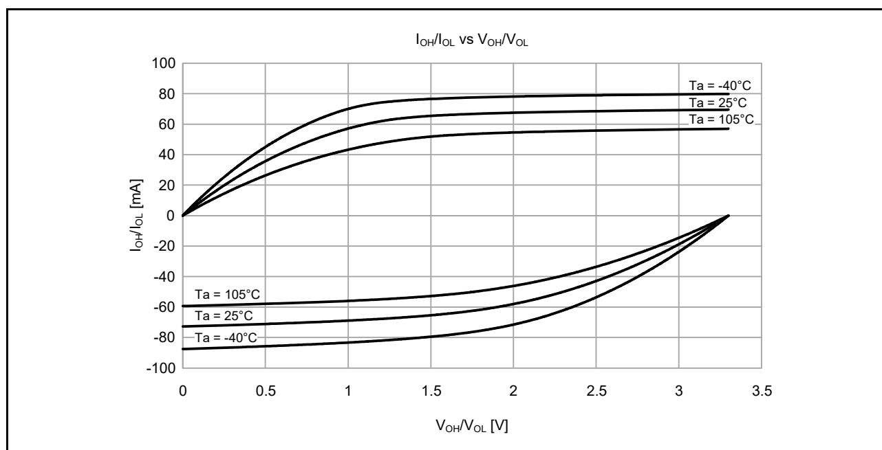
Figure 48.14 V_{OH}/V_{OL} and I_{OH}/I_{OL} temperature characteristics at V_{CC} = 3.3 V when middle drive output is selected (reference data)
