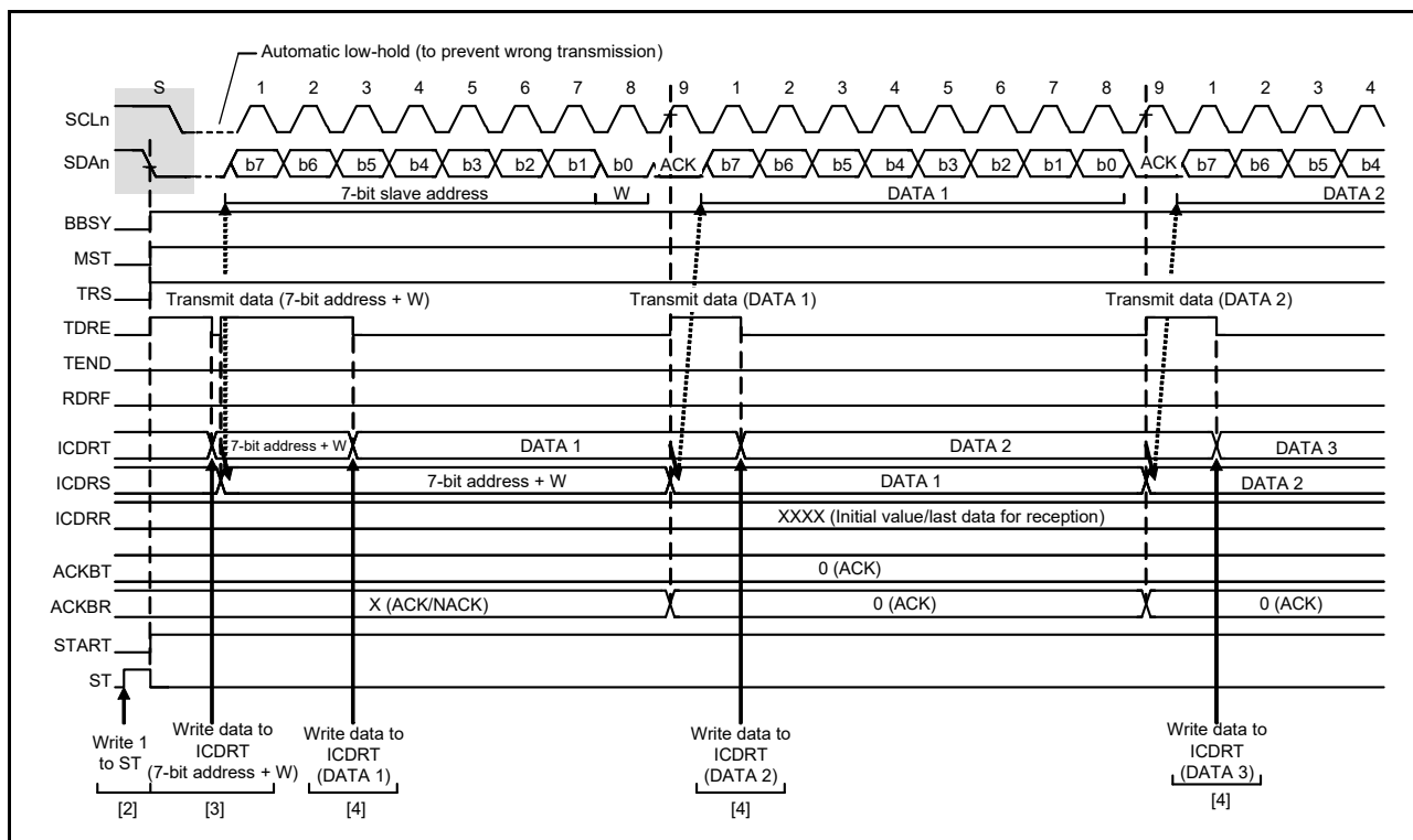
Figure 29.7 Master transmit operation timing (1) (7-bit address format)
