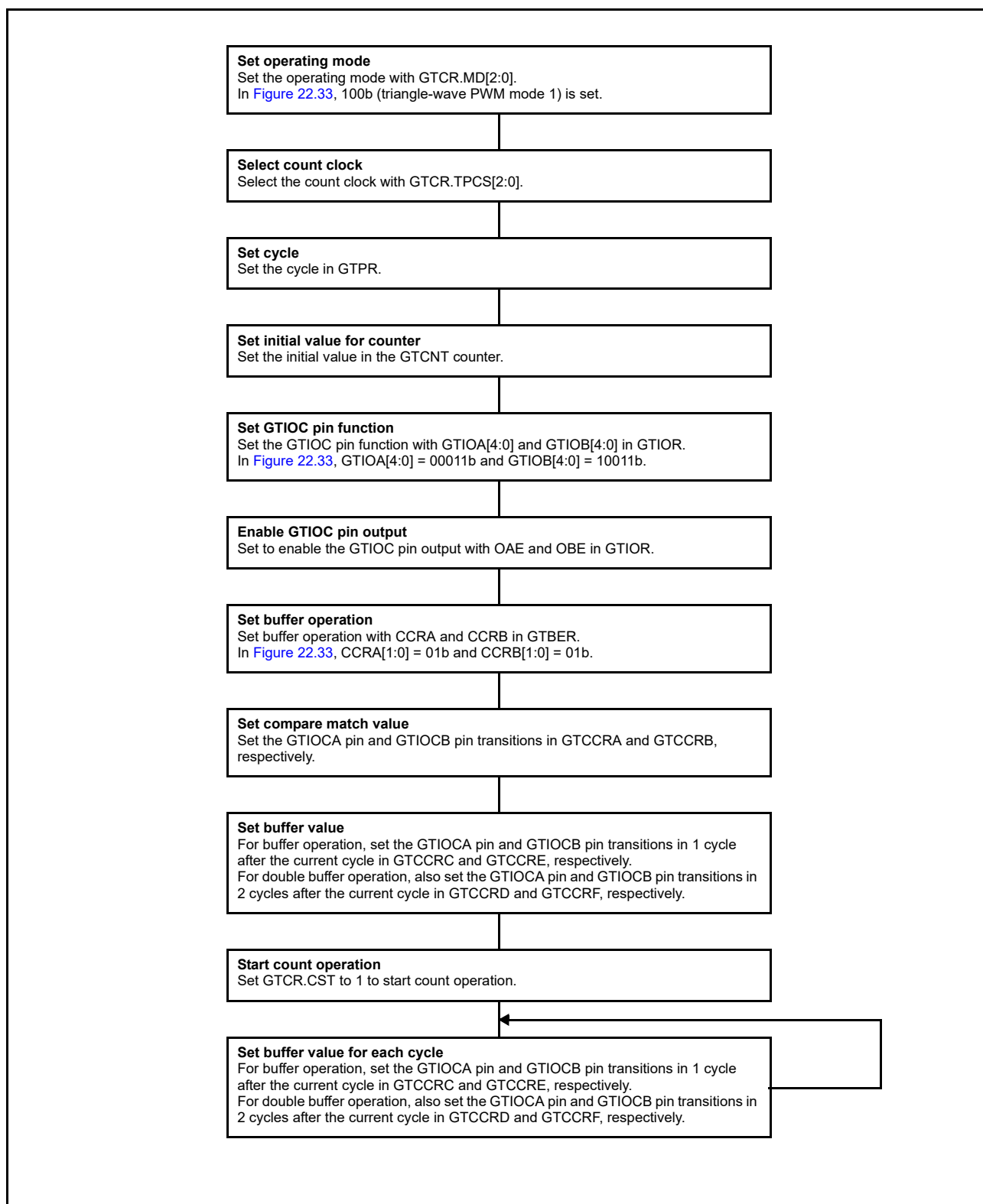
Figure 22.34 Example setting for triangle-wave PWM mode 1
