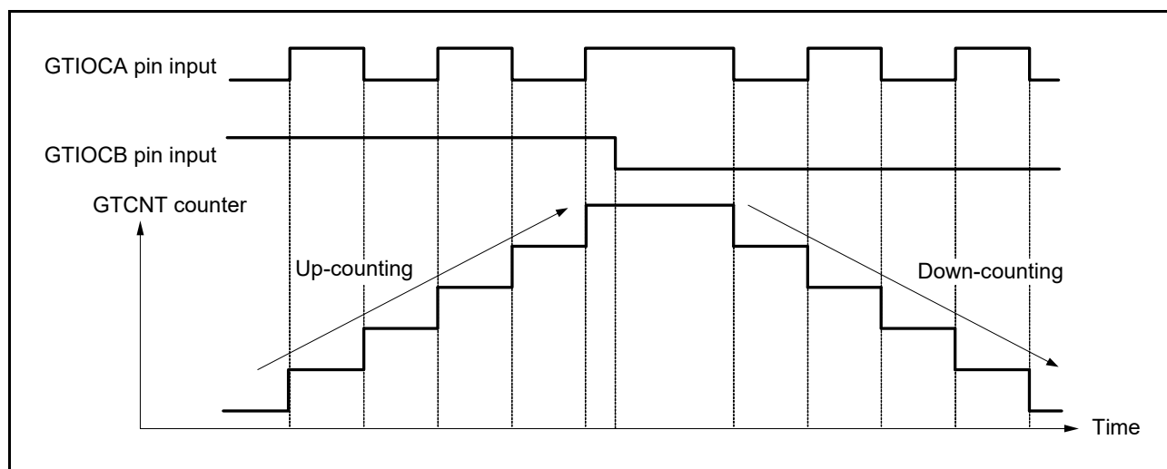
Figure 22.70 Example of phase counting mode 2 (C)
