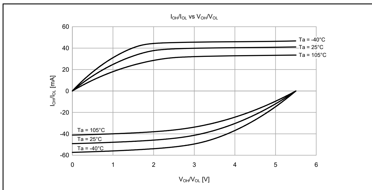
Figure 48.6 V_{OH}/V_{OL} and I_{OH}/I_{OL} temperature characteristics at V_{CC} = 5.5 V when low drive output is selected (reference data)
