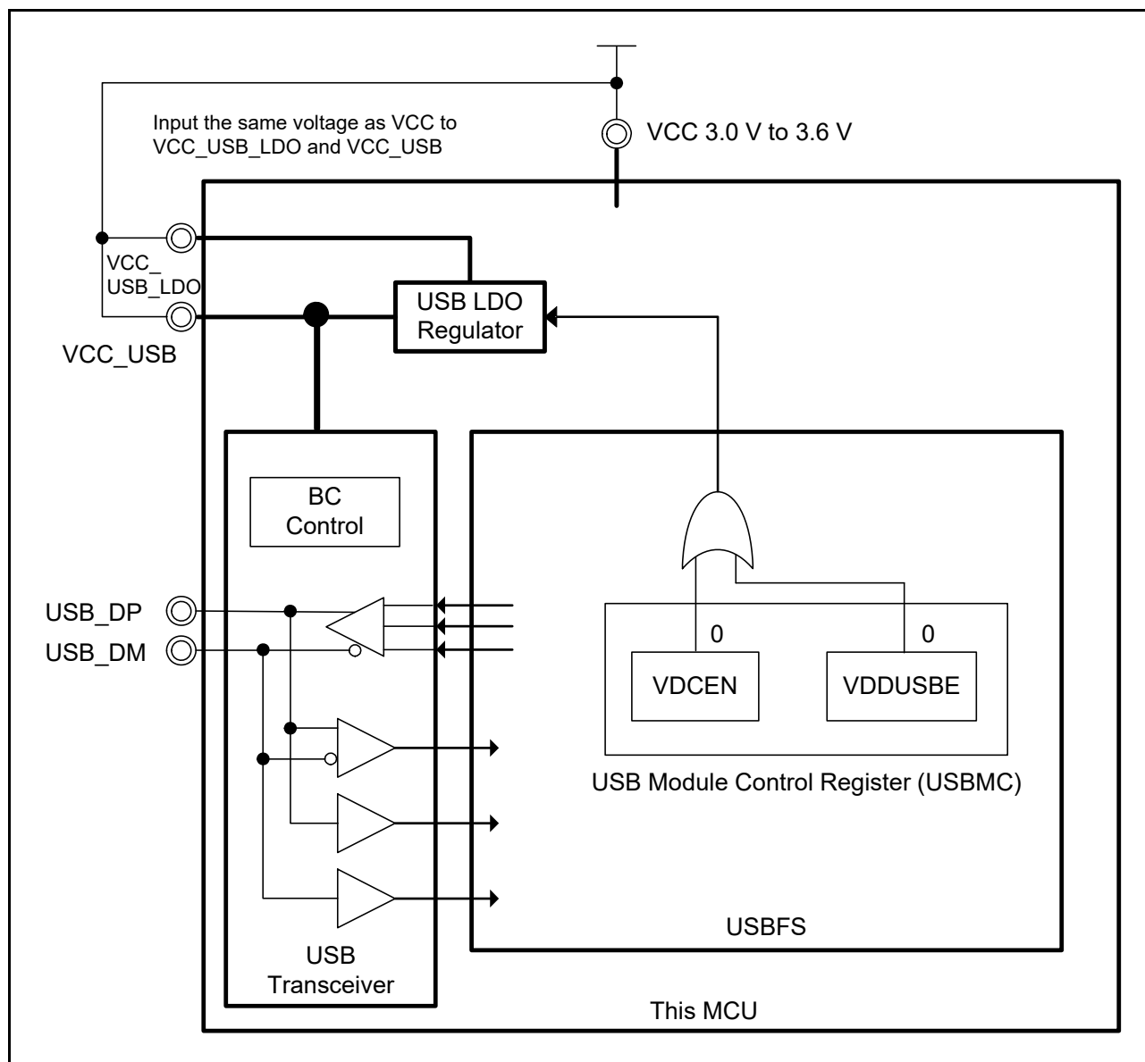
Figure 27.2 Example of power supply connection when the USB LDO regulator is not used
