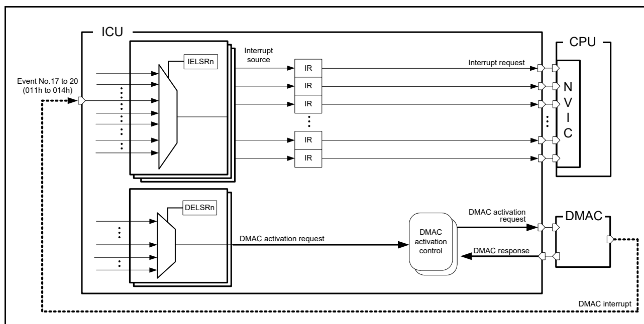
Figure 13.3 DMAC request trigger and interrupt path
