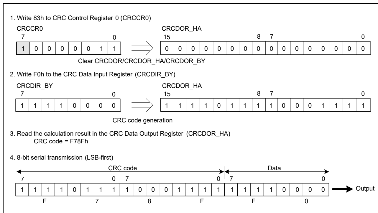
Figure 32.2 LSB-first data transmission
