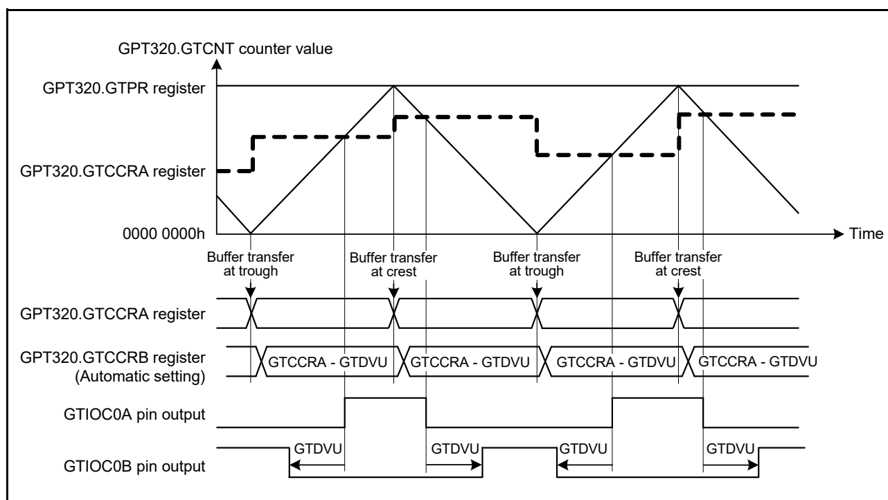
Figure 22.42 Example of automatic compare-match value setting function with dead time with triangle-wave PWM mode 2 or 3, and active-high
