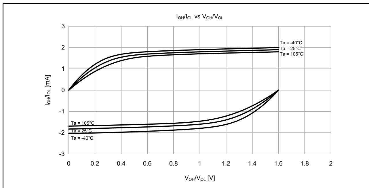
Figure 48.3 V_{OH}/V_{OL} and I_{OH}/I_{OL} temperature characteristics at V_{CC} = 1.6 V when low drive output is selected (reference data)
