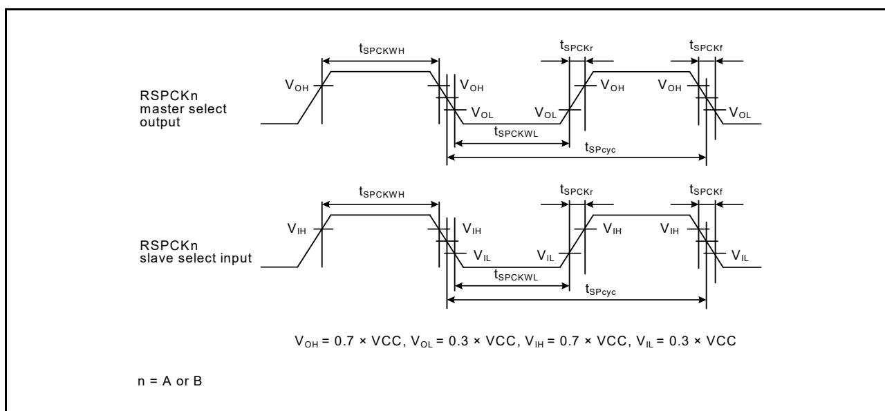
Figure 48.52 SPI clock timing
