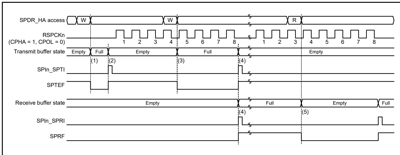
Figure 31.27 Operation example of SPIn_SPTI and SPIn_SPRI interrupts when CPHA = 1, CPOL = 0
