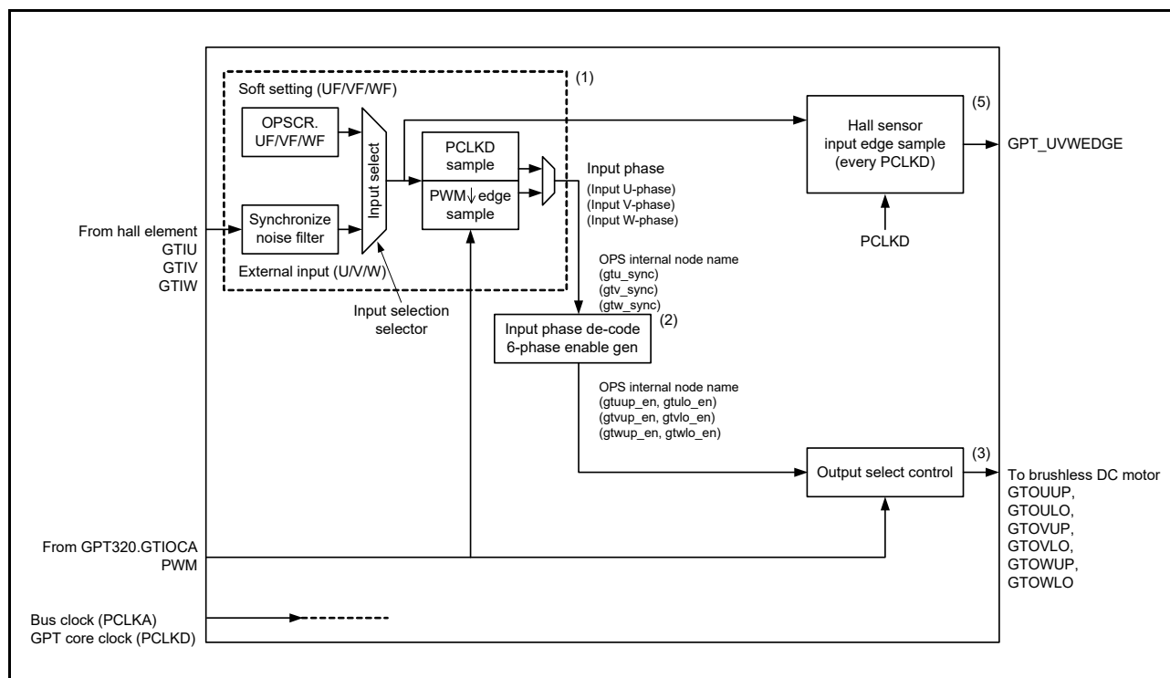
Figure 22.77 Conceptual diagram of GPT_OPS control flow
