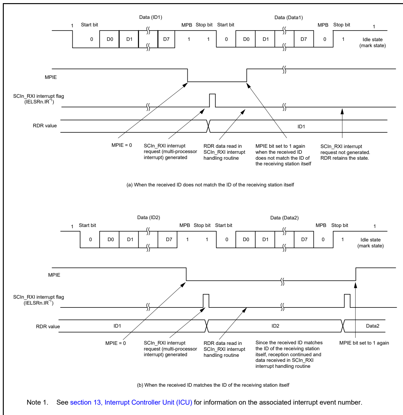
Figure 28.26 Example of SCI reception with 8-bit data, multi-processor bit, and 1 stop bit
