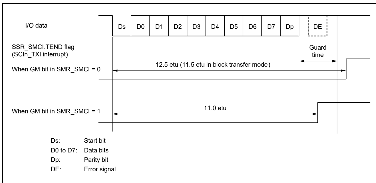
Figure 28.53 SSR.TEND flag generation timing during transmission
