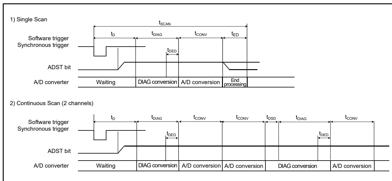
Figure 35.24 Scan conversion timing activated by software or synchronous trigger ELC input
