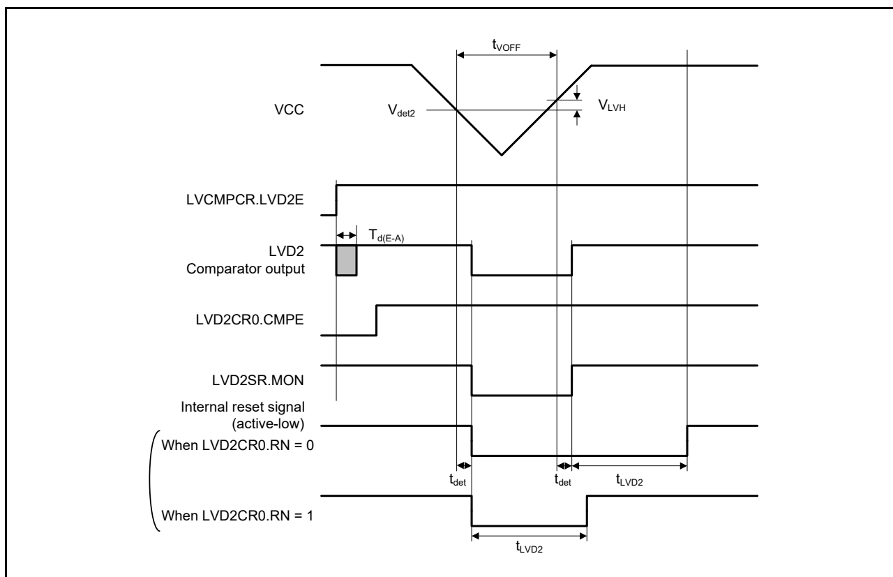
Figure 48.77 Voltage detection circuit timing ( V_{det2} )
