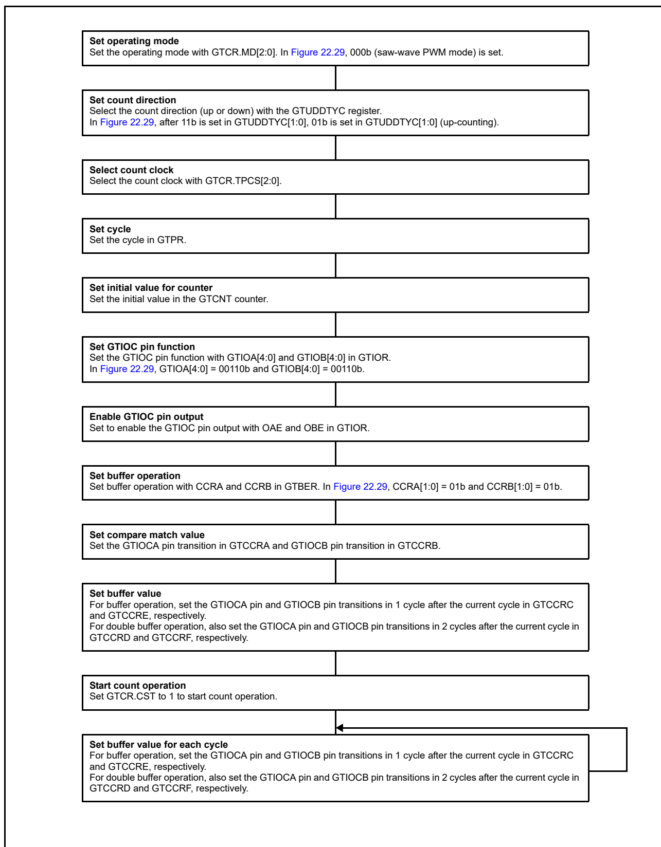
Figure 22.30 Example setting for saw-wave PWM mode
