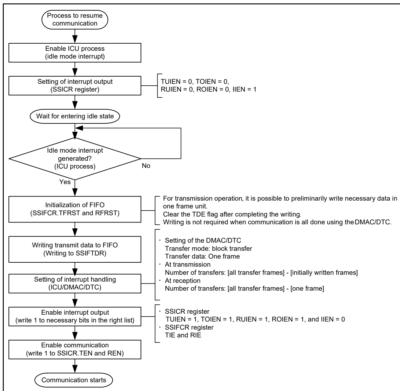
Figure 33.54 Procedure to resume communication (CPU operation)
