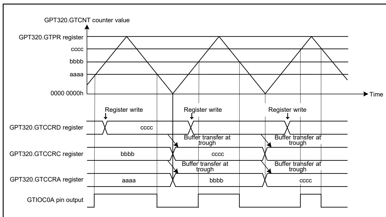
Figure 22.23 Example of GTCCRA and GTCCRB double buffer operation with output compare, triangle waves, buffer operation at trough, output toggled at GTCCRA compare match, and output retained at cycle end
