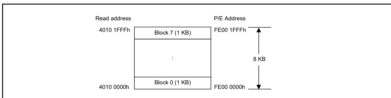
Figure 44.3 Mapping of the data flash memory
