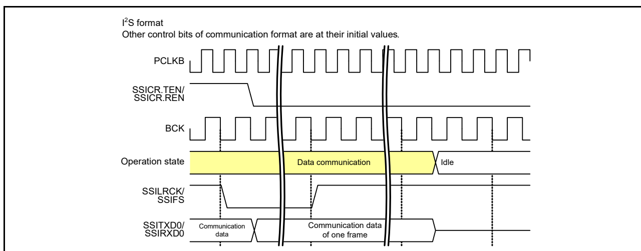
Figure 33.44 Halt from data communication without padding bits
