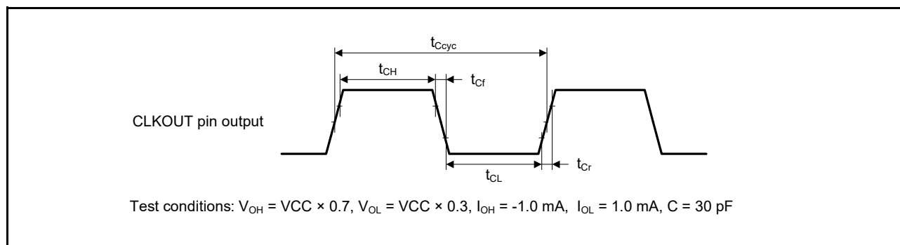
Figure 48.64 CLKOUT output timing
