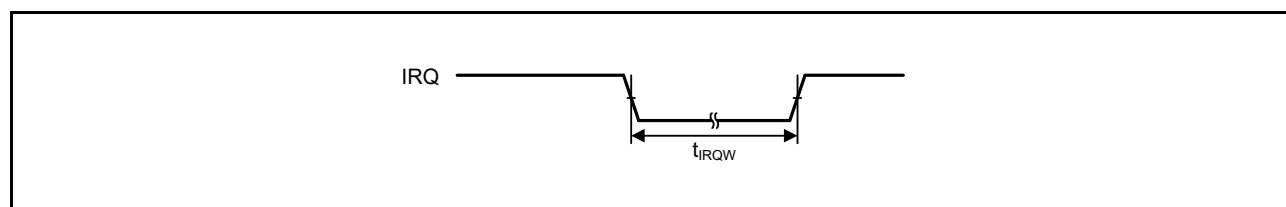
Figure 48.37 IRQ interrupt input timing
