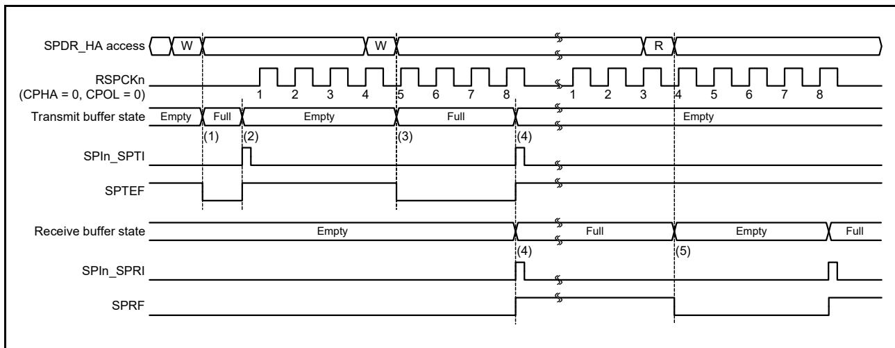
Figure 31.26 Operation example of SPIn_SPTI and SPIn_SPRI interrupts when CPHA = 0, CPOL = 0
