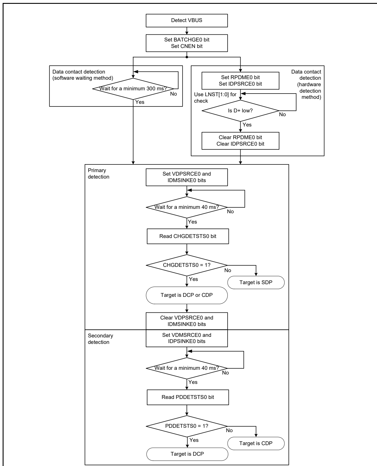
Figure 27.24 Process flow for operating as portable device
