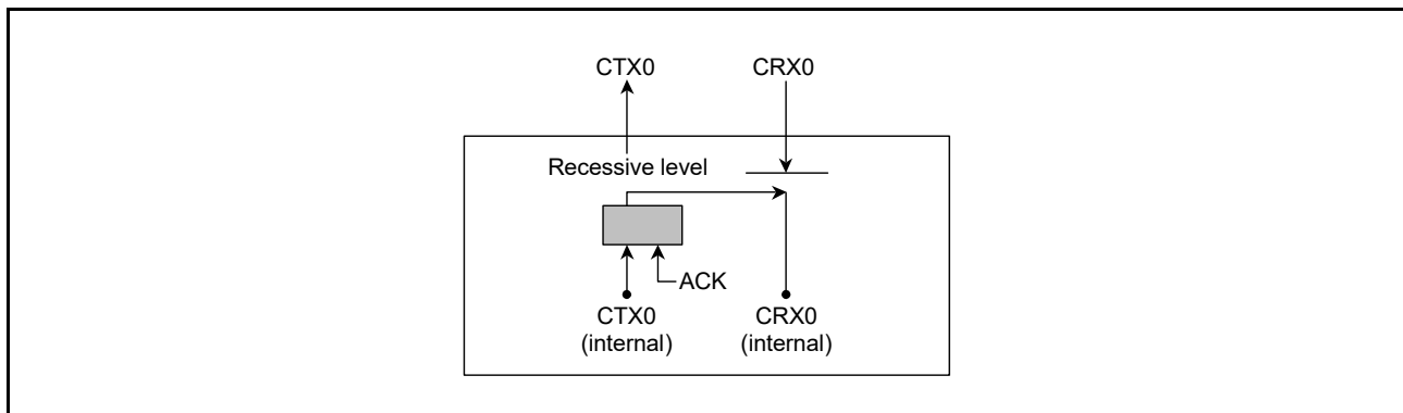
Figure 30.8 Connection when self-test mode 1 is selected
