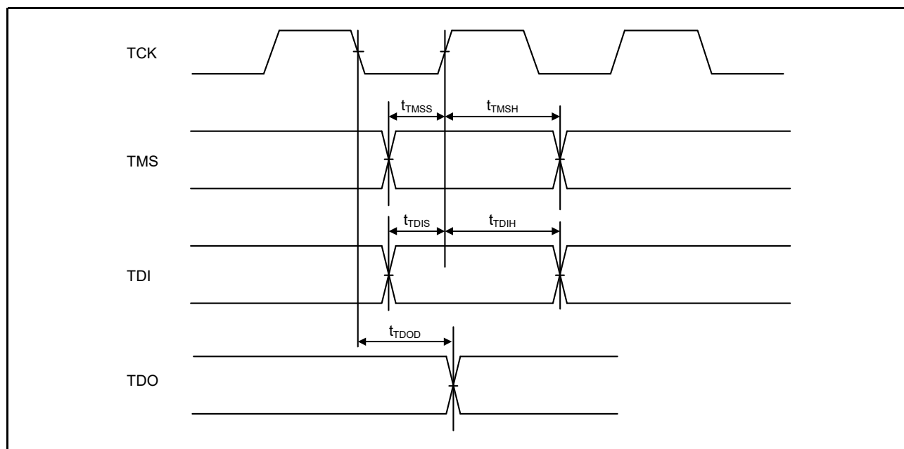
Figure 48.86 JTAG input/output timing
