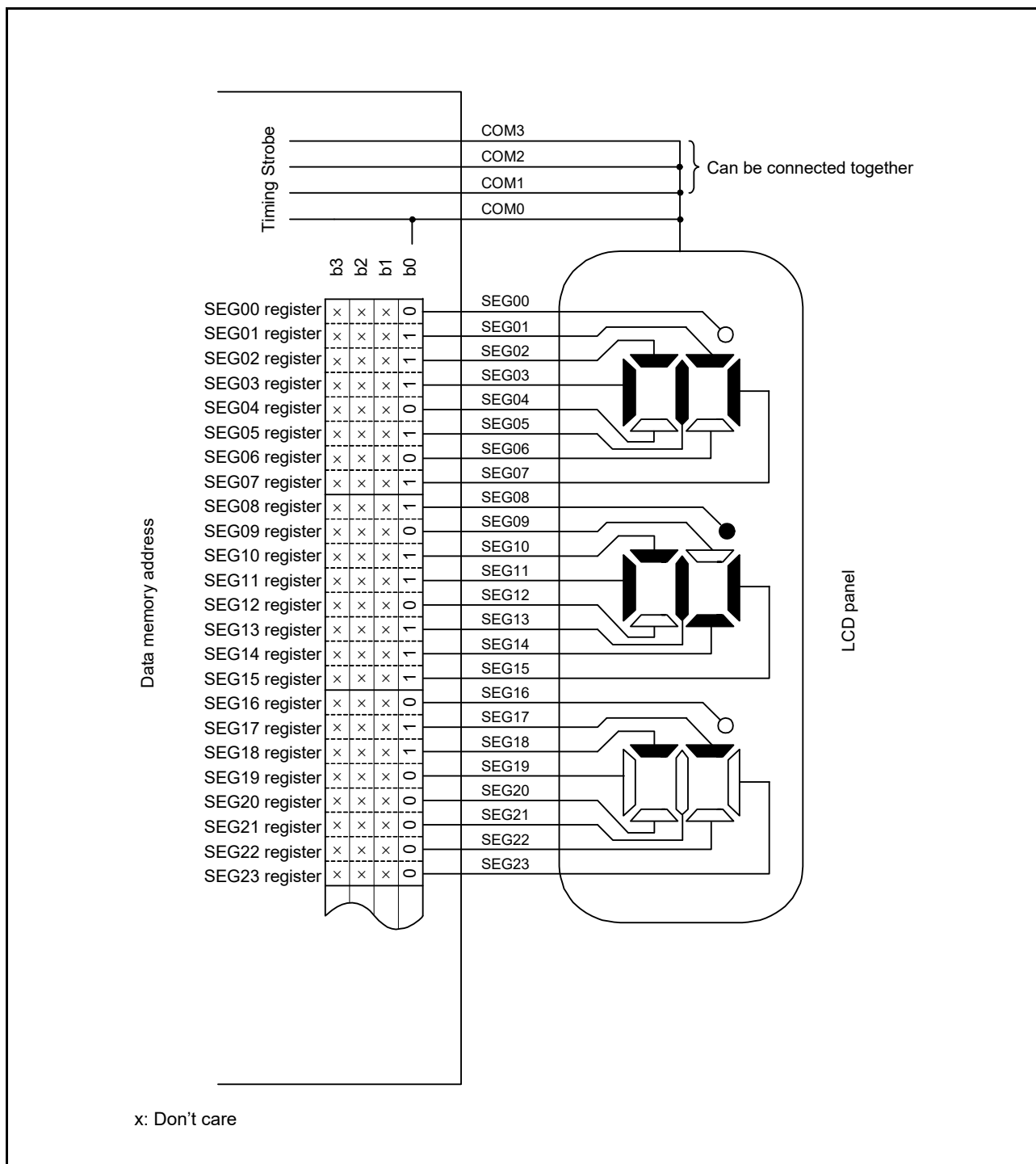
Figure 45.19 Example of connecting static LCD panel
