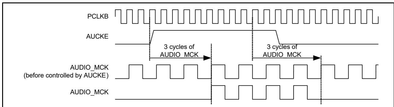
Figure 33.23 Stop/resume of AUDIO_MCK
