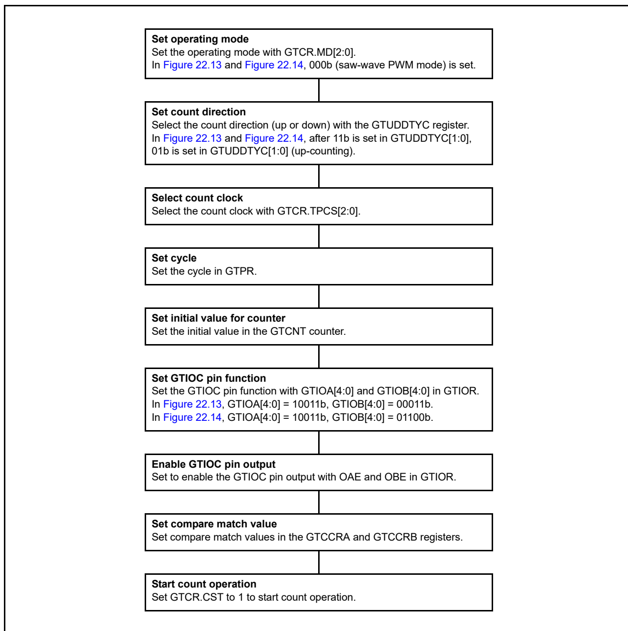
Figure 22.15 Example setting for toggled output operation
