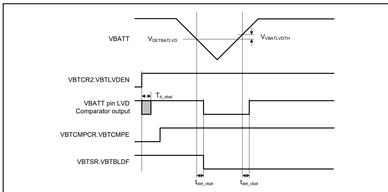
Figure 48.80 VBATT pin voltage detection circuit timing
