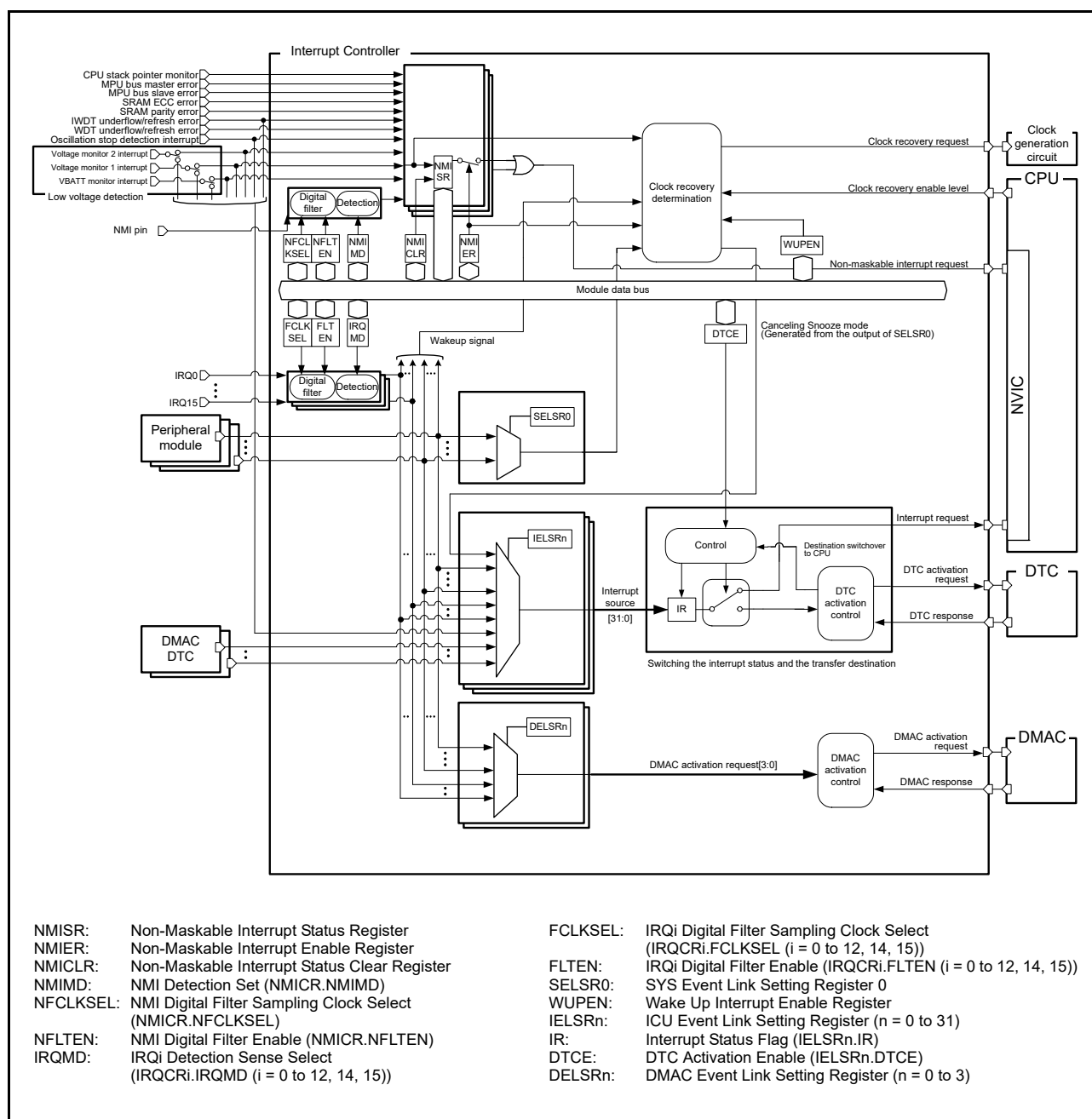
Figure 13.1 ICU block diagram
