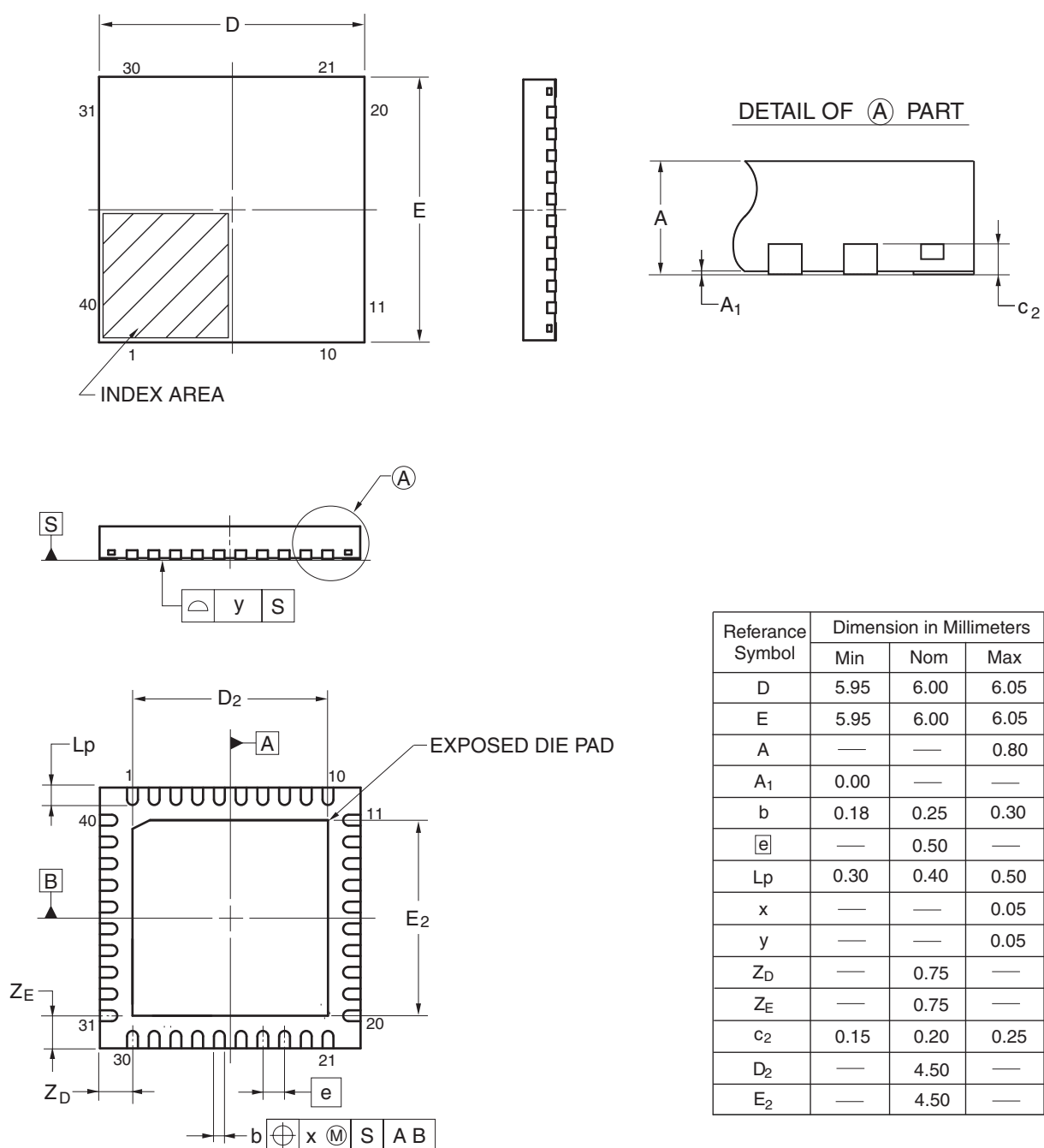
Figure 2.7 40-pin QFN
