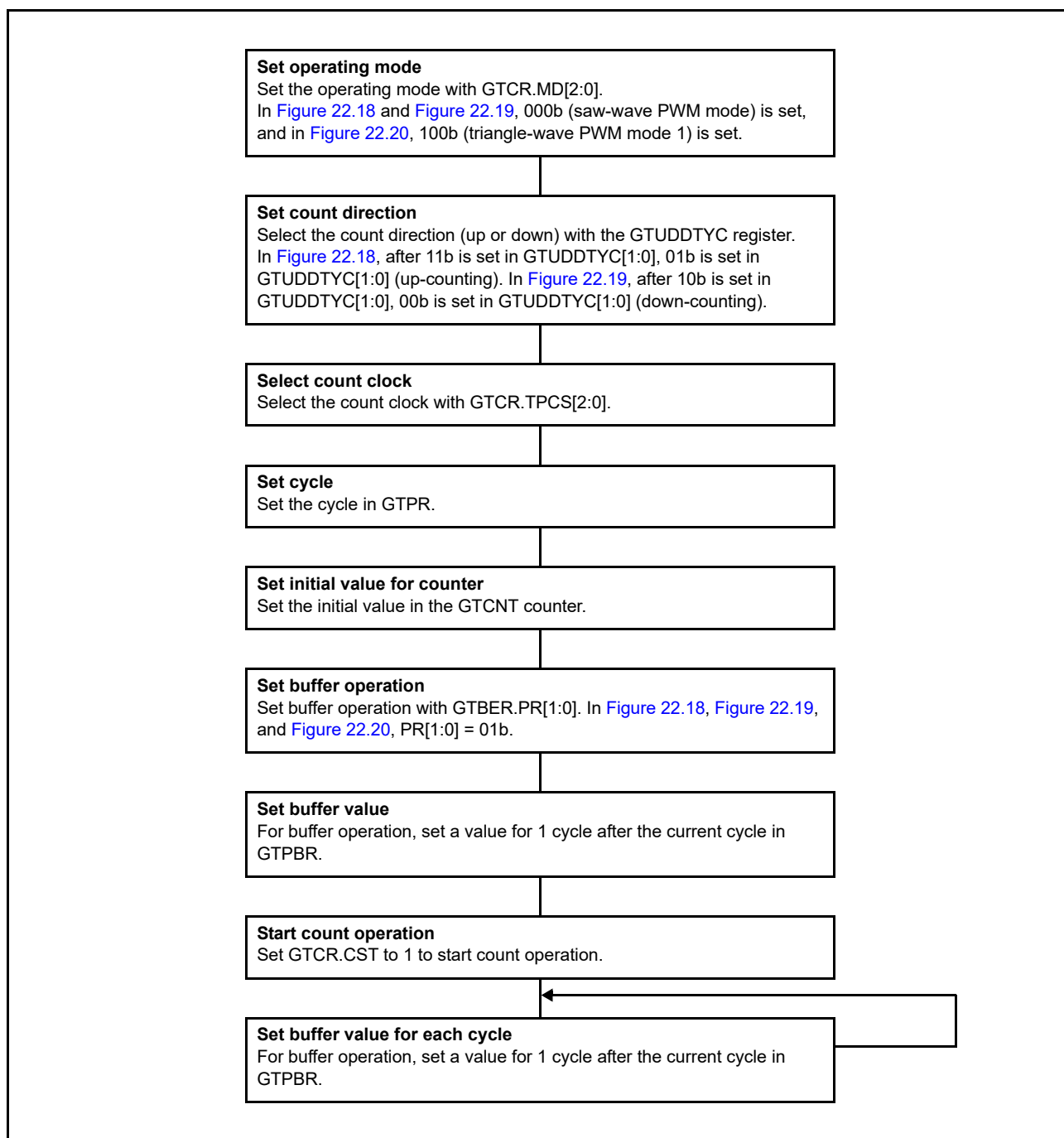
Figure 22.21 Example for setting GTPR buffer operation
