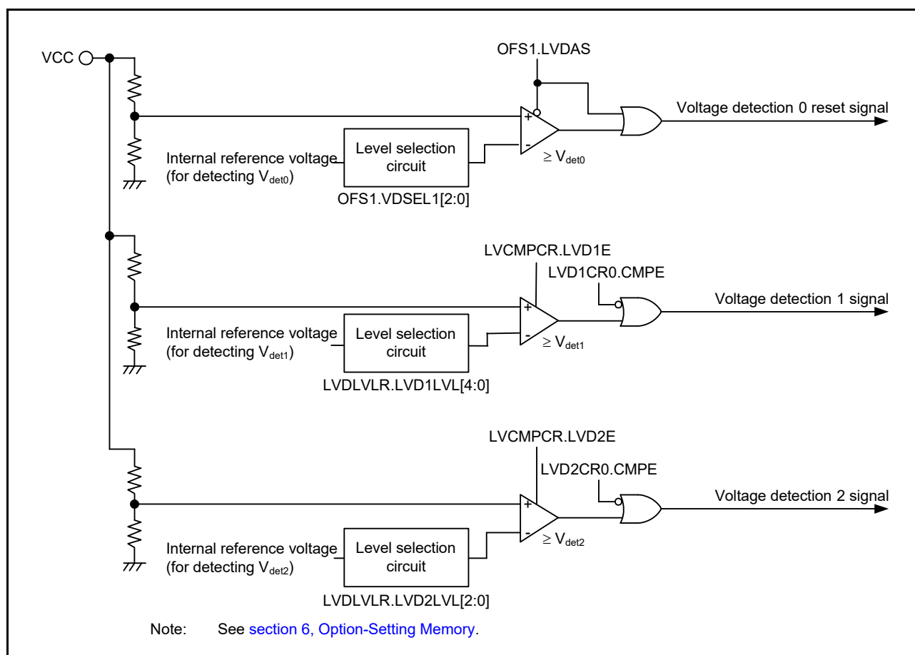
Figure 7.1 Voltage detection 0, 1, and 2 block diagram
