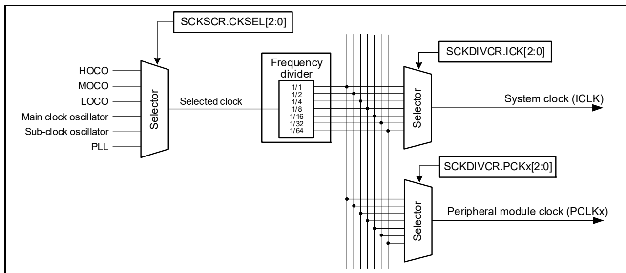
Figure 8.8 Clock source selector block diagram
