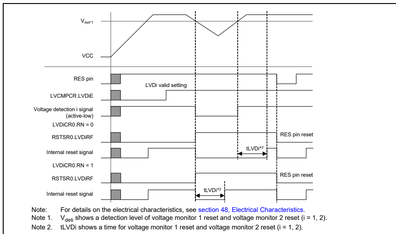
Figure 5.2 Example of operations during voltage monitor 1 and voltage monitor 2 resets
