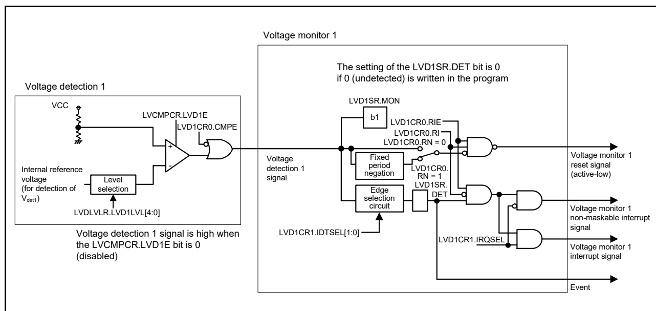
Figure 7.2 Voltage monitor 1 interrupt/reset circuit block diagram
