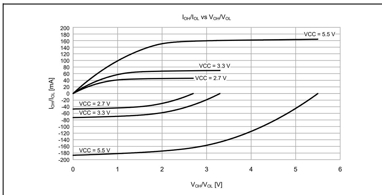
Figure 48.12 V_{OH}/V_{OL} and I_{OH}/I_{OL} voltage characteristics at T_a = 25^\circ\text{C} when middle drive output is selected (reference data)
