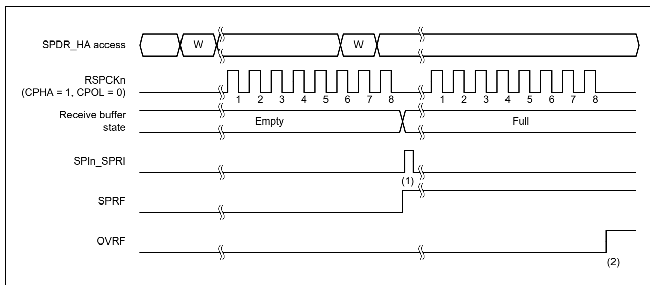
Figure 31.24 Operation example when SPCR.TXMD = 0
