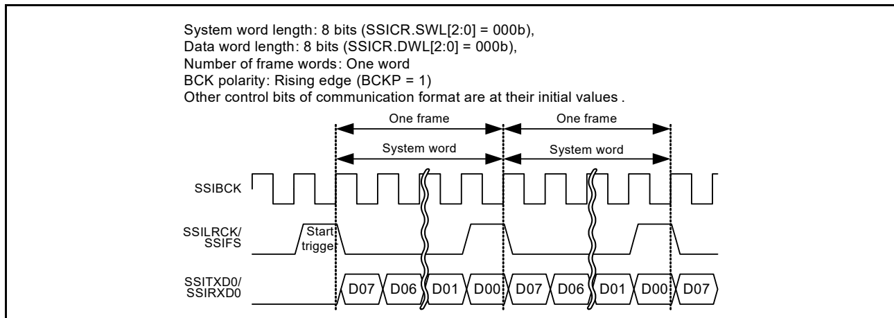
Figure 33.36 Short frame in monaural format without padding, with the system word length = data word length
