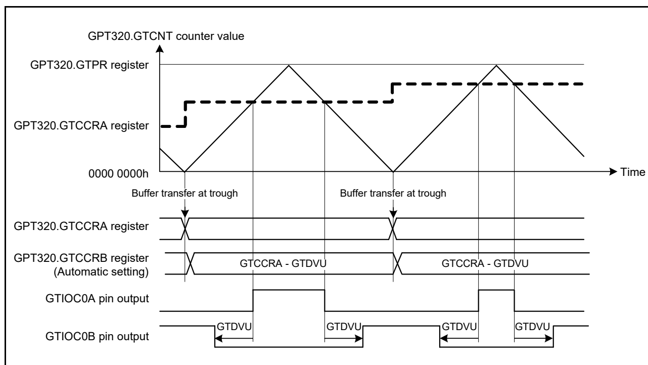
Figure 22.41 Example of automatic compare-match value setting function with dead time with triangle-wave PWM mode 1, and active-high
