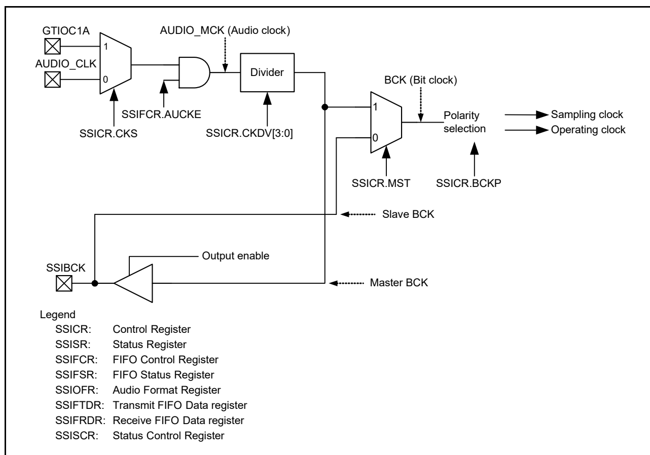
Figure 33.3 SSIE clock configuration
