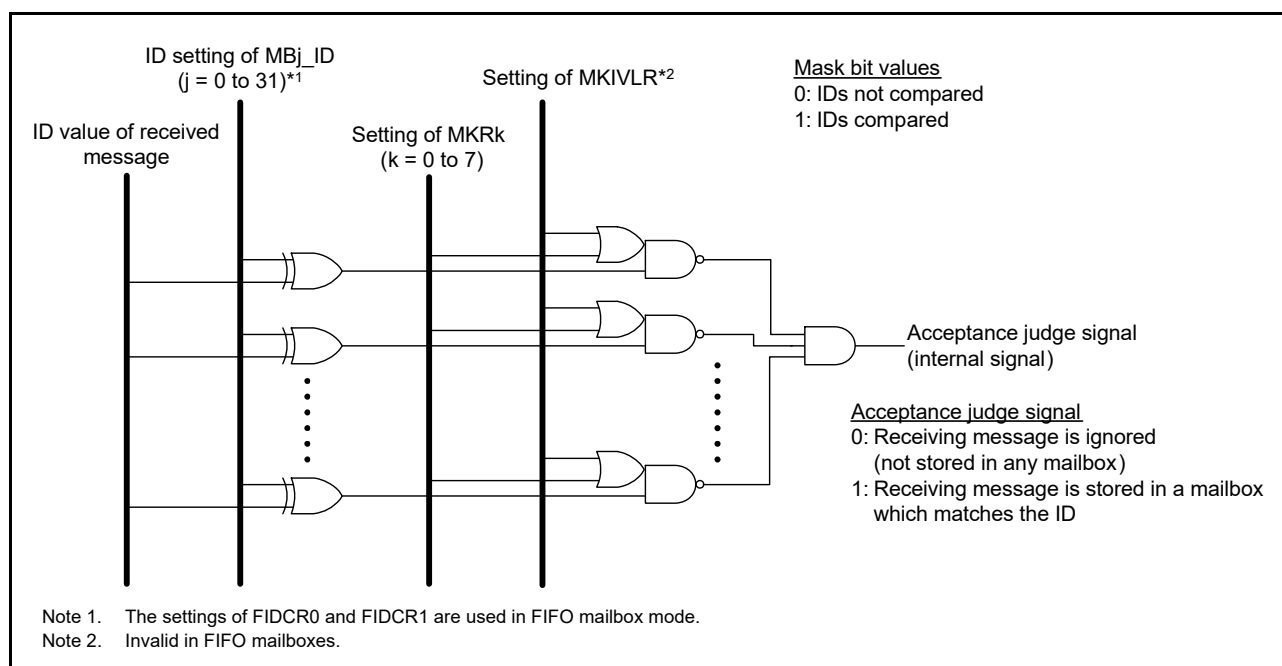
Figure 30.17 Acceptance filtering
