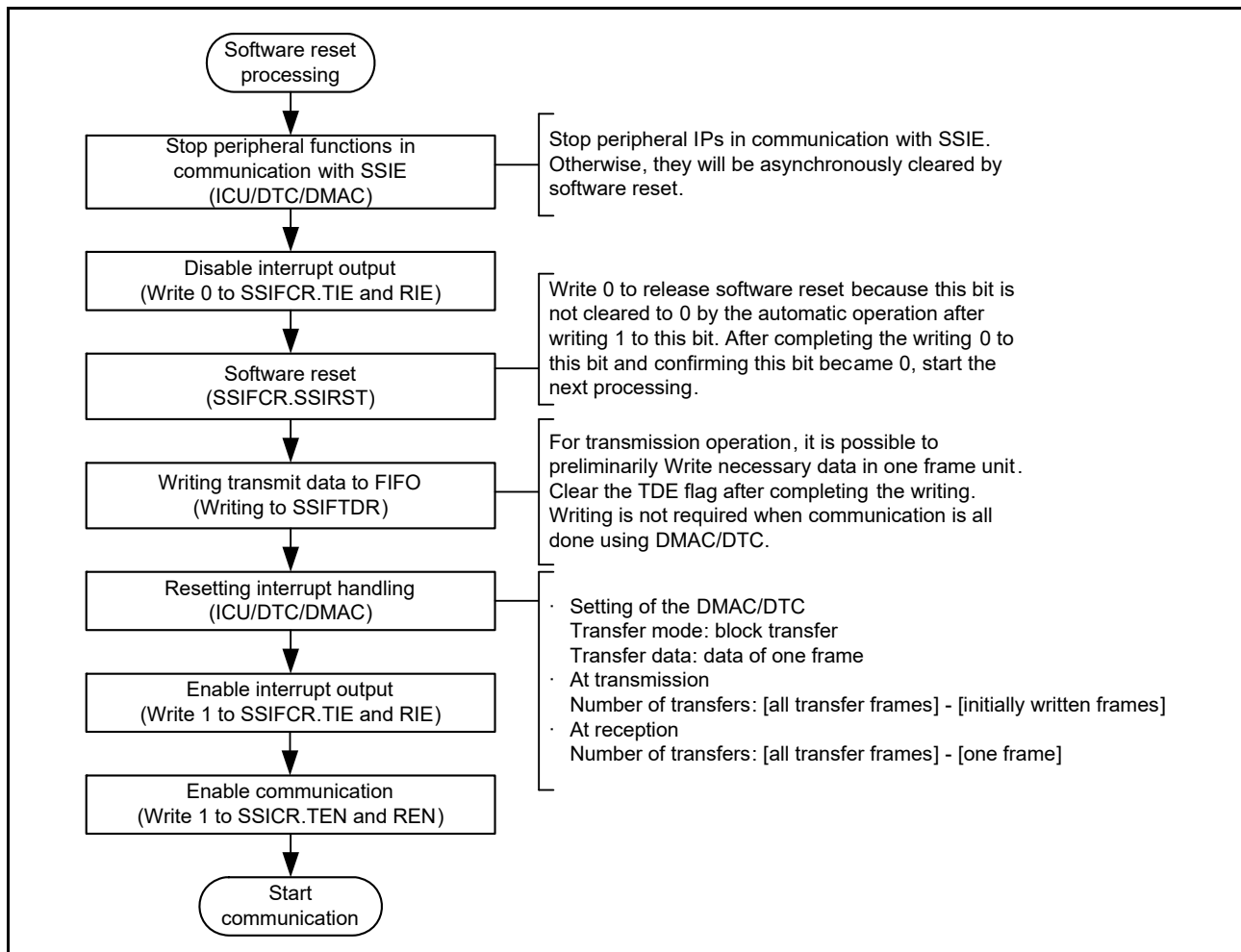
Figure 33.57 Software reset procedure (CPU operation)
