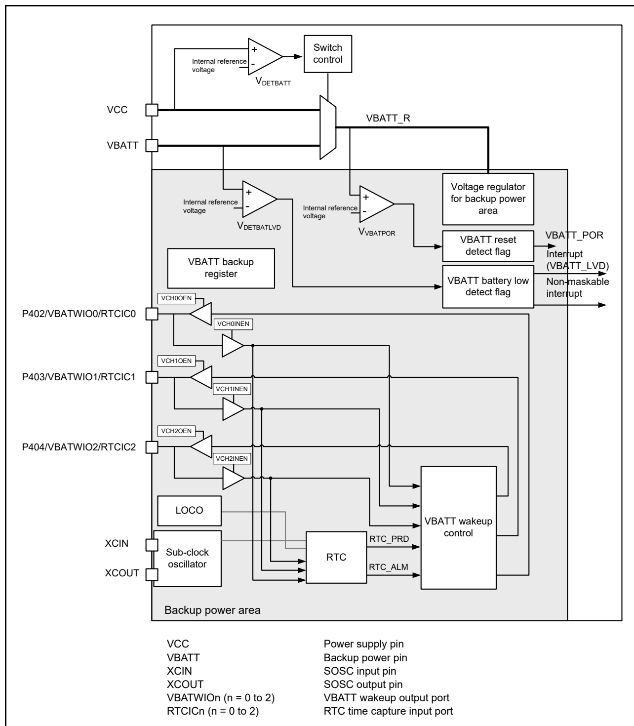
Figure 11.1 Configuration of the battery backup function
