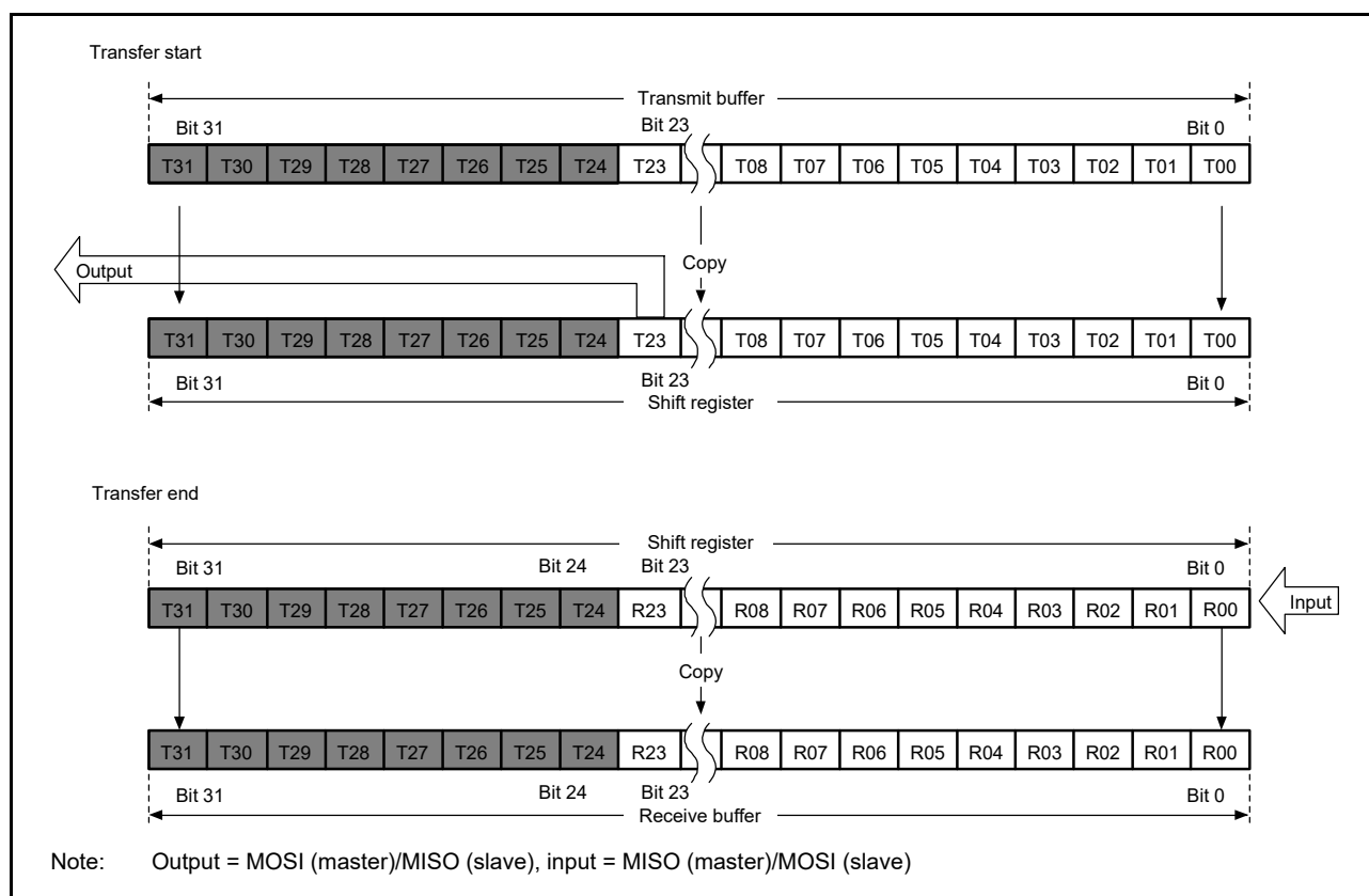
Figure 31.15 MSB-first transfer with 24-bit data and parity disabled
