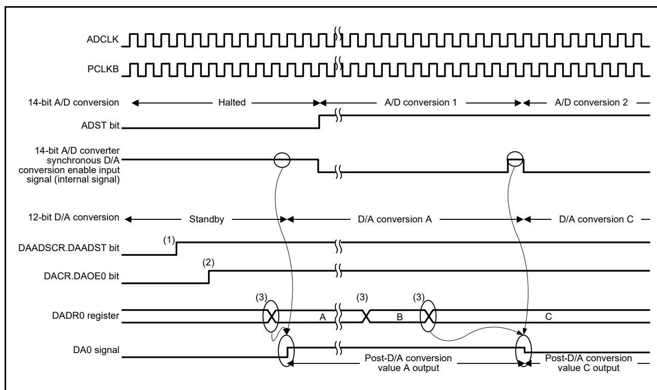
Figure 36.3 Example of conversion when DAC12 is synchronized with ADC14
