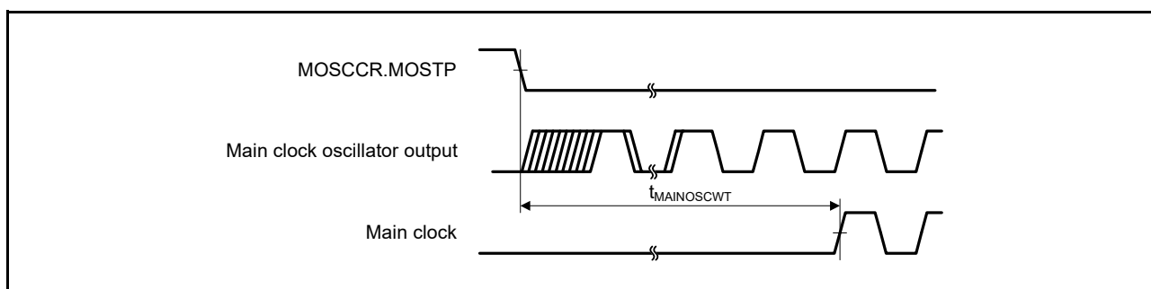
Figure 48.28 Main clock oscillation start timing
