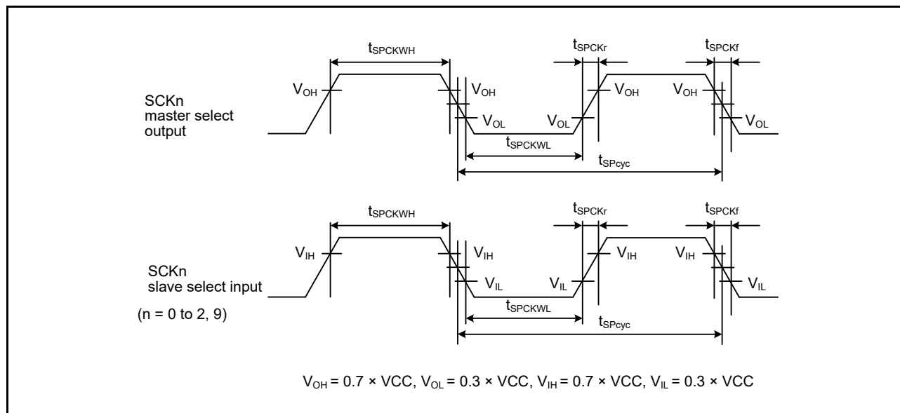
Figure 48.46 SCI simple SPI mode clock timing
