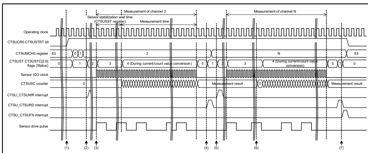
Figure 41.15 Timing of self-capacitance multiscan mode when the measurement start condition is a software trigger
