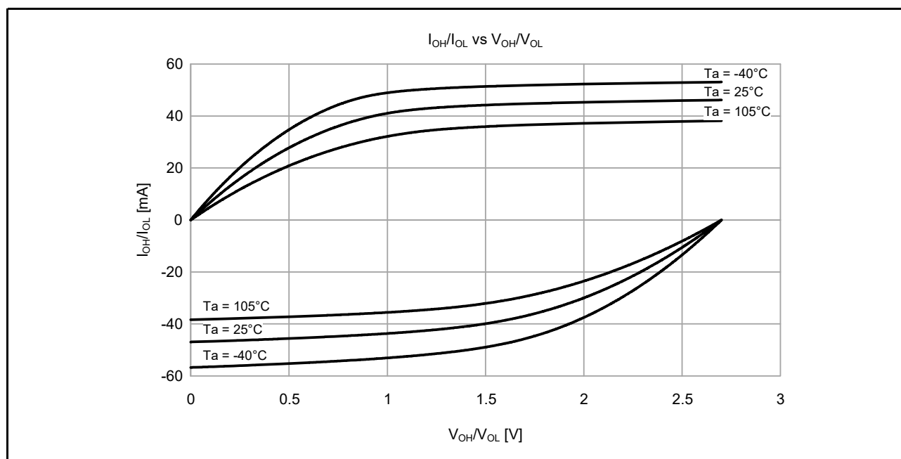
Figure 48.13 V_{OH}/V_{OL} and I_{OH}/I_{OL} temperature characteristics at V_{CC} = 2.7\text{ V} when middle drive output is selected (reference data)
