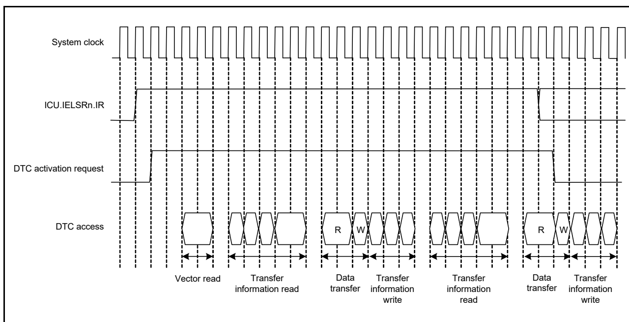
Figure 17.11 Example 3 of DTC operation timing for chain transfer
