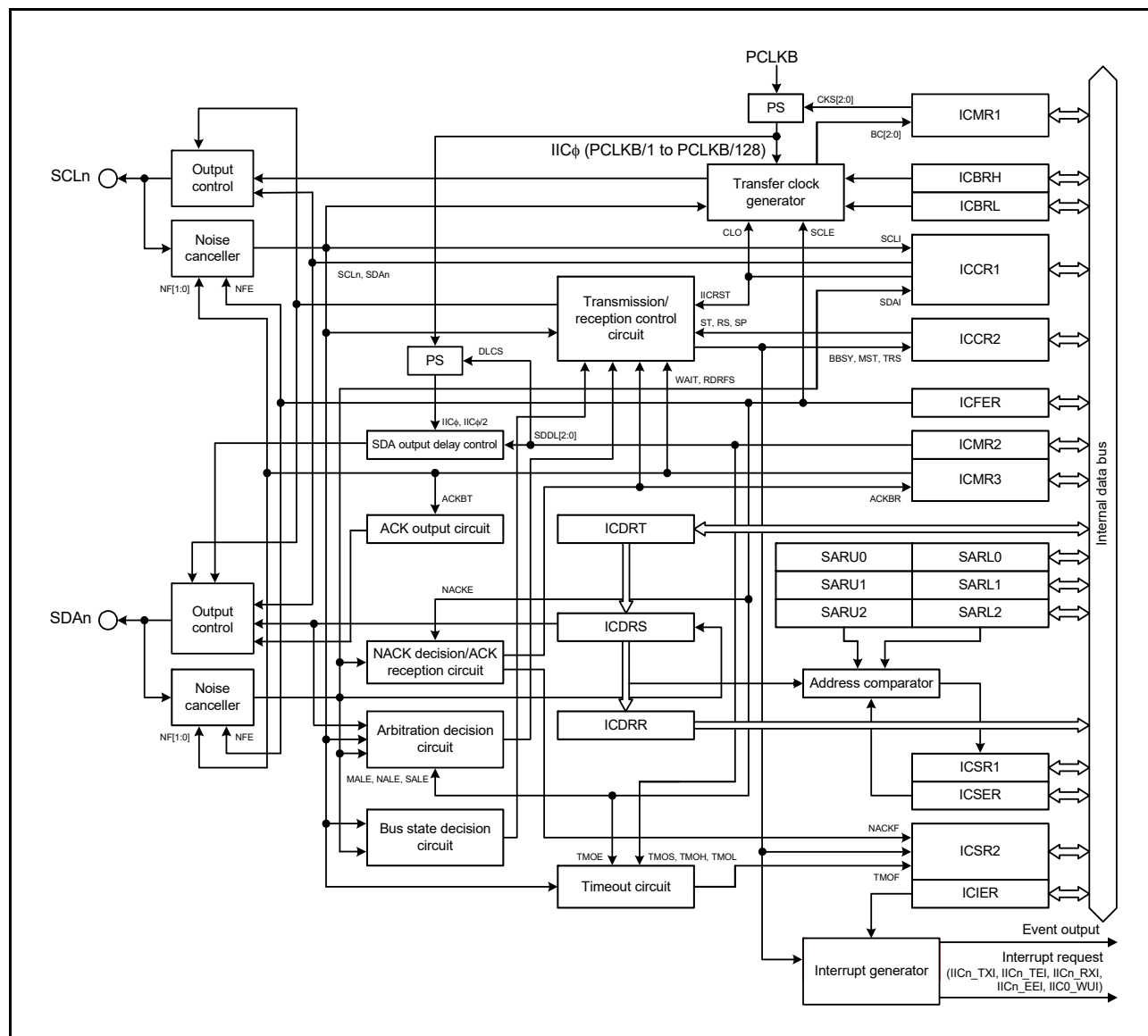
Figure 29.1 IIC block diagram
