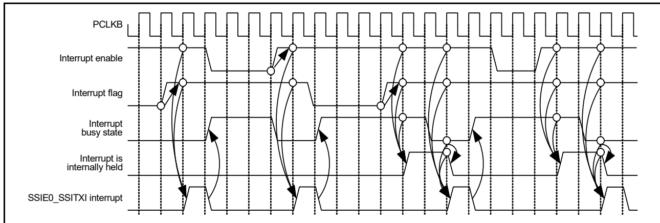
Figure 33.56 SSIE0_SSITXI interrupt timing diagram
