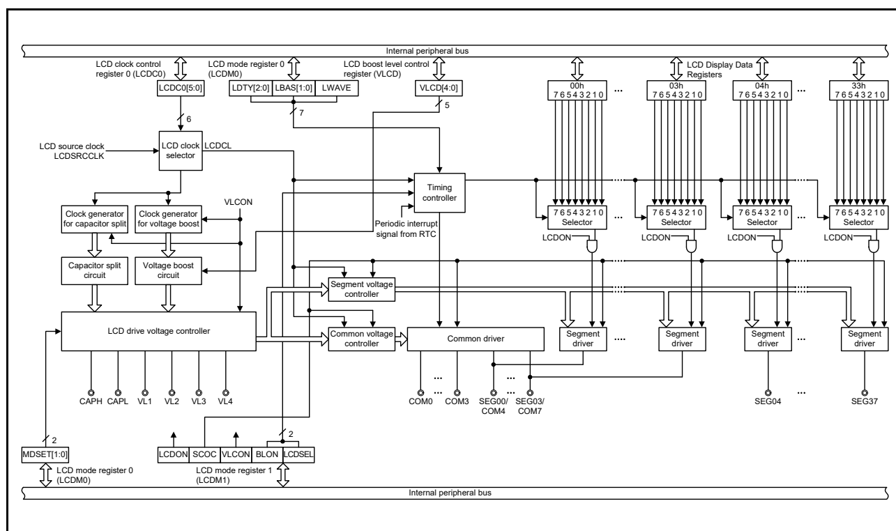
Figure 45.1 SLCDC block diagram
