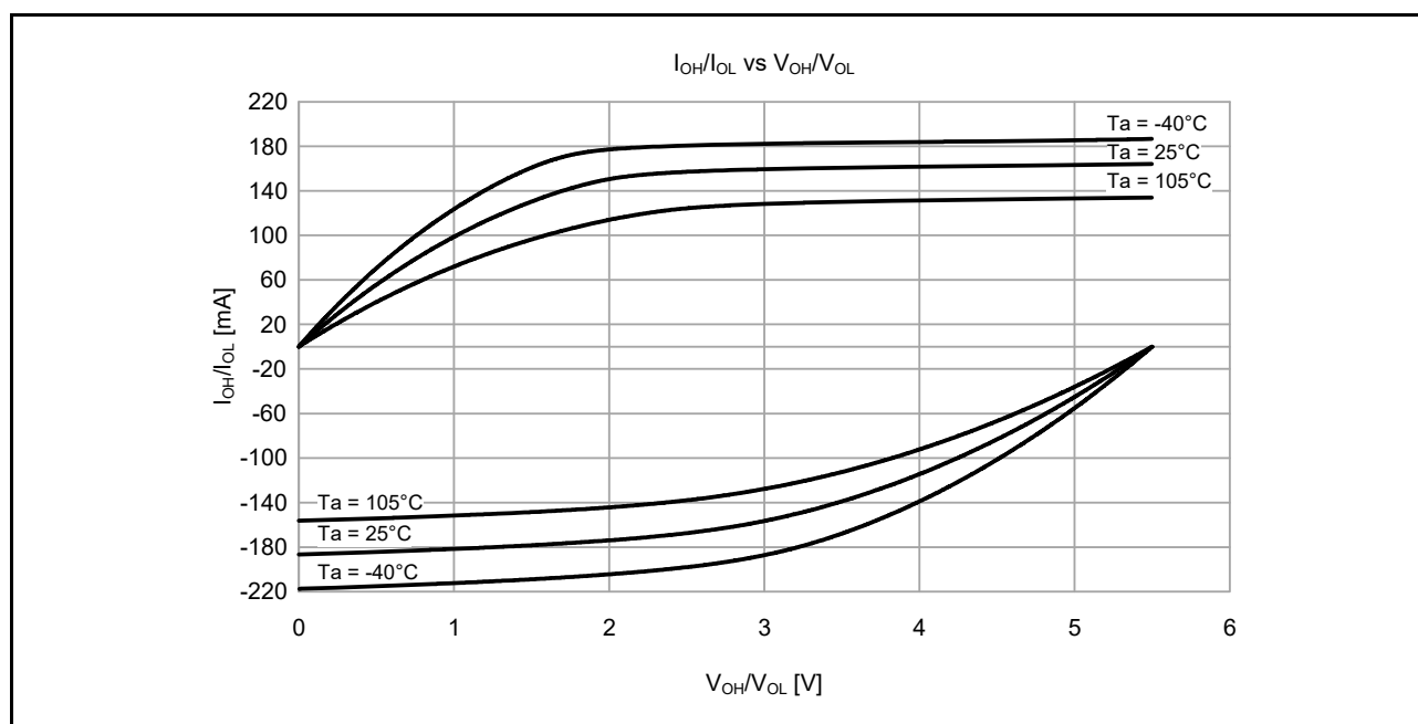
Figure 48.15 V_{OH}/V_{OL} and I_{OH}/I_{OL} temperature characteristics at V_{CC} = 5.5 V when middle drive output is selected (reference data)
