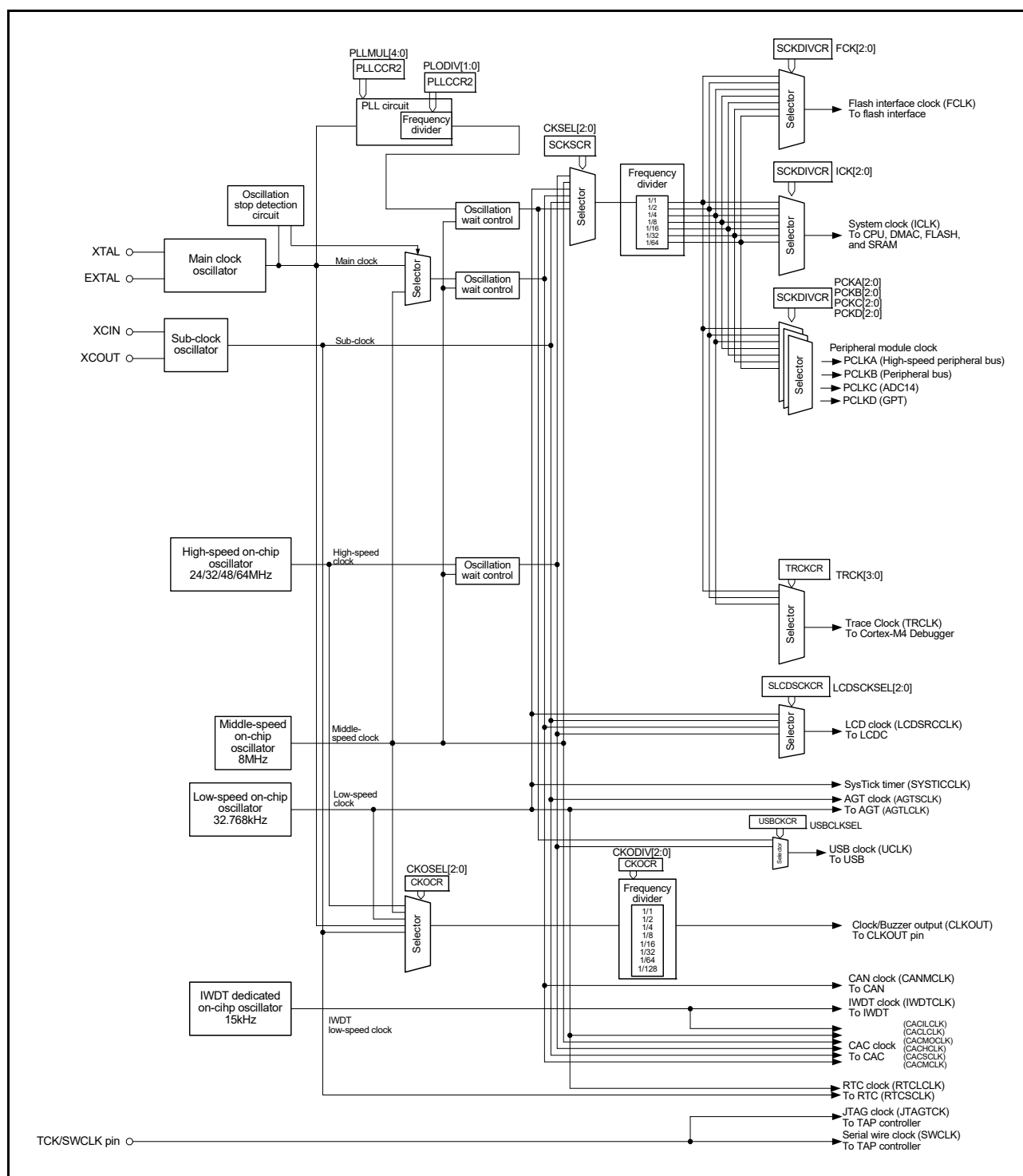
Figure 8.1 Clock generation circuit block diagram
