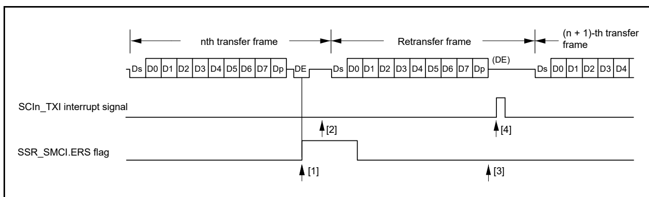
Figure 28.52 Data retransfer operation in SCI transmission mode
