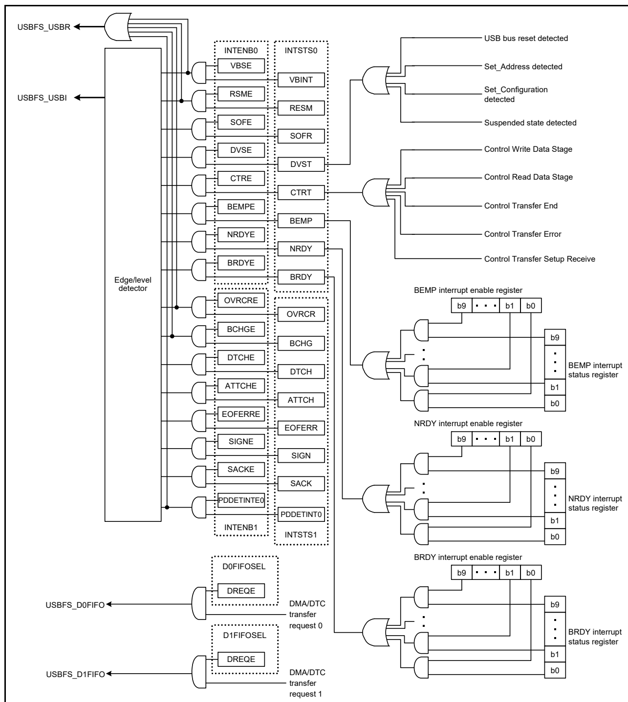
Figure 27.11 USBFS interrupt-related circuits
