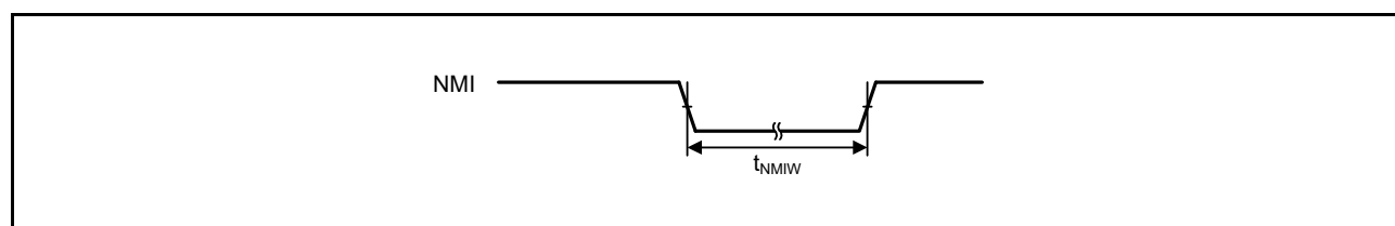
Figure 48.36 NMI interrupt input timing
