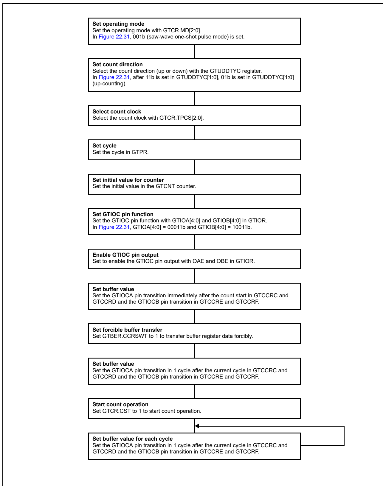
Figure 22.32 Example setting for saw-wave one-shot pulse mode
