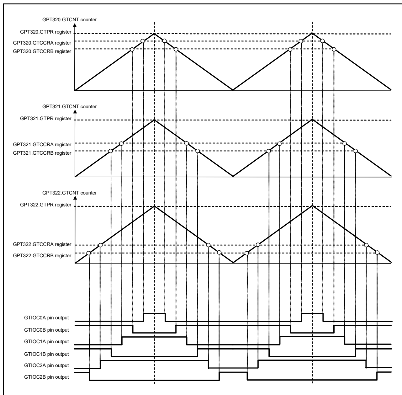
Figure 22.64 Example of 3-phase triangle-wave complementary PWM output
