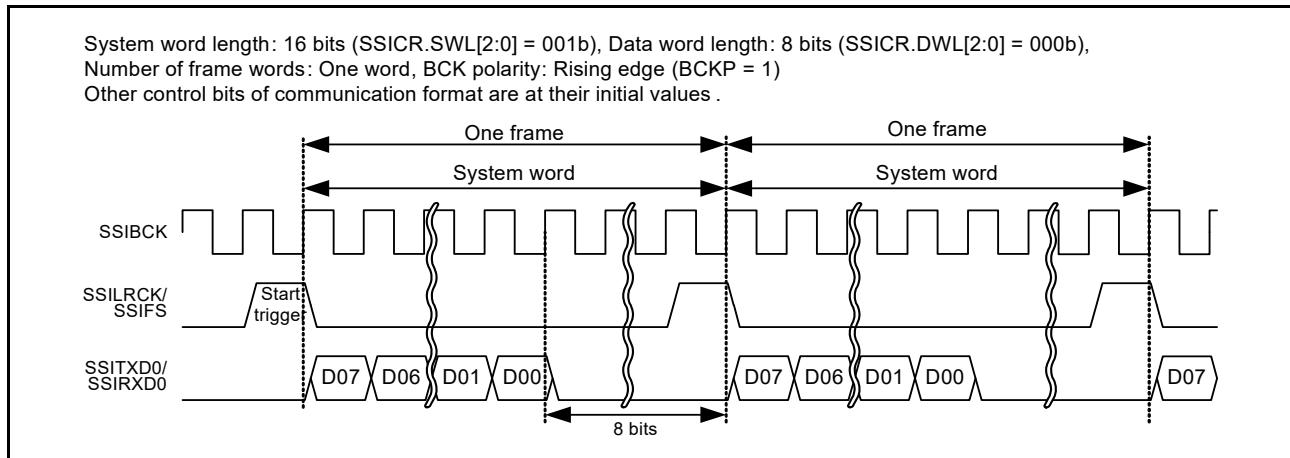
Figure 33.37 Short frame in monaural format with padding, with system word length > data word length
