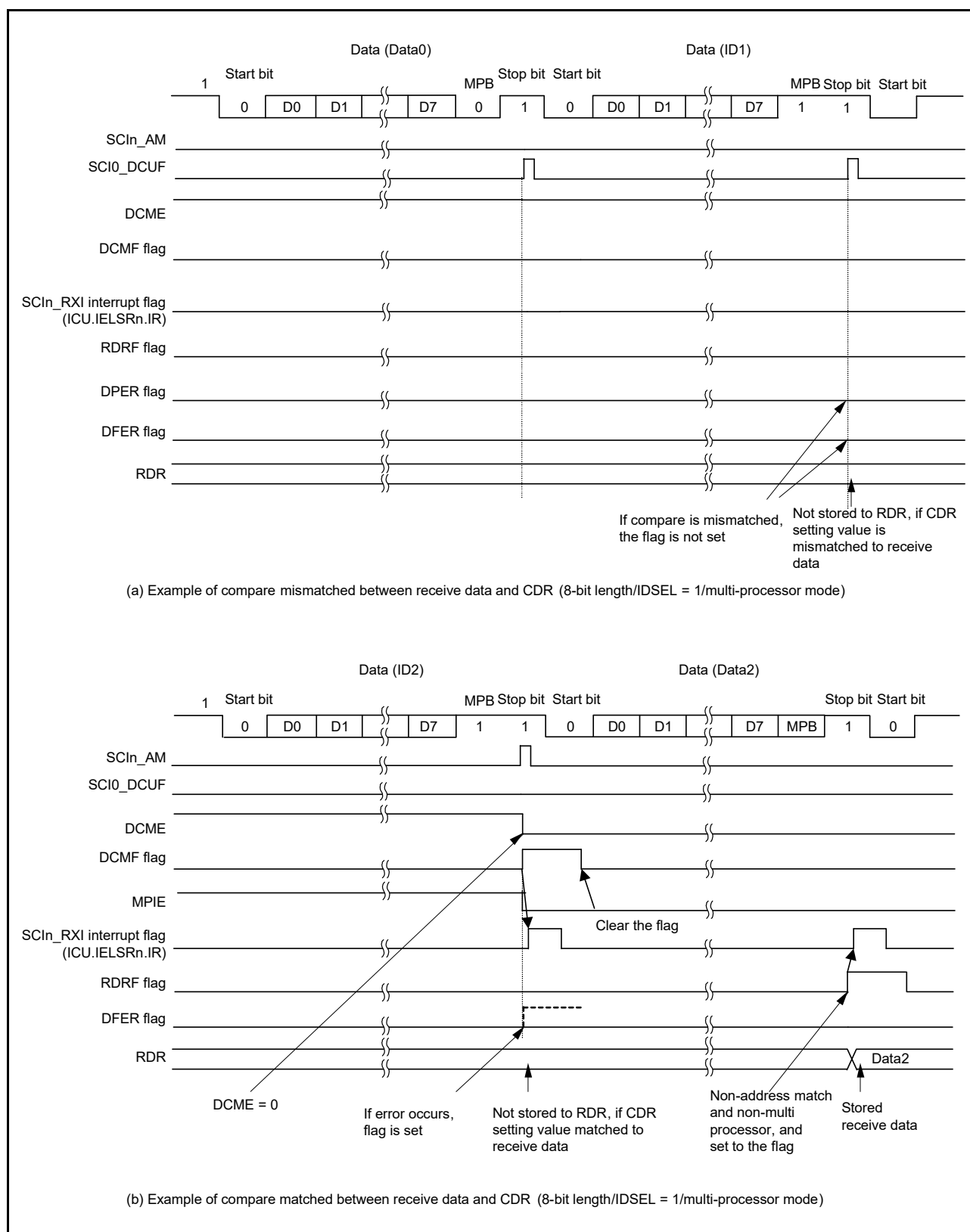
Figure 28.6 Example of address match (2) in multi-processor mode
