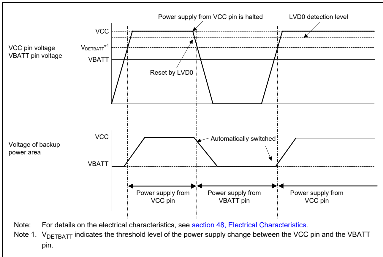
Figure 11.3 Switching sequence for the battery backup function
