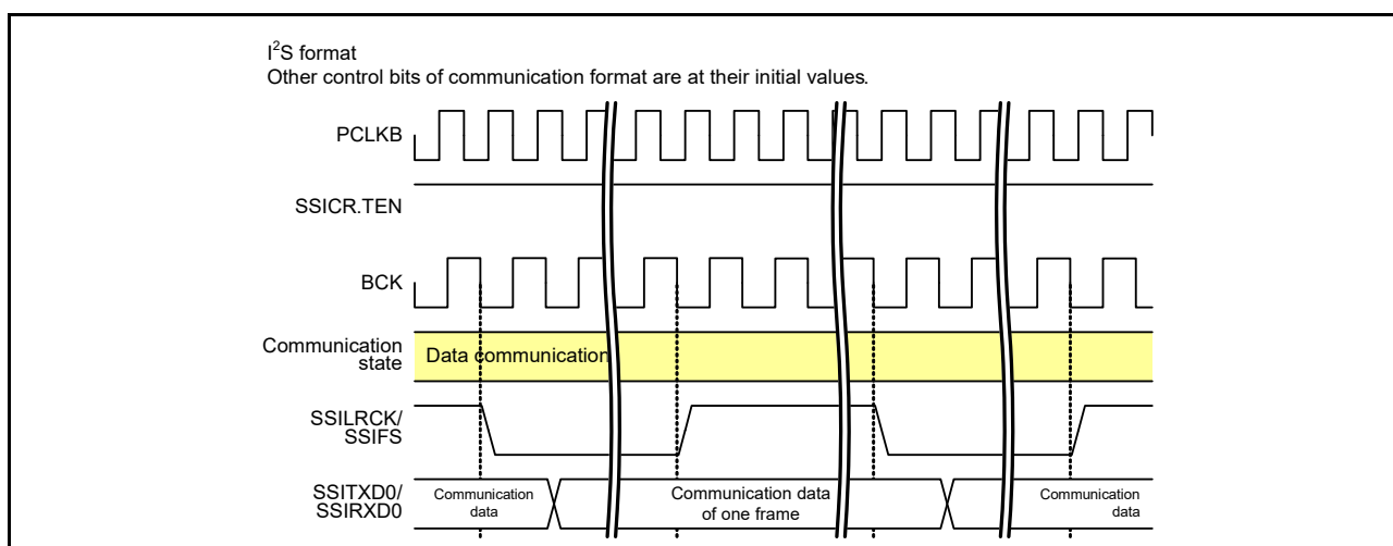
Figure 33.43 Continuation of data communication
