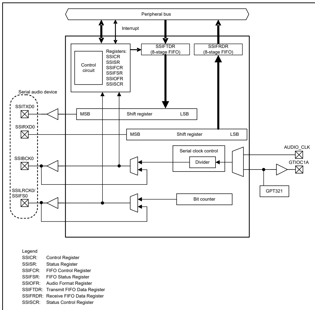
Figure 33.2 SSIE block diagram (SSIE0)
