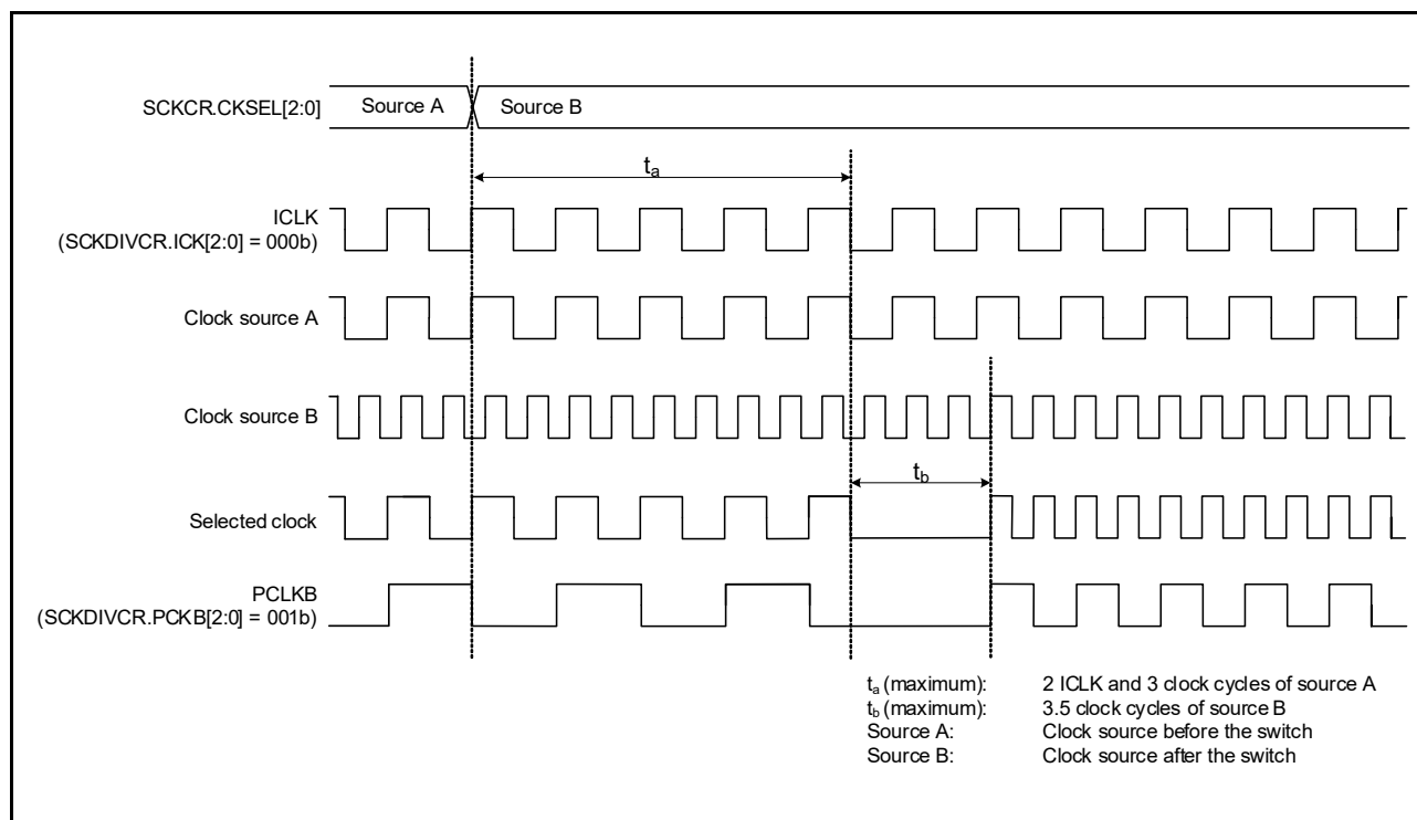
Figure 8.9 Clock source switching timing diagram
