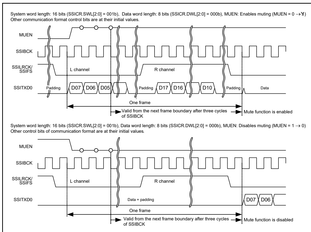
Figure 33.4 Transmit data with the mute function set
