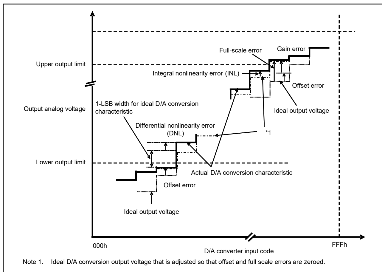
Figure 48.71 Illustration of D/A converter characteristic terms
