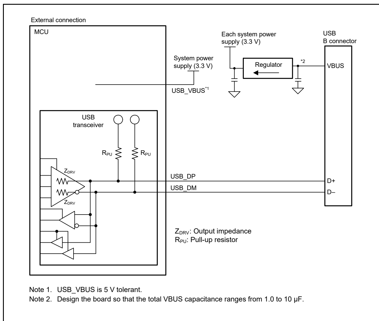
Figure 27.8 Example device connection in bus-powered state 1
