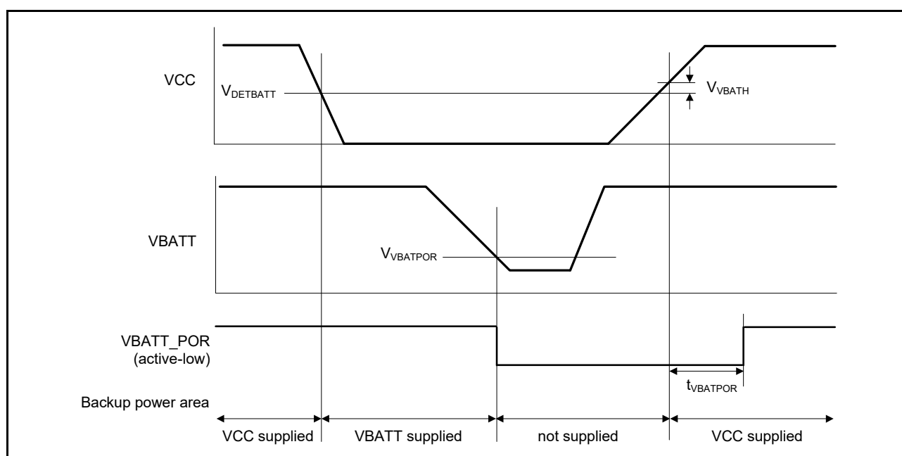
Figure 48.79 VBATT_POR reset timing
