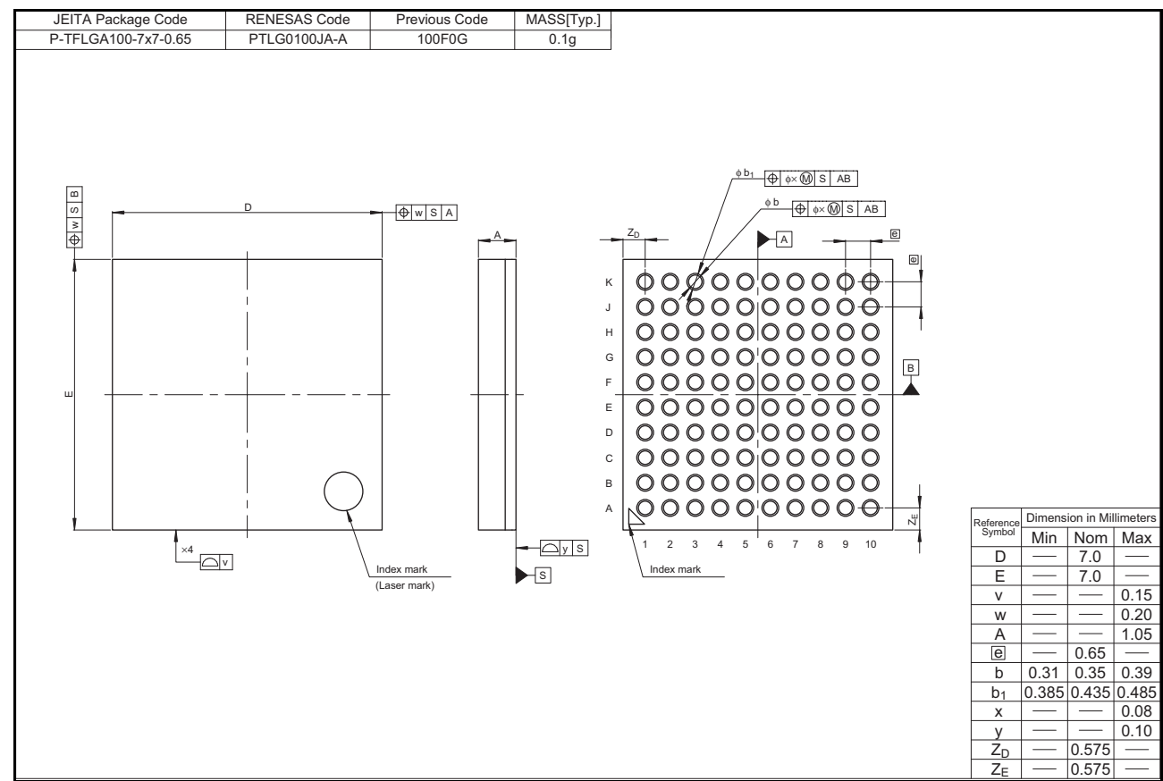
Figure 2.1 100-pin LGA
