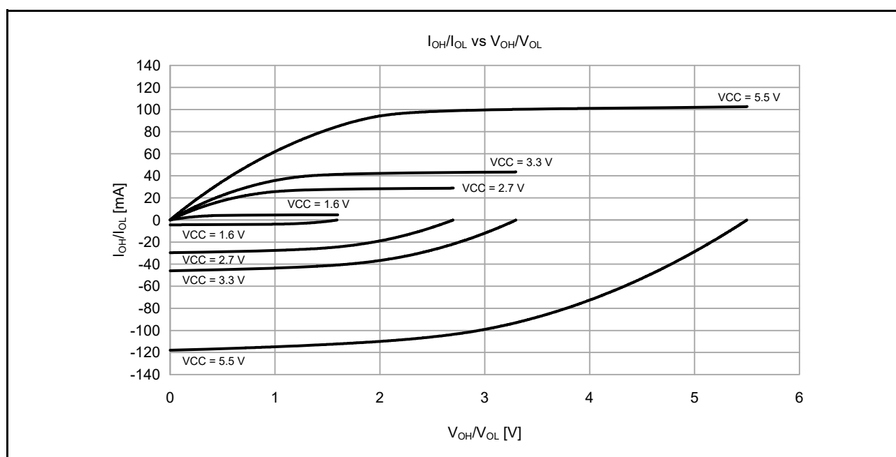
Figure 48.7 V_{OH}/V_{OL} and I_{OH}/I_{OL} voltage characteristics at T_a = 25^\circ\text{C} when middle drive output is selected (reference data)
