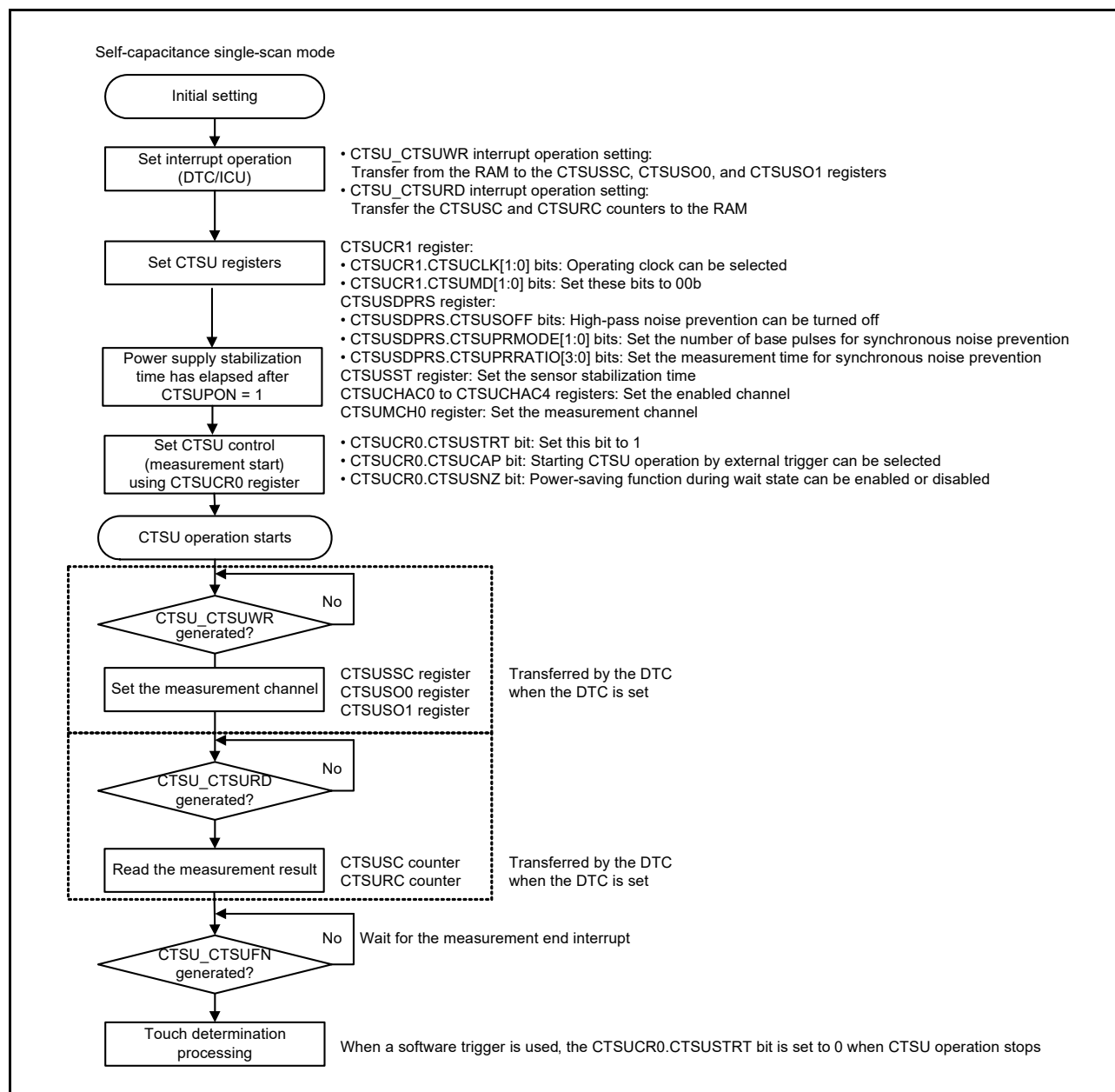
Figure 41.12 Software flow and example operation for self-capacitance single scan mode
