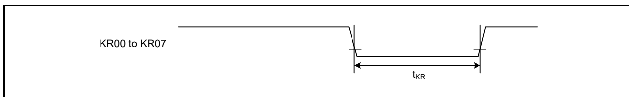
Figure 48.43 Key interrupt input timing
