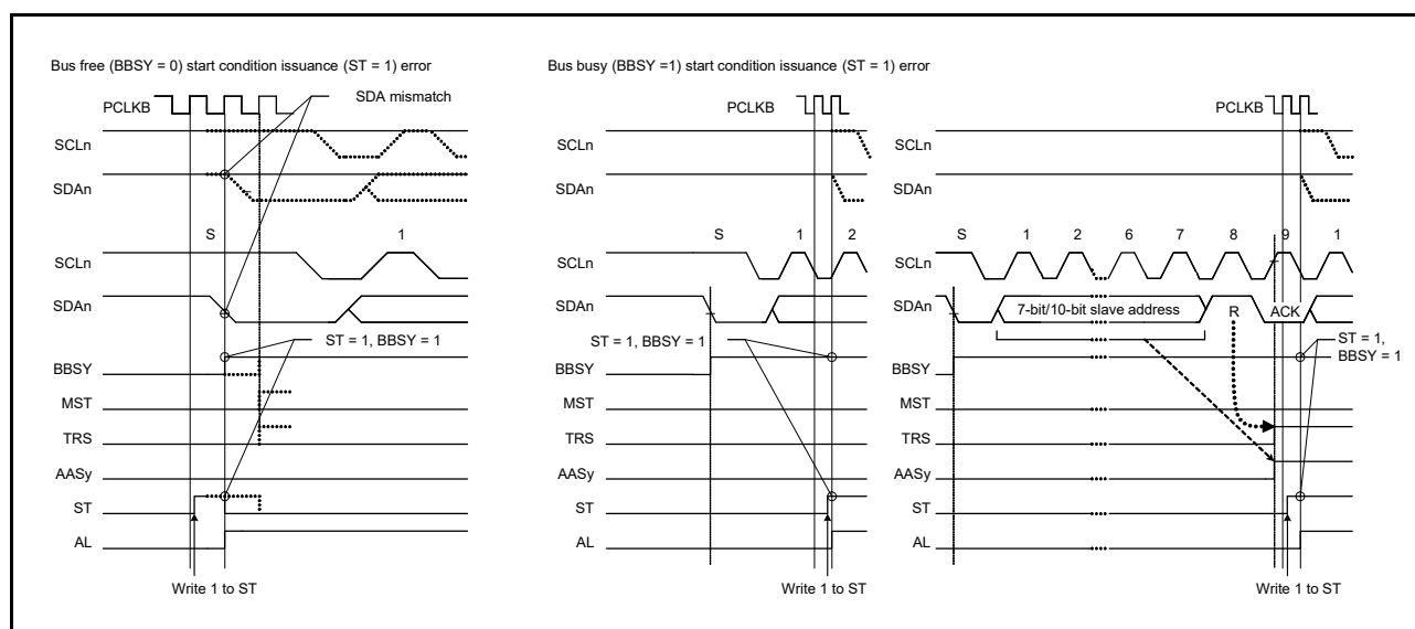
Figure 29.42 Arbitration-lost when start condition is issued (MALE = 1)
