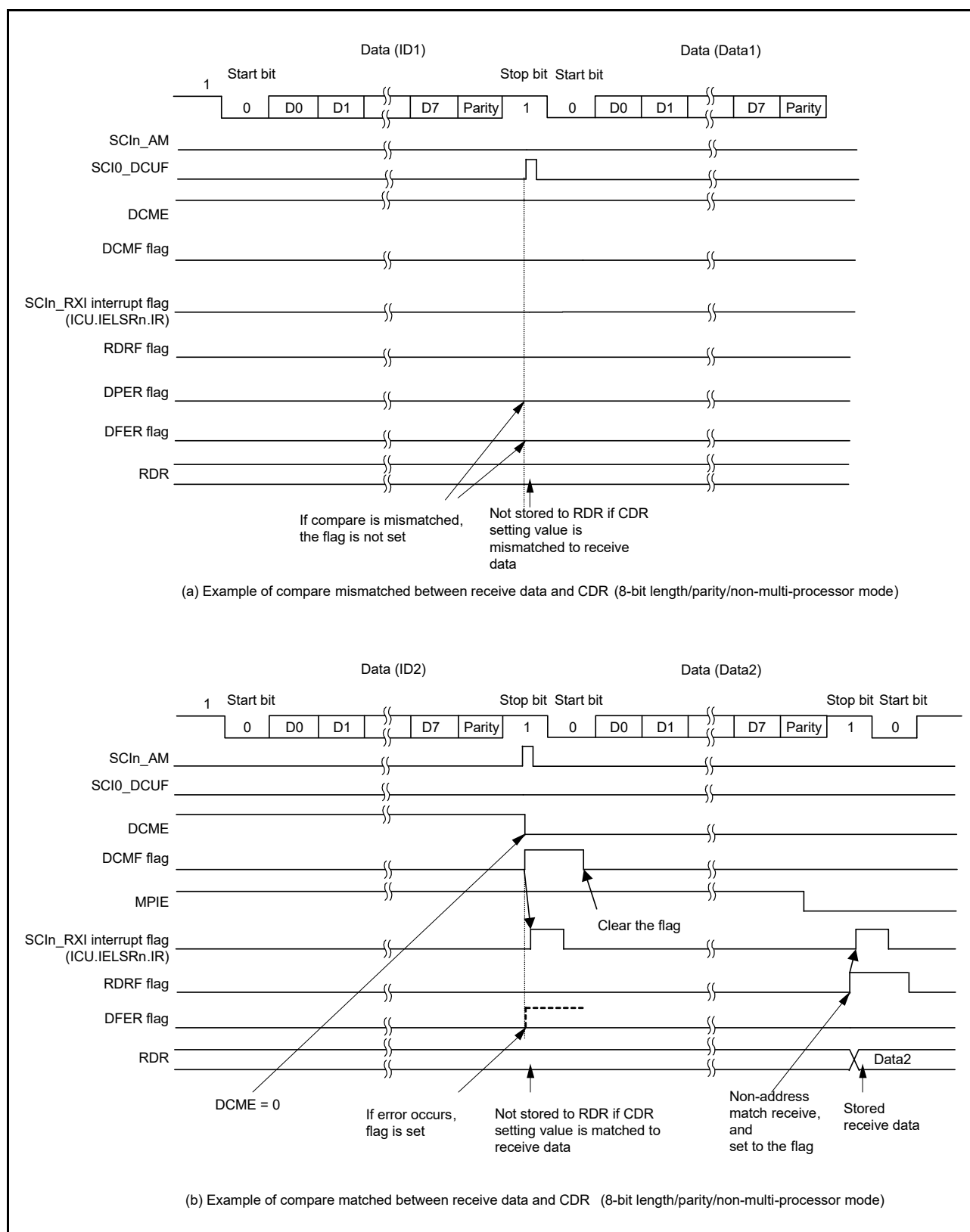
Figure 28.5 Example of address match (1) in non-multi-processor mode
