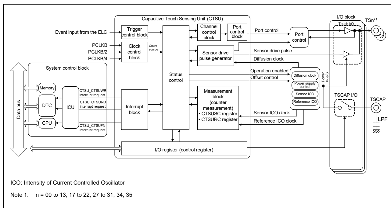
Figure 41.3 CTSU block diagram
