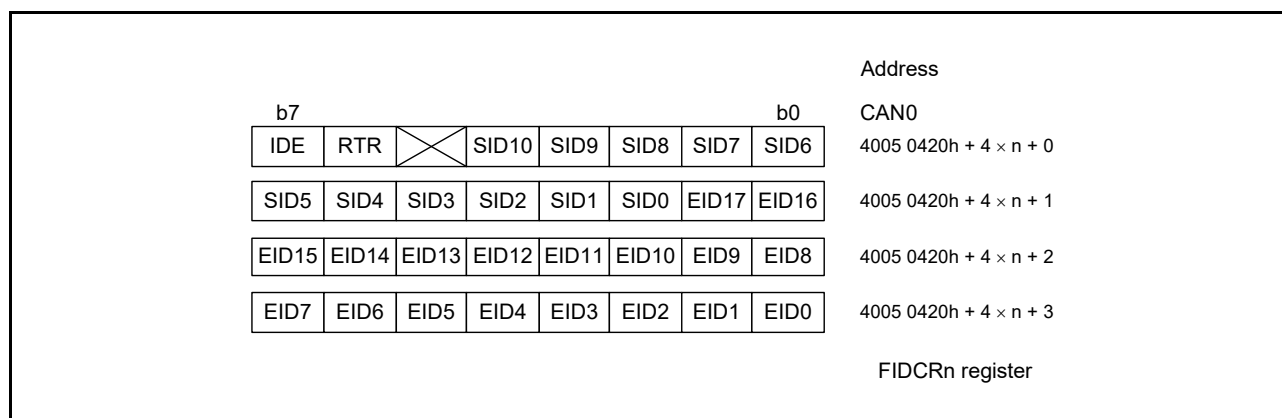
Figure 30.15 Structure of FIDCRn (n = 0, 1)
