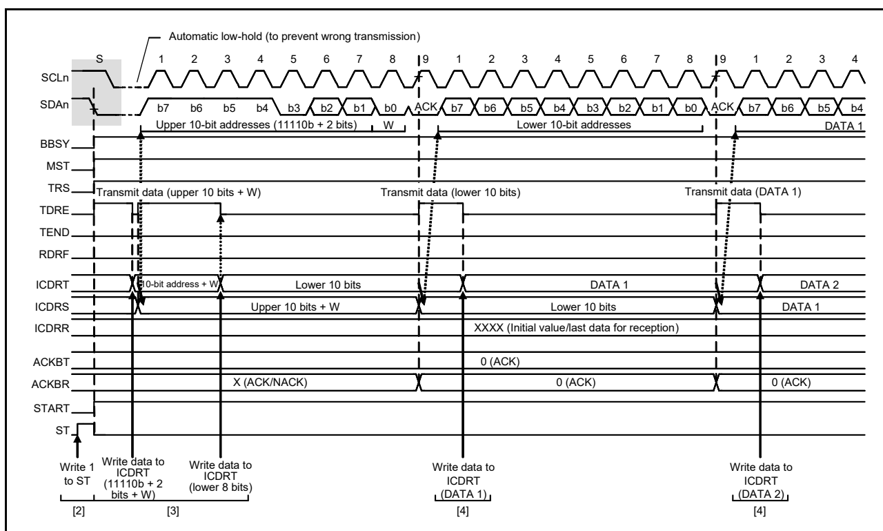
Figure 29.8 Master transmit operation timing (2) (10-bit address format)
