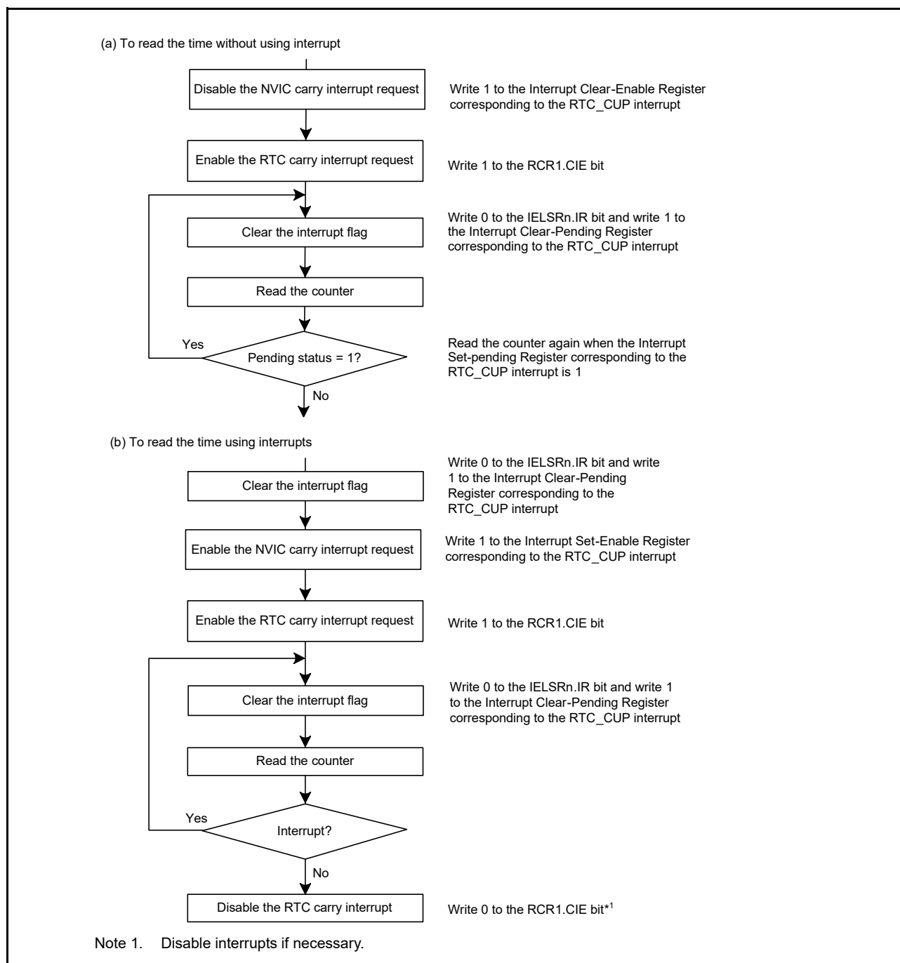
Figure 24.6 Reading time
