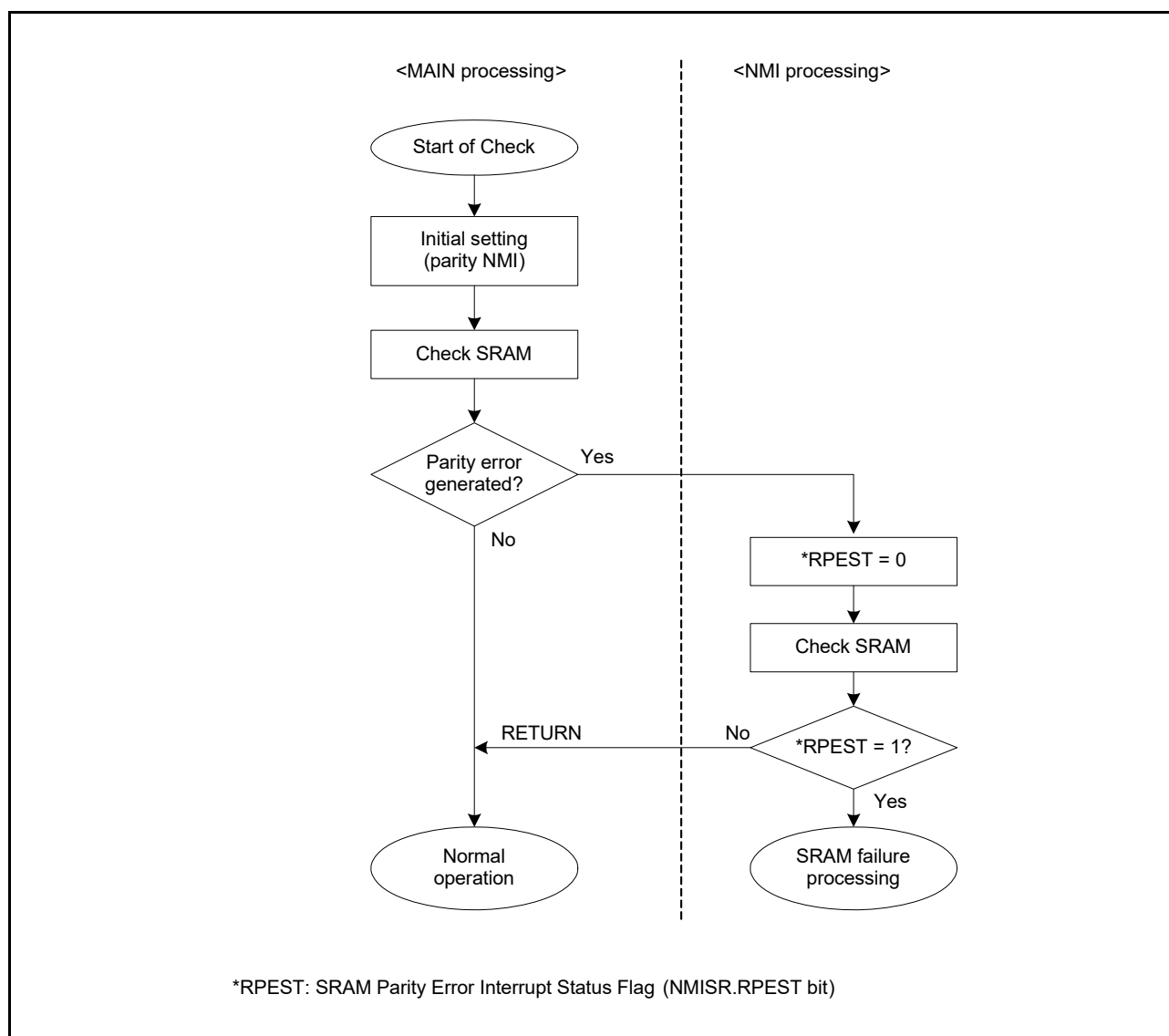
Figure 43.3 Flow of SRAM parity check when SRAM parity interrupt is enabled
