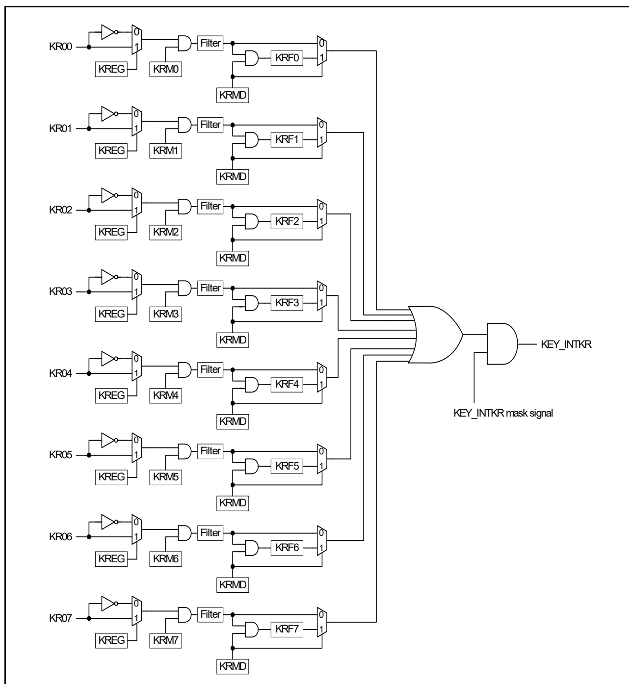
Figure 20.1 Key interrupt function block diagram
