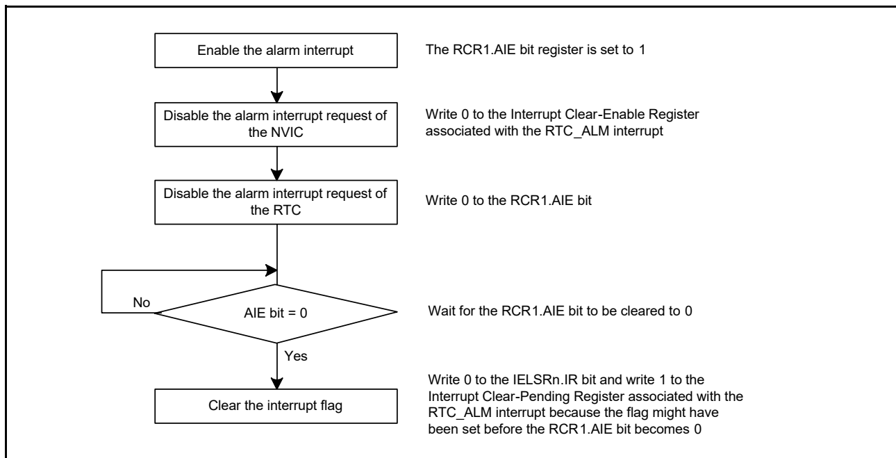
Figure 24.8 Procedure for disabling alarm interrupt request
