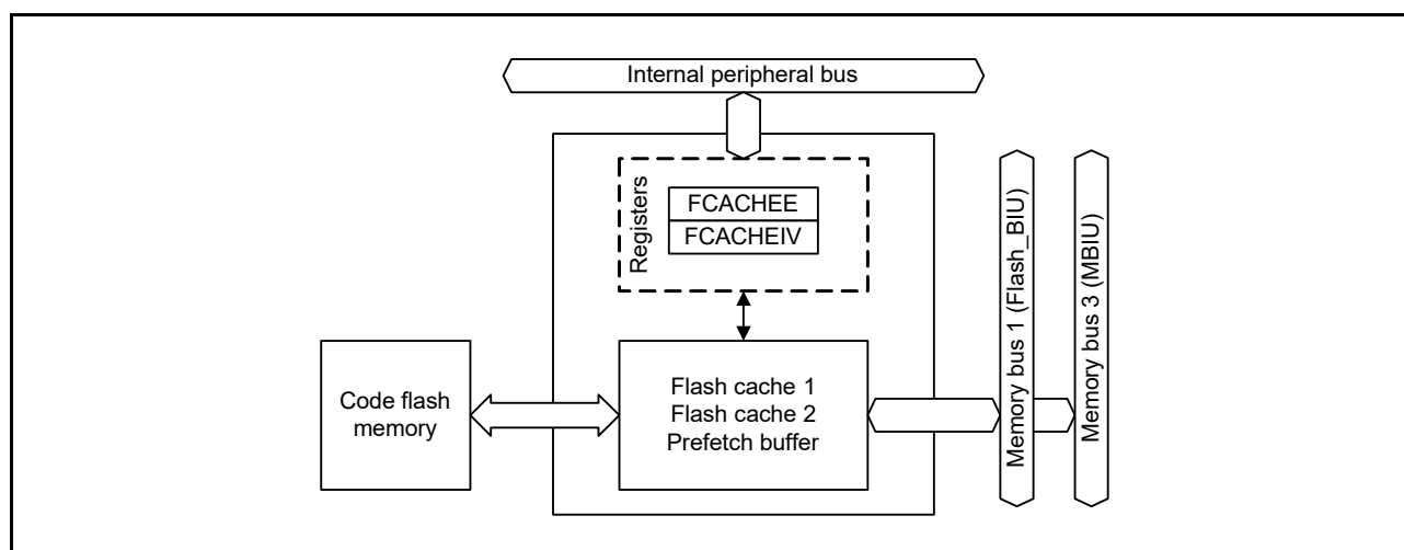
Figure 44.4 FCACHE block diagram
