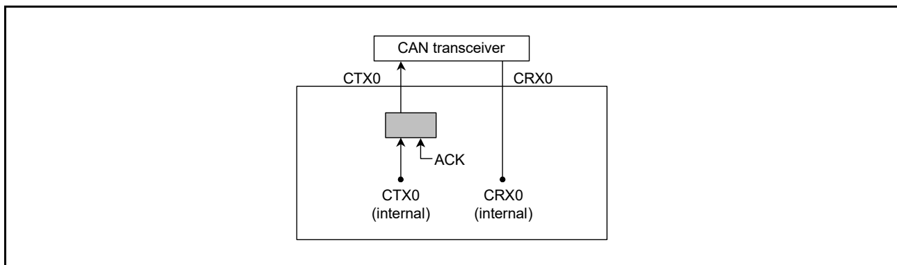
Figure 30.7 Connection when self-test mode 0 is selected
