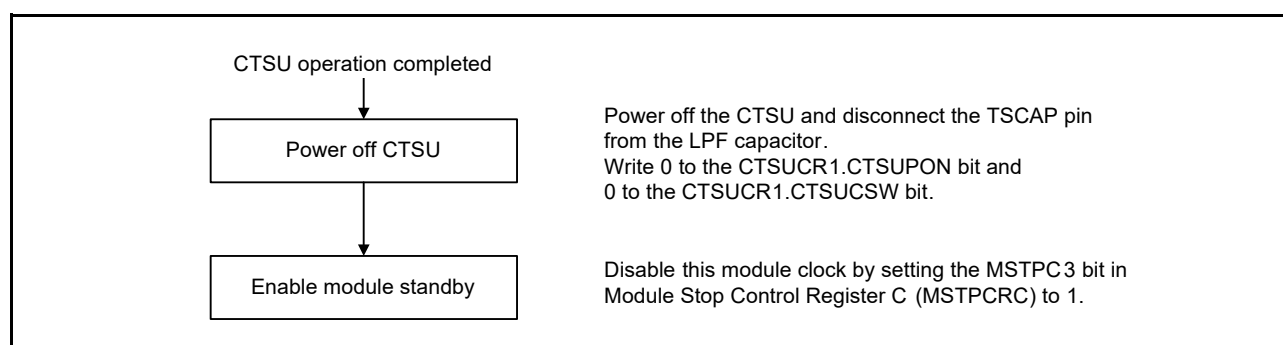
Figure 41.10 CTSU stopping flow
