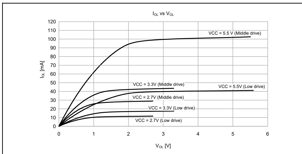
Figure 48.16 V_{OH}/V_{OL} and I_{OH}/I_{OL} voltage characteristics at T_a = 25^\circ\text{C}
