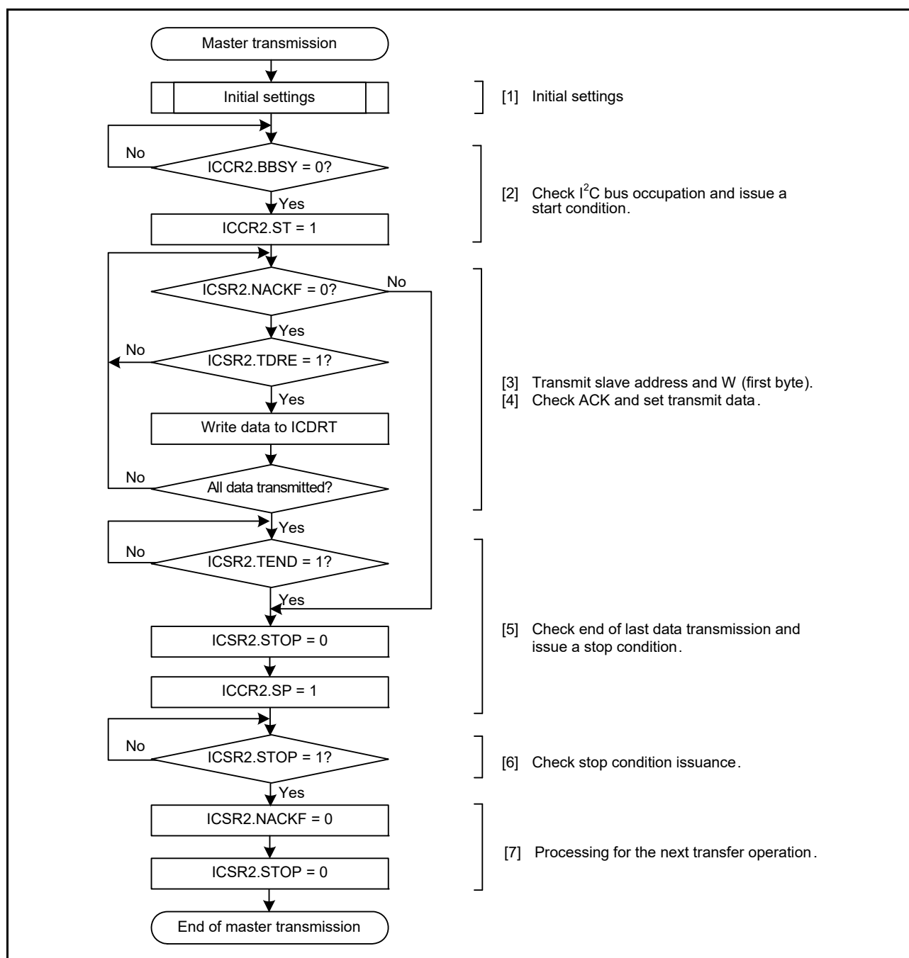
Figure 29.6 Example of master transmission flow
