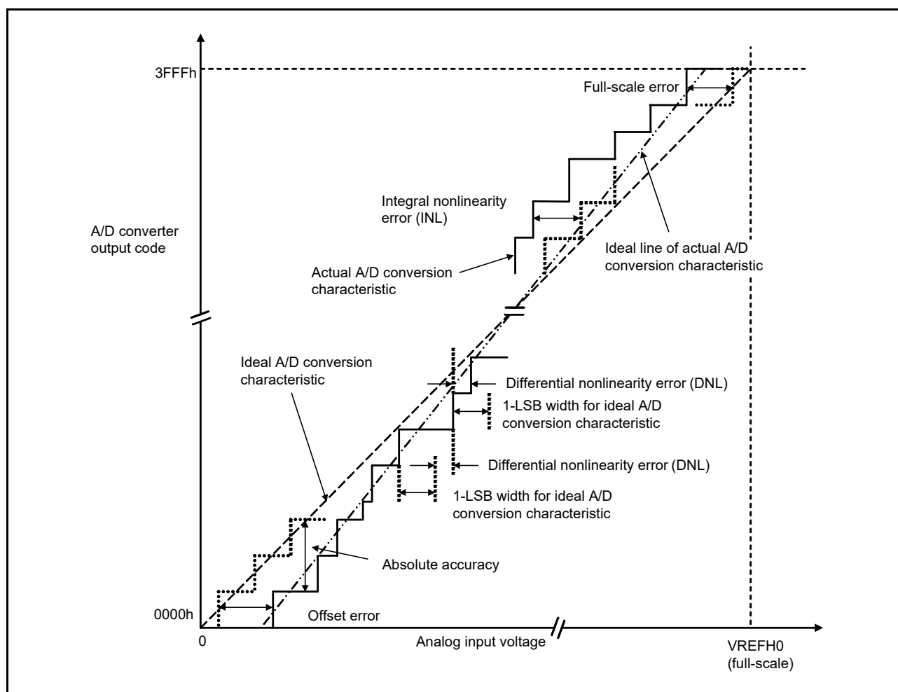
Figure 48.70 Illustration of 14-bit A/D converter characteristic terms
