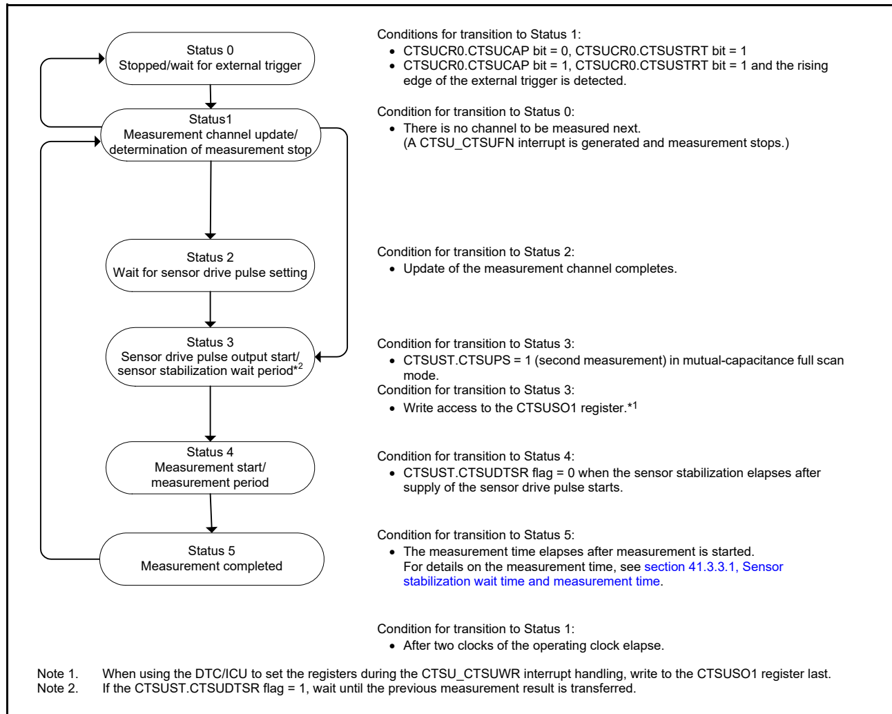
Figure 41.11 Status operation transitions
