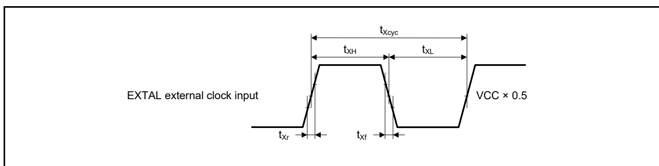
Figure 48.25 EXTAL external clock input timing
