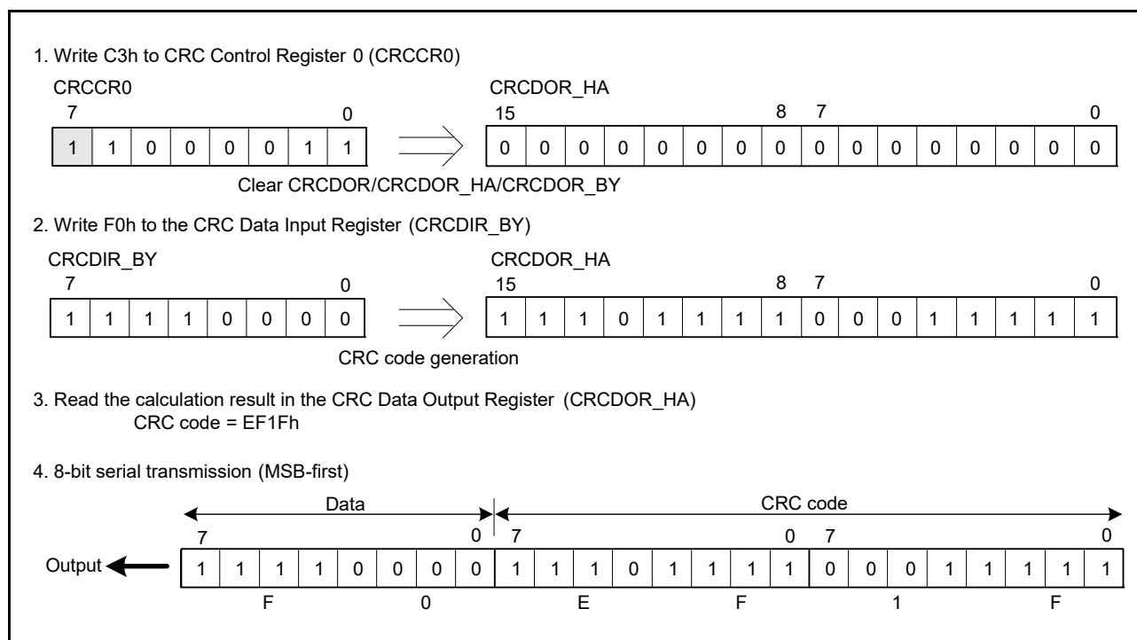
Figure 32.3 MSB-first data transmission
