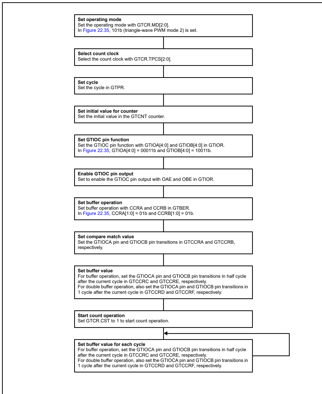
Figure 22.36 Example setting for triangle-wave PWM mode 2
