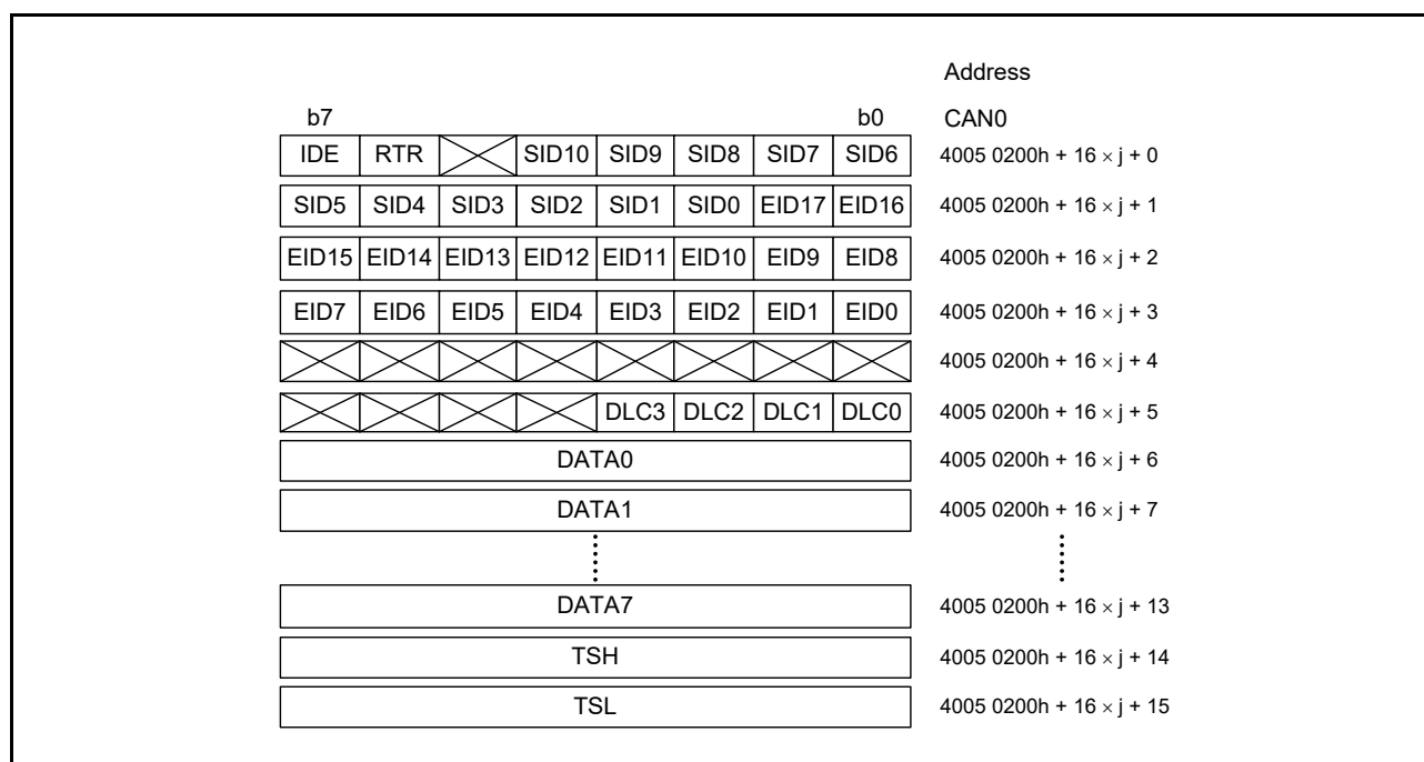
Figure 30.13 Structure of mailbox register (j = 0 to 31)
