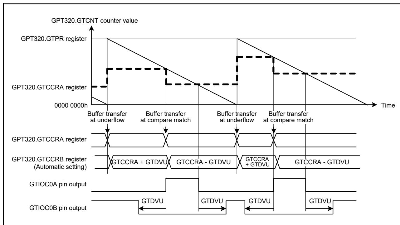
Figure 22.40 Example of automatic dead time setting function operation with saw-wave one-shot pulse mode, down-counting, and active-high
