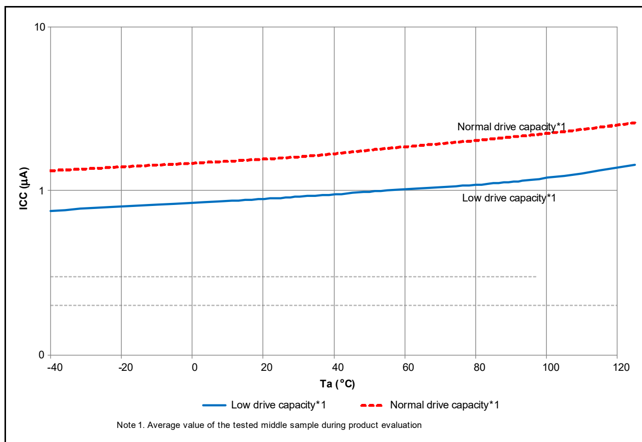
Figure 48.23 Temperature dependency of RTC operation with VCC off (reference data)
