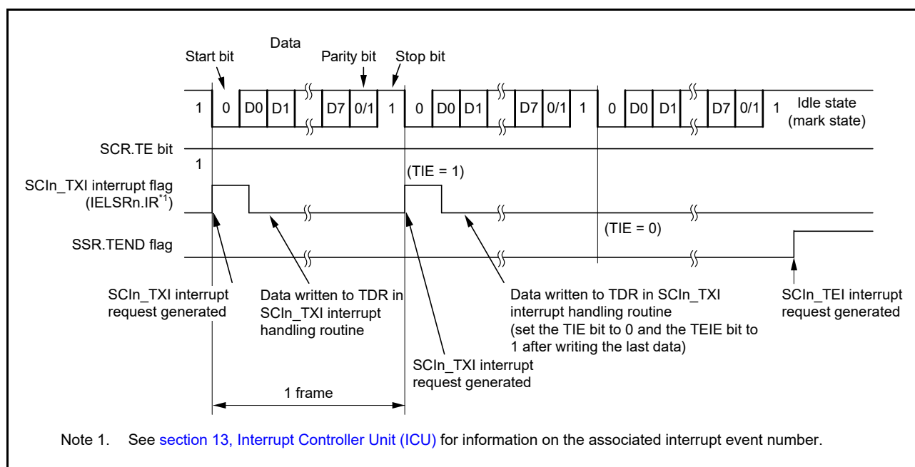
Figure 28.11 Example operation of serial transmission in asynchronous mode (3) with 8-bit data, parity bit, 1 stop bit, CTS function not used, and from the middle of transmission until transmission completion
