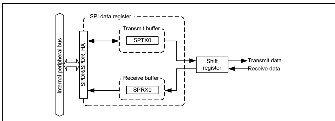
Figure 31.2 Configuration of SPDR/SPDR_HA
