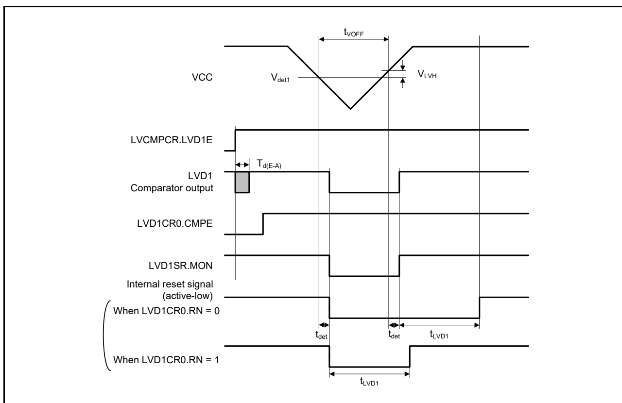
Figure 48.76 Voltage detection circuit timing ( V_{det1} )
