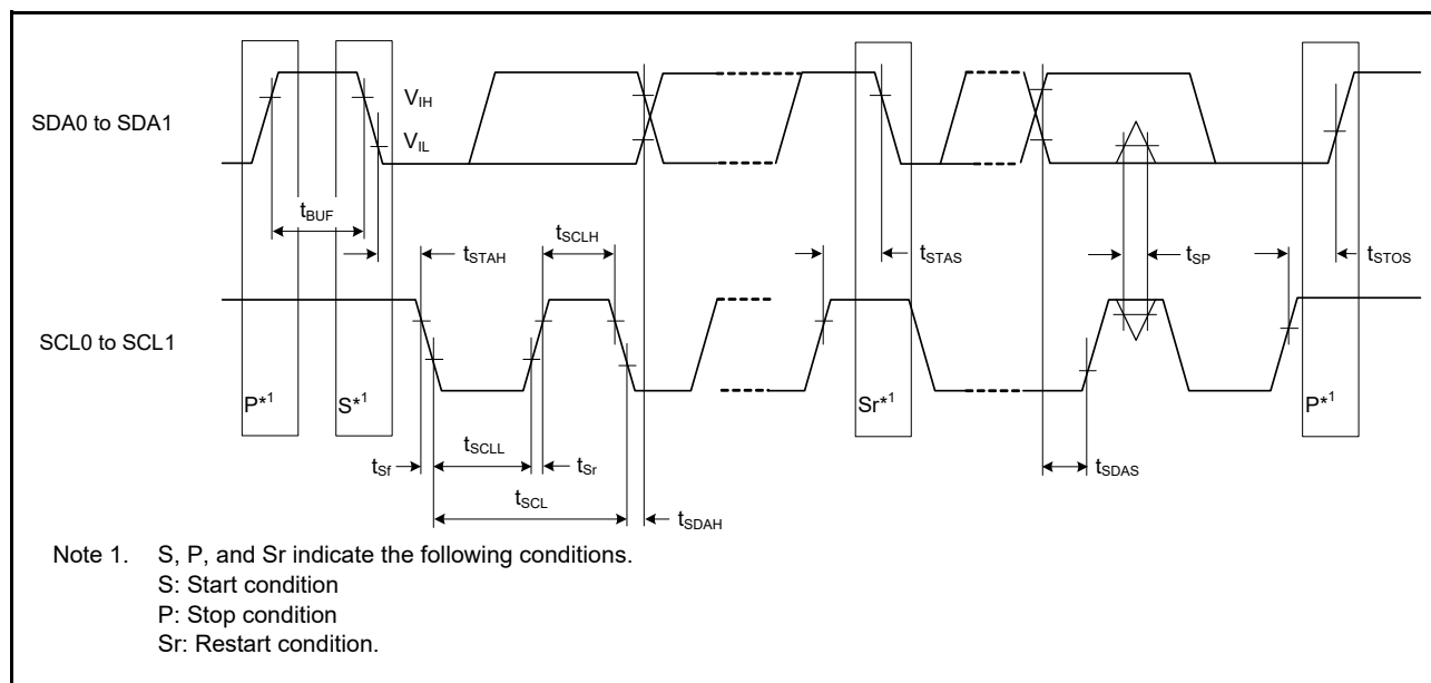
Figure 48.59 IIC bus interface input/output timing
