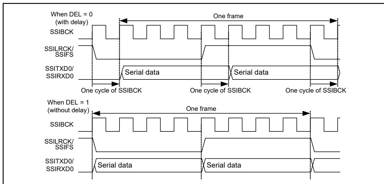
Figure 33.6 Setting of delay in serial data
