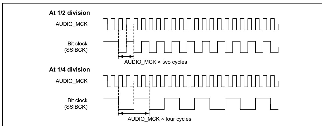
Figure 33.5 Sampling frequencies in master mode communication
