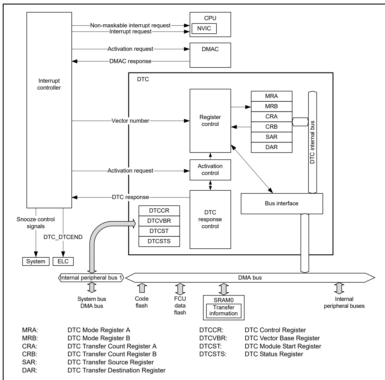
Figure 17.1 DTC block diagram
