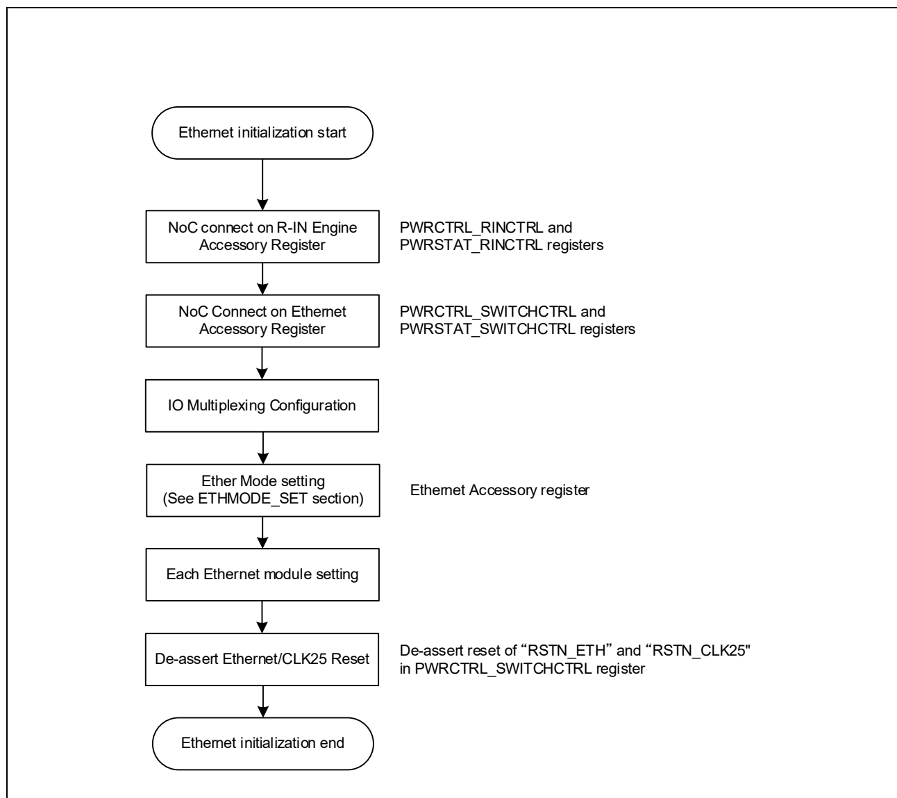
Figure 8.3 Initializing of Ethernet Flowchart
