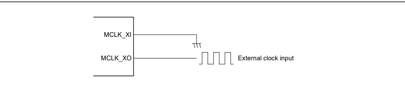
Figure 3.3 Example of External Clock Connection
