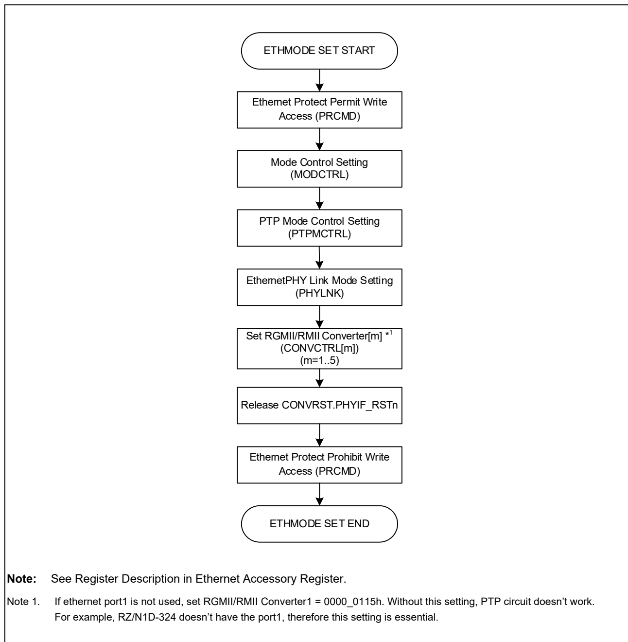
Figure 8.4 ETHMODE_SET Flowchart
