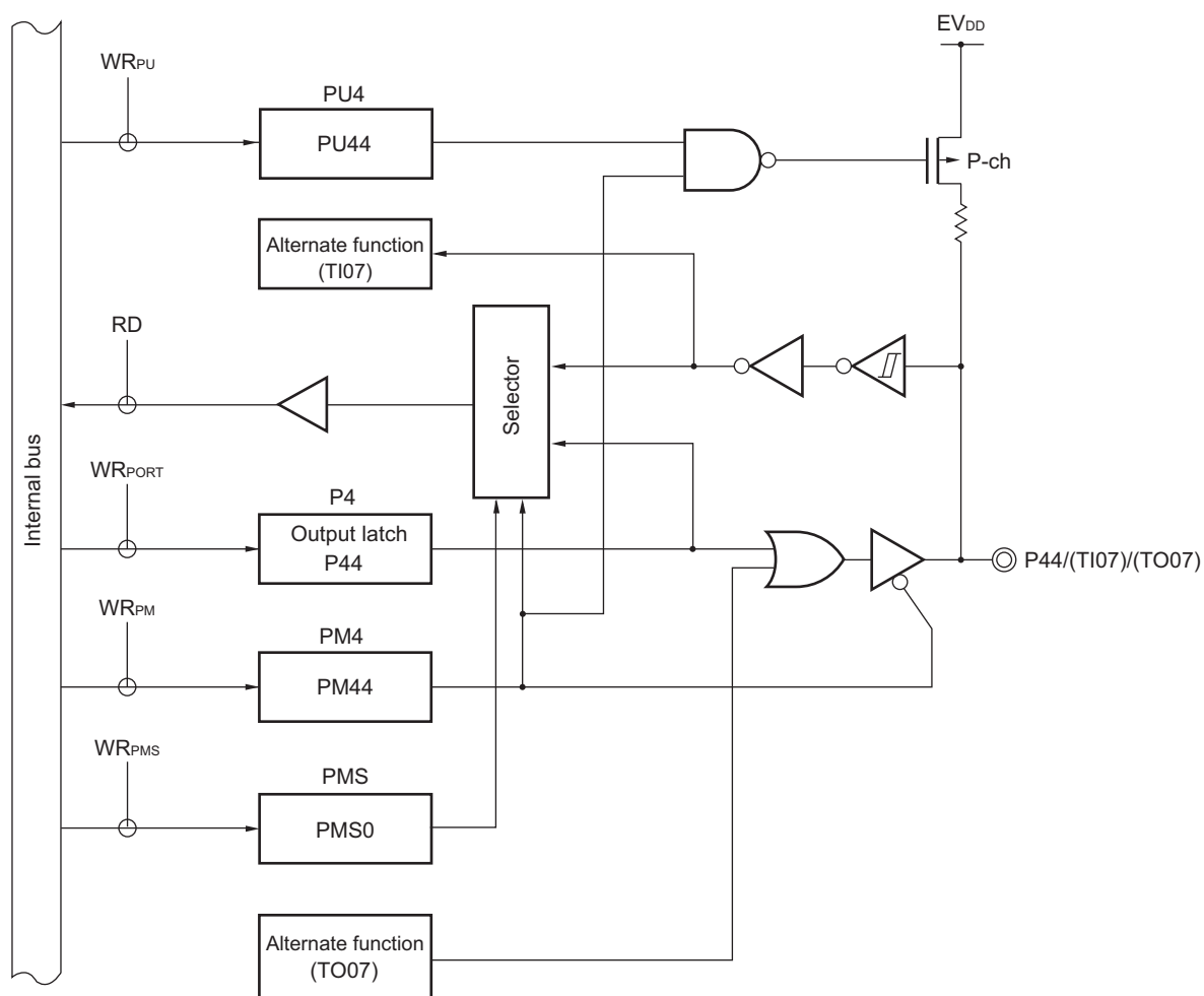
Figure 4-33. Block Diagram of P44
