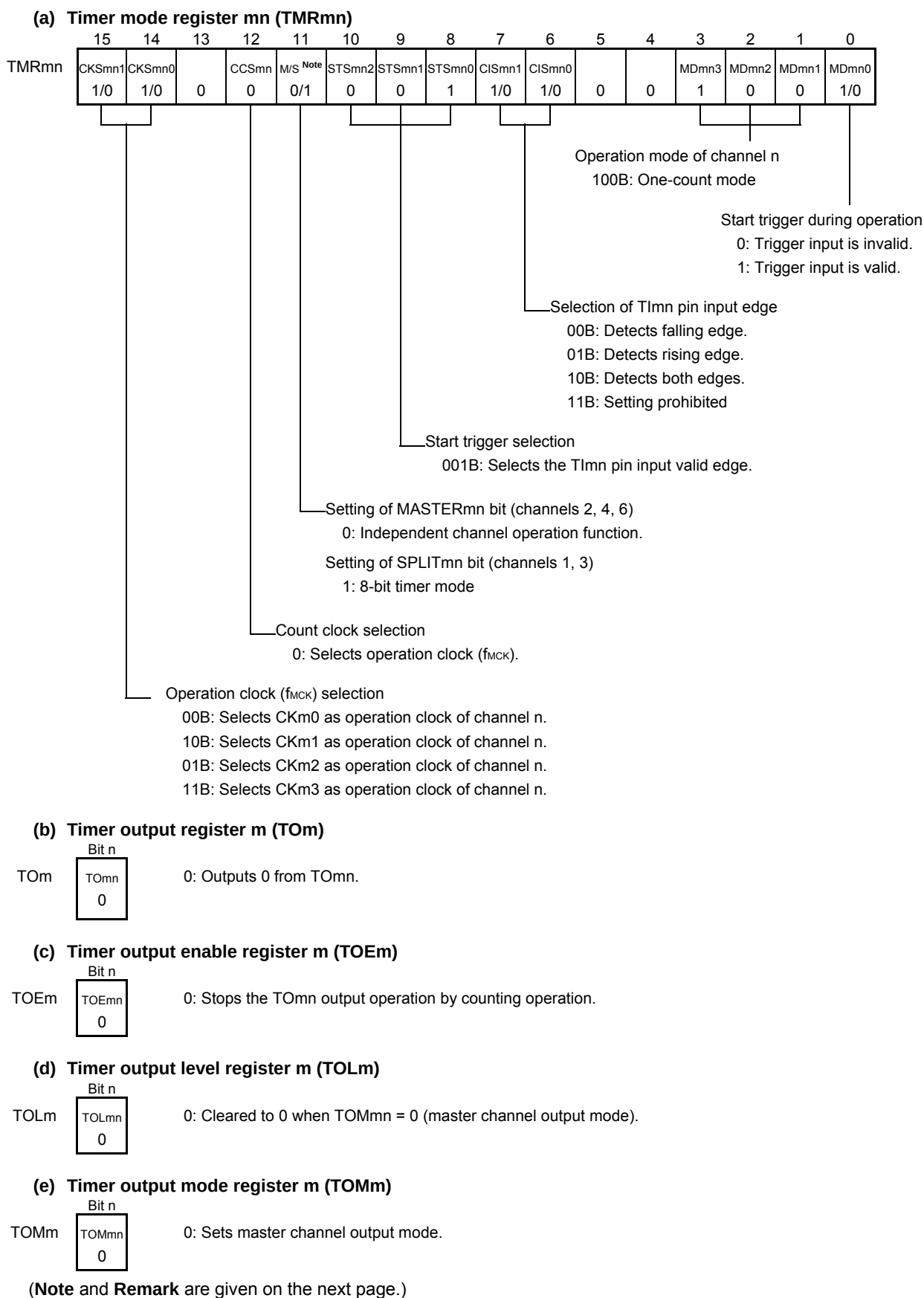
Figure 6-67 Example of Set Contents of Registers to Delay Counter
