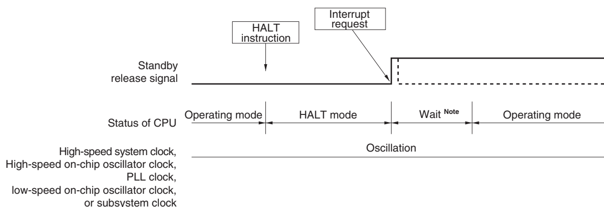
Figure 24-4. HALT Mode Release by Interrupt Request Generation
