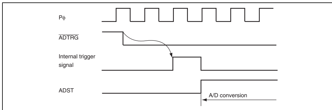
Figure 21.6 External Trigger Input Timing
