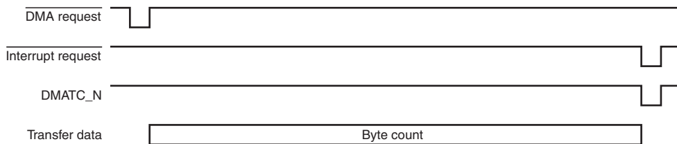
Figure 11.4 DMA Transfer Conditions
