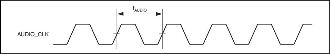
Figure 33.41 AUDIO_CLK Input Timing
