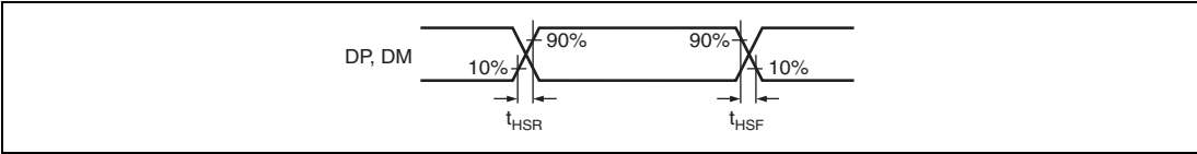
Figure 33.58 DP and DM Output Timing (High-Speed)
