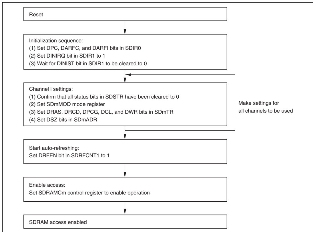
Figure 10.25 (a) SDRAMC Setting Procedure (Basic Setting Example)
