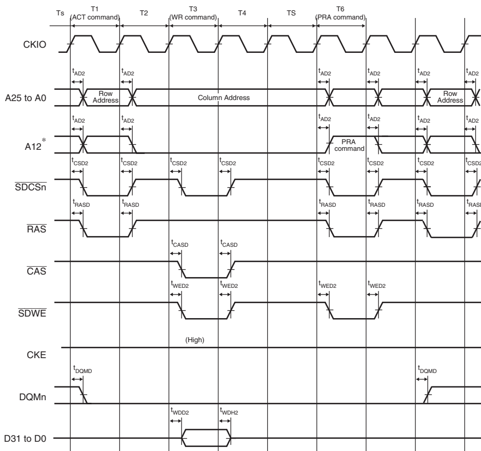
Figure 33.17 SDRAM Space: Single-Write Bus Timing (DCL = 2 (2 Cycles), DRCD = 1 (2 Cycles), DPCG = 1 (2 Cycles))
