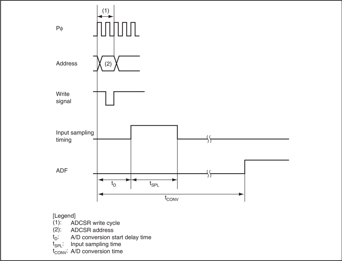
Figure 21.5 A/D Conversion Timing
