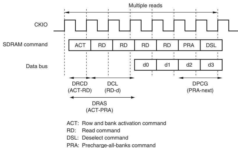
Figure 10.29 Multiple Read Timing Example 1
