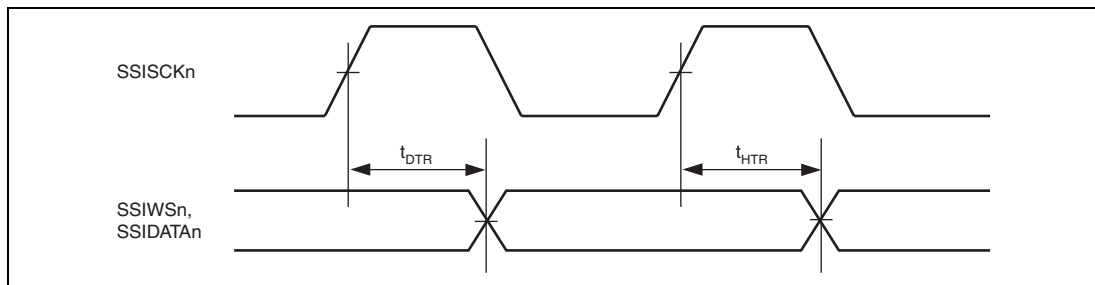
Figure 33.37 SSIF Transmit Timing (1)
