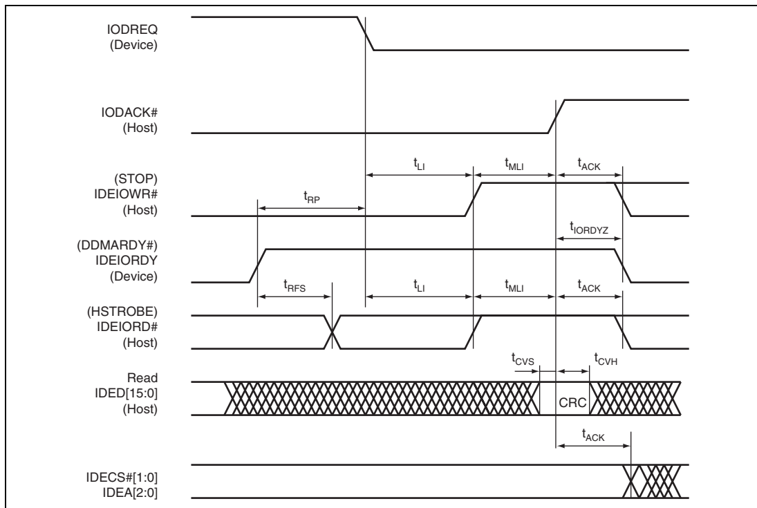
Figure 33.74 Device Terminating Ultra DMA Data-Out Burst
