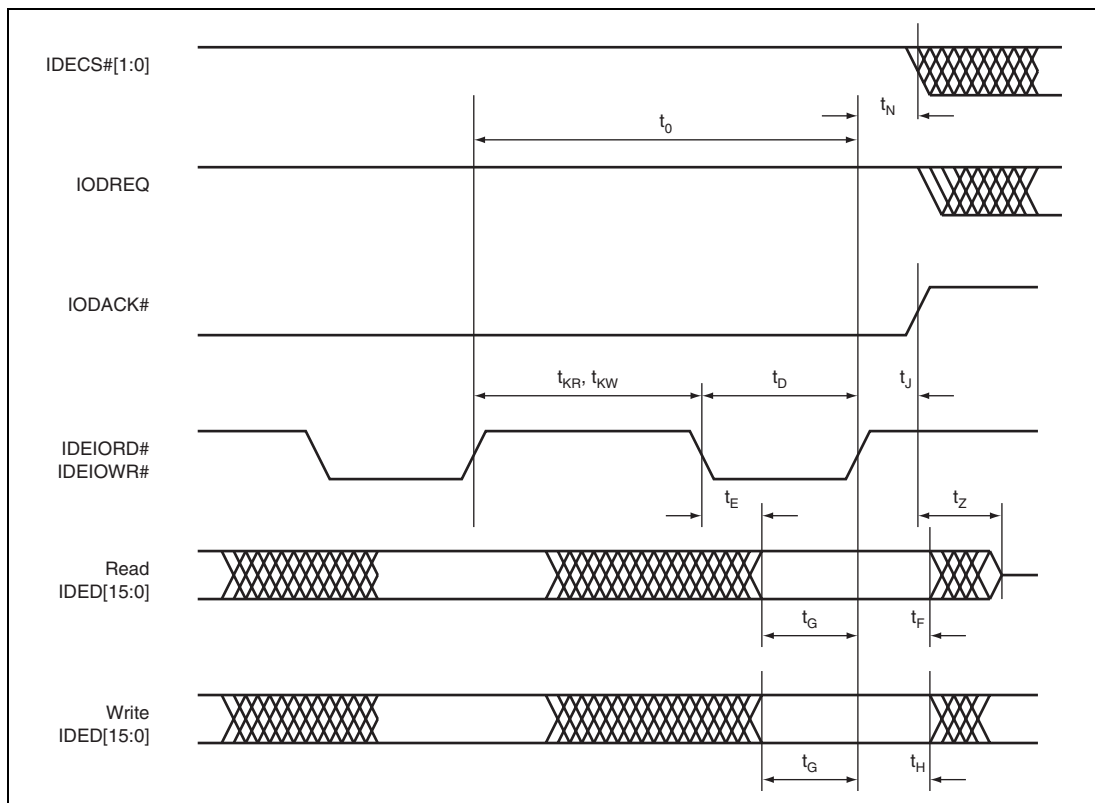
Figure 33.64 Host Terminating Multiword DMA Data Burst
