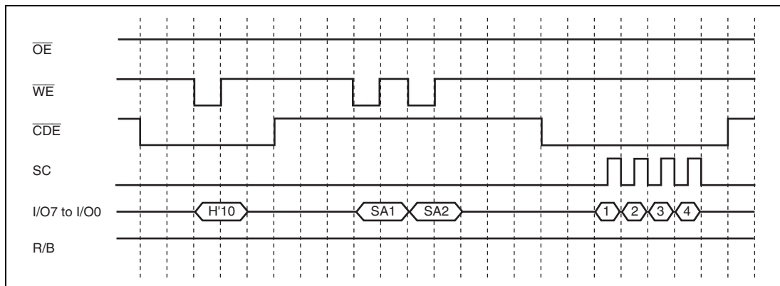
Figure 23.6 Programming Operation Timing for AND-Type Flash Memory (1)
