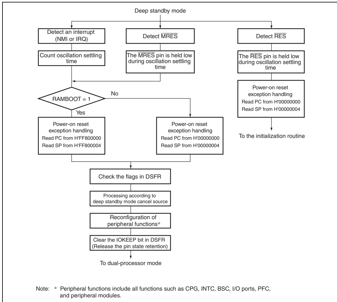
Figure 30.4 Flowchart of Canceling Deep Standby Mode
