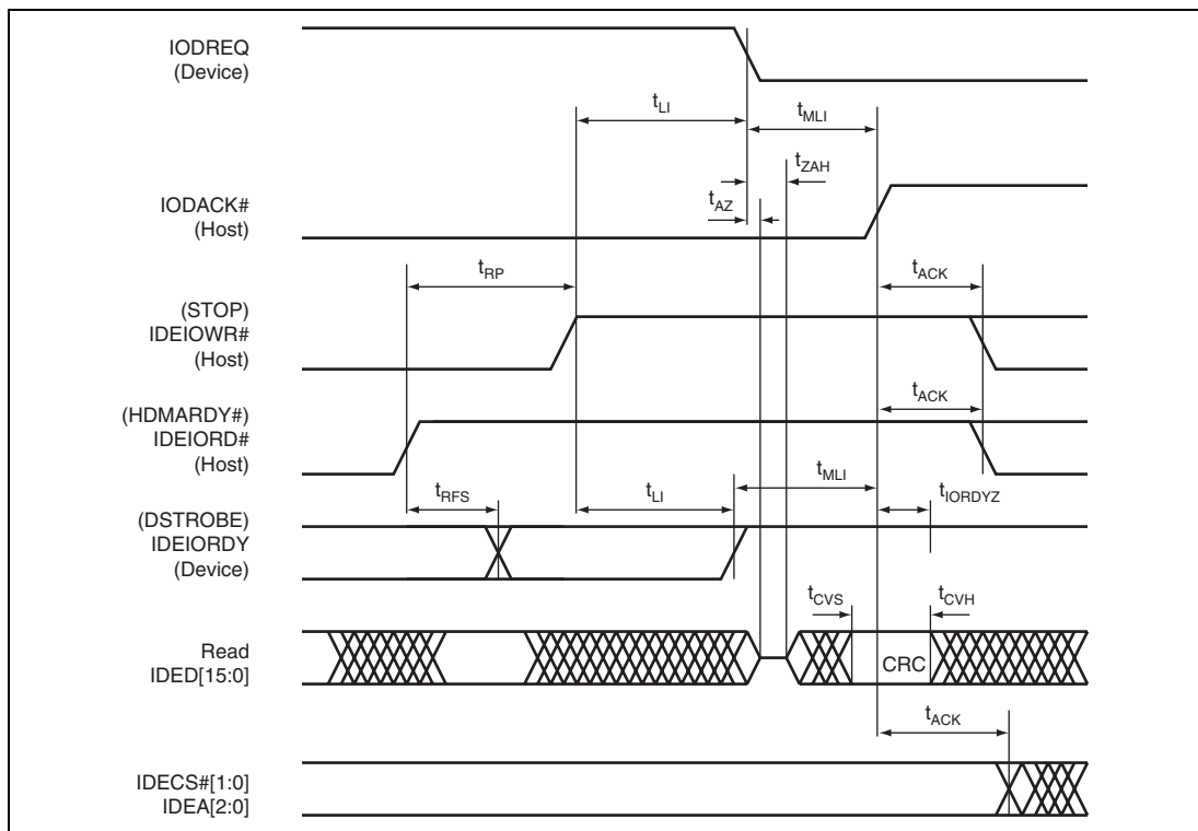
Figure 33.69 Host Terminating Ultra DMA Data-In Burst
