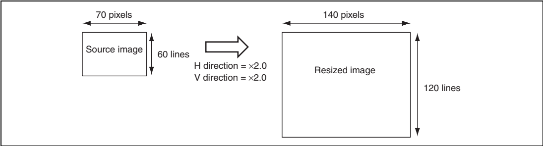
Figure 26.46 Example of Duplicate-line Setting of Enlargement Resizing (2)
