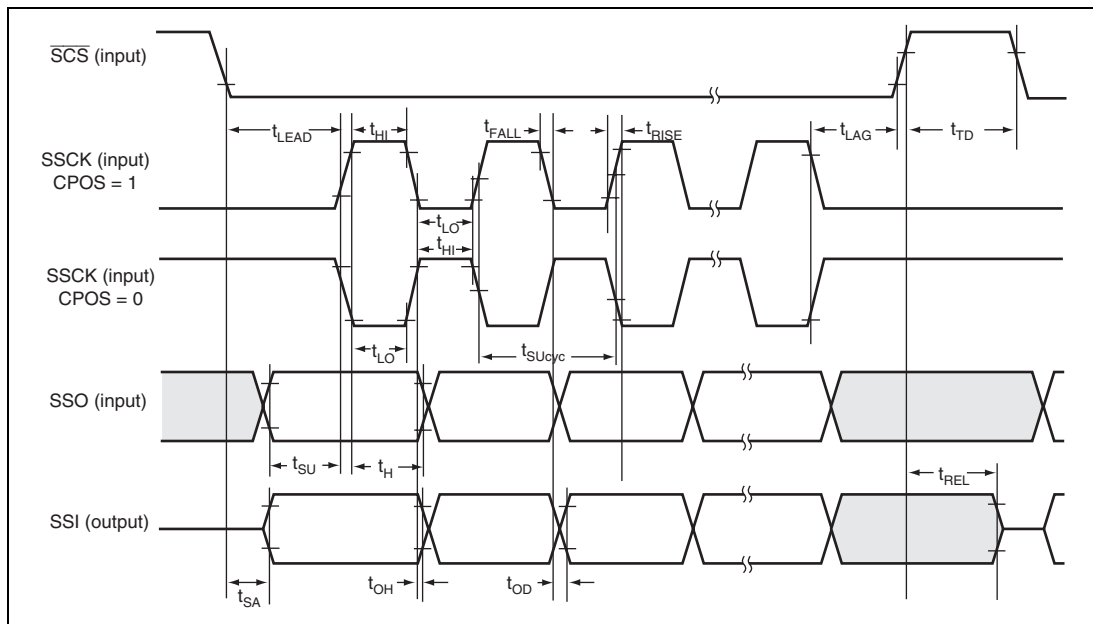
Figure 33.33 SSU Timing (Slave, CPHS = 1)
