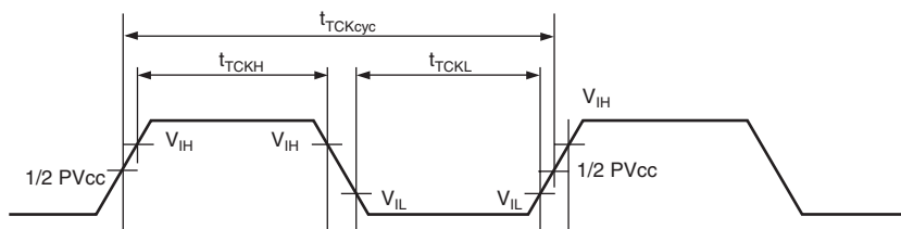
Figure 33.88 TCK Input Timing
