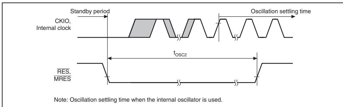
Figure 33.6 Oscillation Settling Time on Return from Standby (Return by Reset)
