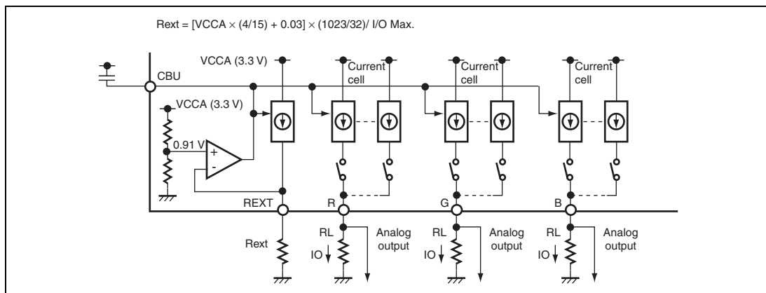
Figure 26.59 Current Cells and Analog Outputs
