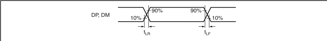
Figure 33.54 DP and DM Output Timing (Low-Speed)
