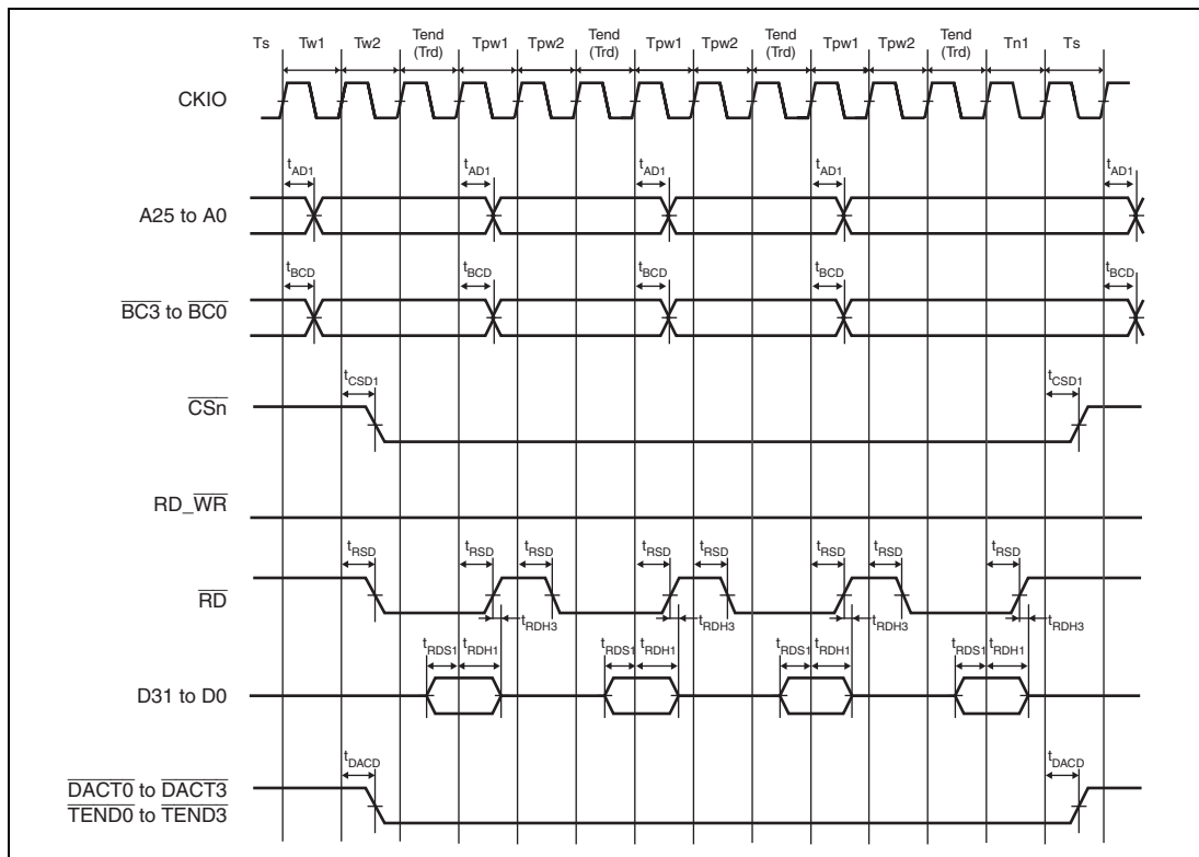
Figure 33.12 External Address Space: Basic Bus Timing
