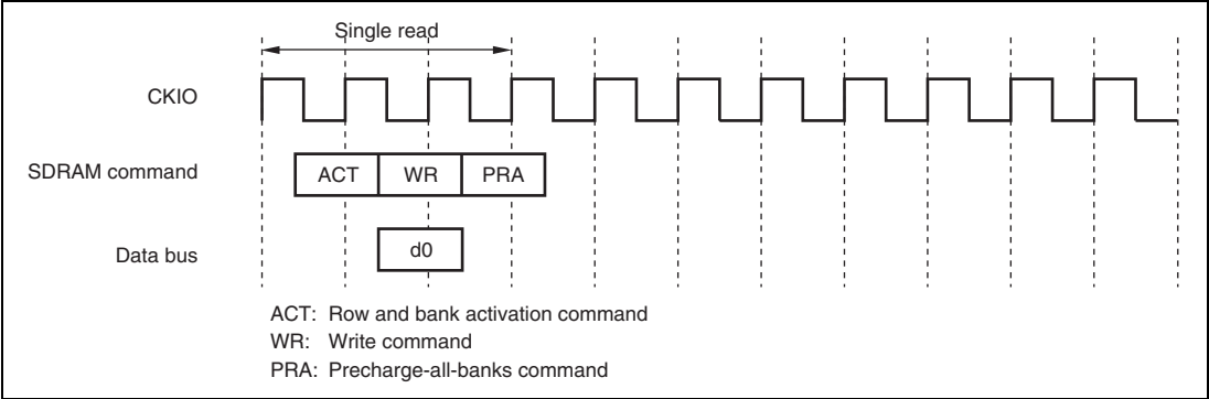
Figure 10.21 Single Write Timing Example (Shortest Timing Settings)
