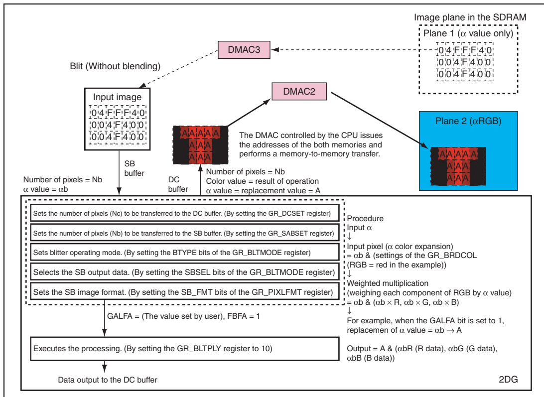
Figure 26.31 Example of Color Gradation Processing (1)
