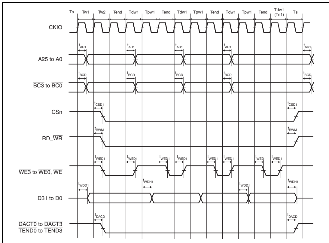
Figure 33.14 External Address Space: Basic Bus Timing
