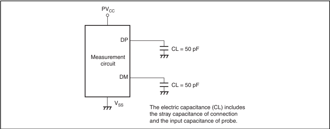
Figure 33.57 Measurement Circuit (Full-Speed)
