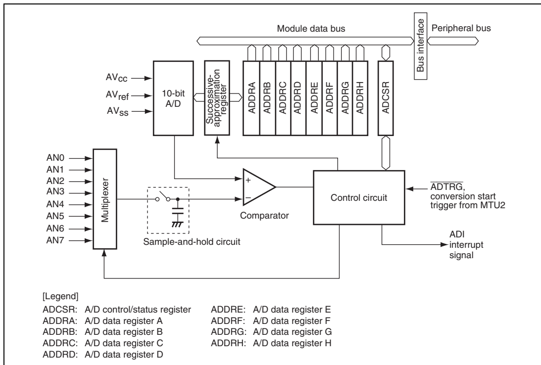
Figure 21.1 Block Diagram of A/D Converter
