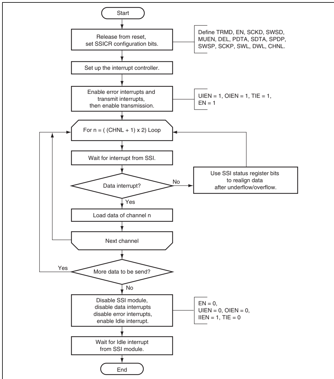
Figure 19.21 Transmission Using Interrupt Data Flow Control
