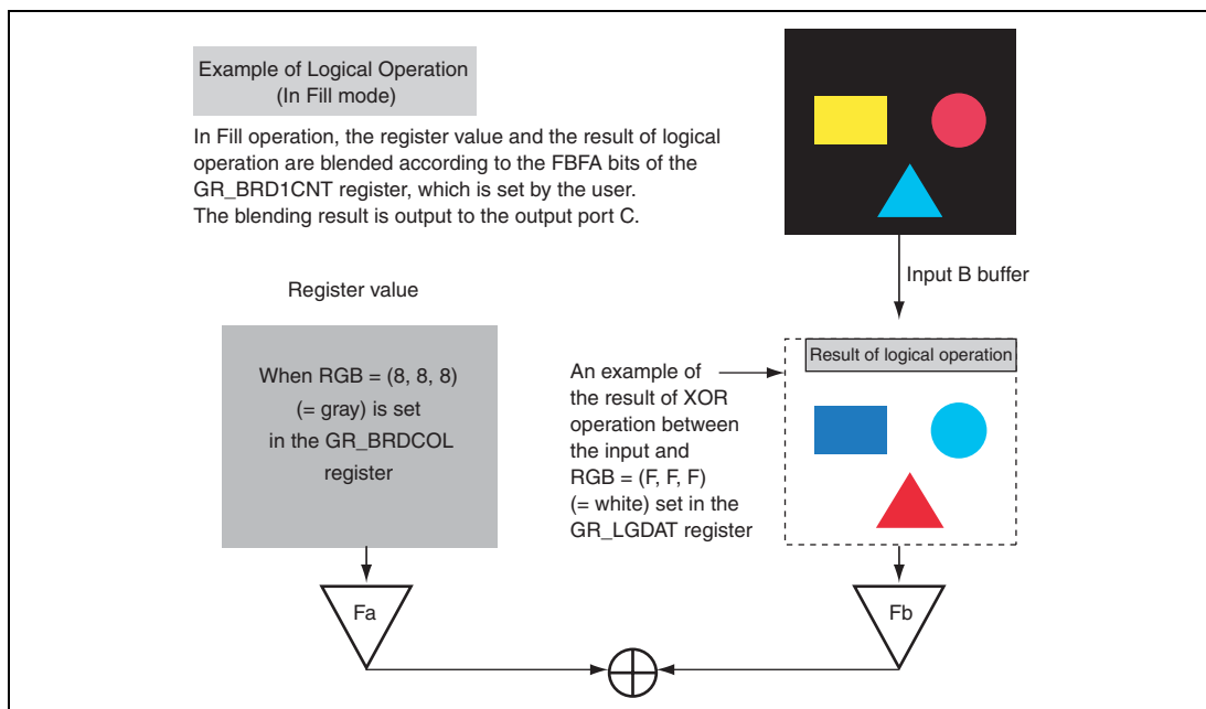
Figure 26.30 Example of Logical Operations
