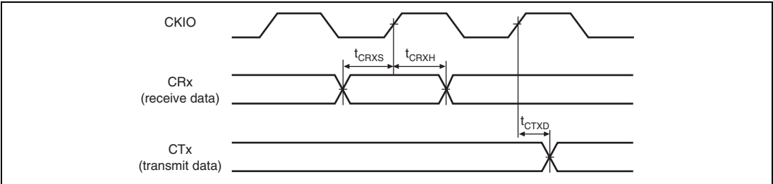
Figure 33.42 RCAN-TL1 Input/Output Timing
