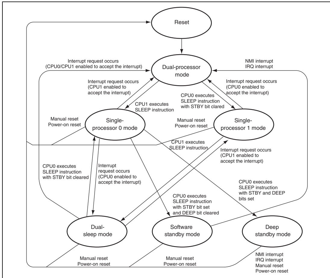
Figure 30.1 Transitions of States in Power-Down Modes
