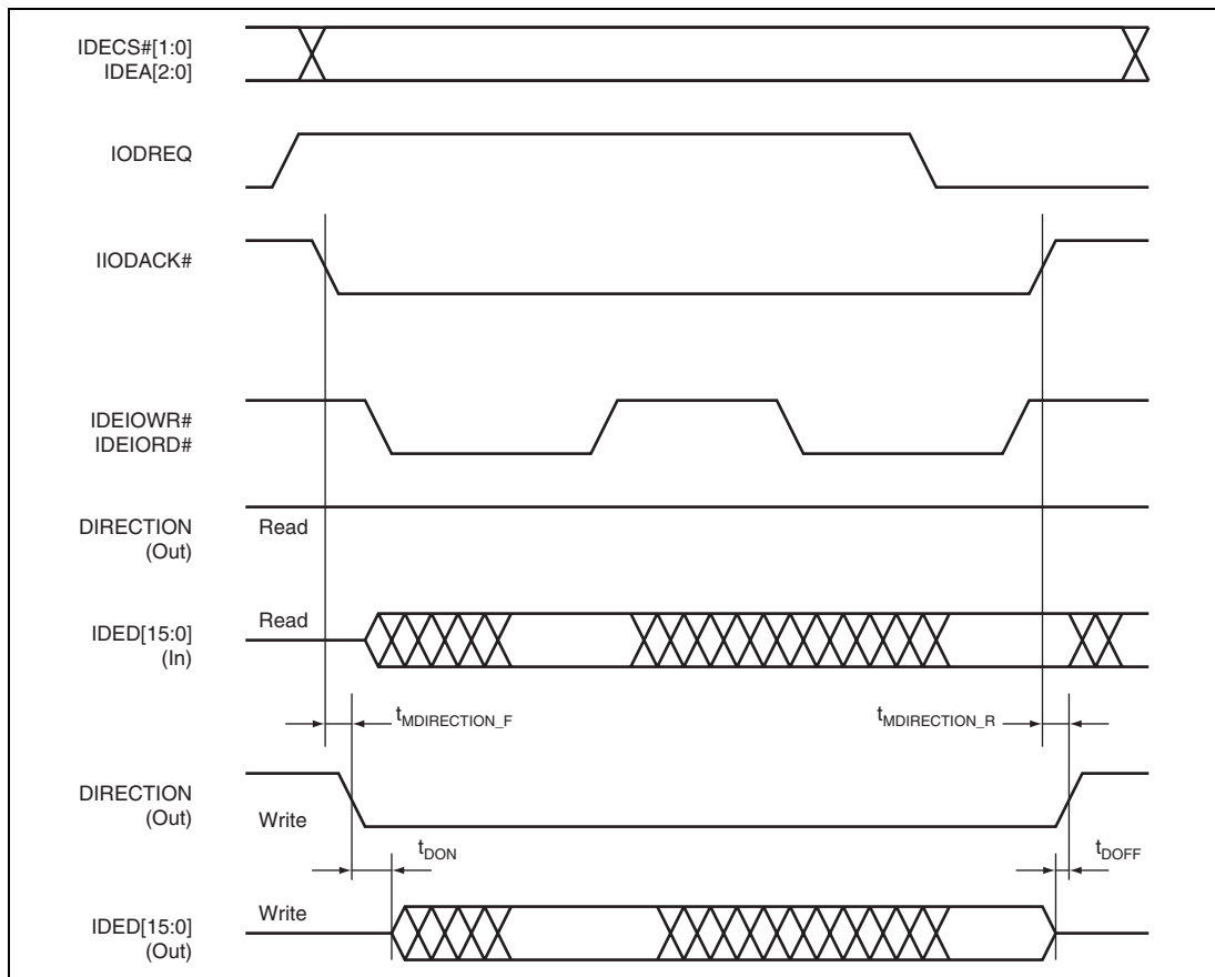
Figure 33.77 Multiword DMA Data Transfer (DIRECTION)
