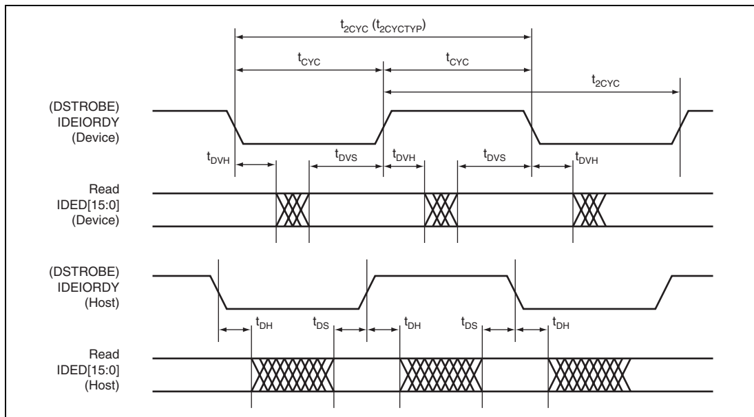
Figure 33.66 Sustained Ultra DMA Data-In Burst
