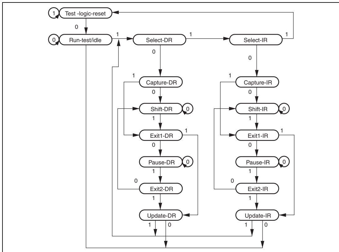
Figure 31.2 TAP Controller State Transitions
