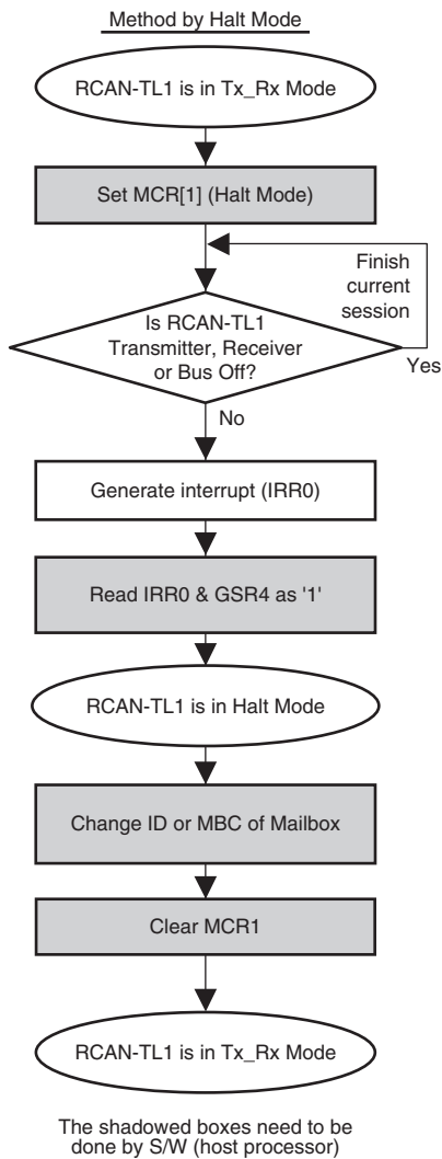
Figure 20.25 Change ID of receive box or Change receive box to transmit box
