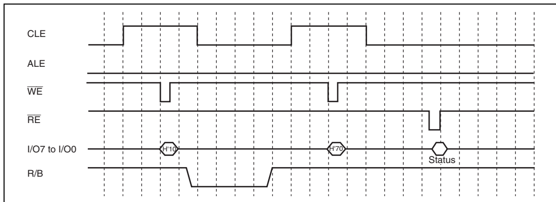
Figure 23.10 Programming Operation Timing for NAND-Type Flash Memory (2)
