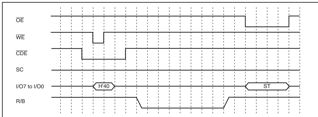
Figure 23.7 Programming Operation Timing for AND-Type Flash Memory (2)
