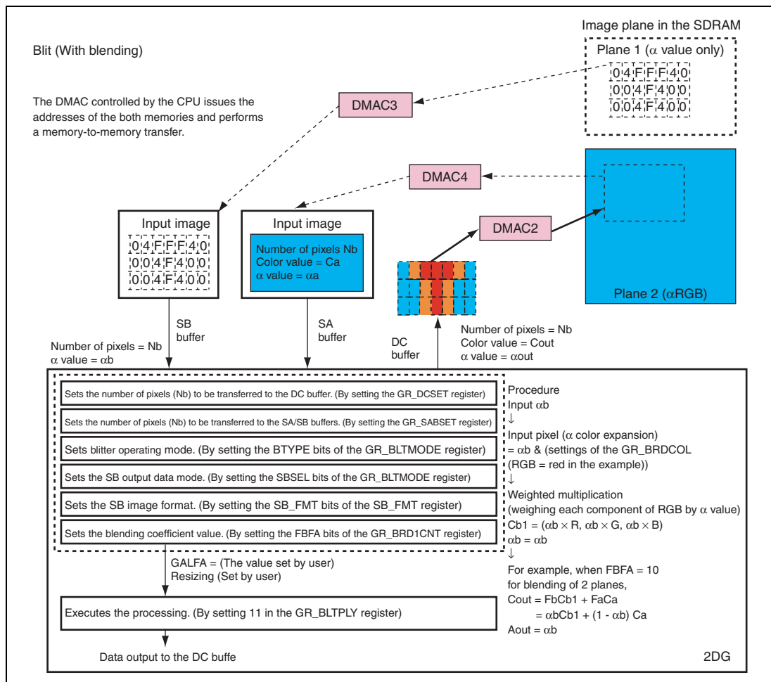
Figure 26.32 Example of Color Gradation Processing (2)
