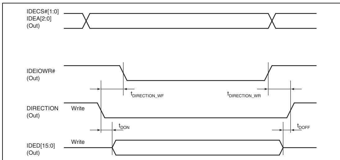
Figure 33.75 PIO Data Transfer to Device (DIRECTION)
