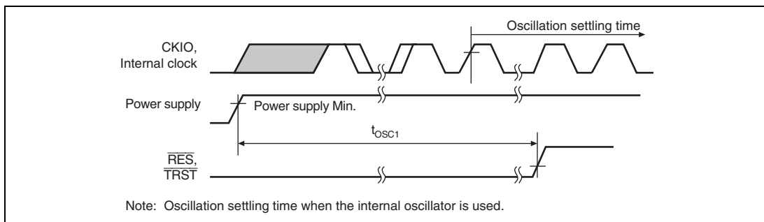
Figure 33.5 Power-On Oscillation Settling Time
