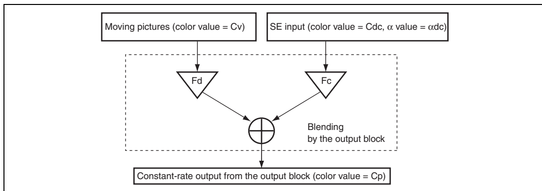
Figure 26.55 Summary of Output Block Operations during Blending
