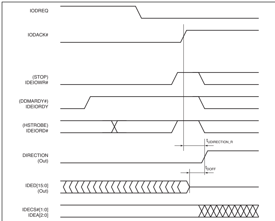
Figure 33.83 Device Terminating Ultra DMA Data-Out Burst (DIRECTION)
