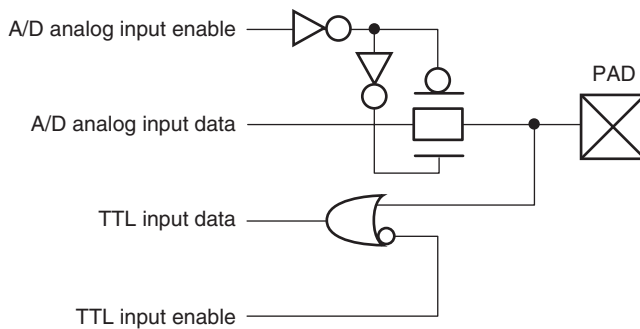
Figure 1.3 (4) Simplified Circuit Diagram (TTL OR Input and A/D Input Buffer)
