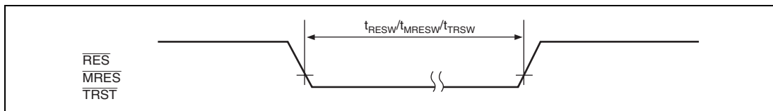
Figure 33.9 Reset Input Timing
