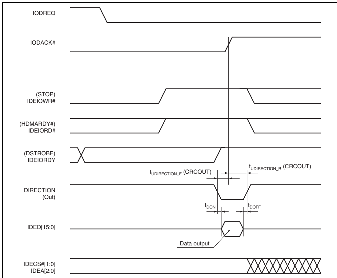
Figure 33.79 Device Terminating Ultra DMA Data-In Burst (DIRECTION)
