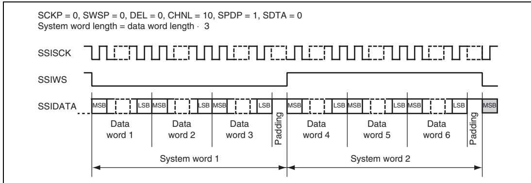
Figure 19.8 Multi-Channel Format (6 Channels with High Padding)
