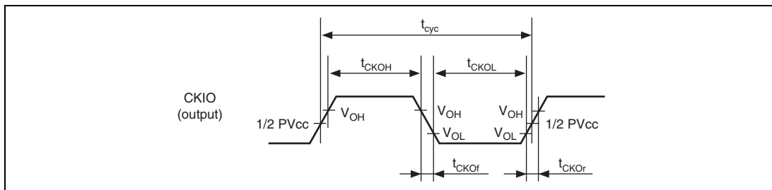
Figure 33.4 CKIO Clock Output Timing
