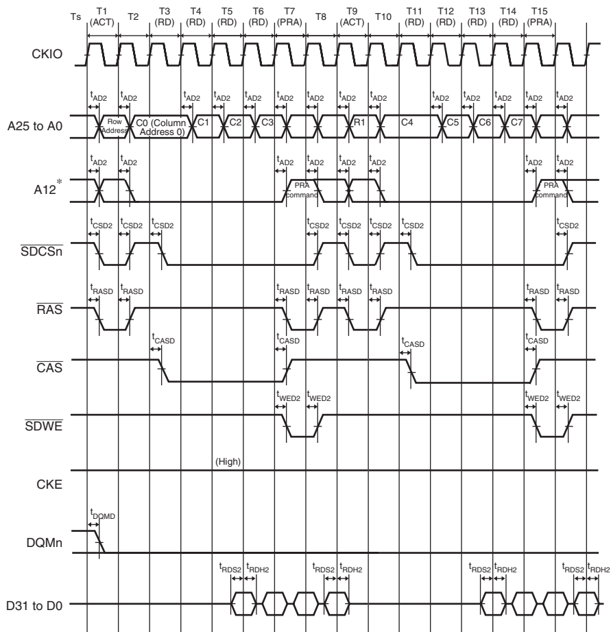
Figure 33.20 SDRAM Space: Bus Timing of Multiple-Read Across Rows (8 Data Accesses, DCL = 2 (2 Cycles), DRCD = 1 (2 Cycles), DPCG = 1 (2 Cycles))
