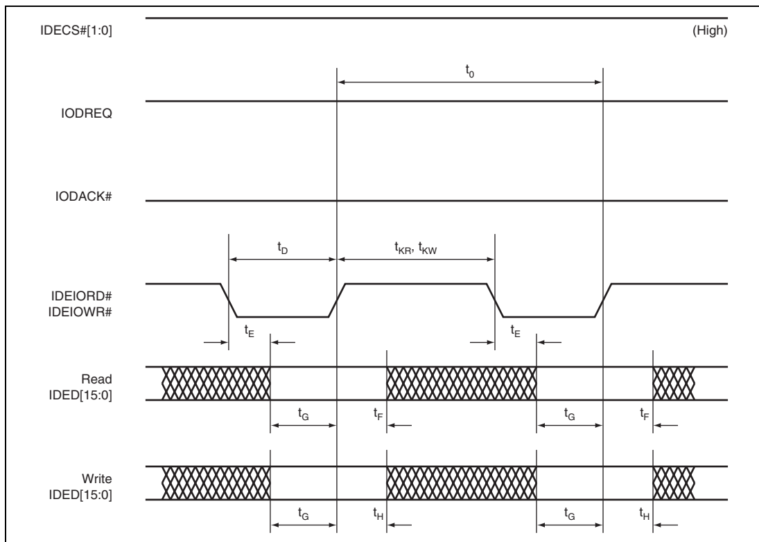
Figure 33.62 Sustaining Multiword DMA Data Burst
