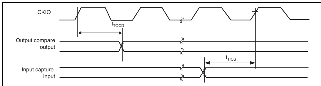
Figure 33.26 MTU2 Input/Output Timing
