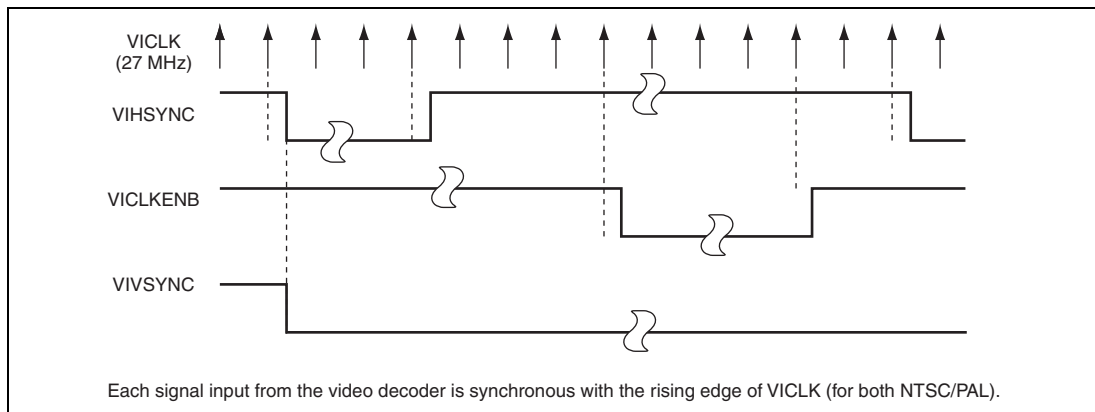
Figure 26.7 Relations between Externally Input Sync Signal and VICLK
