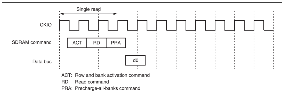
Figure 10.20 Single Read Timing Example (Shortest Timing Settings)
