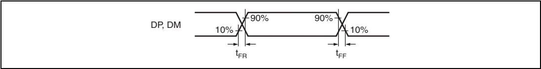
Figure 33.56 DP and DM Output Timing (Full-Speed)
