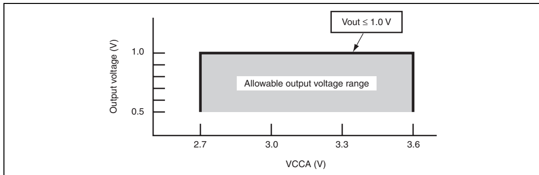
Figure 26.60 Allowable Analog Ouput Voltage Range
