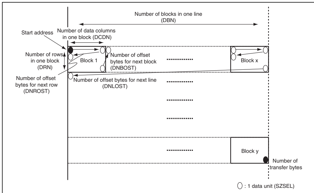
Figure 11.2 Specifying Two-Dimensional Blocks
