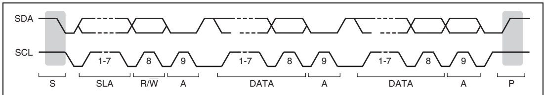
Figure 18.4 I 2 C Bus Timing
