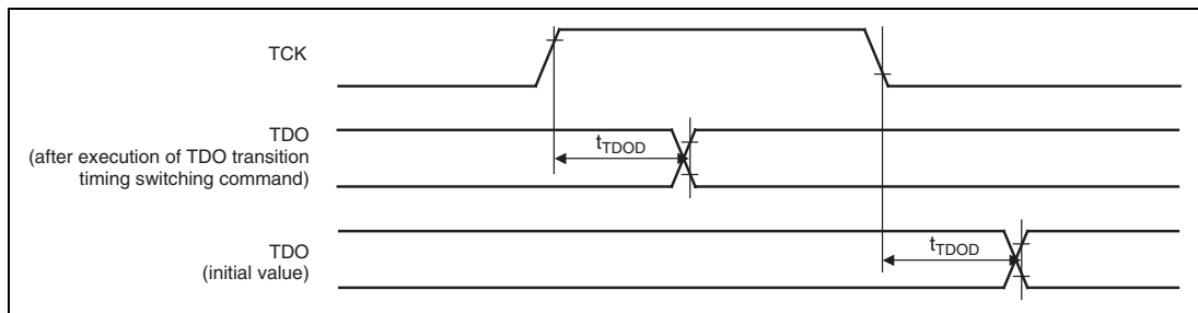
Figure 31.3 H-UDI Data Transfer Timing
