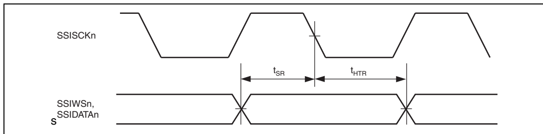
Figure 33.40 SSIF Receive Timing (2)
