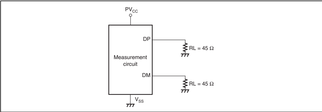
Figure 33.59 Measurement Circuit (High-Speed)
