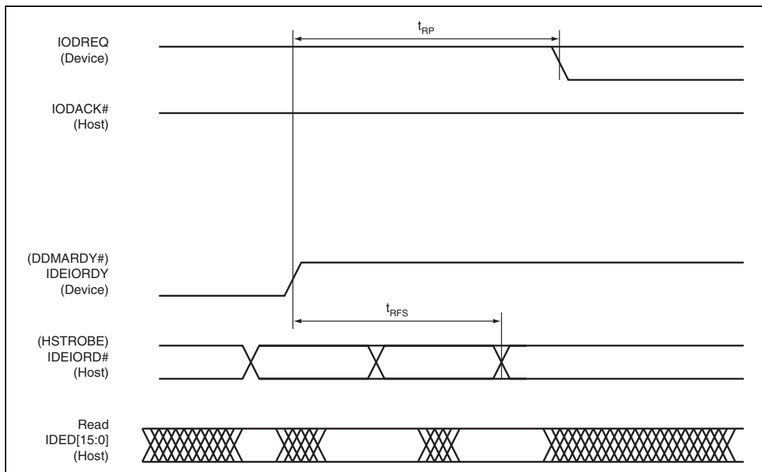
Figure 33.72 Device Pausing Ultra DMA Data-Out Burst
