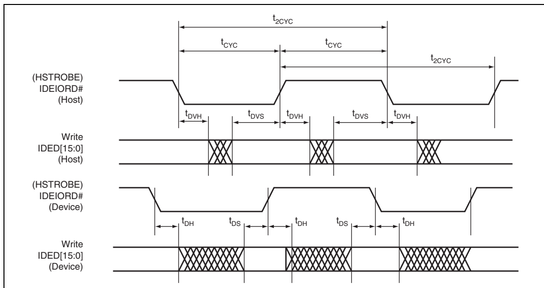
Figure 33.71 Sustained Ultra DMA Data-Out Burst
