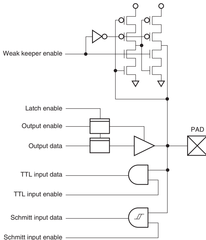
Figure 1.3 (14) Simplified Circuit Diagram (Bidirectional Buffer, TTL AND Input, Schmitt AND Input, with Latch and Weak Keeper)
