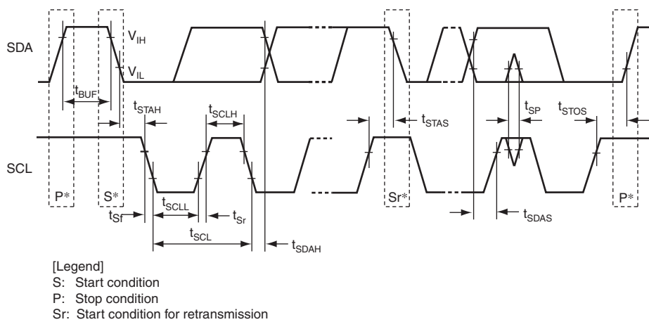
Figure 33.35 (1) IIC3 Input/Output Timing
