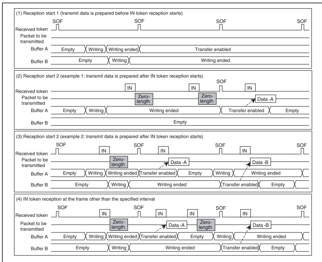
Figure 24.14 Example of Data Setup Function Operation
