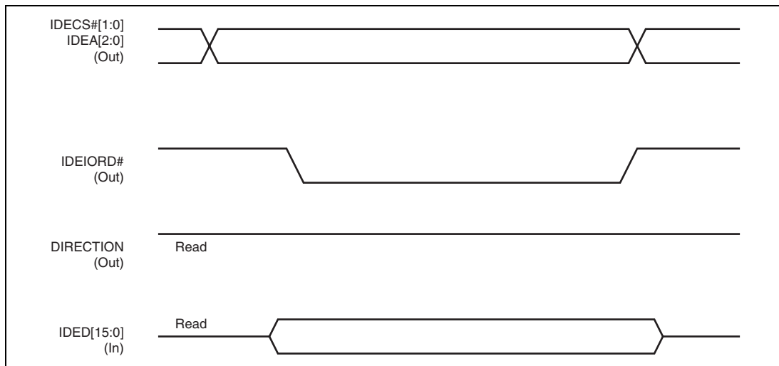
Figure 33.76 PIO Data Transfer from Device (DIRECTION)
