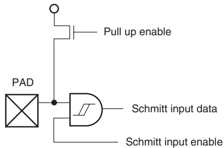
Figure 1.3 (2) Simplified Circuit Diagram (Schmitt AND Input Buffer with Pull-Up)
