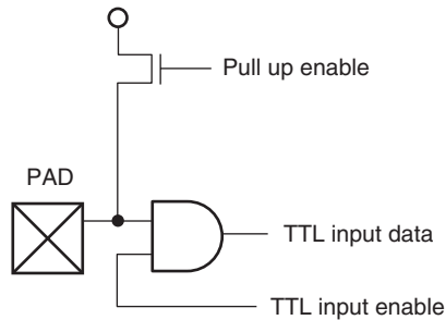
Figure 1.3 (3) Simplified Circuit Diagram (TTL AND Input Buffer with Pull-Up)
