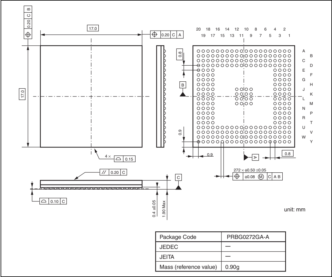
Figure C.1 Package Dimensions
