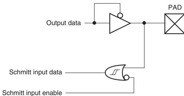
Figure 1.3 (15) Simplified Circuit Diagram (Open Drain Output and Schmitt OR Input Buffer)
