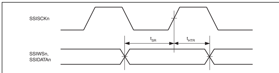
Figure 33.39 SSIF Receive Timing (1)
