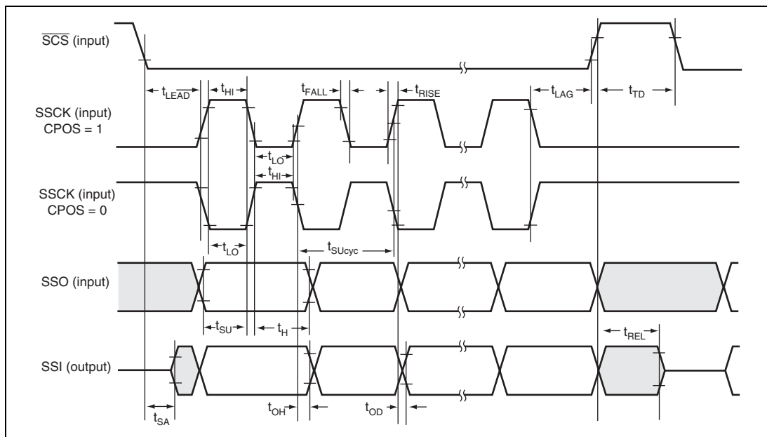
Figure 33.34 SSU Timing (Slave, CPHS = 0)
