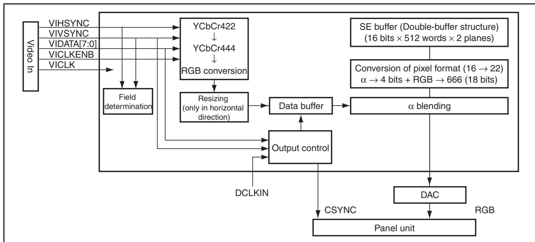
Figure 26.3 Block Diagram of the Output Block
