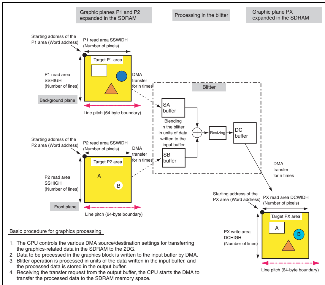
Figure 26.20 Summary of Blitter Operations
