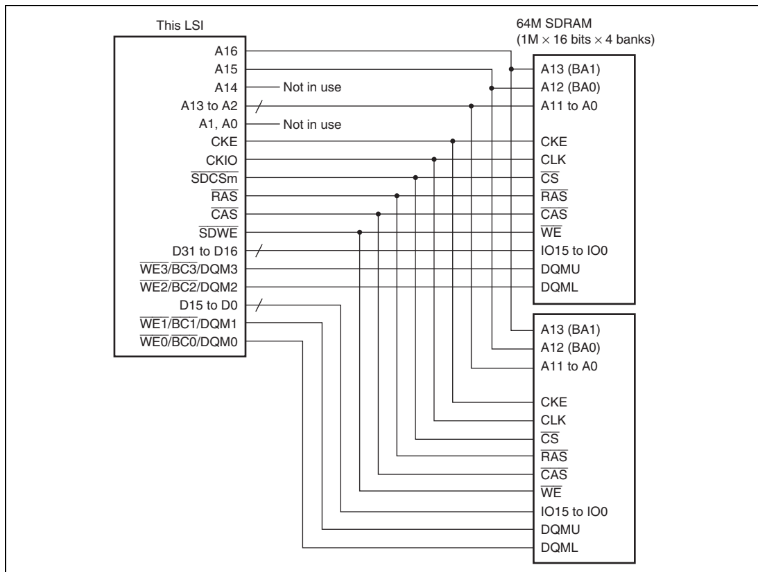
Figure 10.46 Example of Connecting a 32-Bit Data-Width SDRAM
