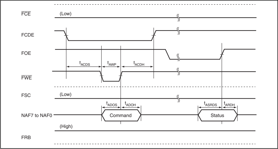
Figure 33.48 AND Type Flash Memory Status Read Timing
