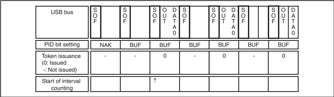
Figure 24.2 Whether a Token is Issued or Not when IITV = 1
