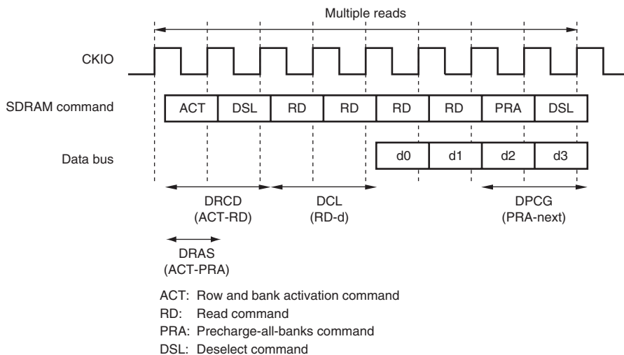
Figure 10.30 Multiple Read Timing Example 2
