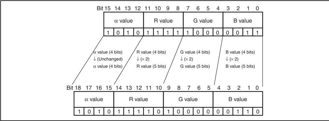
Figure 26.17 Pixel Format Conversion 1 in Blitter
