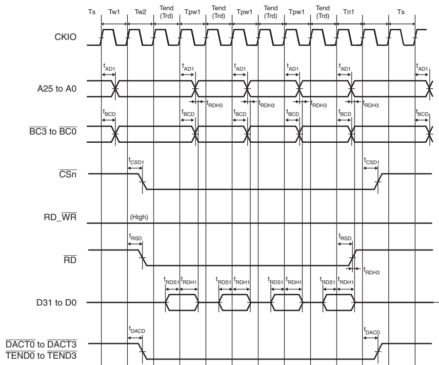
Figure 33.13 External Address Space: Basic Bus Timing
