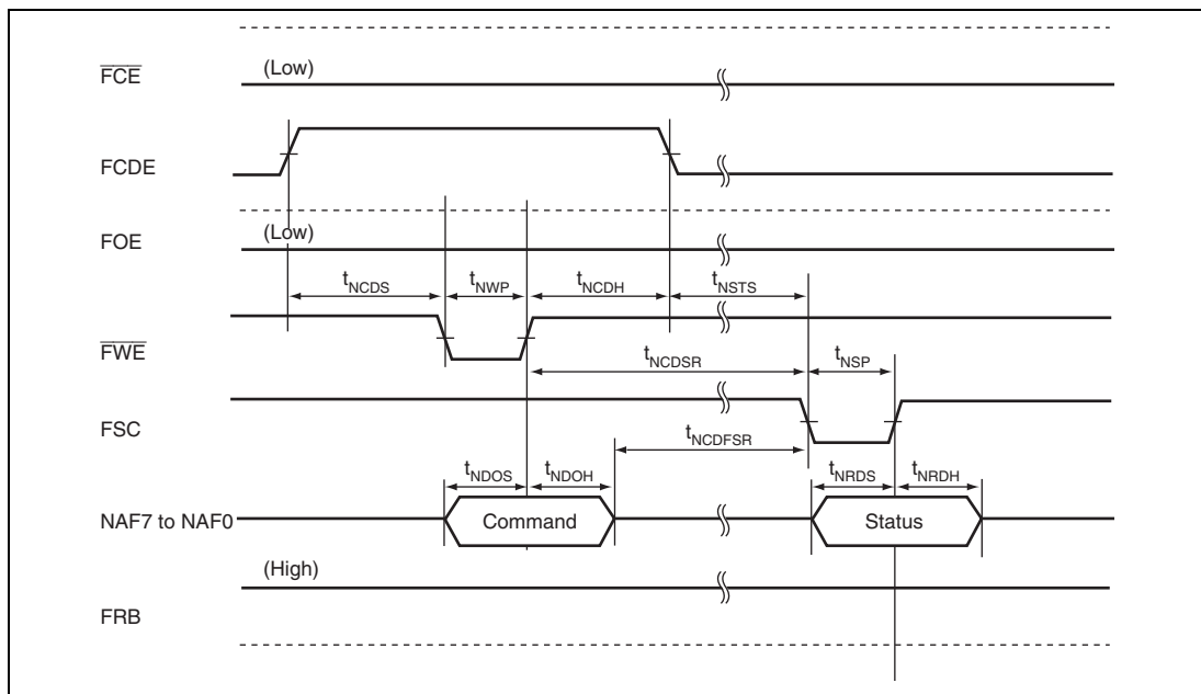
Figure 33.53 NAND Type Flash Memory Status Read Timing
