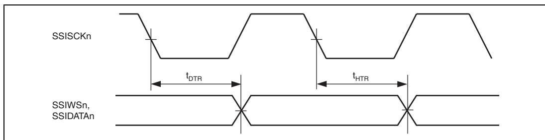
Figure 33.38 SSIF Transmit Timing (2)
