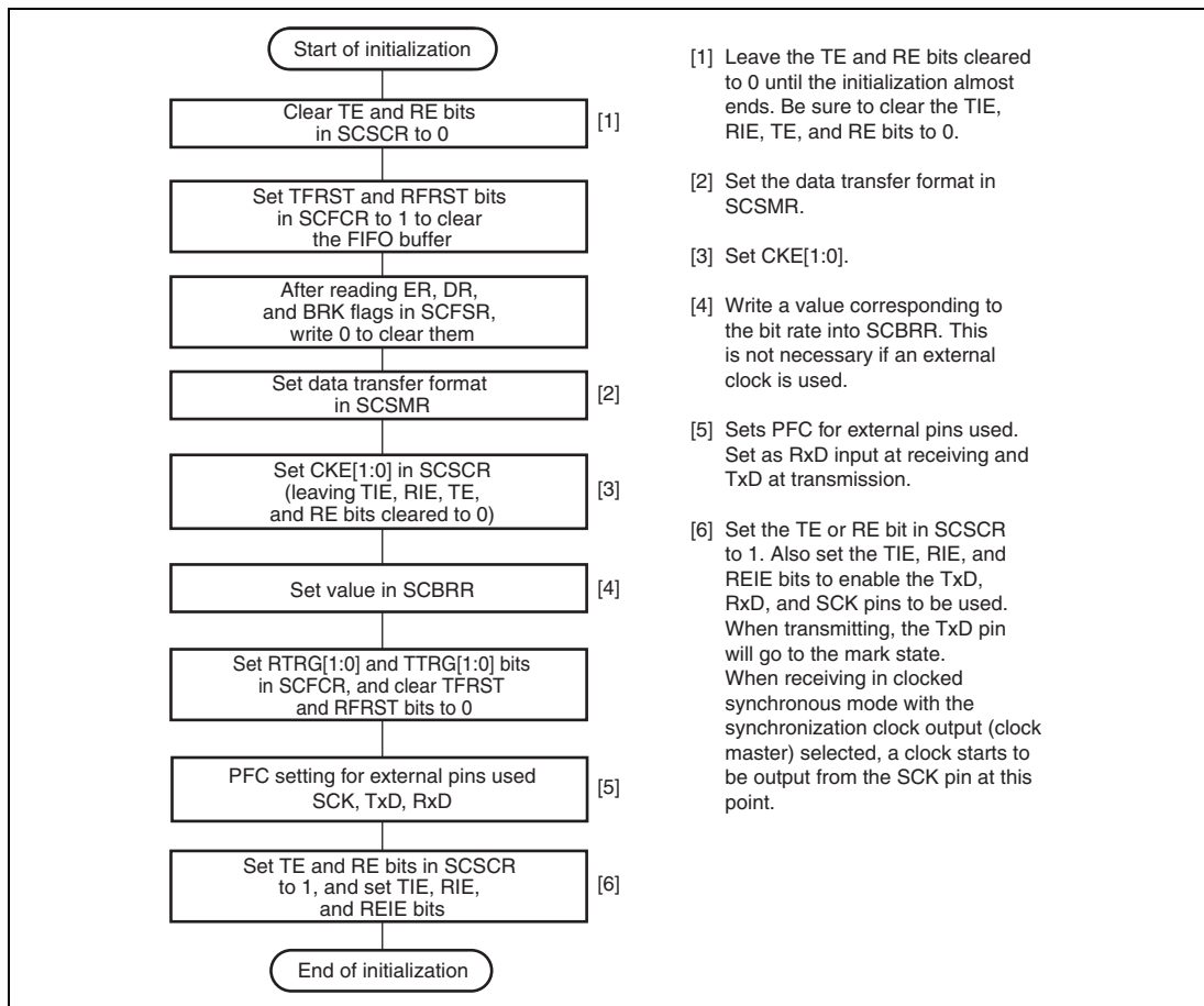
Figure 16.12 Sample Flowchart for SCIF Initialization
