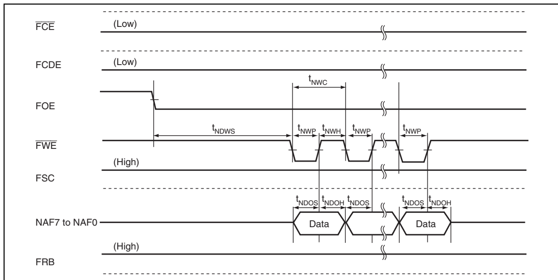
Figure 33.52 NAND Type Flash Memory Data Write Timing
