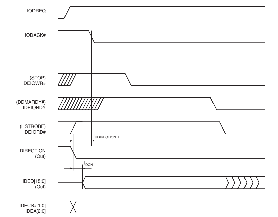
Figure 33.81 Initiating Ultra DMA Data-Out Burst (DIRECTION)
