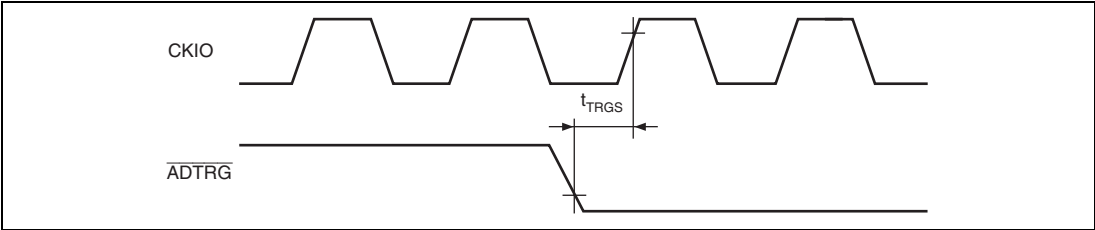
Figure 33.43 A/D Converter External Trigger Input Timing
