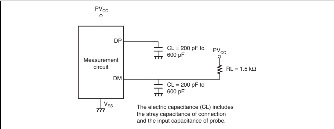
Figure 33.55 Measurement Circuit (Low-Speed)
