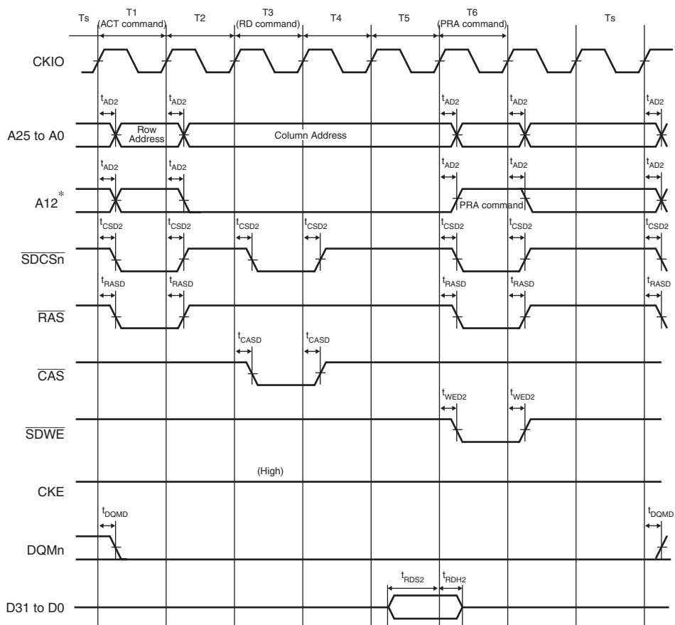
Figure 33.16 SDRAM Space: Single-Read Bus Timing (DCL = 2 (2 Cycles), DRCD = 1 (2 Cycles), DPCG = 1 (2 Cycles))
