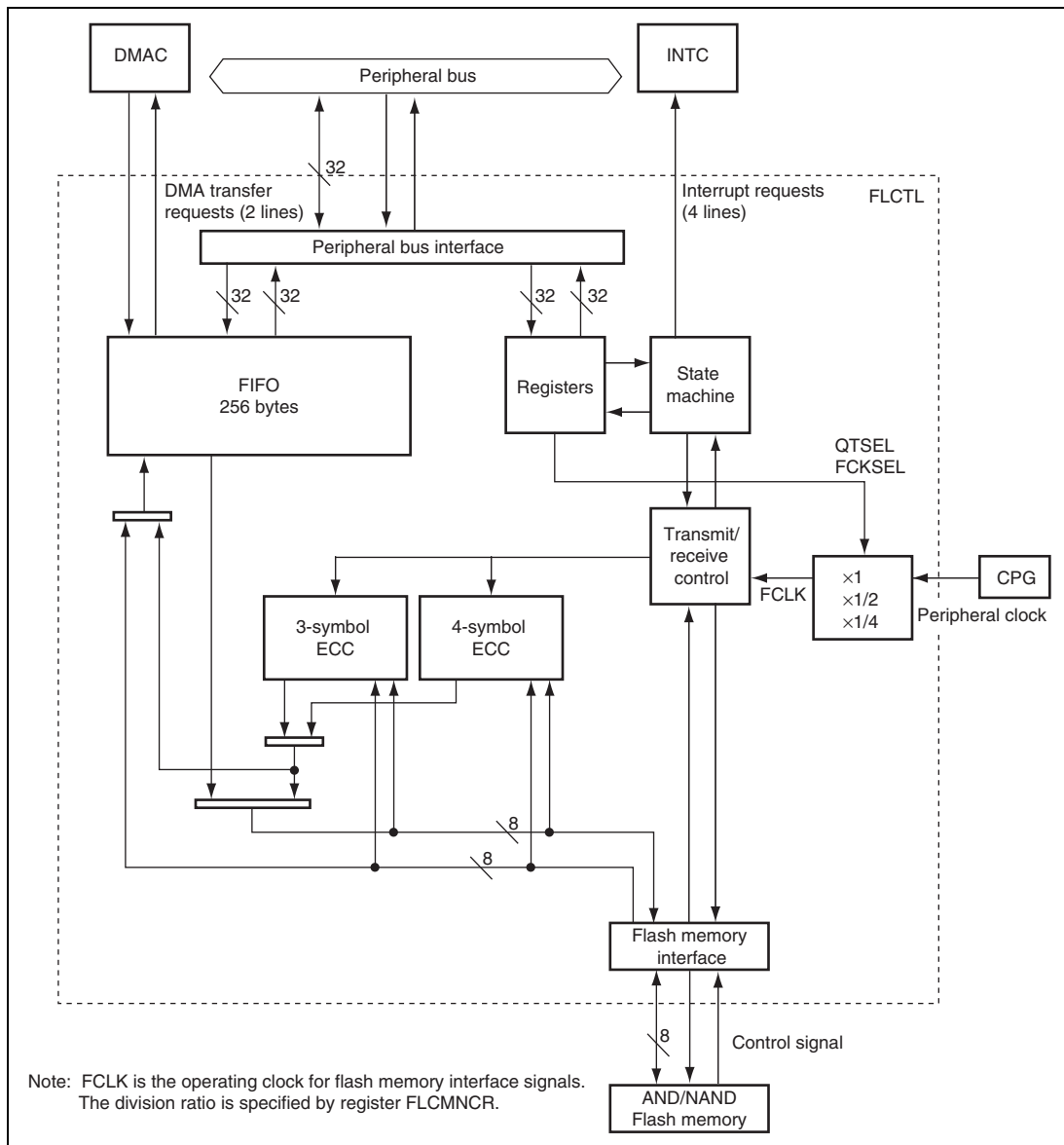
Figure 23.1 FLCTL Block Diagram
