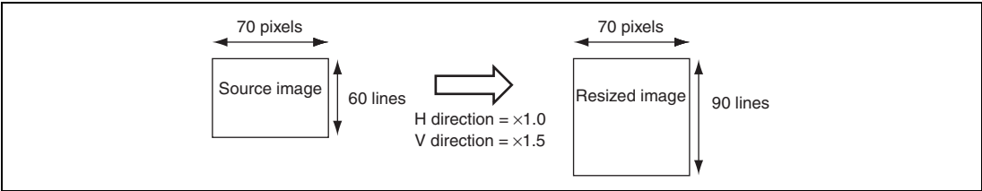
Figure 26.45 Example of Duplicate-line Setting of Enlargement Resizing (1)
