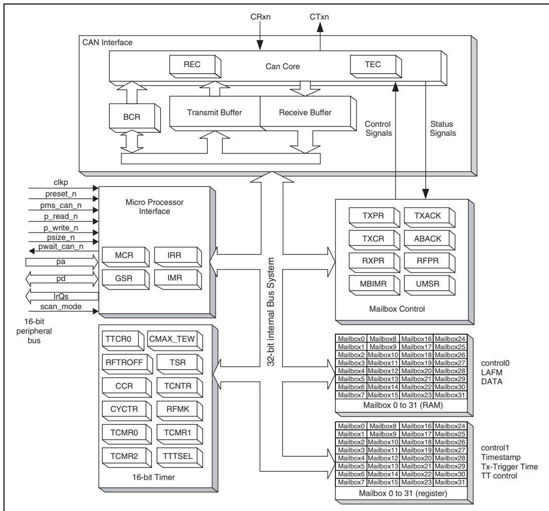
Figure 20.1 RCAN-TL1 architecture
