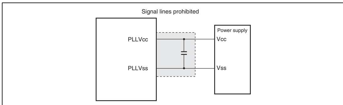
Figure 5.5 Note on Using a PLL Oscillation Circuit
