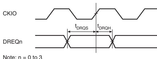
Figure 33.24 DREQ Input Timing
