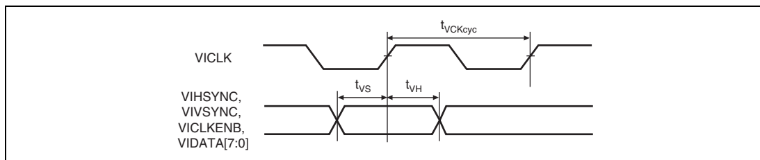
Figure 33.84 Video Input Timing
