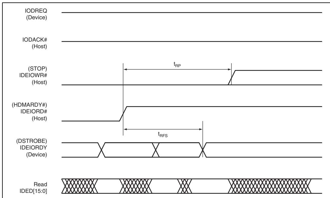
Figure 33.67 Host Pausing Ultra DMA Data-In Burst
