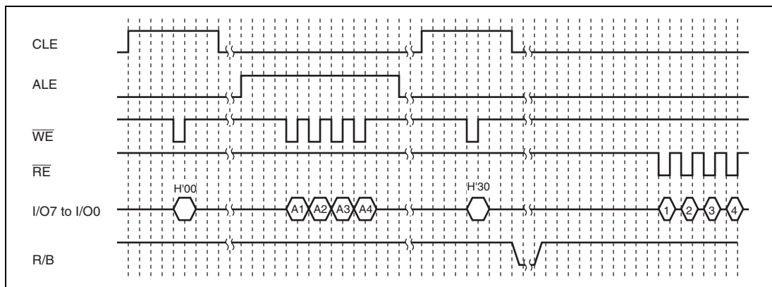
Figure 23.11 Read Operation Timing for NAND-Type Flash Memory
