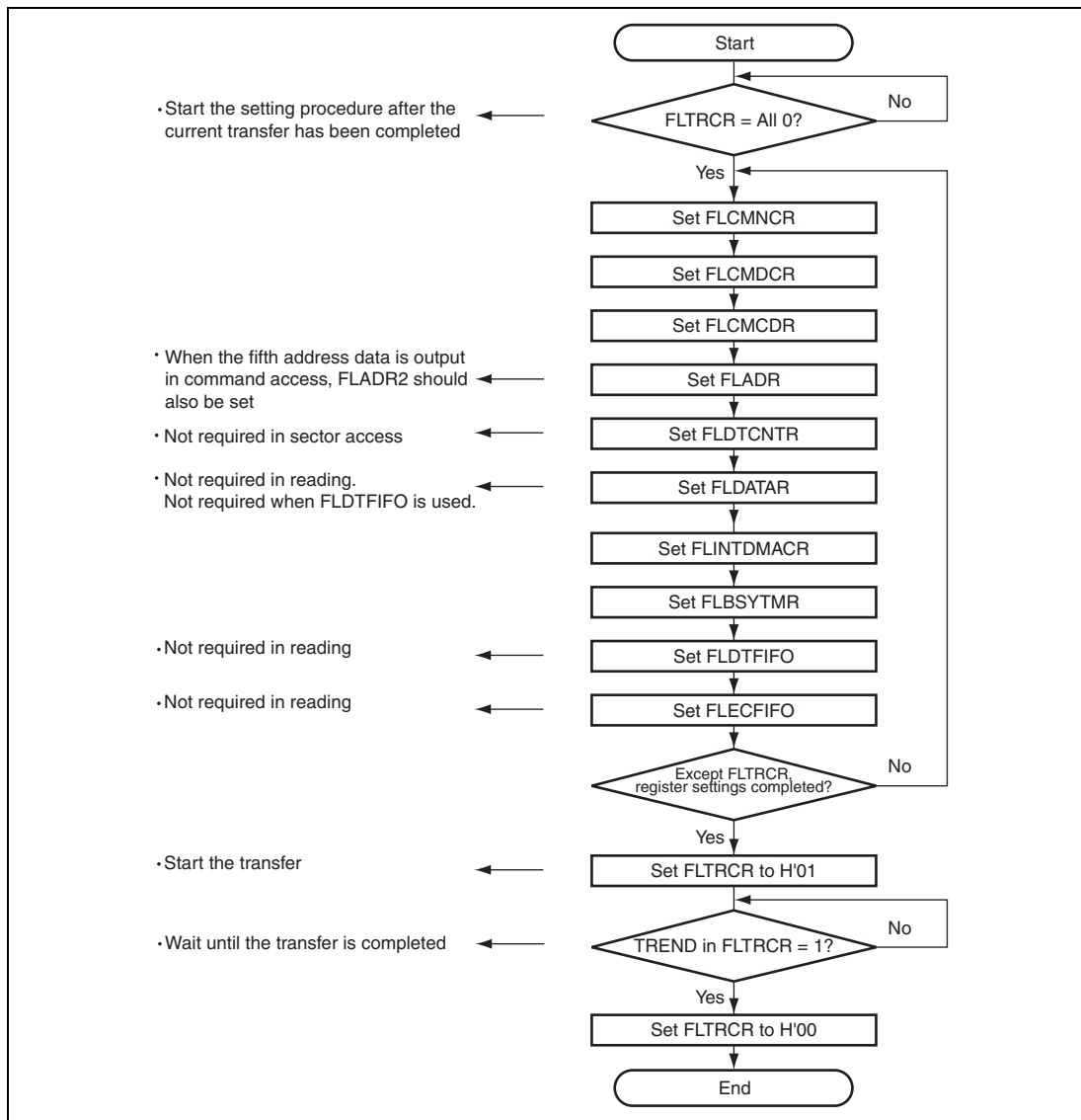
Figure 23.3 Register Setting Flow
