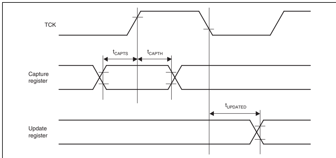
Figure 33.90 Boundary Scan Input/Output Timing
