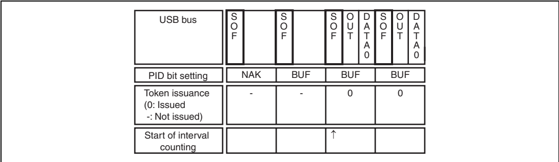
Figure 24.1 Whether a Token is Issued or Not when IITV = 0
