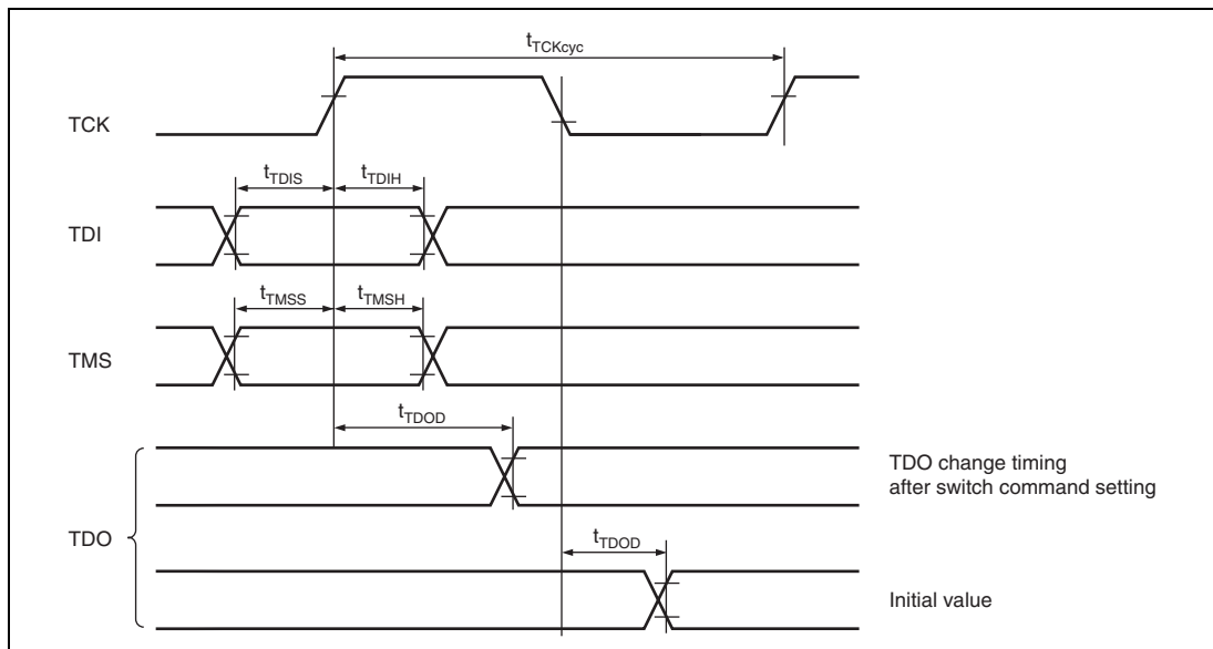
Figure 33.89 H-UDI Data Transfer Timing
