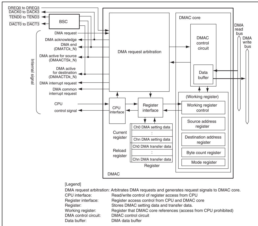
Figure 11.1 DMAC Block Diagram
