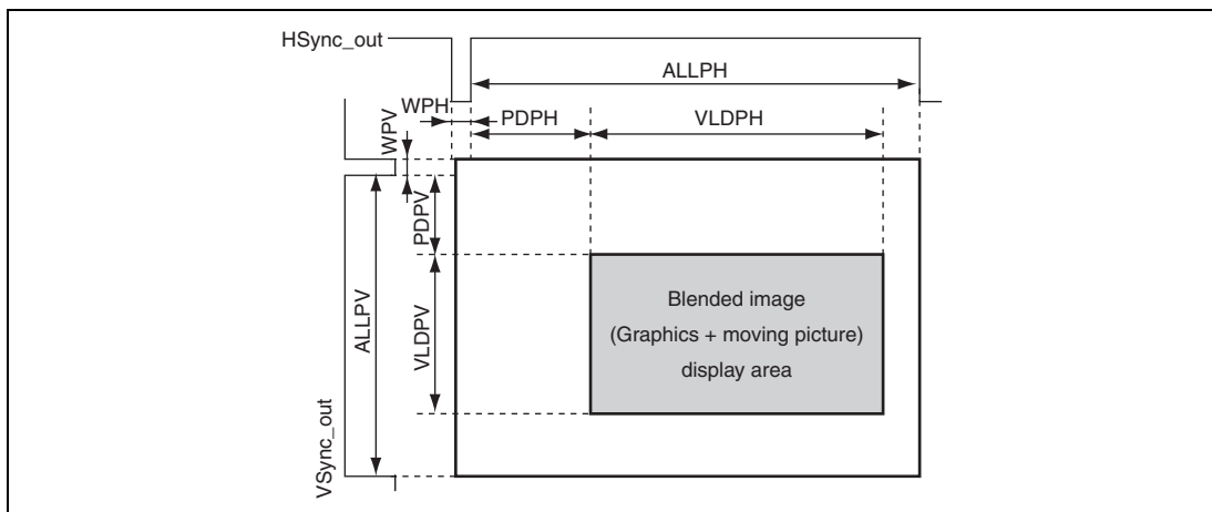
Figure 26.6 Relationship between Panel Output and Register Settings
