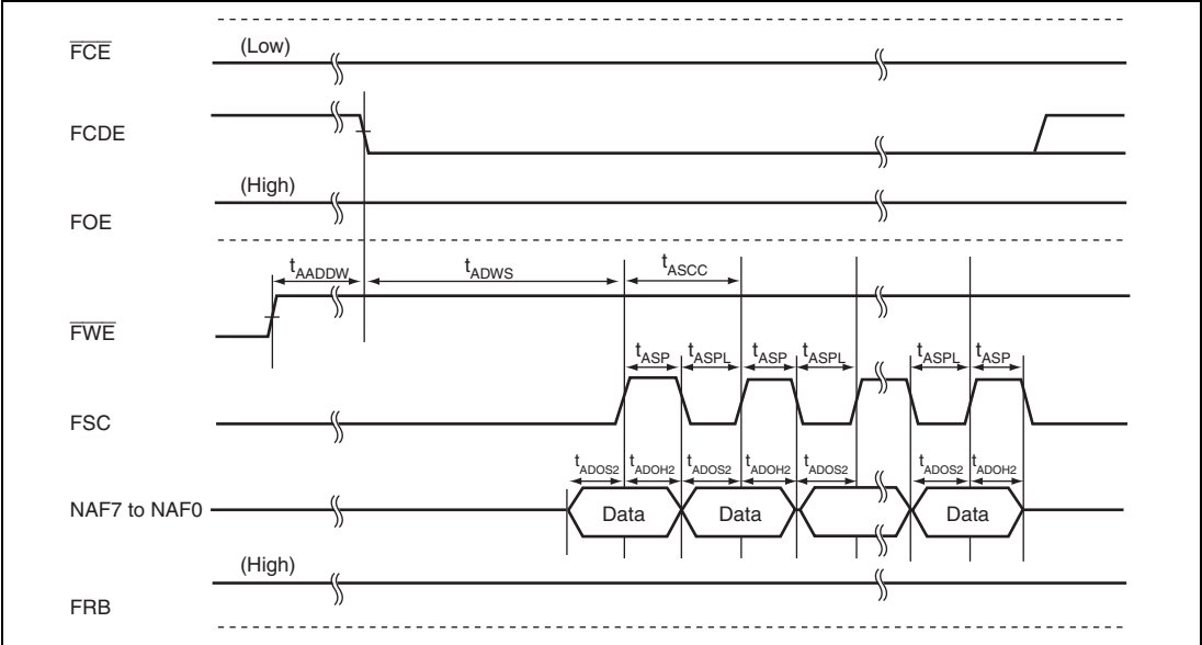
Figure 33.47 AND Type Flash Memory Data Write Timing
