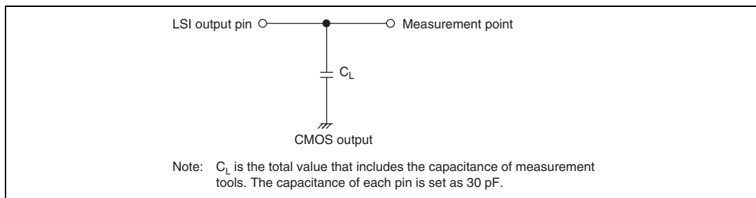
Figure 33.91 Output Load Circuit
