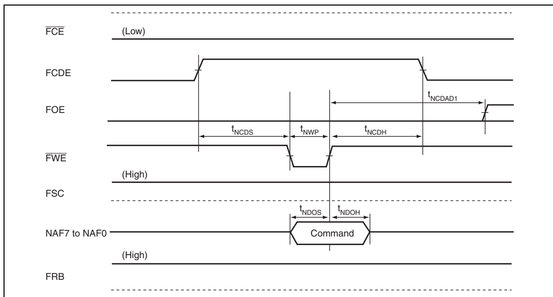
Figure 33.49 NAND Type Flash Memory Command Issuance Timing
