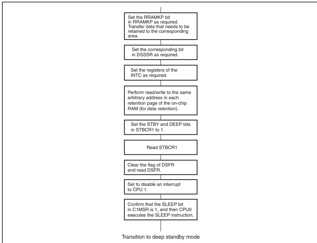
Figure 30.3 Flowchart of Transition to Deep Standby Mode
