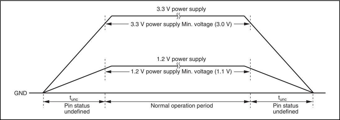
Figure 35.1 Power-on/Power-off Sequence
