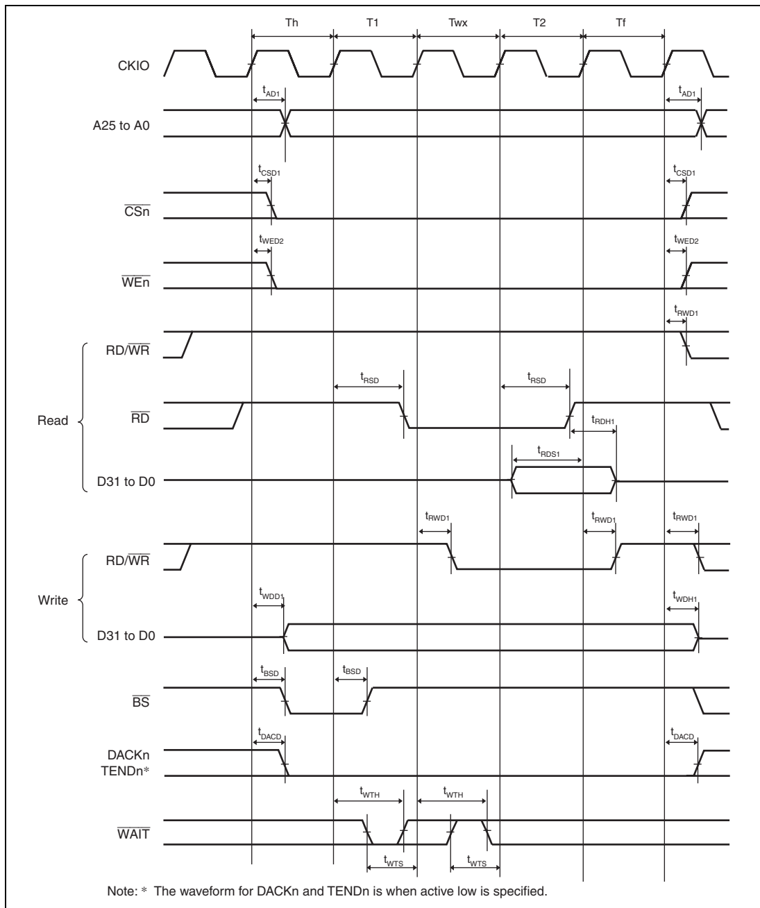
Figure 35.20 Bus Cycle of SRAM with Byte Selection (SW = 1 Cycle, HW = 1 Cycle, One Asynchronous External Wait Cycle, BAS = 1 (Write Cycle WE Control))
