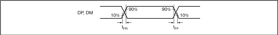
Figure 35.74 DP and DM Output Timing (Full-Speed)
