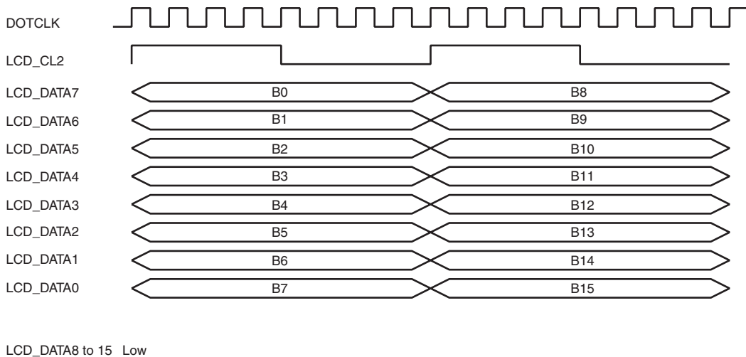
Figure 26.12 Clock and LCD Data Signal Example (STN Monochrome 8-Bit Data Bus Module)
