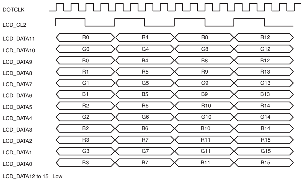
Figure 26.15 Clock and LCD Data Signal Example (STN Color 12-Bit Data Bus Module)
