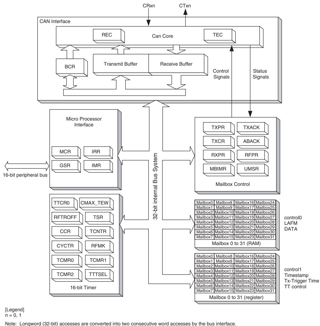
Figure 19.1 RCAN-TL1 architecture
