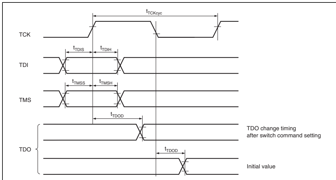
Figure 35.82 H-UDI Data Transfer Timing
