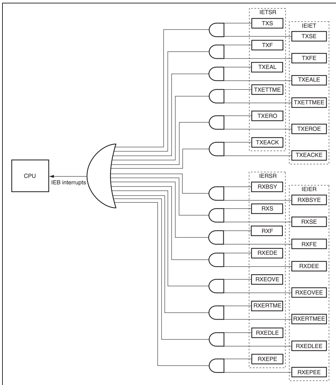
Figure 20.17 Relations between IEB Interrupt Sources
