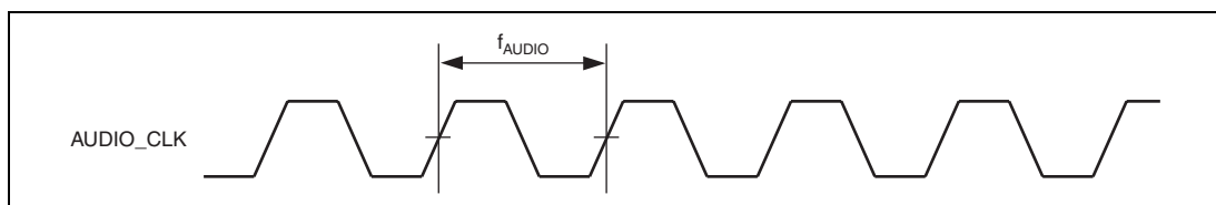
Figure 35.61 AUDIO_CLK Input Timing
