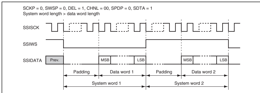
Figure 18.6 MSB-first and Right-Aligned Format (Transmitted and received in the order of padding bits and serial data)
