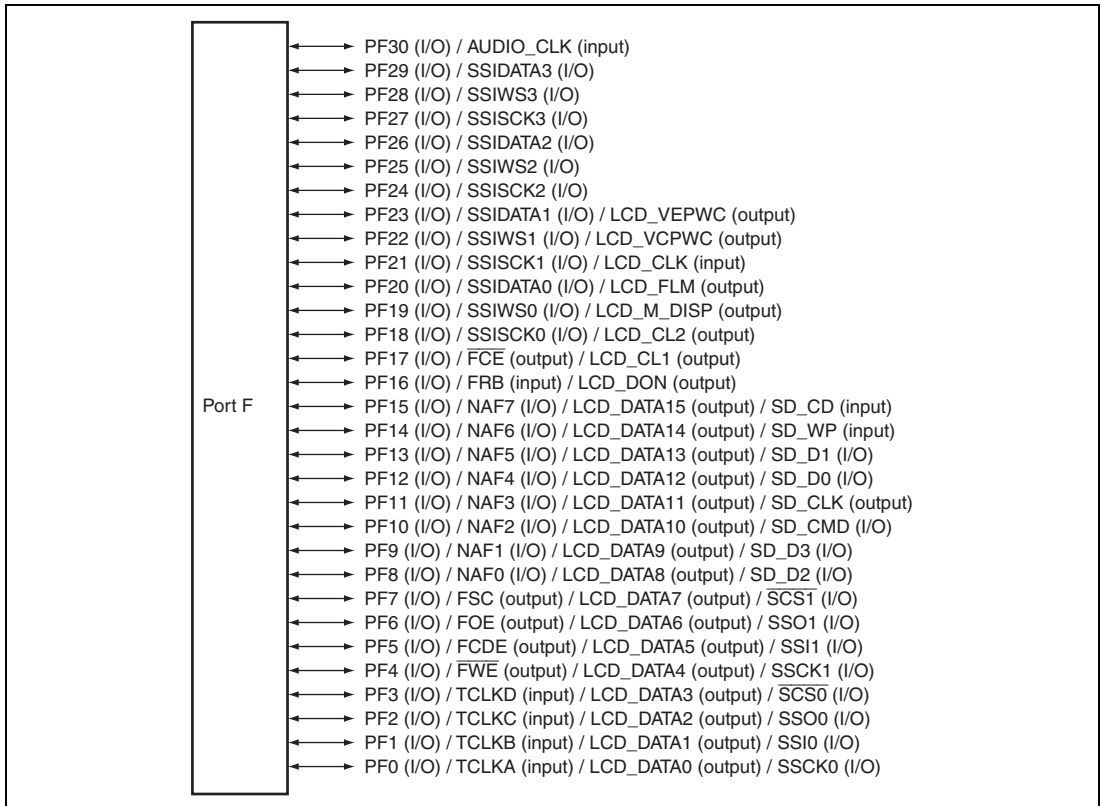
Figure 30.6 Port F
