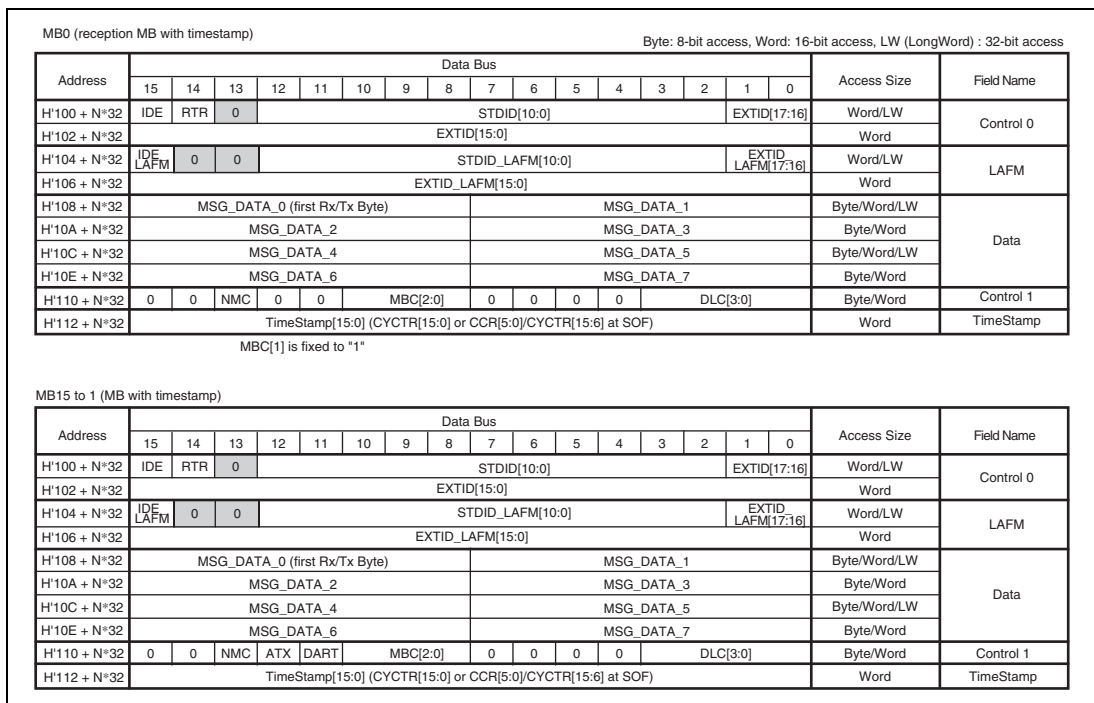
Figure 19.3 Mailbox-N Structure
