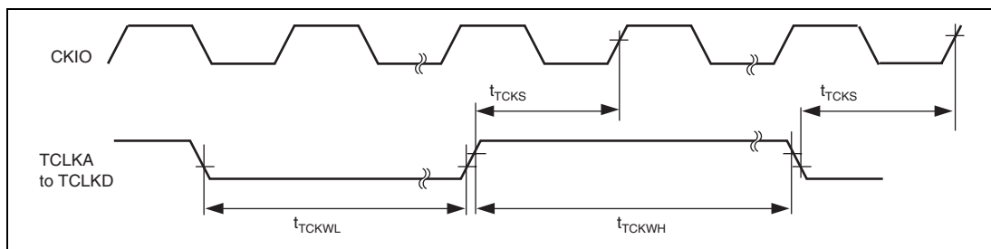
Figure 35.49 MTU2 Clock Input Timing
