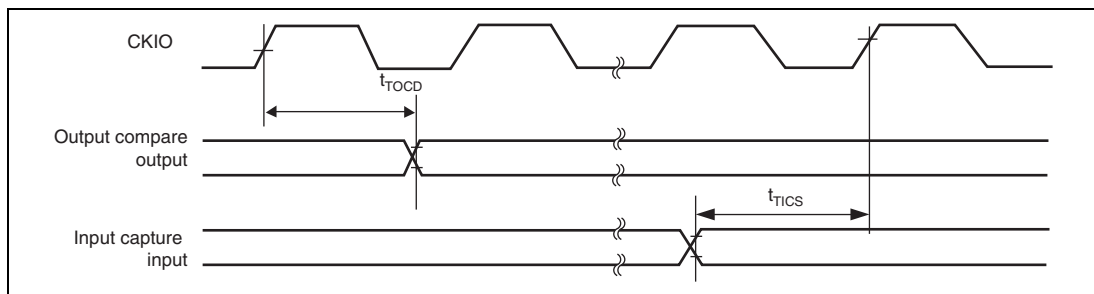
Figure 35.48 MTU2 Input/Output Timing
