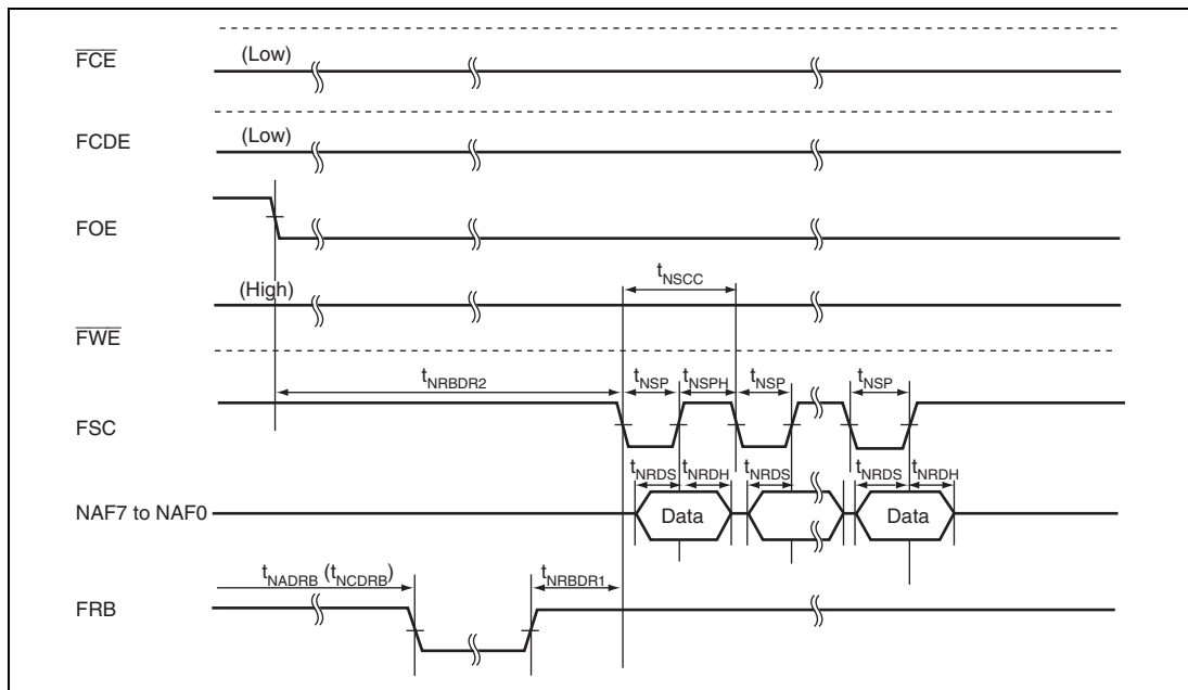
Figure 35.71 NAND Type Flash Memory Data Read Timing
