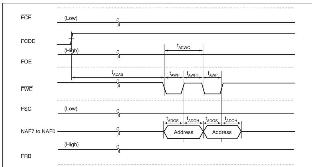
Figure 35.65 AND Type Flash Memory Address Issuance Timing
