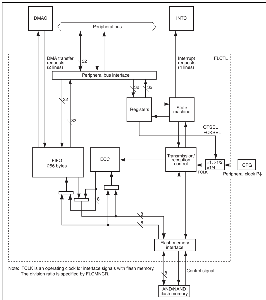
Figure 24.1 FLCTL Block Diagram
