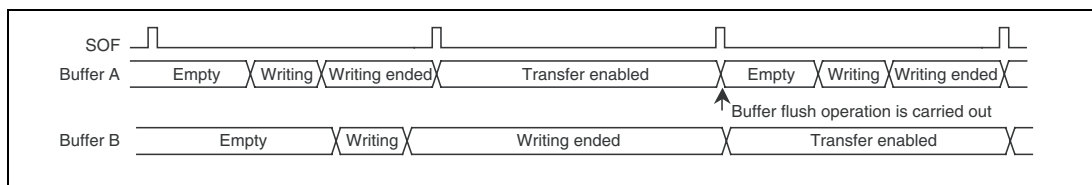
Figure 25.18 Example of Buffer Flush Function Operation
