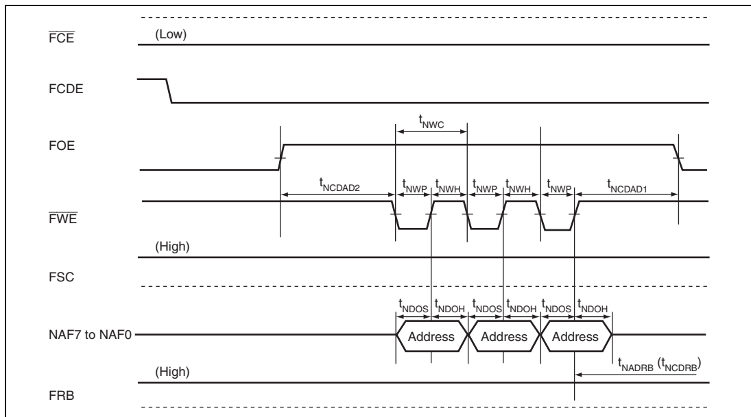
Figure 35.70 NAND Type Flash Memory Address Issuance Timing
