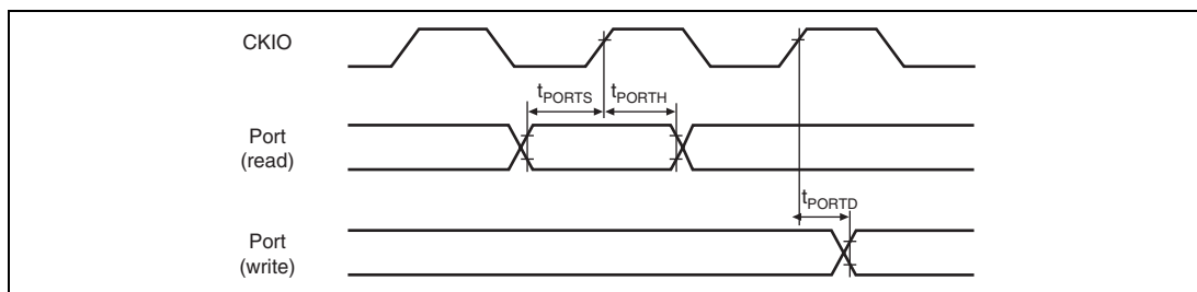
Figure 35.80 I/O Port Timing
