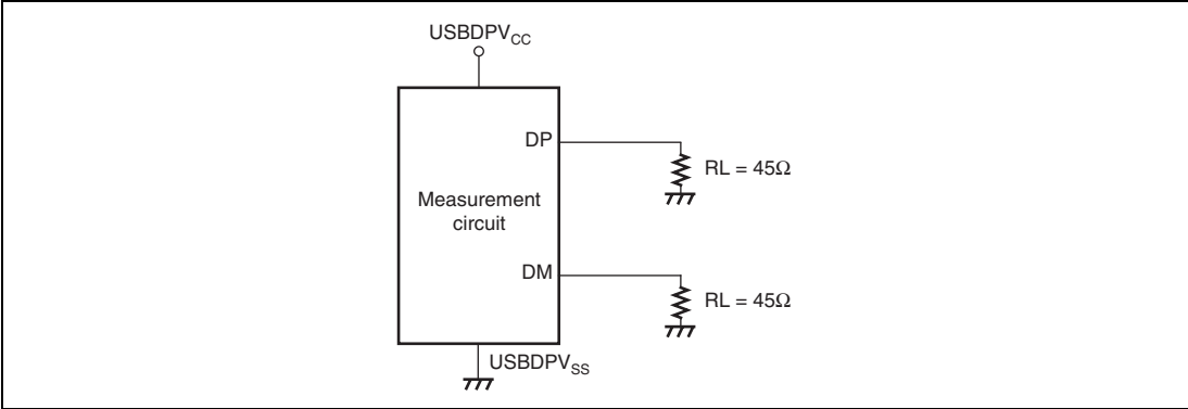
Figure 35.77 Measurement Circuit (High-Speed)
