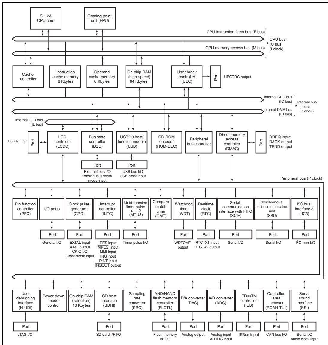
Figure 1.1 Block Diagram
