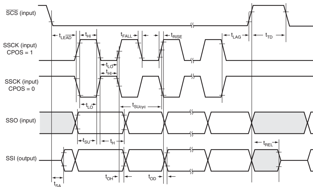
Figure 35.56 SSU Timing (Slave, CPHS = 0)
