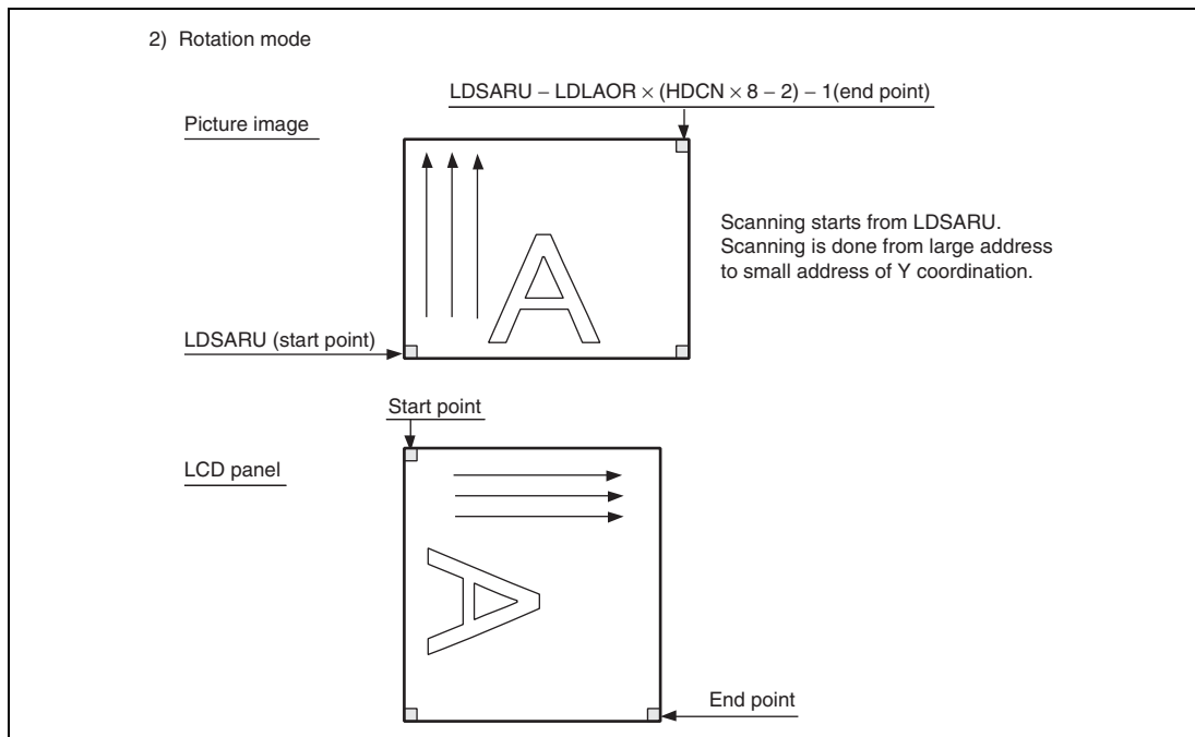
Figure 26.10 Operation for Hardware Rotation (Rotation Mode)
