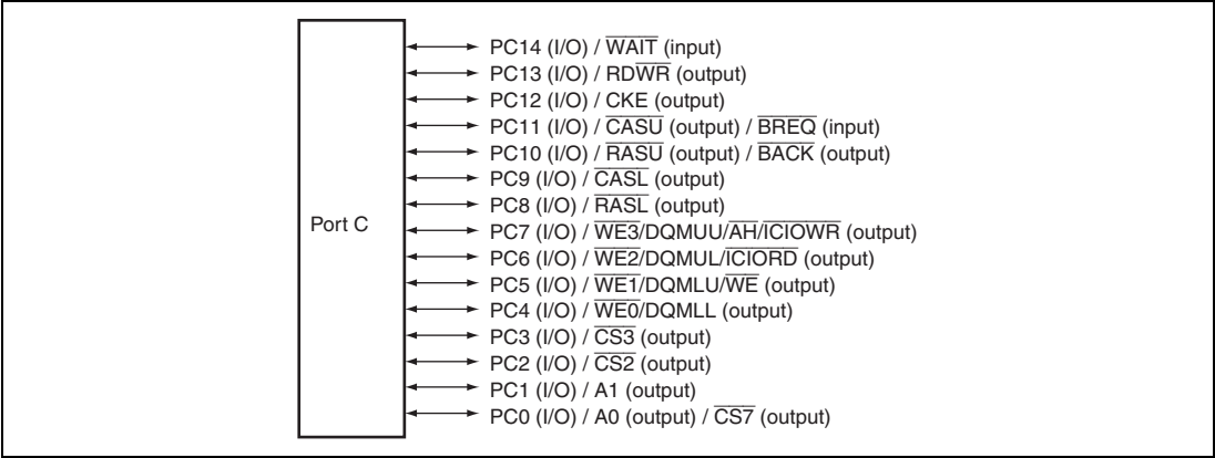
Figure 30.3 Port C
