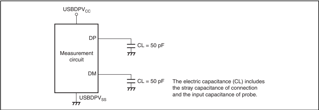
Figure 35.75 Measurement Circuit (Full-Speed)
