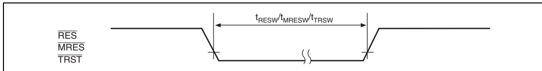
Figure 35.9 Reset Input Timing
