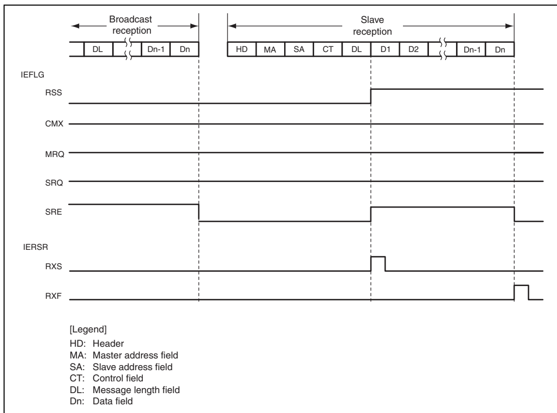
Figure 20.14 Slave Receive Operation Timing
