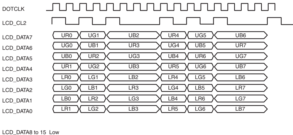
Figure 26.19 Clock and LCD Data Signal Example (DSTN Color 8-Bit Data Bus Module)
