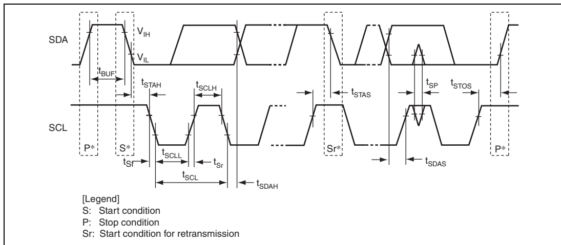
Figure 35.57 (1) IIC3 Input/Output Timing
