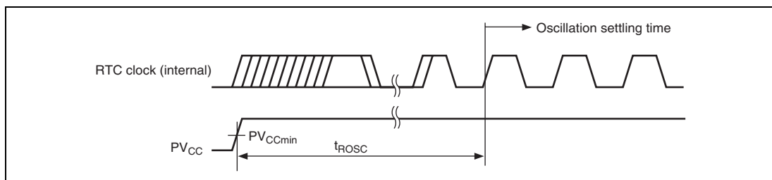
Figure 35.8 RTC Clock Oscillation Settling Time
