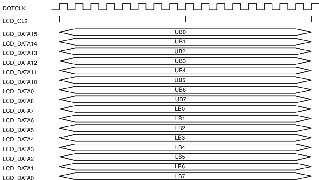
Figure 26.18 Clock and LCD Data Signal Example (DSTN Monochrome 16-Bit Data Bus Module)
