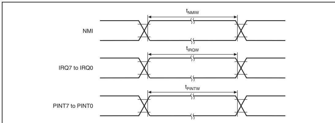
Figure 35.10 Interrupt Signal Input Timing
