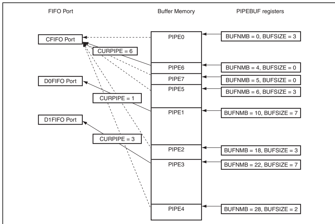
Figure 25.9 Example of a Buffer Memory Map
