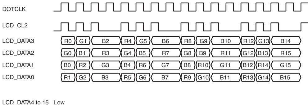
Figure 26.13 Clock and LCD Data Signal Example (STN Color 4-Bit Data Bus Module)
