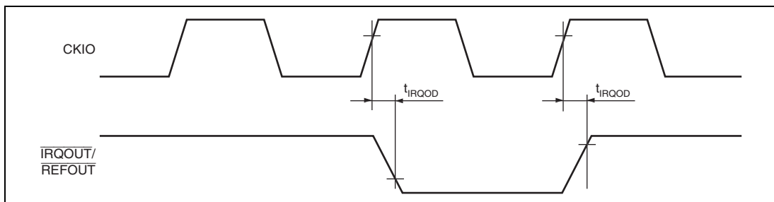
Figure 35.11 Interrupt Signal Output Timing
