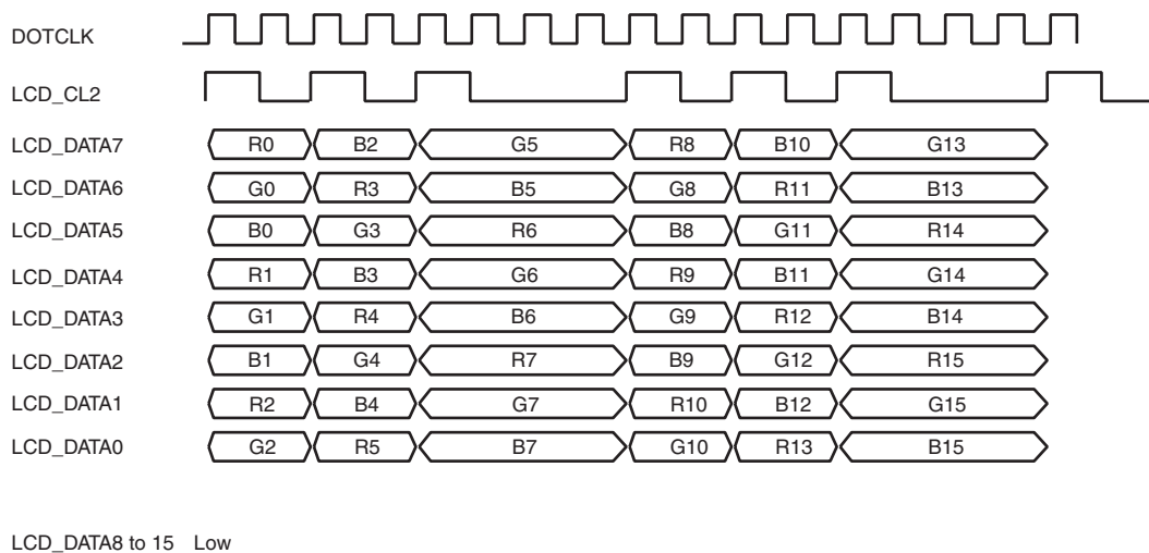
Figure 26.14 Clock and LCD Data Signal Example (STN Color 8-Bit Data Bus Module)
