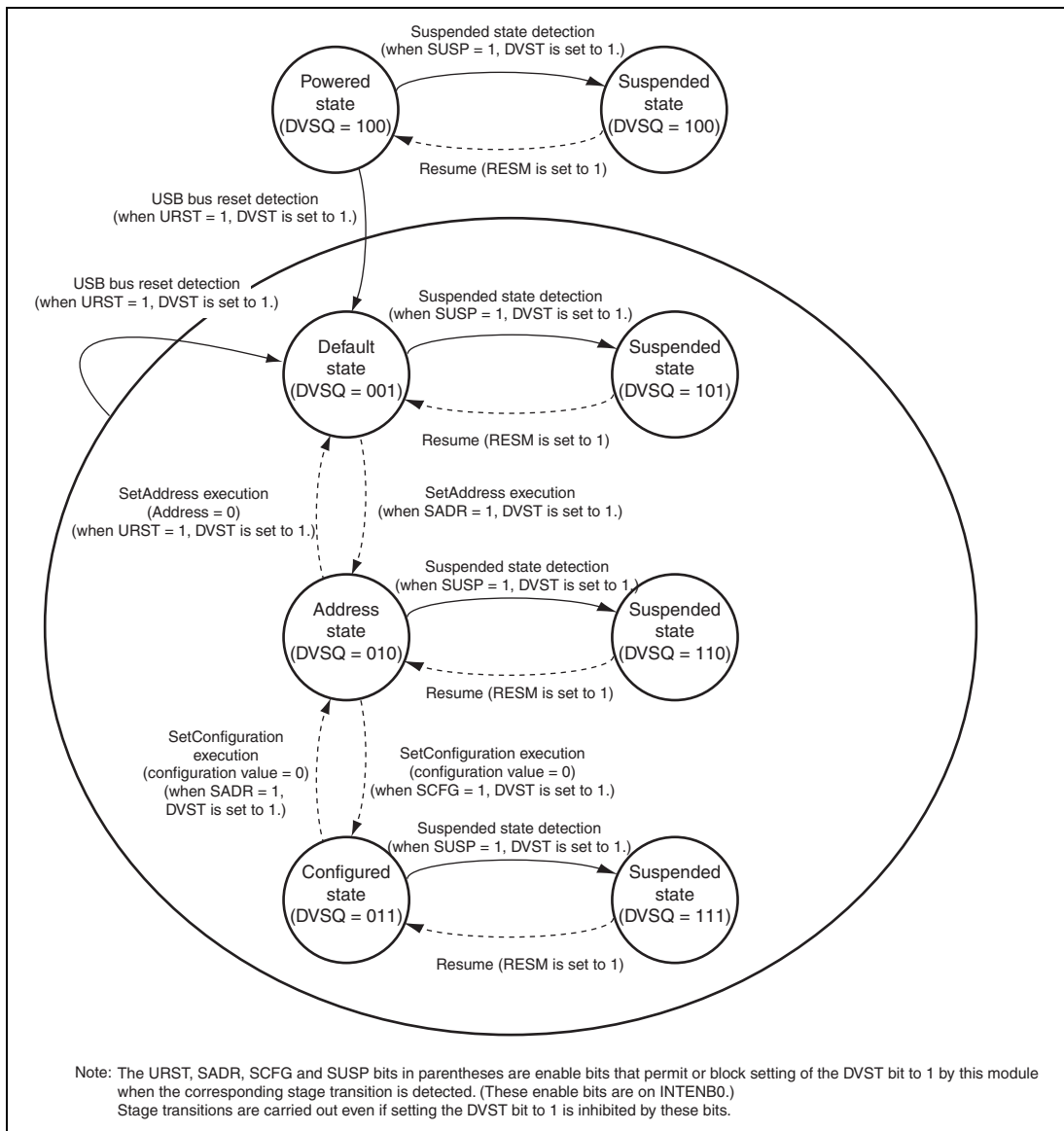
Figure 25.6 Device State Transitions
