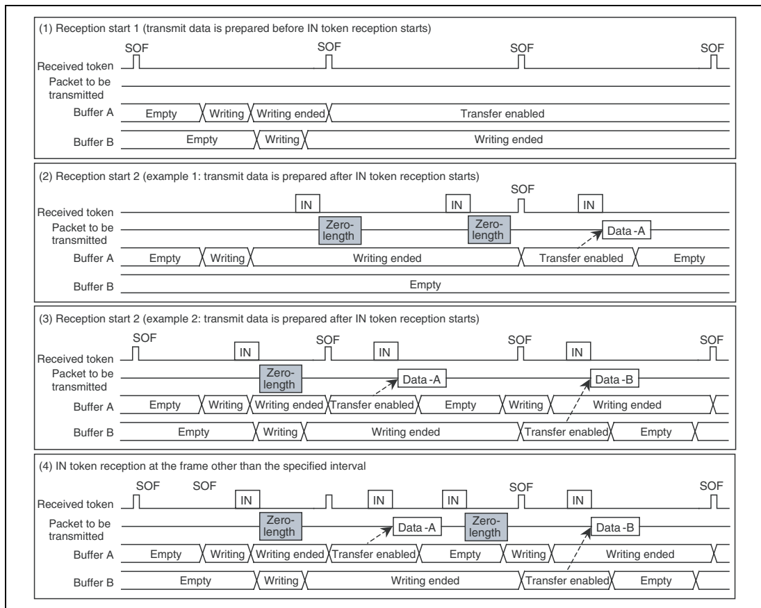
Figure 25.17 Example of Data Setup Function Operation
