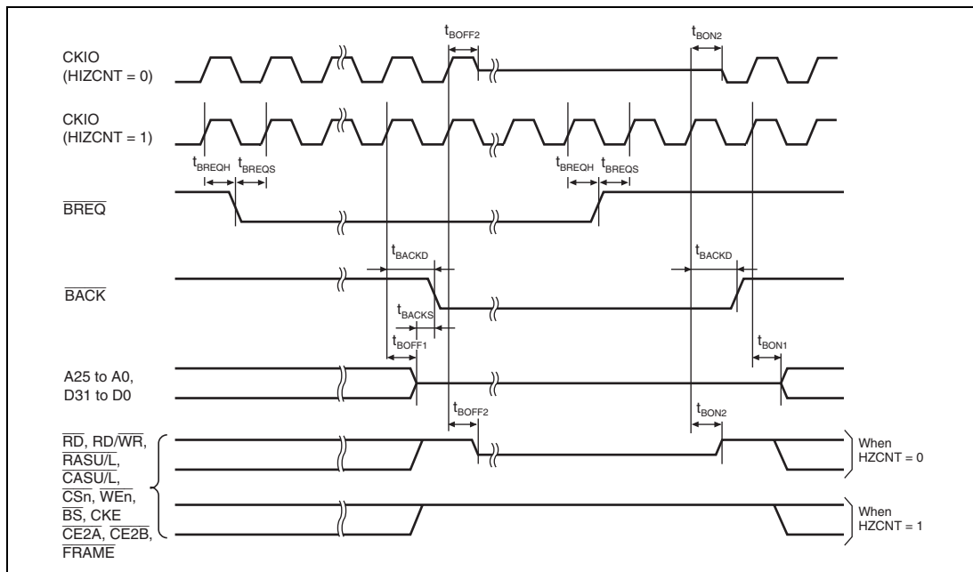
Figure 35.12 Bus Release Timing
