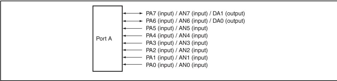
Figure 30.1 Port A
