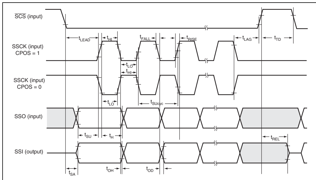
Figure 35.55 SSU Timing (Slave, CPHS = 1)
