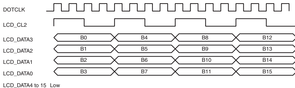
Figure 26.11 Clock and LCD Data Signal Example (STN Monochrome 4-Bit Data Bus Module)
