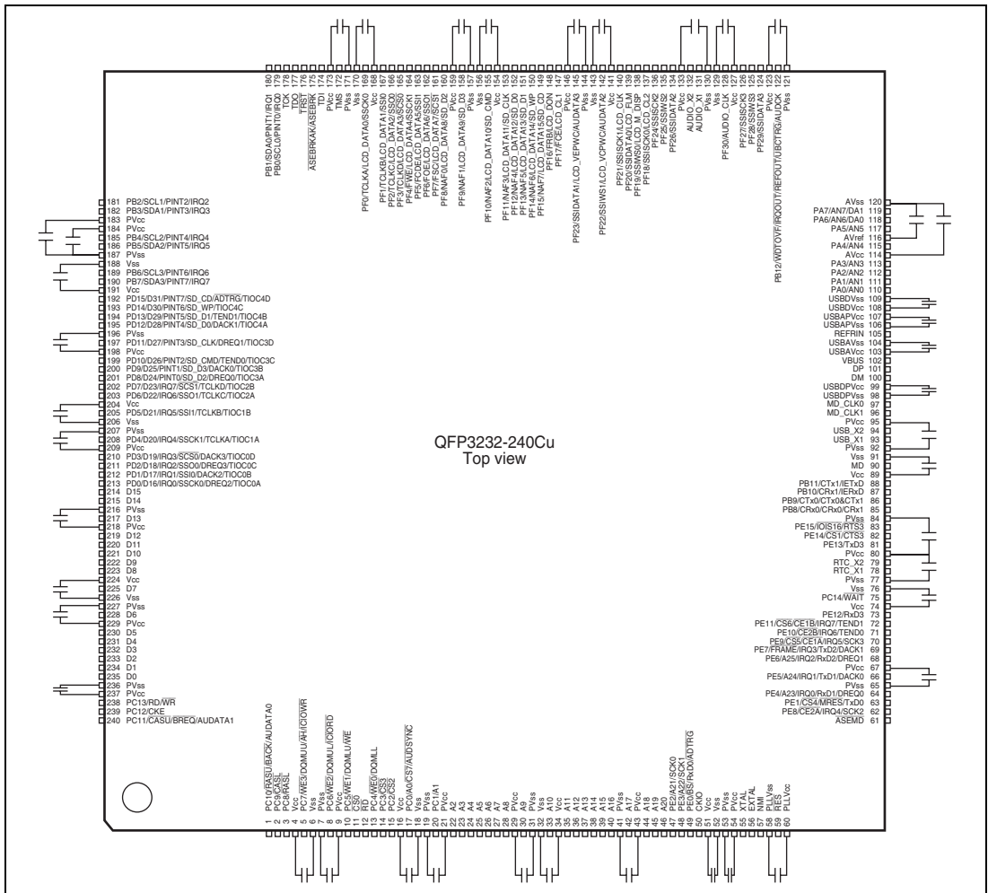
Figure 35.84 Example of Externally Allocated Capacitors
