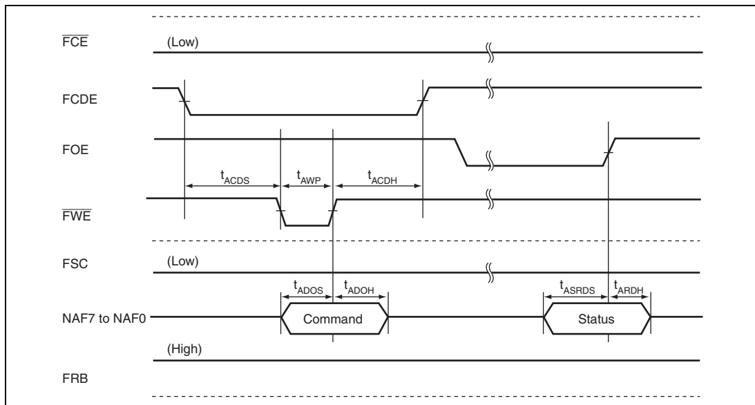
Figure 35.68 AND Type Flash Memory Status Read Timing
