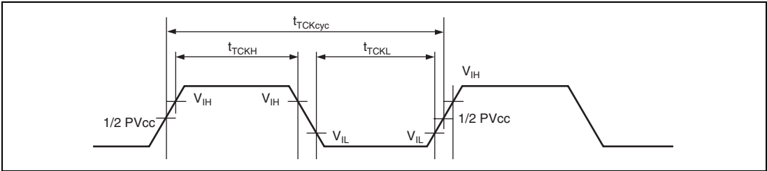
Figure 35.81 TCK Input Timing
