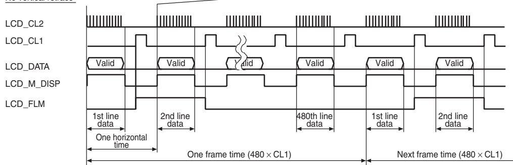
Figure 26.24 Clock and LCD Data Signal Example (16-Bit Interface Color 640 × 480)
