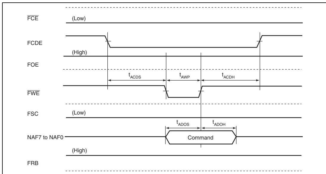
Figure 35.64 AND Type Flash Memory Command Issuance Timing
