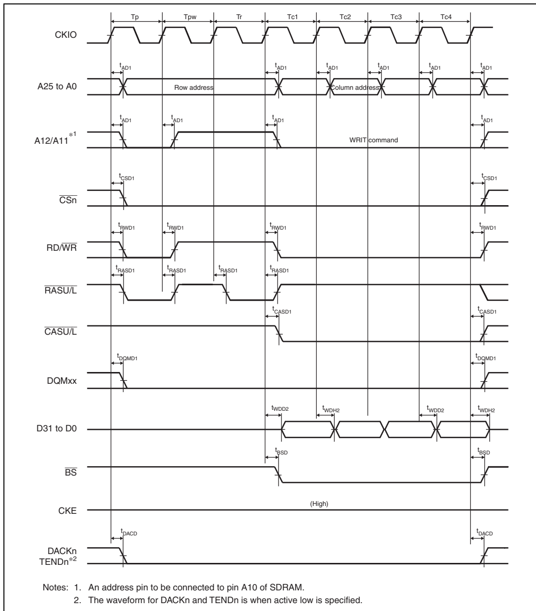
Figure 35.35 Synchronous DRAM Burst Write Bus Cycle (Four Write Cycles) (Bank Active Mode: PRE + ACT + WRITE Commands, Different Row Addresses, WTRCD = 0 Cycle, TRWL = 0 Cycle)
