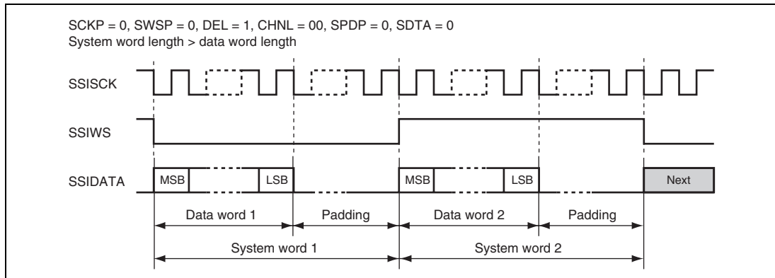
Figure 18.5 MSB-first and Left-Aligned Format (Transmitted and received in the order of serial data and padding bits)
