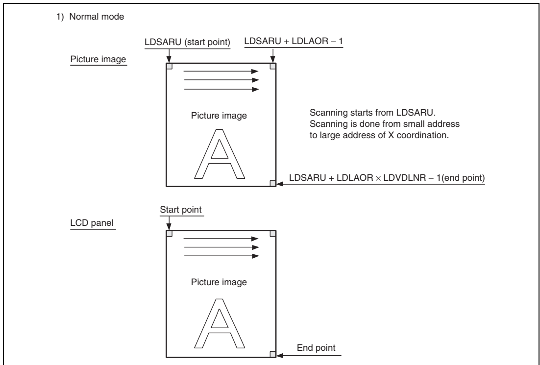
Figure 26.9 Operation for Hardware Rotation (Normal Mode)
