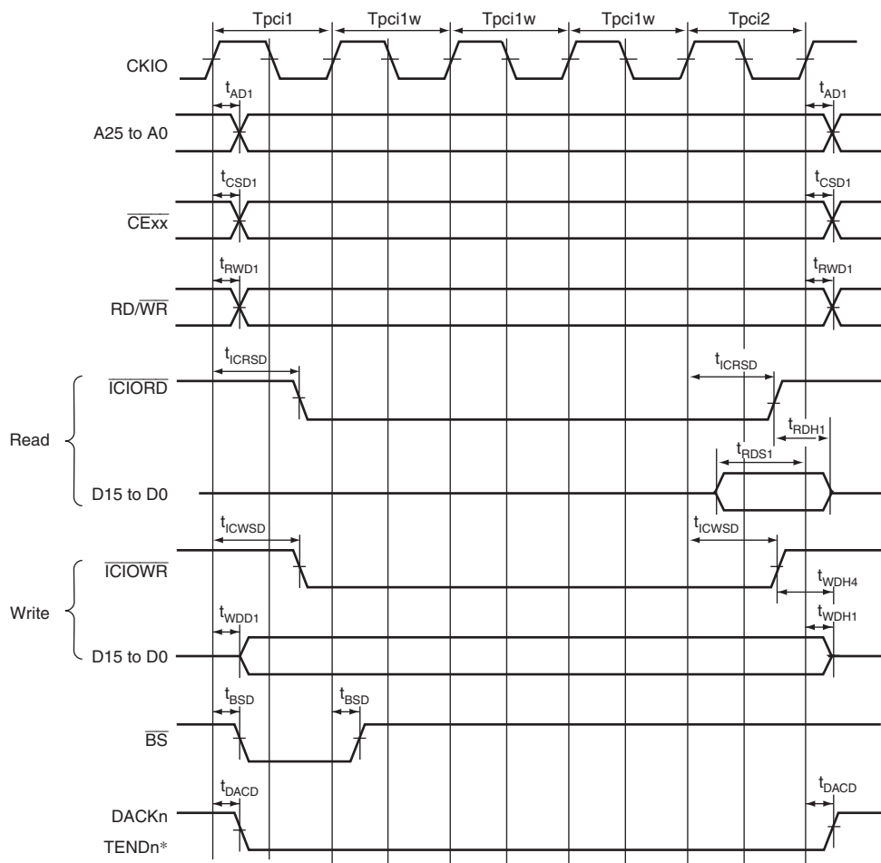
Figure 35.43 PCMCIA I/O Card Bus Cycle (TED = 0 Cycle, TEH = 0 Cycle, No Wait)
