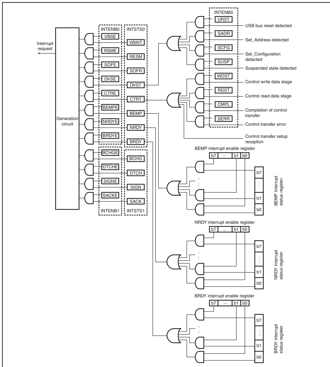
Figure 25.2 Items Relating to Interrupts
