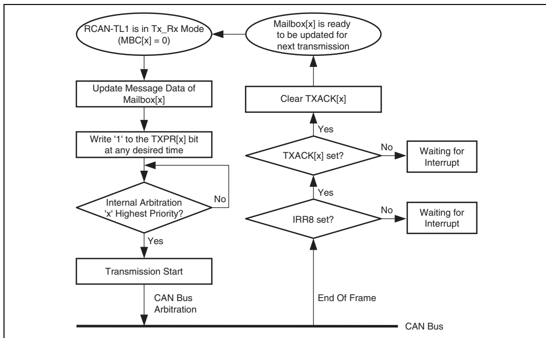
Figure 19.16 Transmission request
