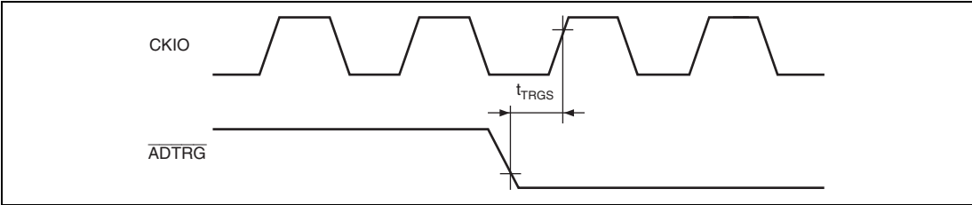
Figure 35.63 A/D Converter External Trigger Input Timing
