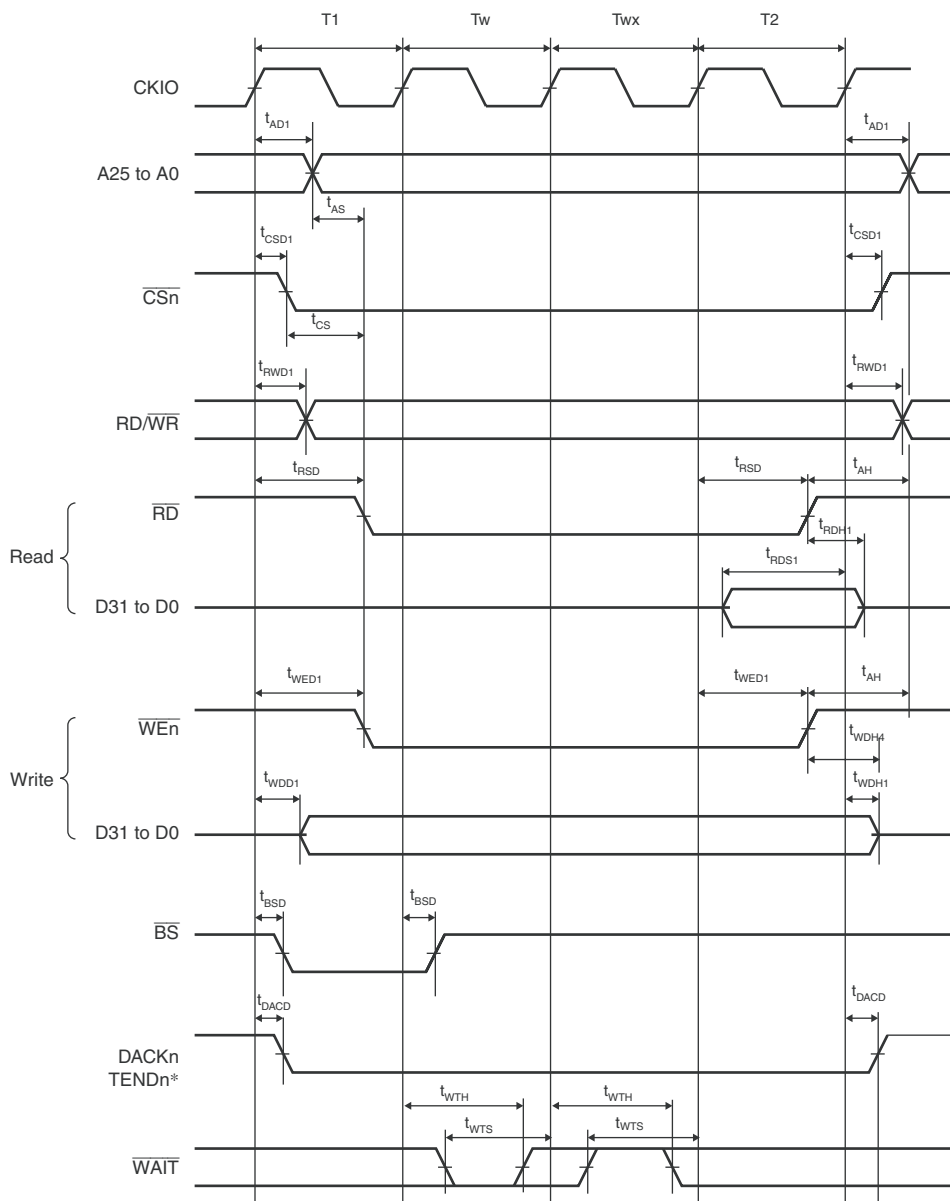
Figure 35.15 Basic Bus Timing for Normal Space (One Software Wait Cycle, One External Wait Cycle))
