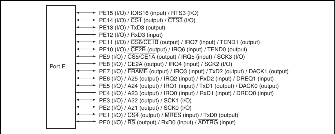
Figure 30.5 Port E
