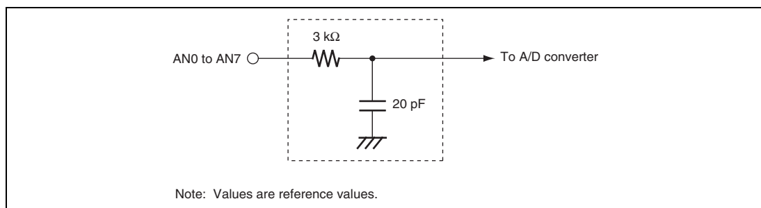
Figure 22.9 Analog Input Pin Equivalent Circuit
