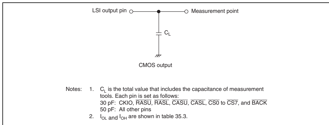
Figure 35.83 Output Load Circuit
