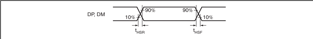
Figure 35.76 DP and DM Output Timing (High-Speed)
