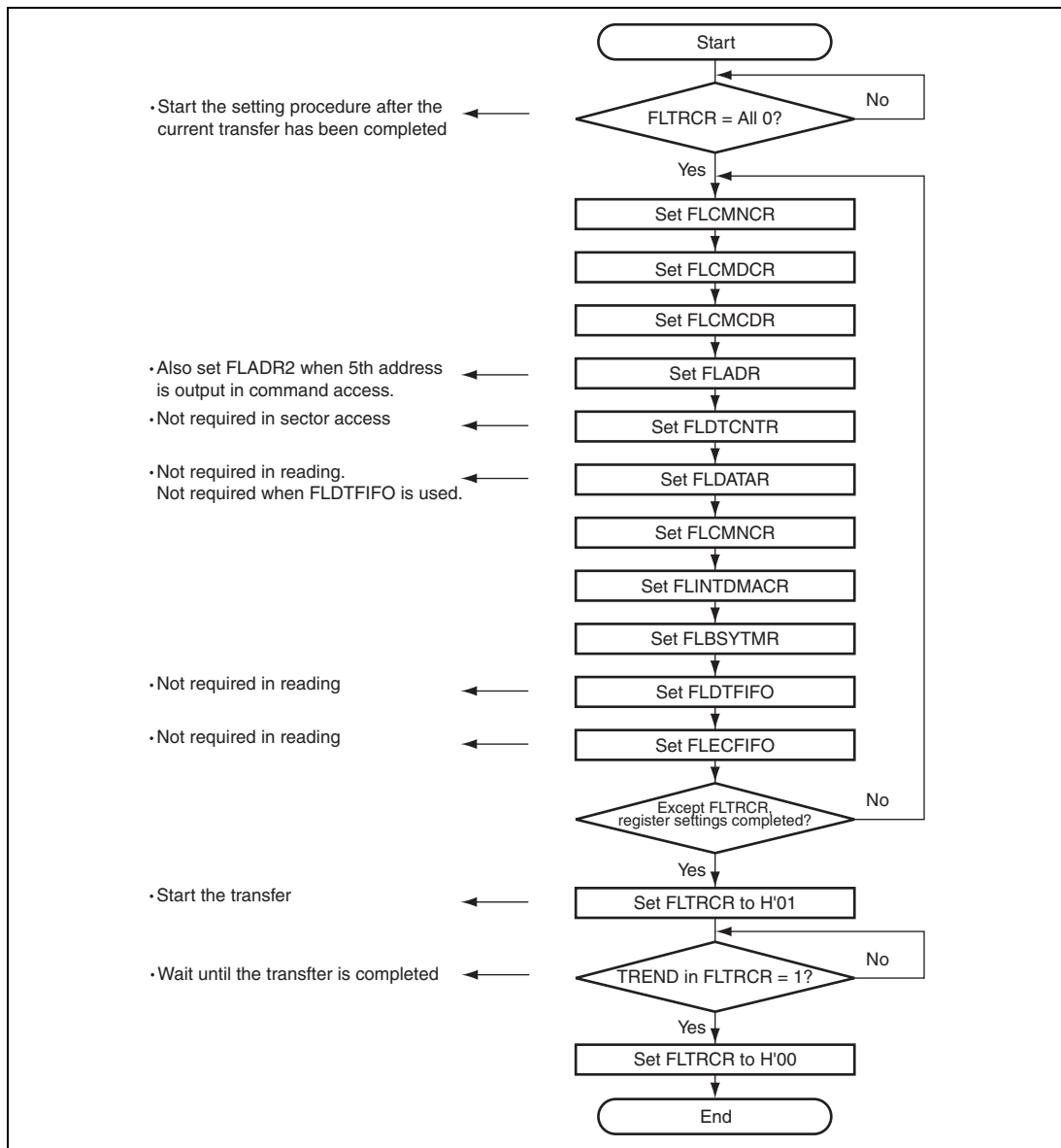
Figure 24.3 Register Setting Flow
