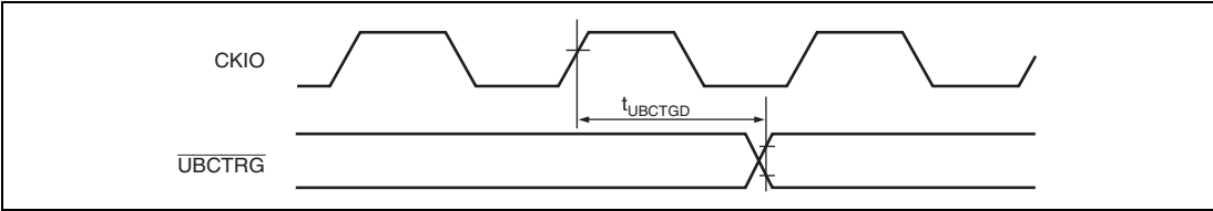
Figure 35.45 UBC Trigger Timing
