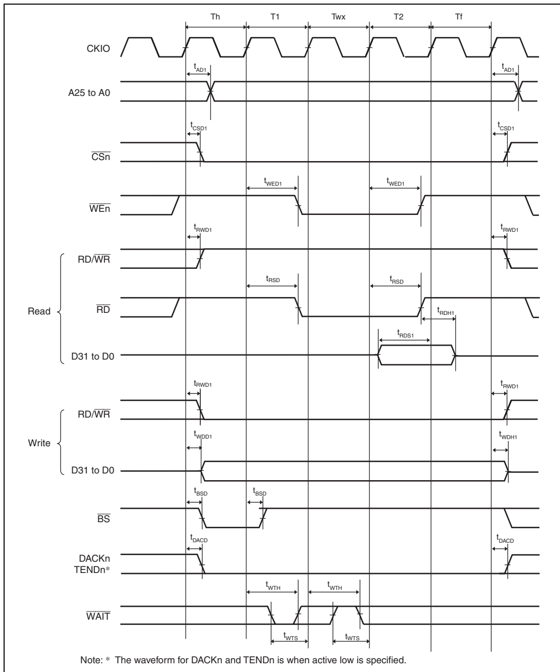
Figure 35.19 Bus Cycle of SRAM with Byte Selection (SW = 1 Cycle, HW = 1 Cycle, One Asynchronous External Wait Cycle, BAS = 0 (Write Cycle UB/LB Control))
