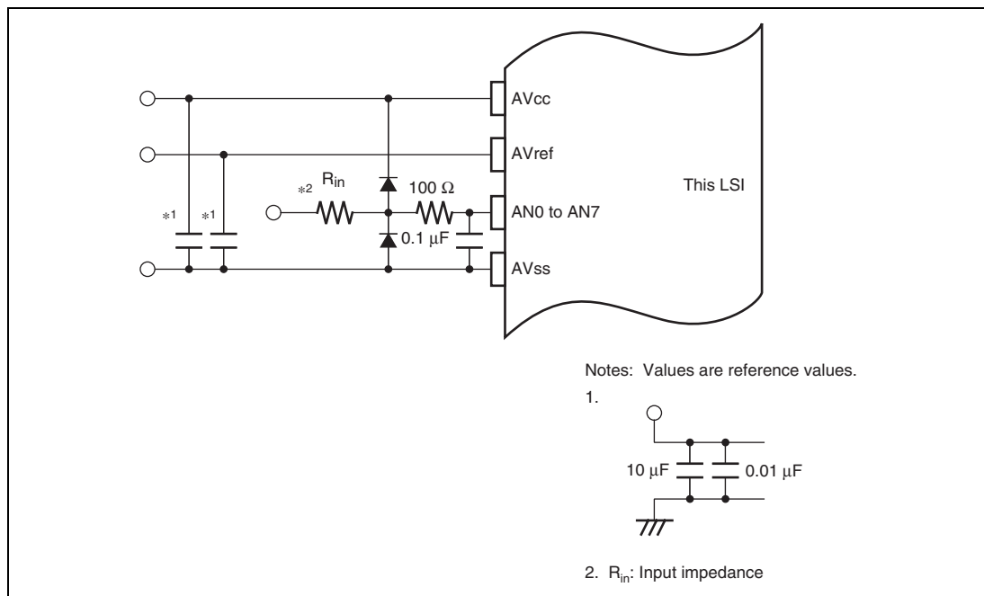
Figure 22.8 Example of Analog Input Protection Circuit
