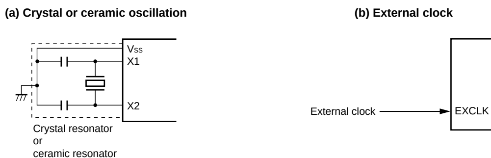
Figure 5-15. Example of External Circuit of X1 Oscillator
