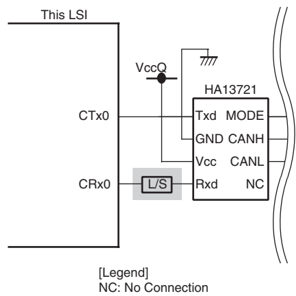
Figure 21.16 High-Speed CAN Interface Using HA13721 1123 Added
