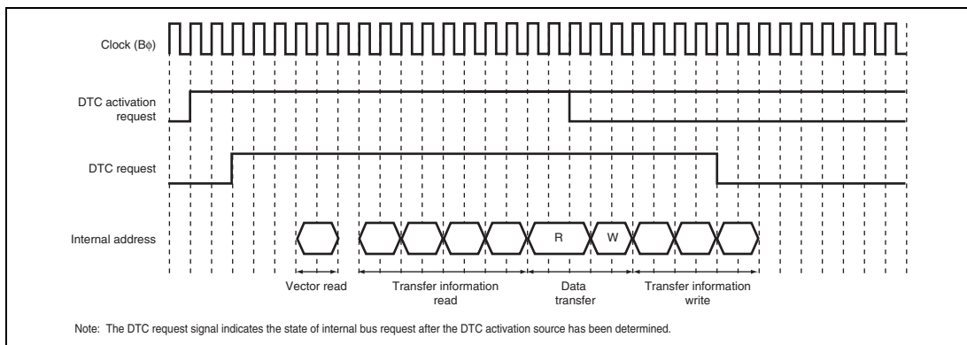
Figure 8.14 Example of DTC Operation Timing: Normal Transfer, Repeat Transfer, DTPR=1 (Activated by On-Chip Peripheral Module; I Φ : B Φ : P Φ = 1 : 1/2 : 1/2; Data Transferred from On-Chip Peripheral Module to On-Chip RAM; Transfer Information is Written in 3 Cycles)
