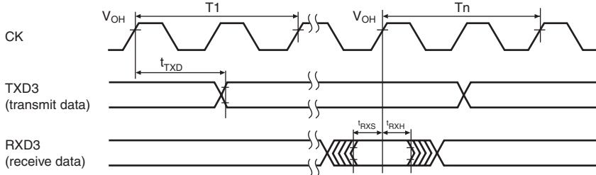
SCI I/O timing (asynchronous mode)
