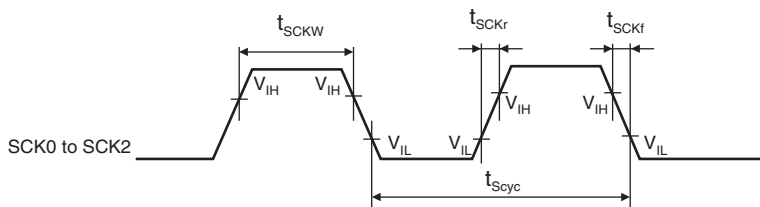
Figure 33.45 Input Clock Timing
