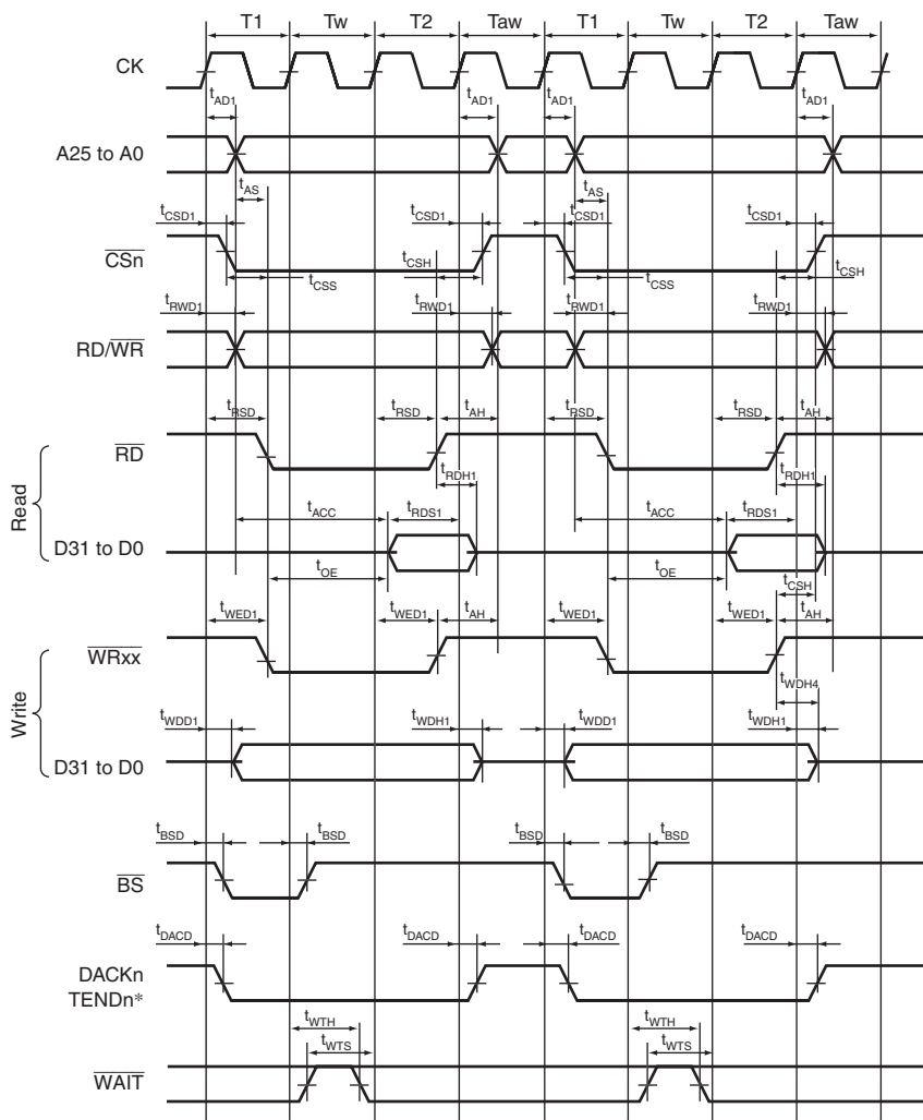
Figure 33.13 Basic Bus Timing for Normal Space (One Software Wait Cycle, External Wait Cycle Valid (WM Bit = 0), No Idle Cycle)
