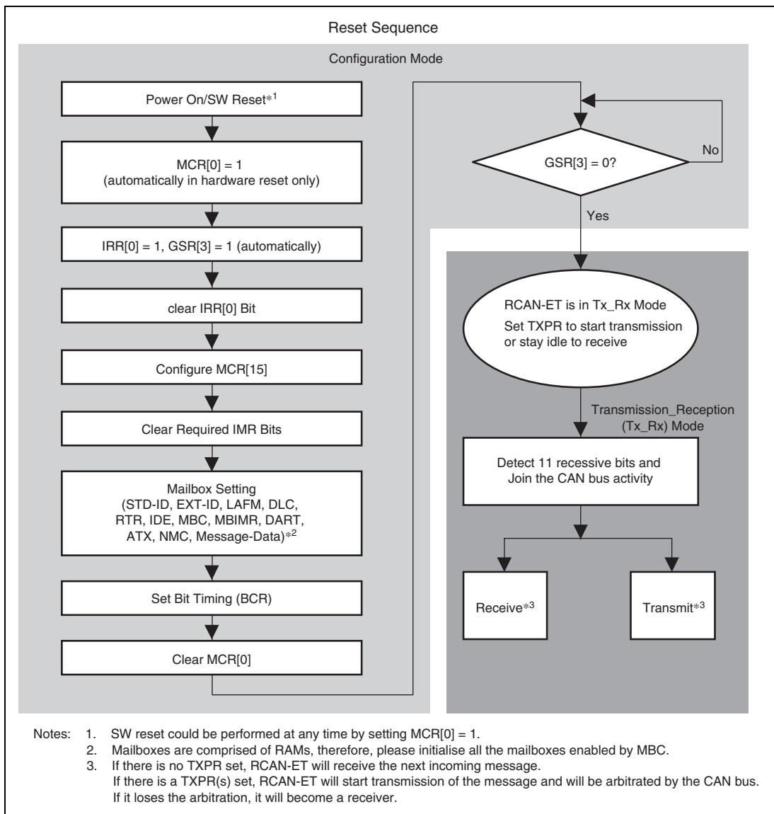
Figure 21.8 Reset Sequence
