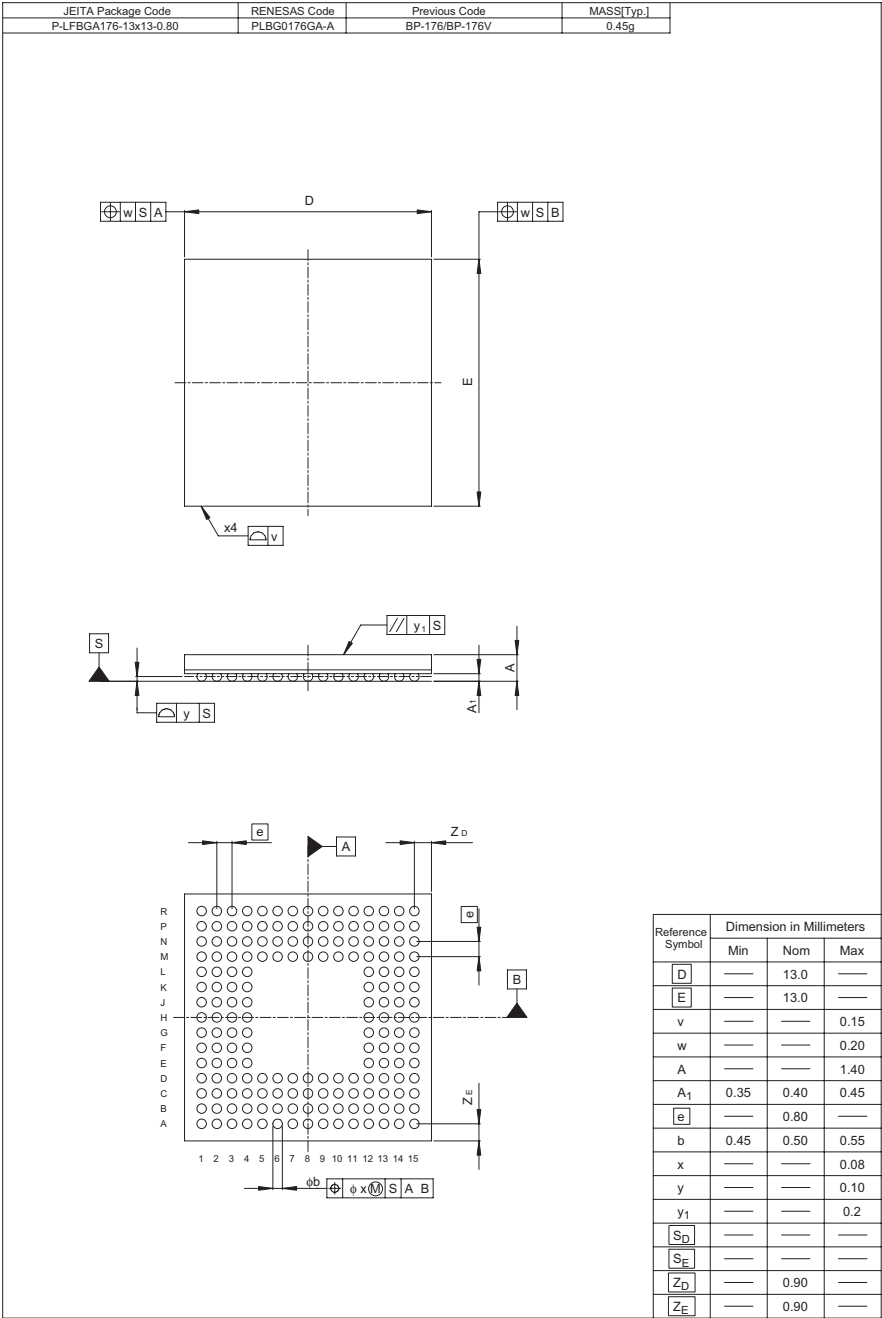
Figure C.3 Package Dimensions (3)
