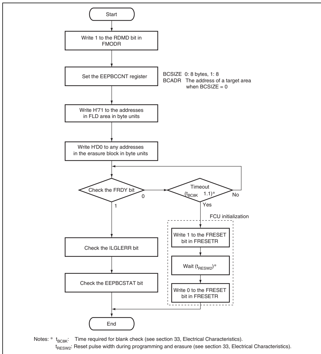
Figure 28.7 Procedure of the FLD Blank Check
