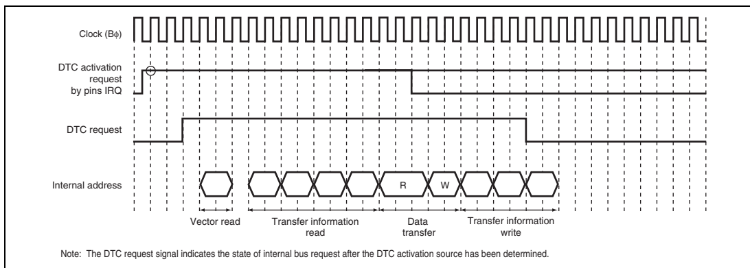
Figure 8.15 Example of DTC Operation Timing: Normal Transfer, Repeat Transfer, (Activated by IRQ; I Φ : B Φ : P Φ = 1 : 1/2 : 1/2; Data Transferred from On-Chip Peripheral Module to On-Chip RAM; Transfer Information is Written in 3 Cycles)
