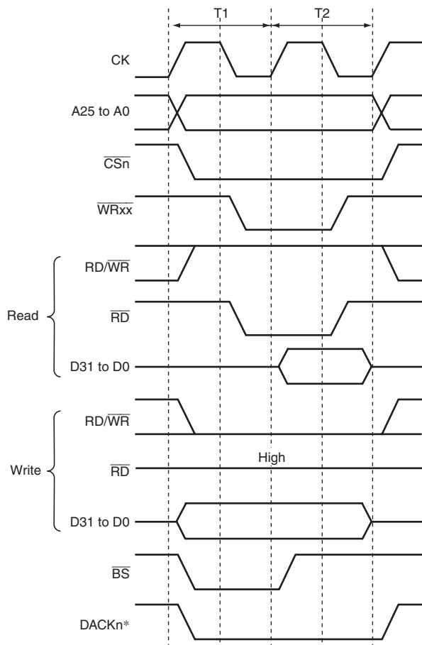
Figure 9.37 Basic Access Timing for SRAM with Byte Selection (BAS = 0)
