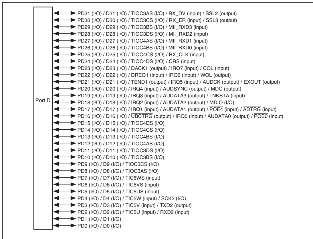
Figure 23.4 Port D
