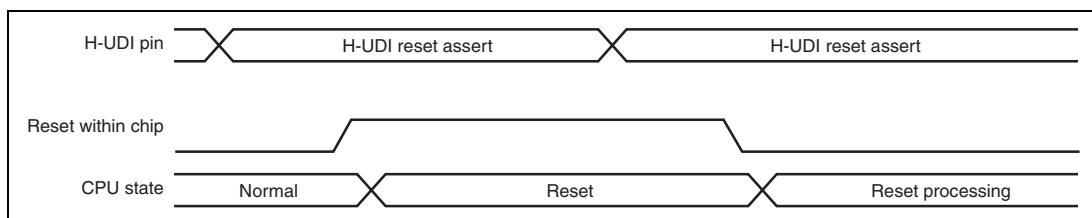
Figure 31.4 H-UDI Reset
