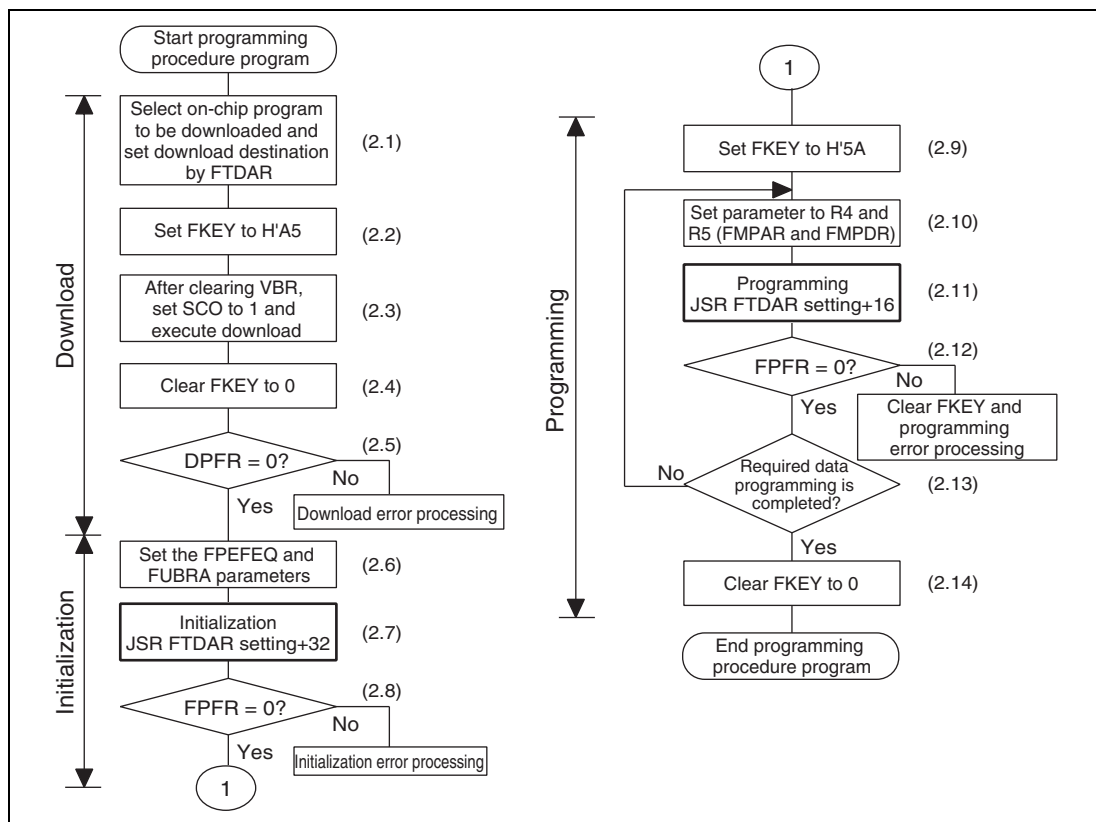
Figure 26.13 Programming Procedure
