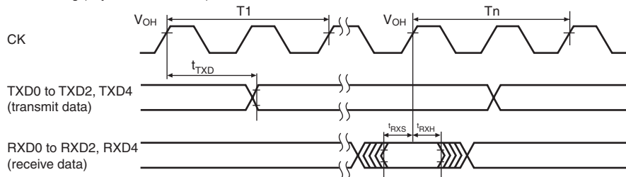
Figure 31.46 SCI Input/Output Timing
