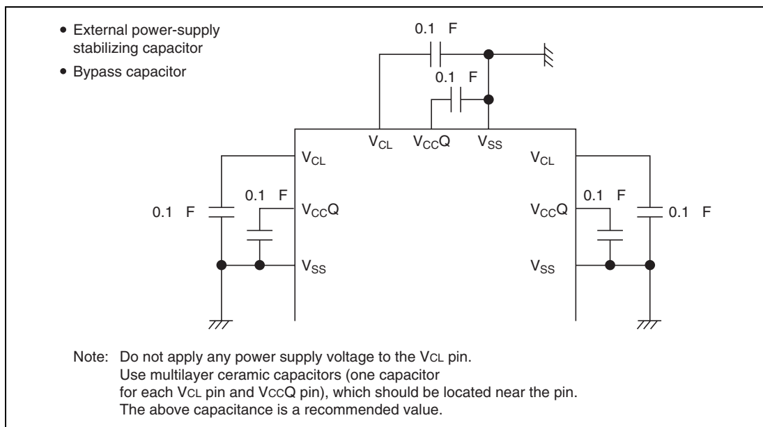
Figure 31.62 Connection of Capacitors
