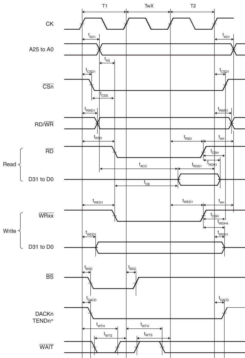
Figure 31.12 Basic Bus Timing for Normal Space (One External Wait Cycle)
