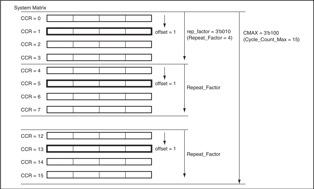
Figure 22.8 System Matrix
