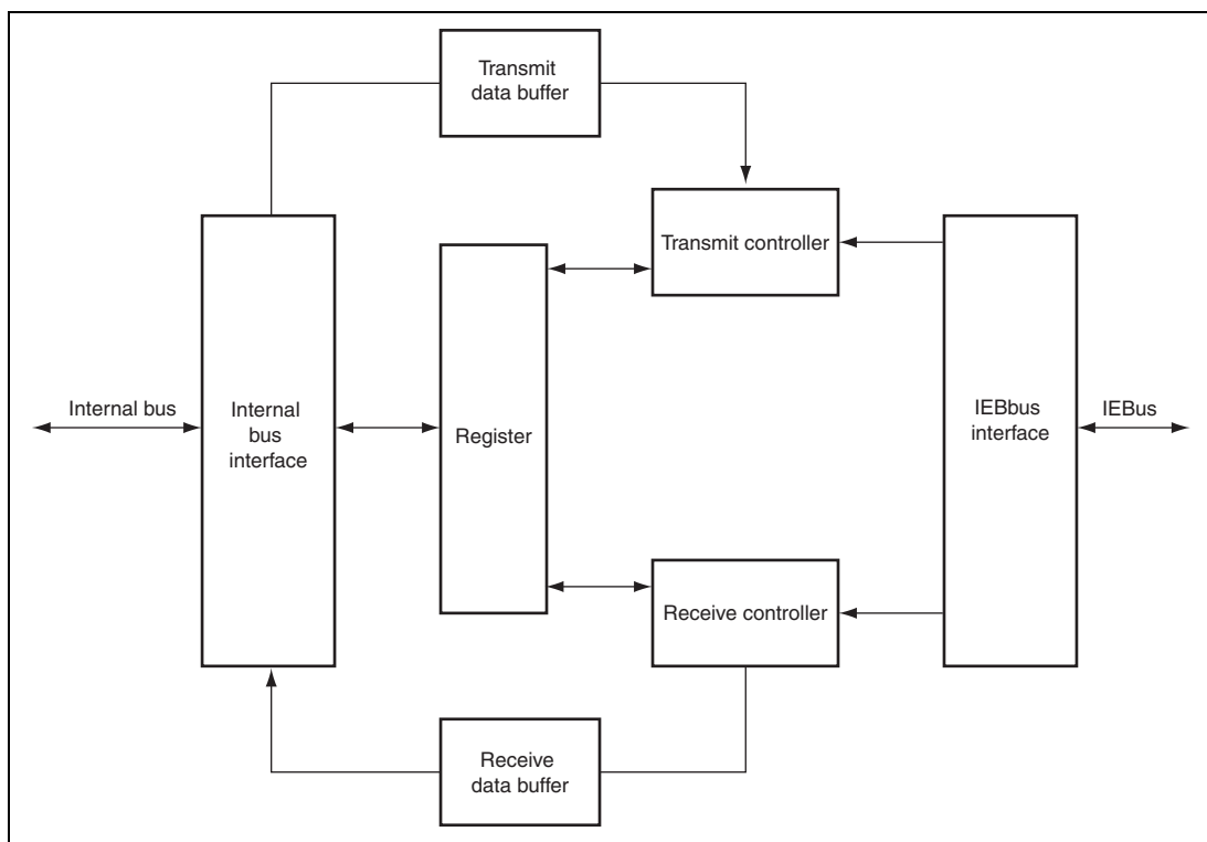
Figure 23.5 Block Diagram
