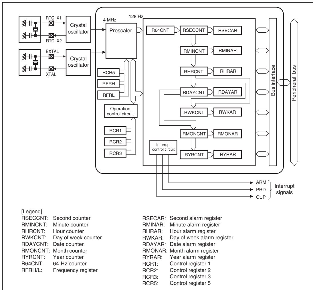
Figure 15.1 Block Diagram
