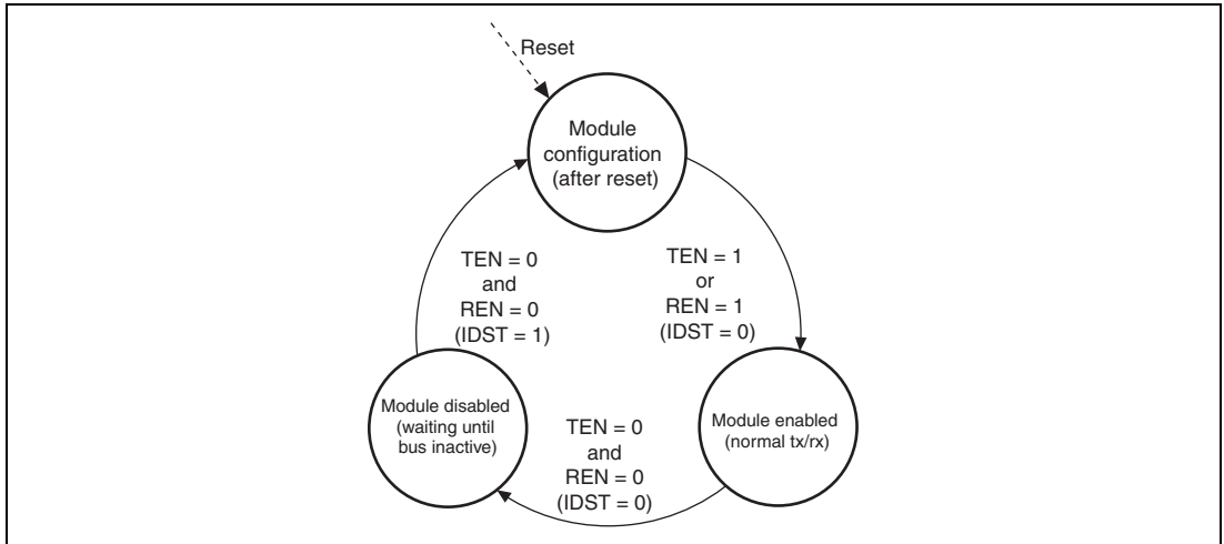
Figure 20.22 Operation Modes
