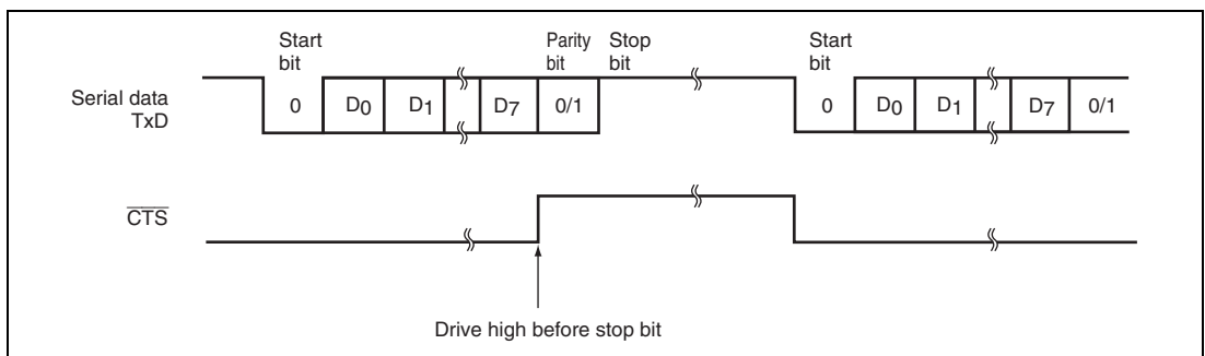
Figure 16.6 Example of Operation Using Modem Control ( \overline{\text{CTS}} )
