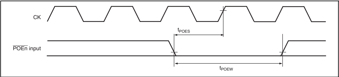
Figure 28.59 \overline{POE} Input Timing
