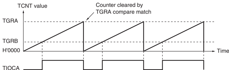
Figure 11.26 Example of PWM Mode 1 Operation
