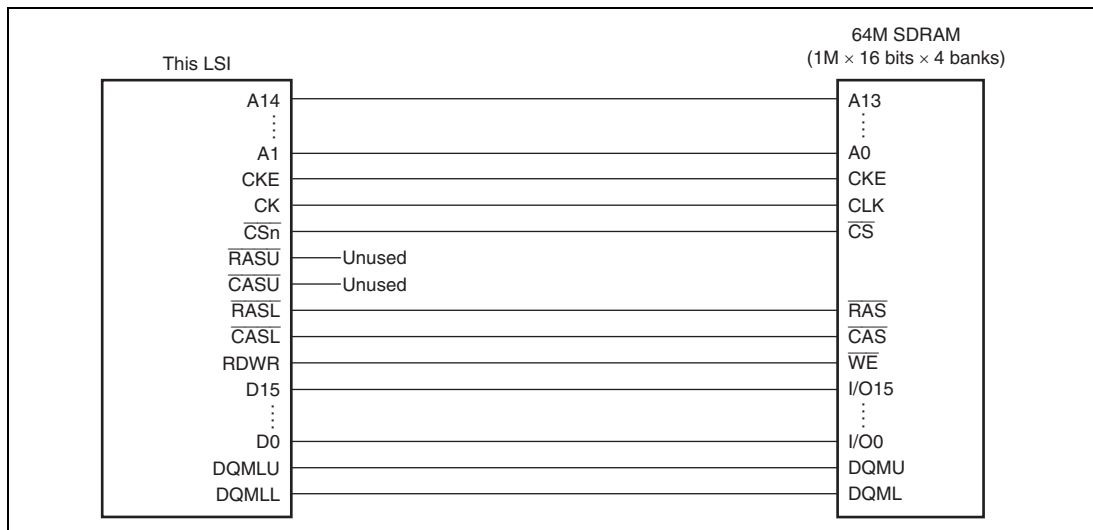
Figure 9.16 Example of 16-Bit Data Width SDRAM Connection ( \overline{RASU} and \overline{CASU} Are Not Used)
