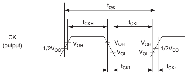
Figure 28.2 CK Clock Output Timing
