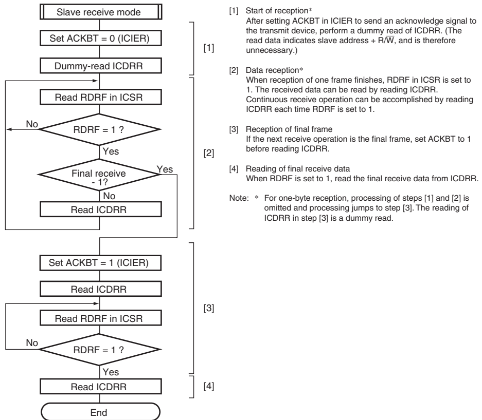
Figure 18.23 Sample Flowchart for Slave Receive Mode
