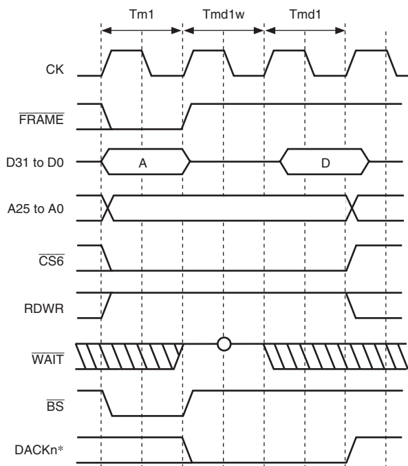
Figure 9.45 Burst MPX Space Access Timing (Single Read, No Wait or Software Wait 1)
