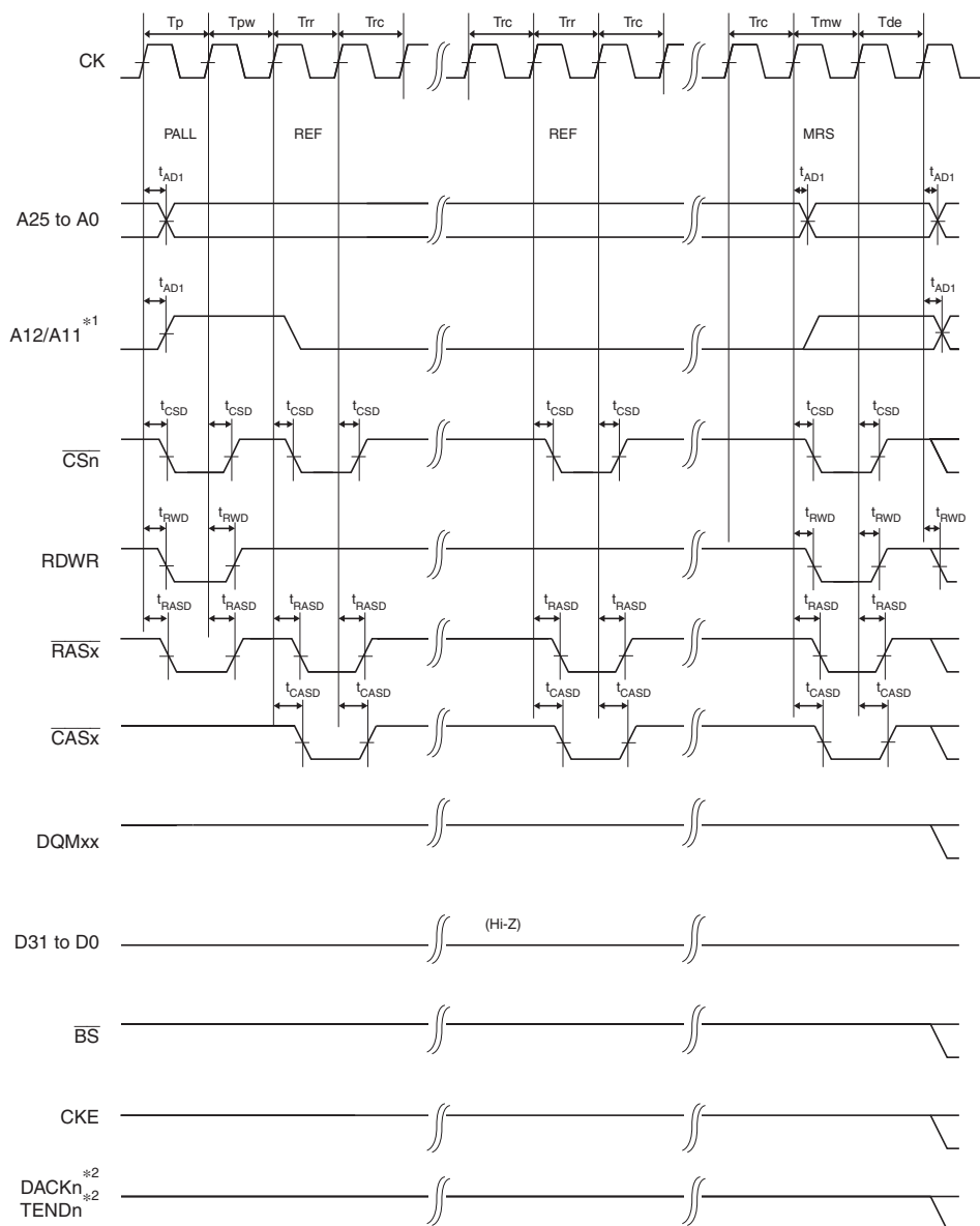
Figure 28.40 Synchronous DRAM Mode Register Write Timing (WTRP = 1 Cycle)
