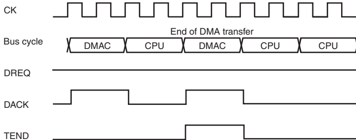
Figure 10.18 DMA Transfer End Timing (in Cycle Steal Level Detection)
