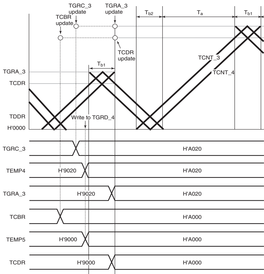
Figure 11.42 Example of PWM Cycle Updating
