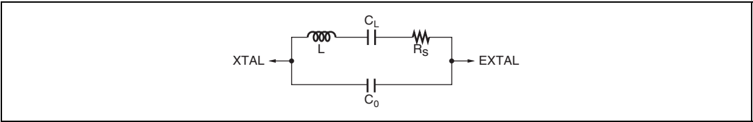
Figure 4.3 Crystal Resonator Equivalent Circuit
