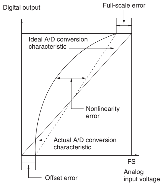
Figure 19.6 Definitions of A/D Conversion Accuracy
