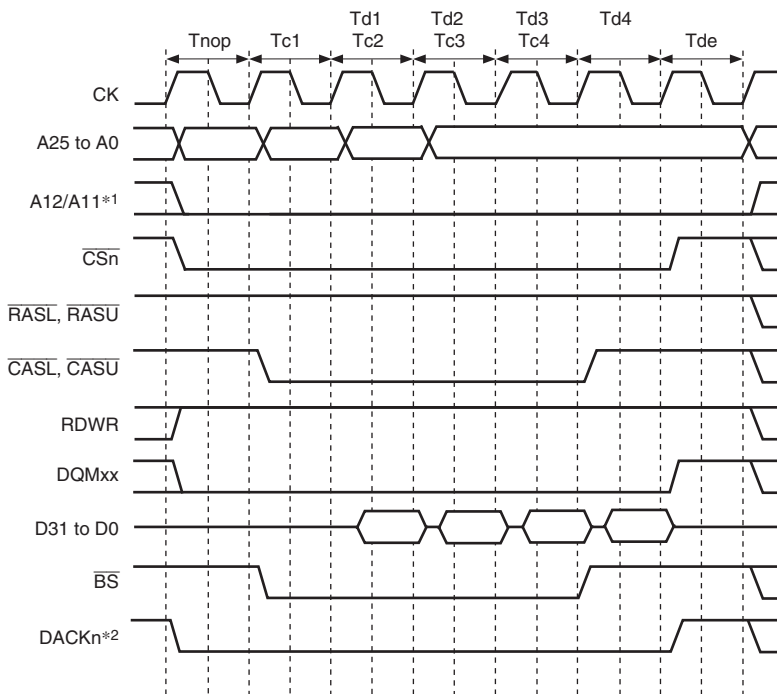
Figure 9.24 Burst Read Timing (Bank Active, Same Row Address)
