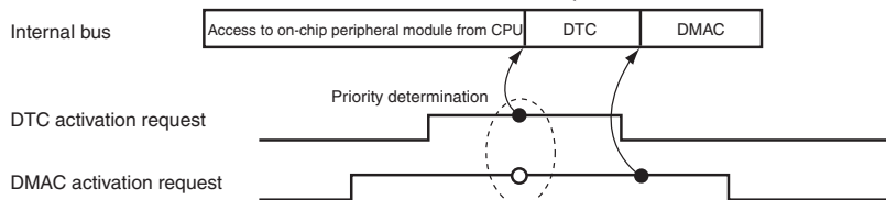
Figure 9.50 Bus Arbitration when DTC and DMAC Compete during External Space Access from CPU
