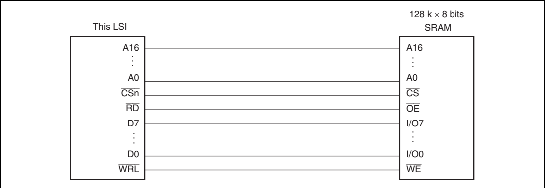
Figure 9.7 Example of 8-Bit Data-Width SRAM Connection
