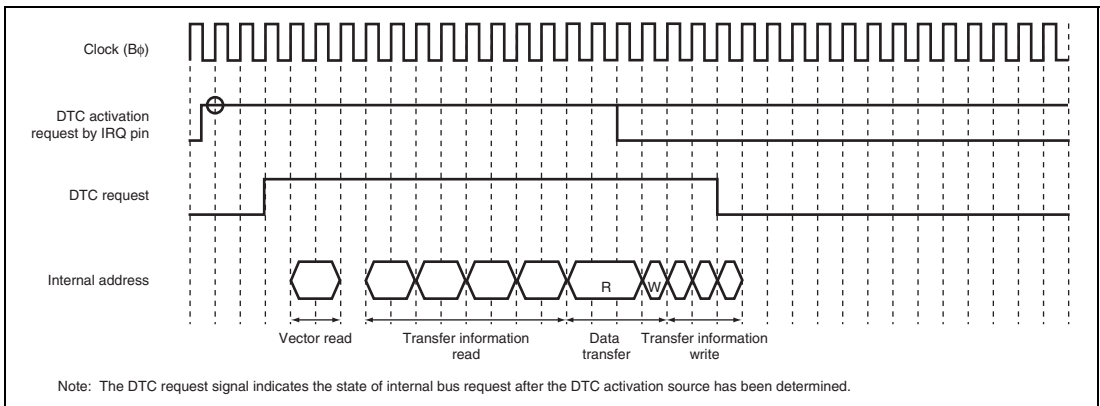
Figure 8.15 Example of DTC Operation Timing: Normal or Repeat Transfer (Activated by IRQ; Iφ: Bφ: Pφ=1: 1/2: 1/2; Data Transferred from On-Chip Peripheral Module to On-Chip RAM; Transfer Information Is Written in 3 Cycles)
