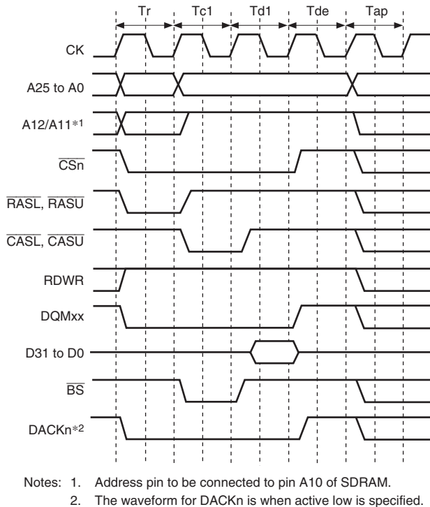
Figure 9.20 Single Read Basic Timing (Auto-Precharge)
