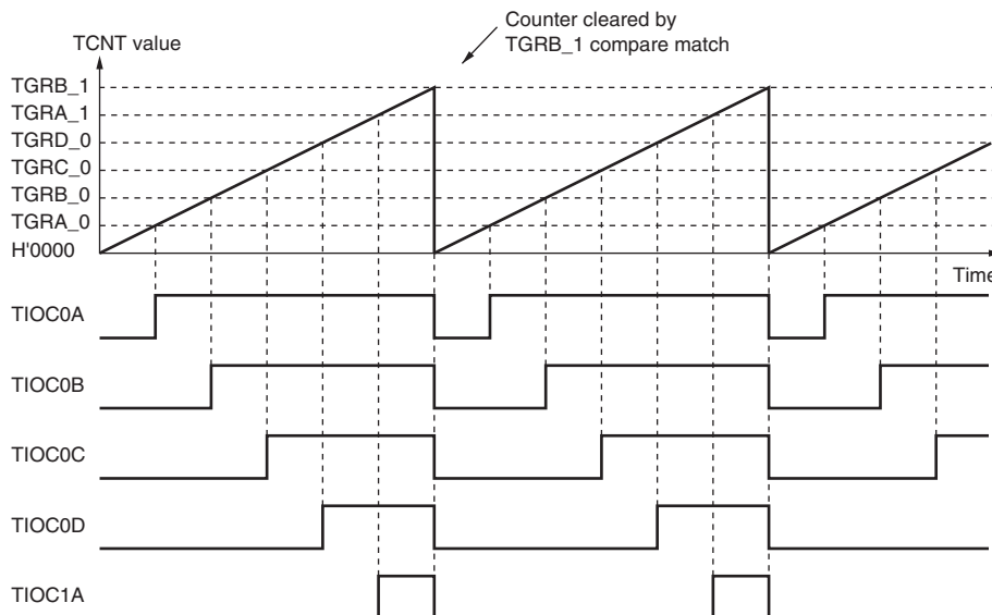
Figure 11.27 Example of PWM Mode 2 Operation
