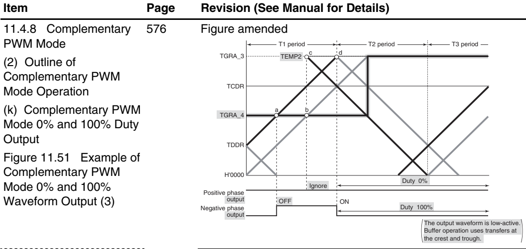
Figure 11.52 Example of Complementary PWM Mode 0% and 100% Waveform Output (4)
