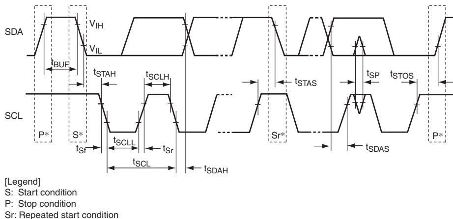
Figure 28.60 I²C2 Input/Output Timing
