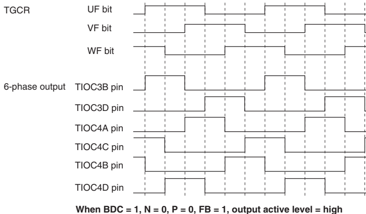
Figure 11.71 Example of Output Phase Switching by Means of UF, VF, WF Bit Settings (1)
