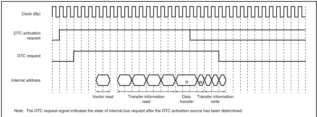
Figure 8.14 Example of DTC Operation Timing: Normal or Repeat Transfer with DTPR = 1 (Activated by On-Chip Peripheral Module; Iφ: Bφ: Pφ=1: 1/2: 1/2; Data Transferred from On-Chip Peripheral Module to On-Chip RAM; Transfer Information Is Written in 3 Cycles)
