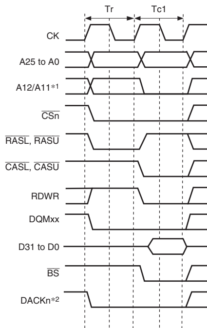
Figure 9.26 Single Write Timing (No Auto-Precharge)
