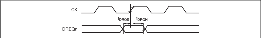
Figure 28.45 DREQ Input Timing
