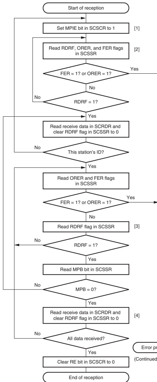
Figure 15.18 Sample Multiprocessor Serial Reception Flowchart (1)
