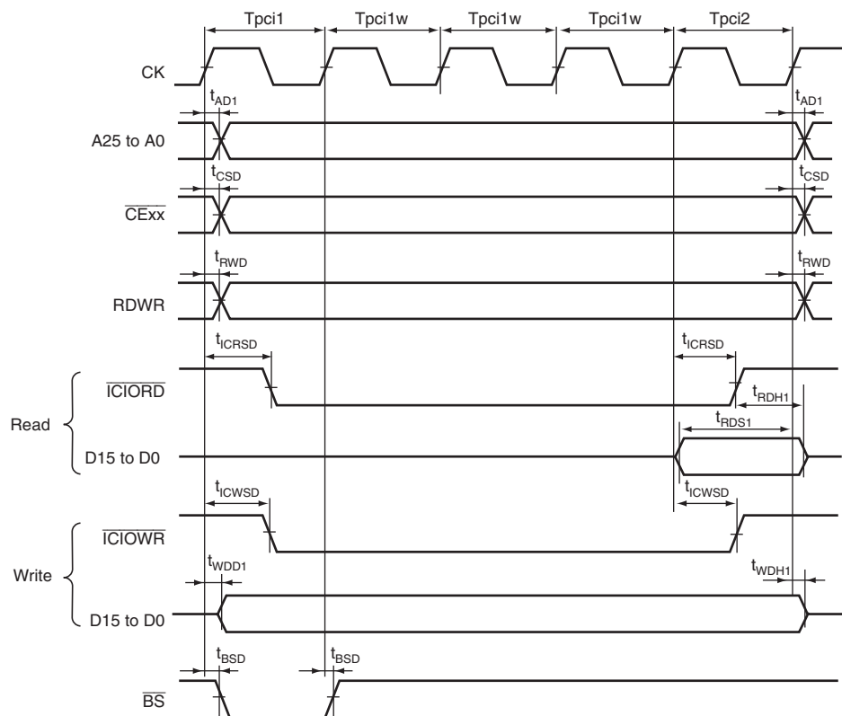
Figure 28.43 PCMCIA I/O Card Interface Bus Timing
