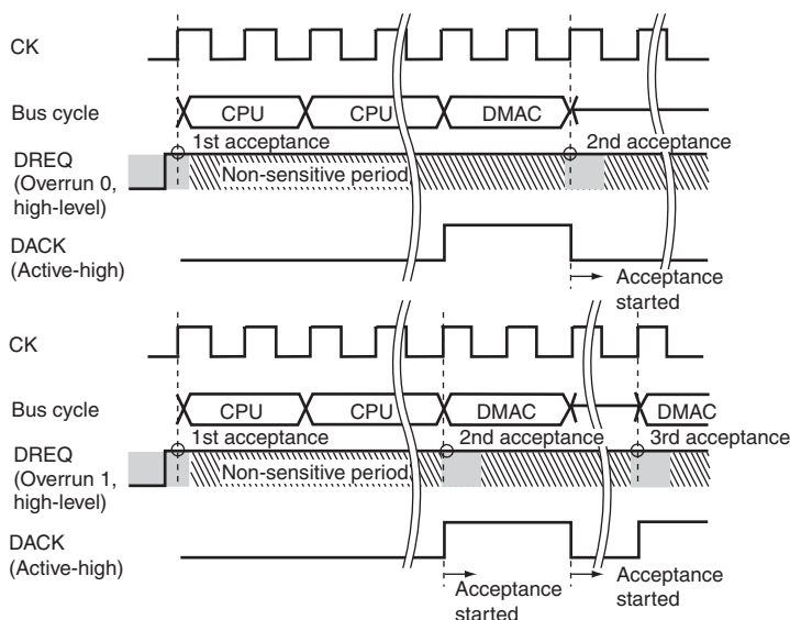
Figure 10.17 Example of DREQ Input Detection in Burst Mode Level Detection
