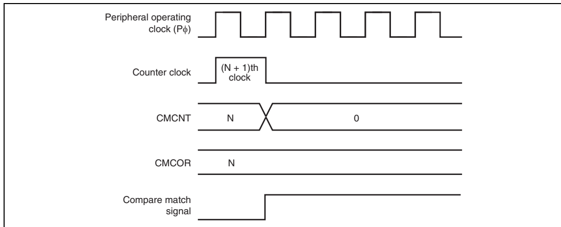
Figure 20.4 Timing of CMF Setting
