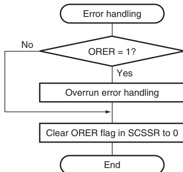
Figure 15.12 Sample Flowchart for Receiving Serial Data (Clock Synchronous Mode) (2)
