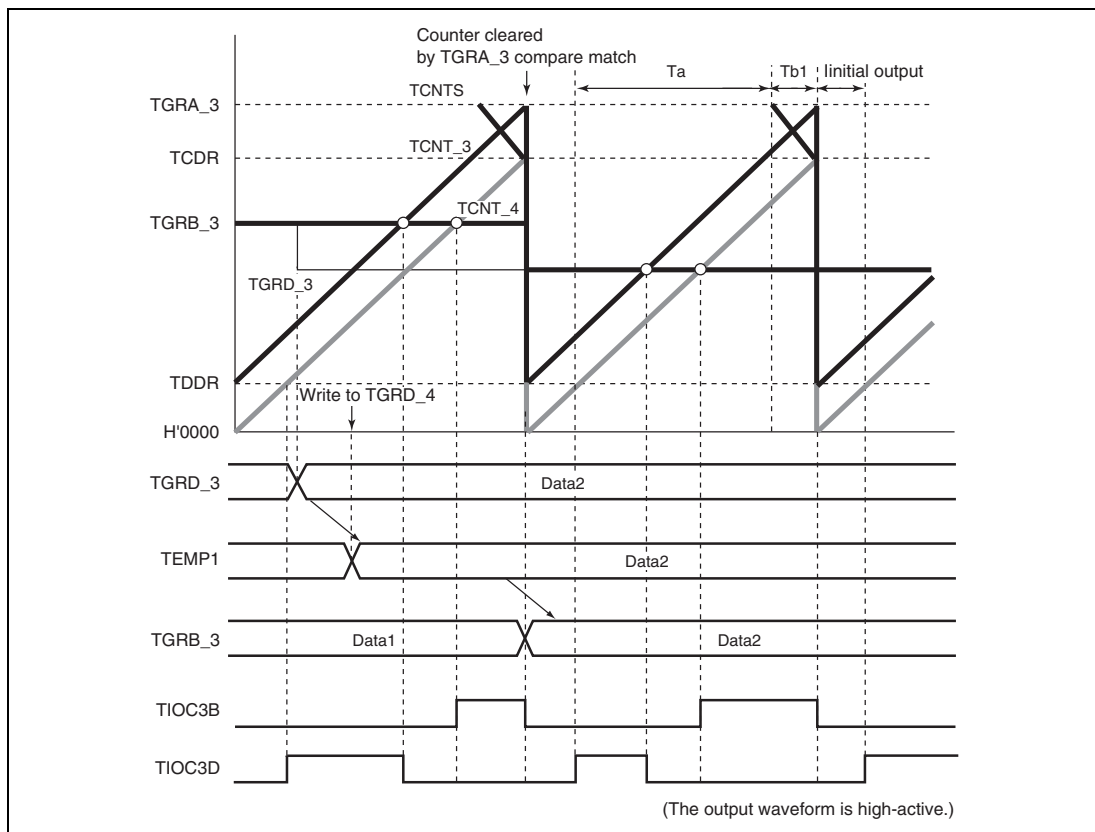
Figure 11.68 Example of Counter Clearing Operation by TGRA_3 Compare Match
