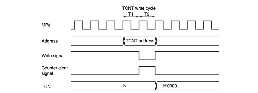
Figure 11.121 Contention between TCNT Write and Clear Operations
