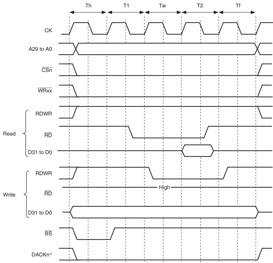
Figure 9.35 Byte Selection SRAM Wait Timing (BAS = 1, SW[1:0] = 01, WR[3:0] = 0001, HW[1:0] = 01)
