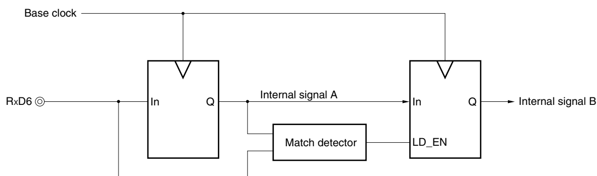
Figure 15-23. Noise Filter Circuit
