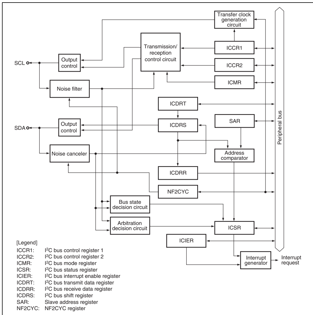
Figure 17.1 Block Diagram
