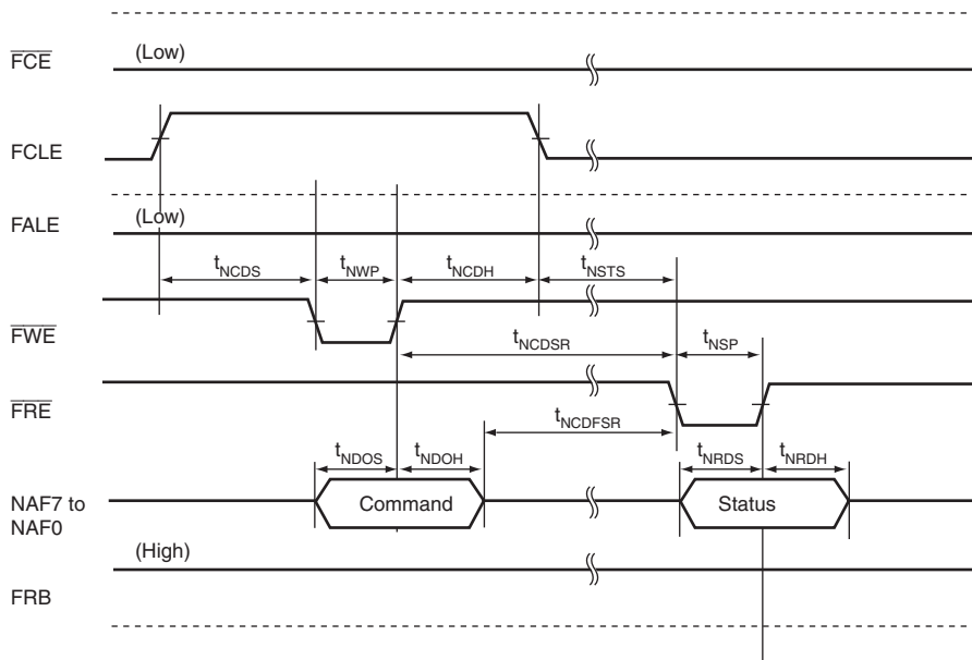
Figure 37.64 NAND Type Flash Memory Status Read Timing
