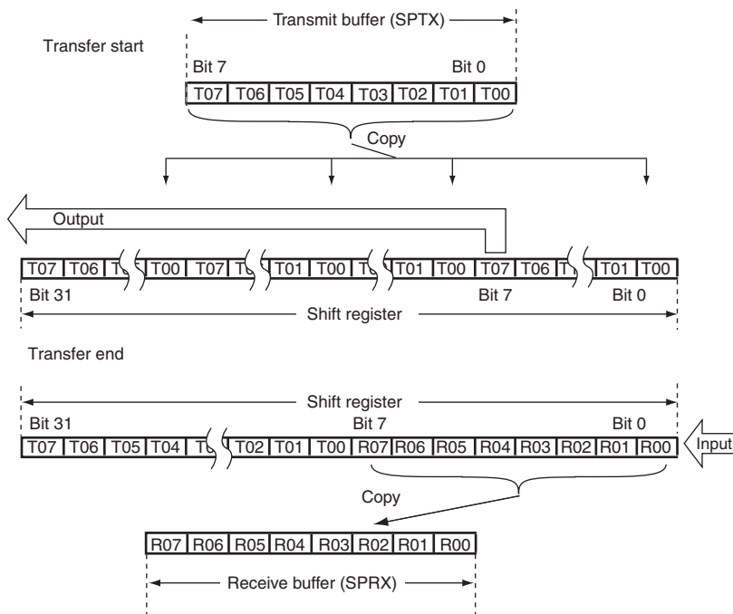
Figure 16.10 MSB First Transfer (8-Bit Data)
