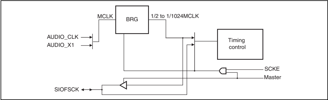
Figure 19.2 Serial Clock Supply
