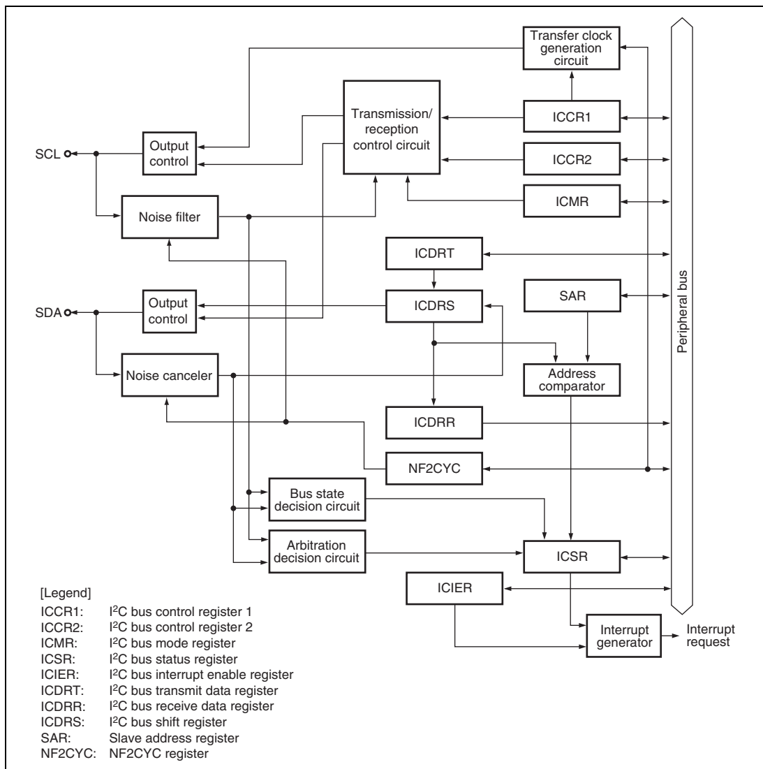
Figure 17.1 Block Diagram
