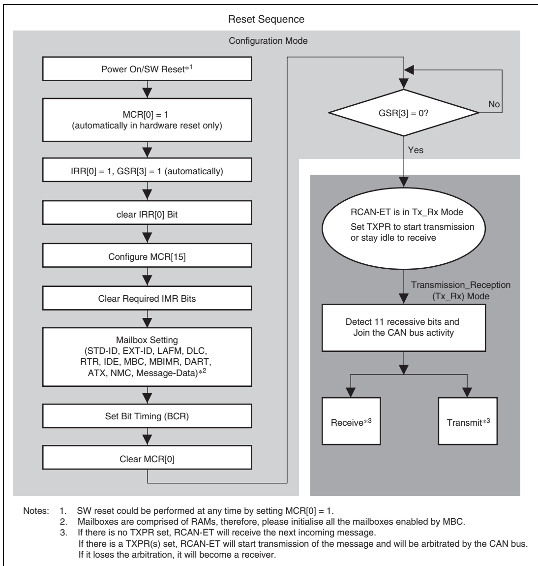
Figure 20.8 Reset Sequence
