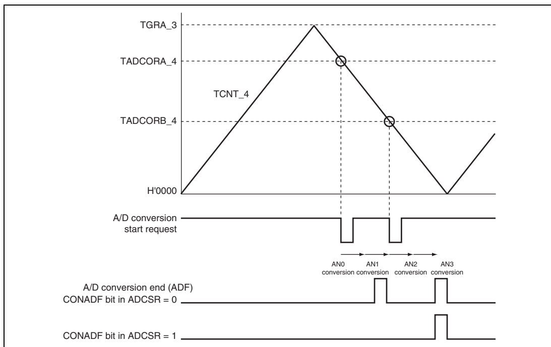
Figure 19.6 2-Channel Scan Mode Operation Example (1)
