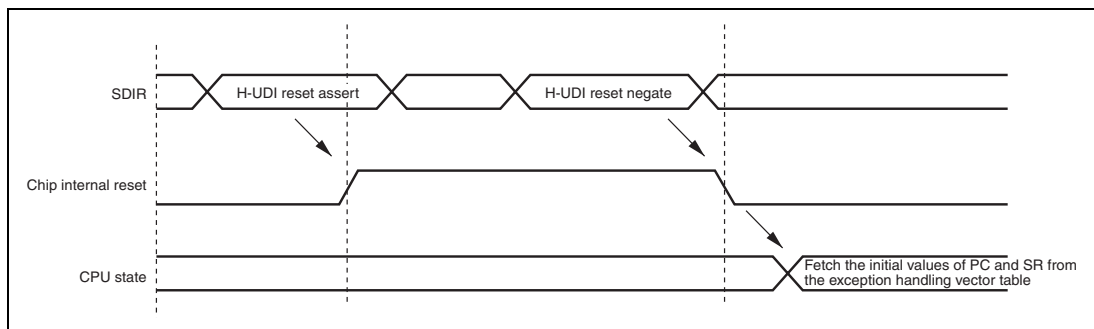
Figure 27.4 H-UDI Reset
