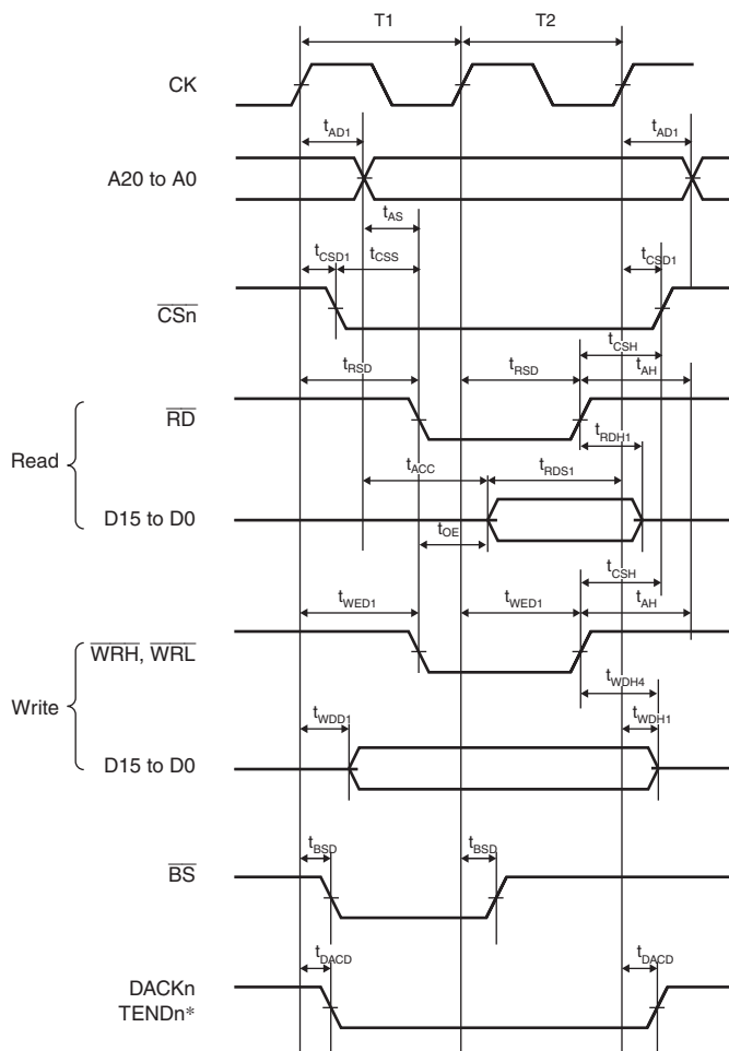
Figure 29.10 Basic Bus Timing for Normal Space (No Wait)
