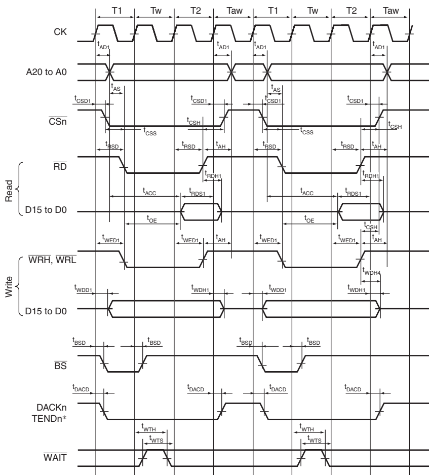
Figure 29.13 Basic Bus Timing for Normal Space (One Software Wait Cycle, External Wait Cycle Valid (WM Bit = 0), No Idle Cycle)
