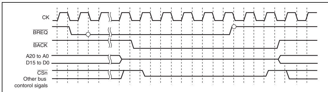
Figure 9.16 Bus Arbitration Timing
