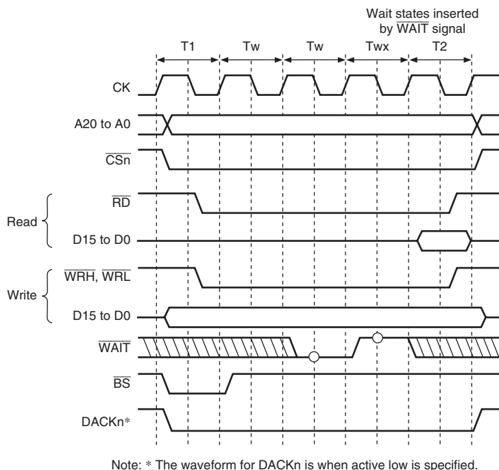
Figure 9.8 Wait Cycle Timing for Normal Space Access (Wait Cycle Insertion Using \overline{\text{WAIT}} Signal)
