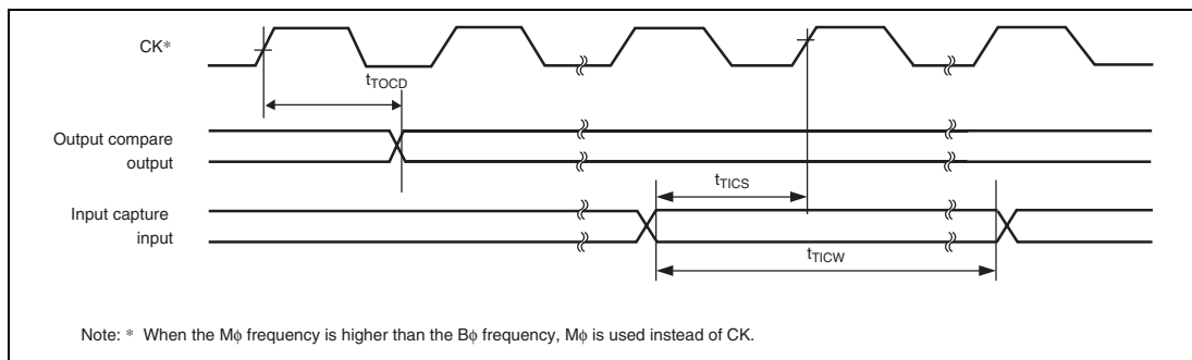
Figure 29.18 MTU2 and MTU2S Input/Output Timing
