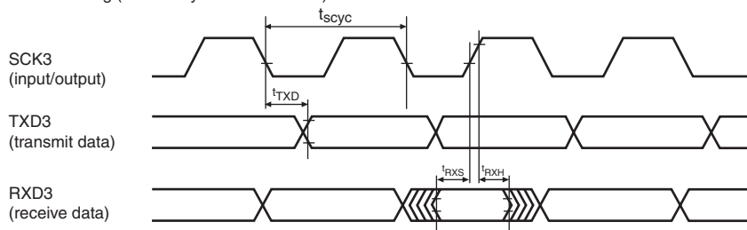
SCI I/O timing (clocked synchronous mode)
