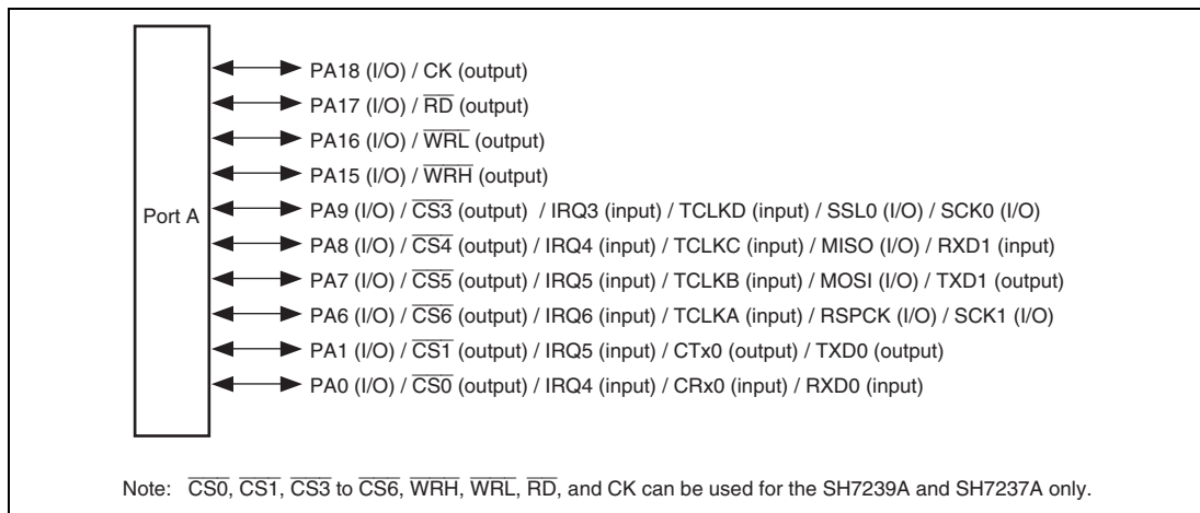
Figure 22.1 Port A
