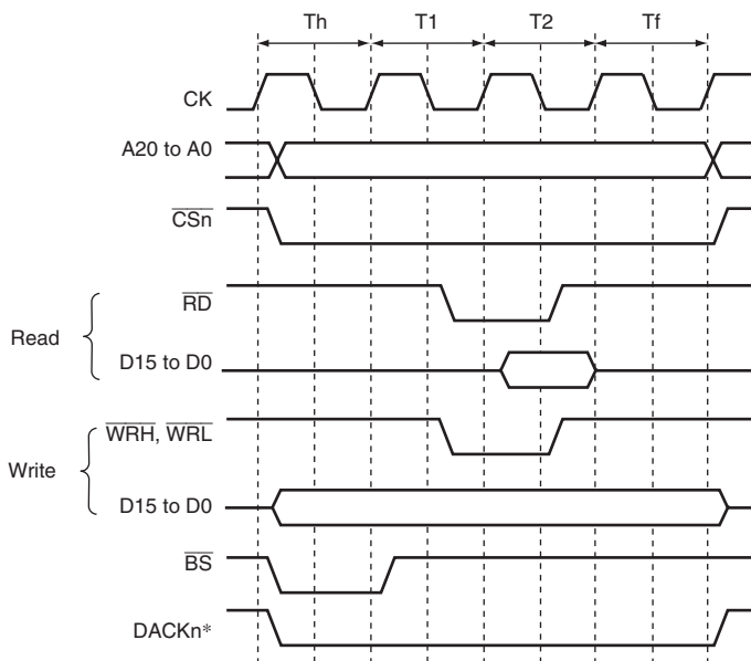
Figure 9.9 \overline{\text{CSn}} Assert Period Expansion
