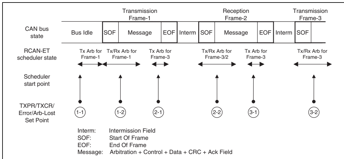
Figure 20.11 Internal Arbitration for Transmission
