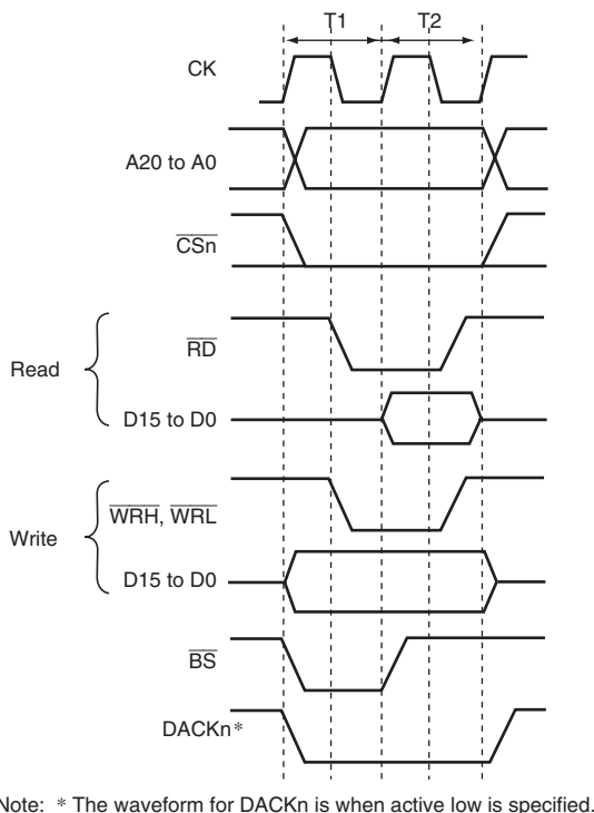
Figure 9.2 Normal Space Basic Access Timing (Access Wait 0)
