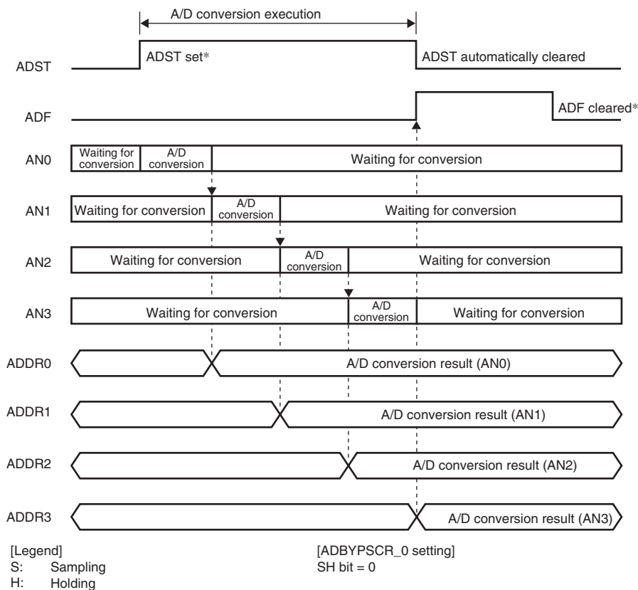
Figure 19.3 Example 2 of A/D_0 Converter Operation (Single-Cycle Scan Mode and Sample-and-Hold Circuit Disabled)
