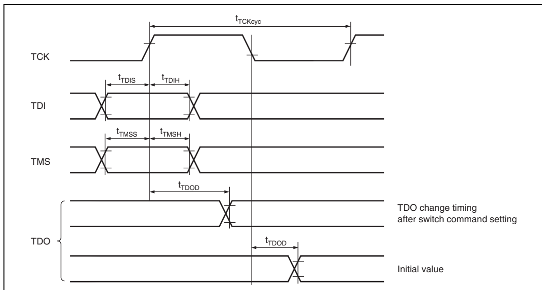
Figure 29.35 H-UDI Data Transmission Timing
