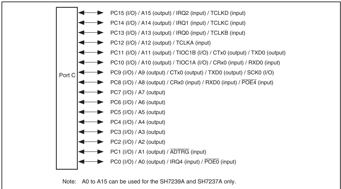
Figure 22.3 Port C
