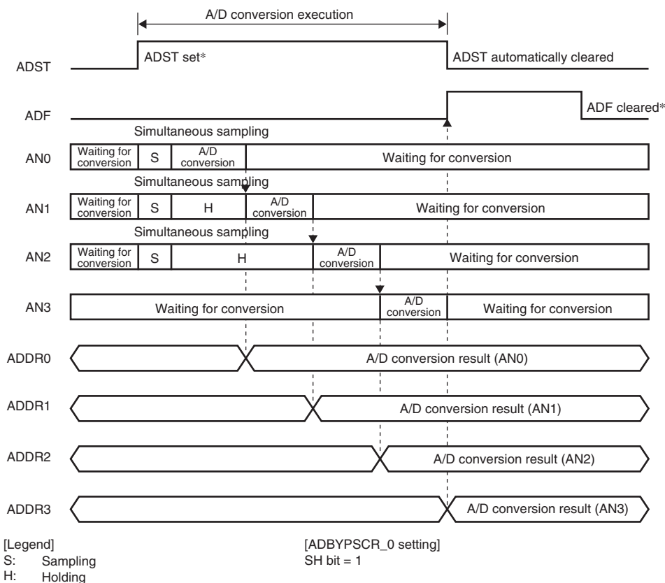
Figure 19.2 Example 1 of A/D_0 Converter Operation (Single-Cycle Scan Mode and Sample-and-Hold Circuit Enabled)
