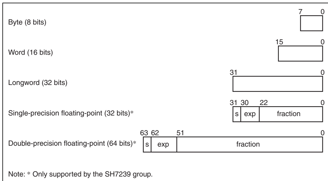
Figure 2.1 Data Format
