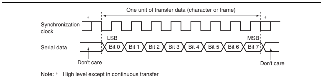
Figure 16.9 Data Format in Clock Synchronous Communication
