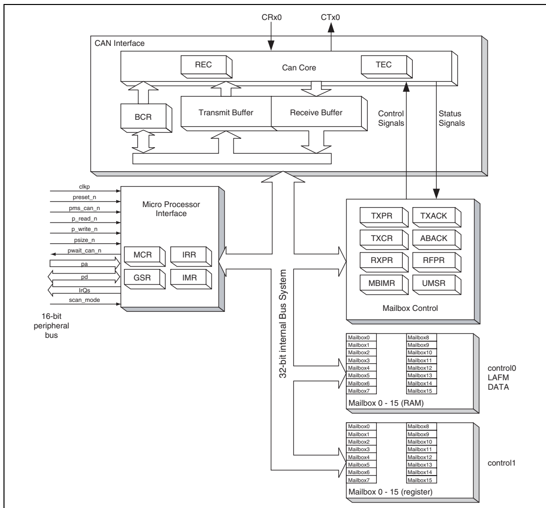
Figure 20.1 RCAN-ET Architecture
