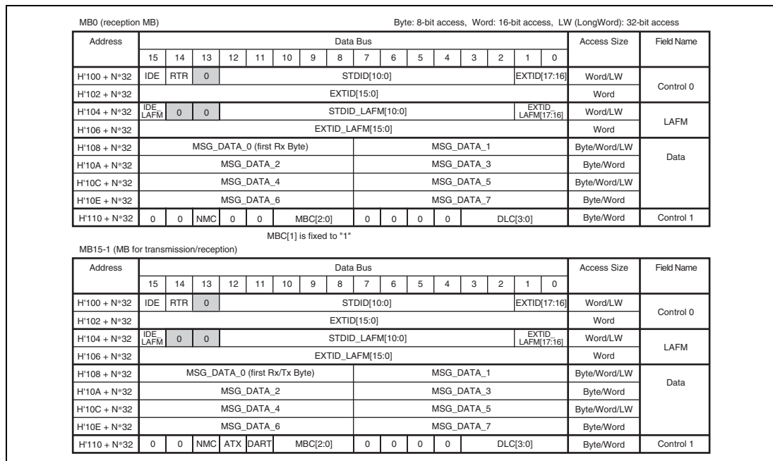
Figure 20.3 Mailbox-N Structure
