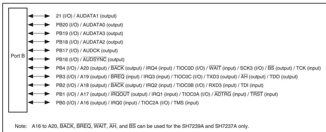
Figure 22.2 Port B
