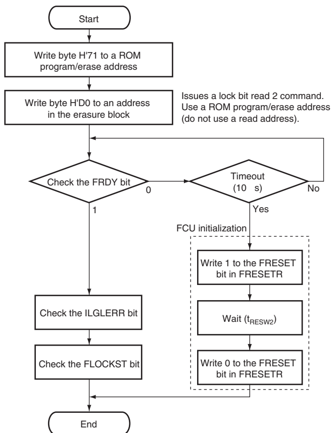
Figure 23.27 Procedure for Reading Lock Bit in Register Read Mode
