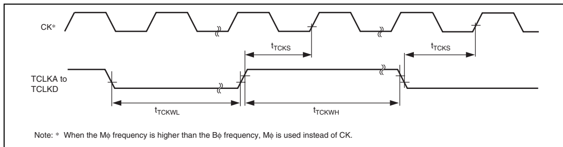
Figure 29.19 MTU2 and MTU2S Clock Input Timing
