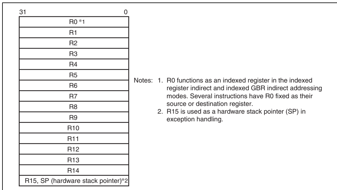
Figure 2.2 General Registers
